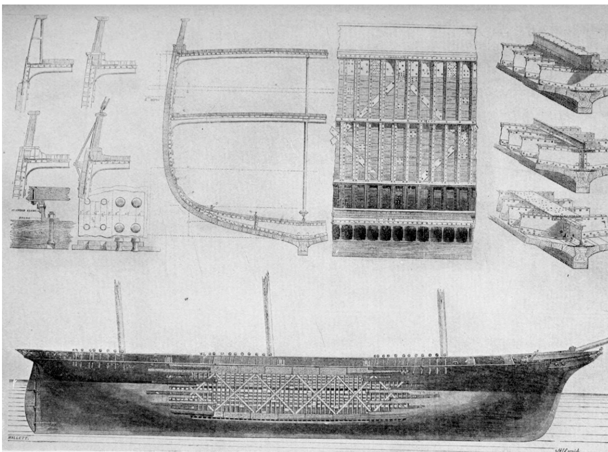
The Composite Construction
