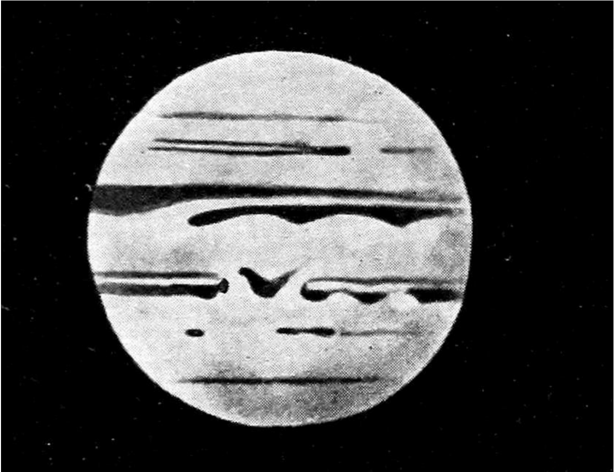
Drawing of Jupiter
