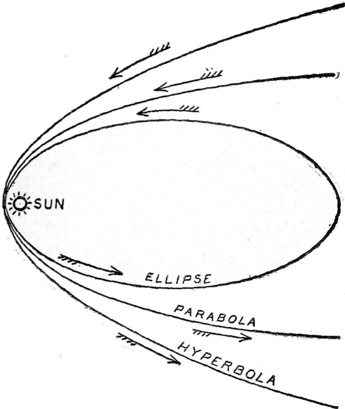
Fig. 17. Ellipse, Parabola, and Hyperbola.
