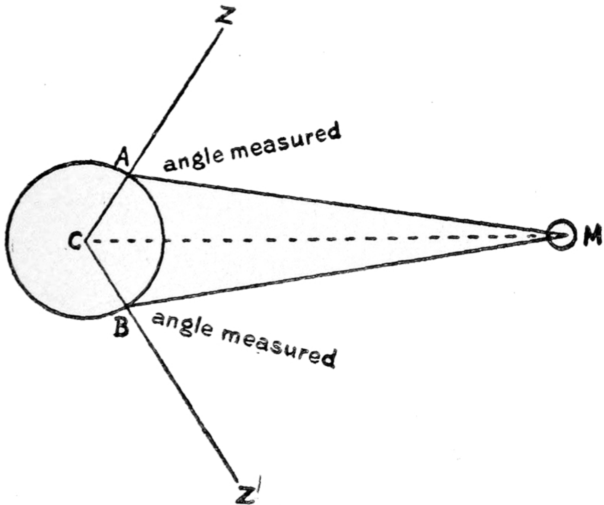
Fig. 12. Parallax of the Moon.
