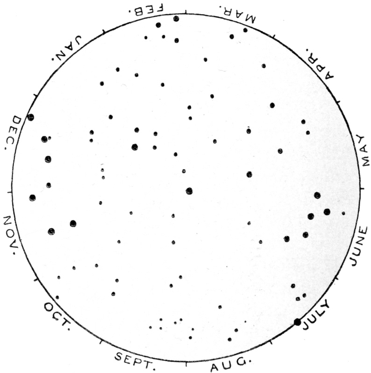
Fig. 18. The North Circumpolar Stars.
