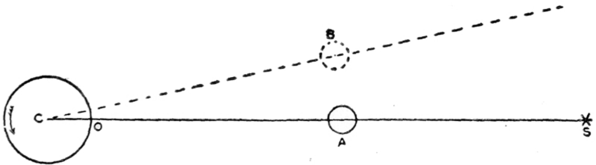
Fig. 9. Sidereal and Solar Time.
