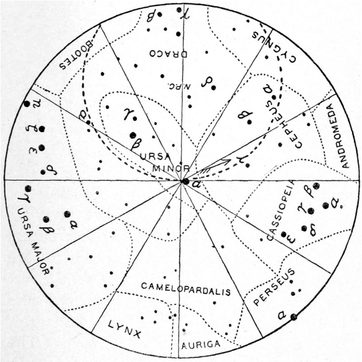
Fig. 19. Key to North Circumpolar Stars.
