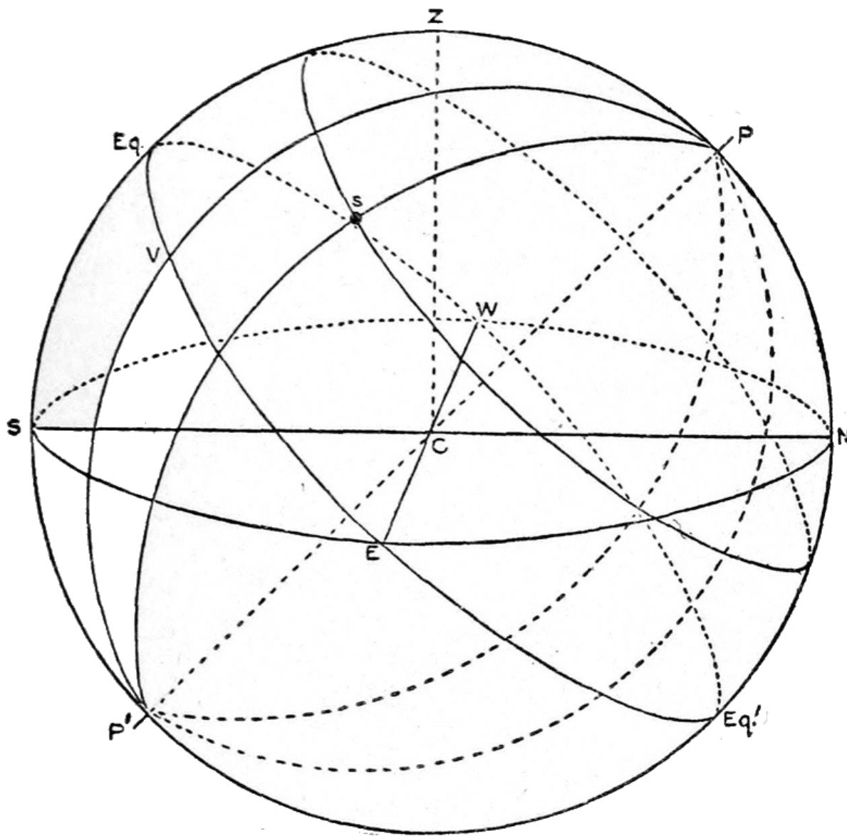
Fig. 3. Right Ascension and Declination.
