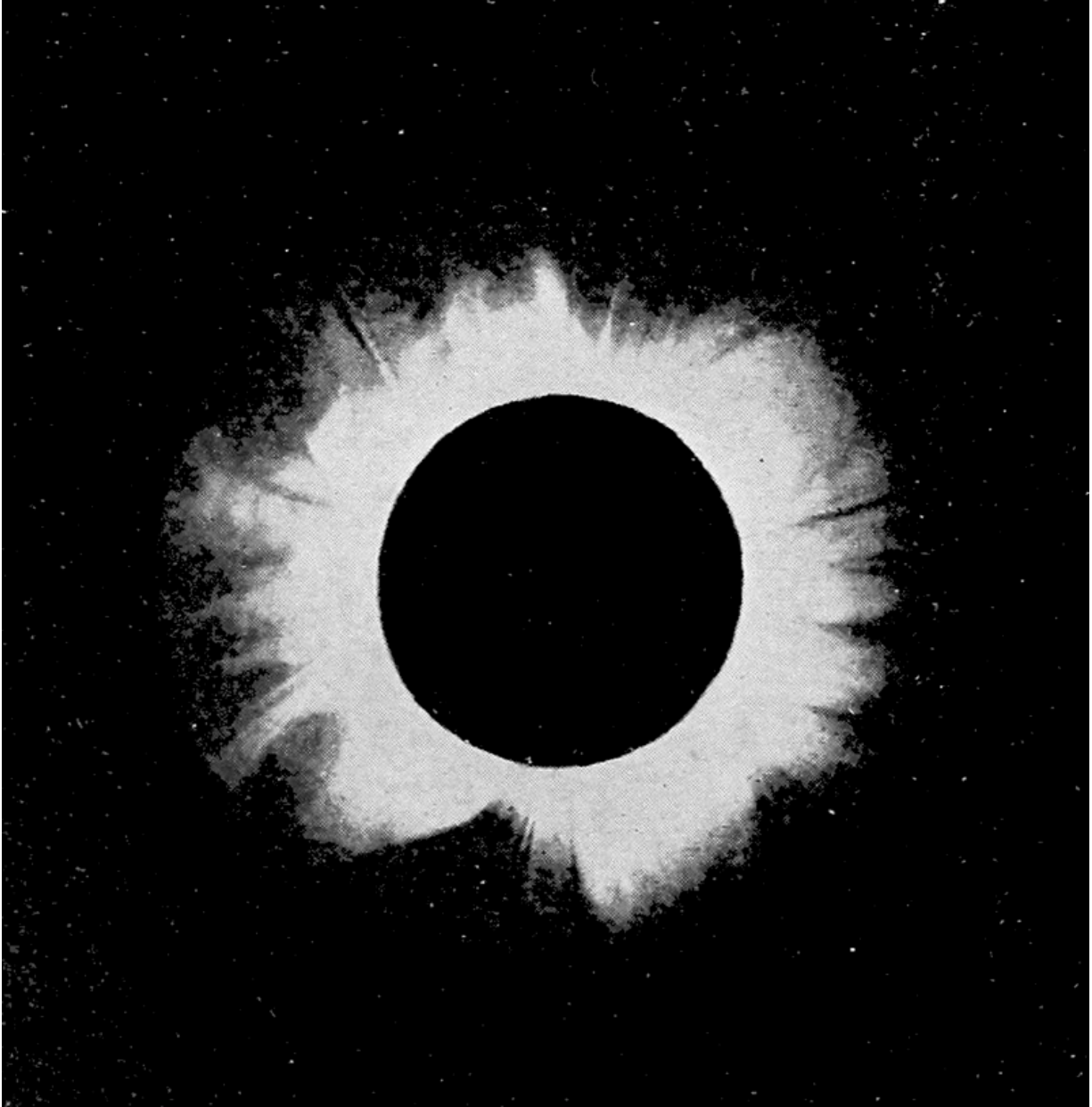
The Solar Corona at the Eclipse of 1871 From drawings.
