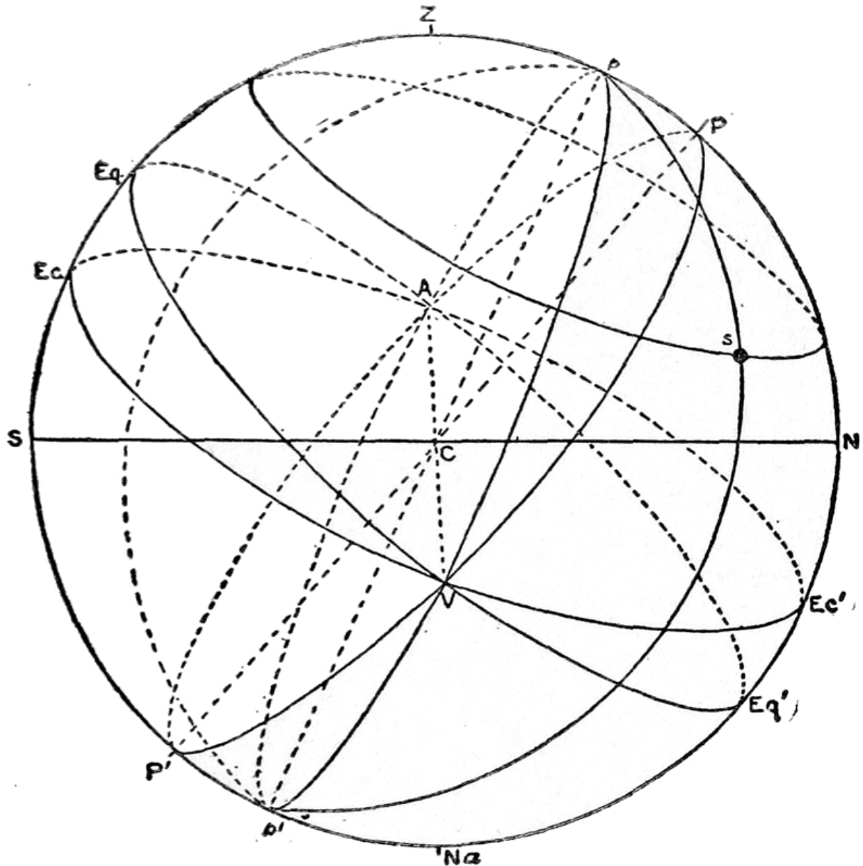
Fig. 4. The Ecliptic and Celestial Latitude and Longitude.
