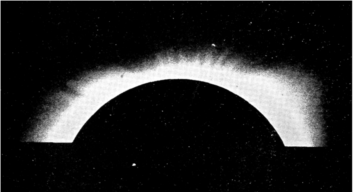
Polar Streamers of the Sun, Eclipse of 1889
