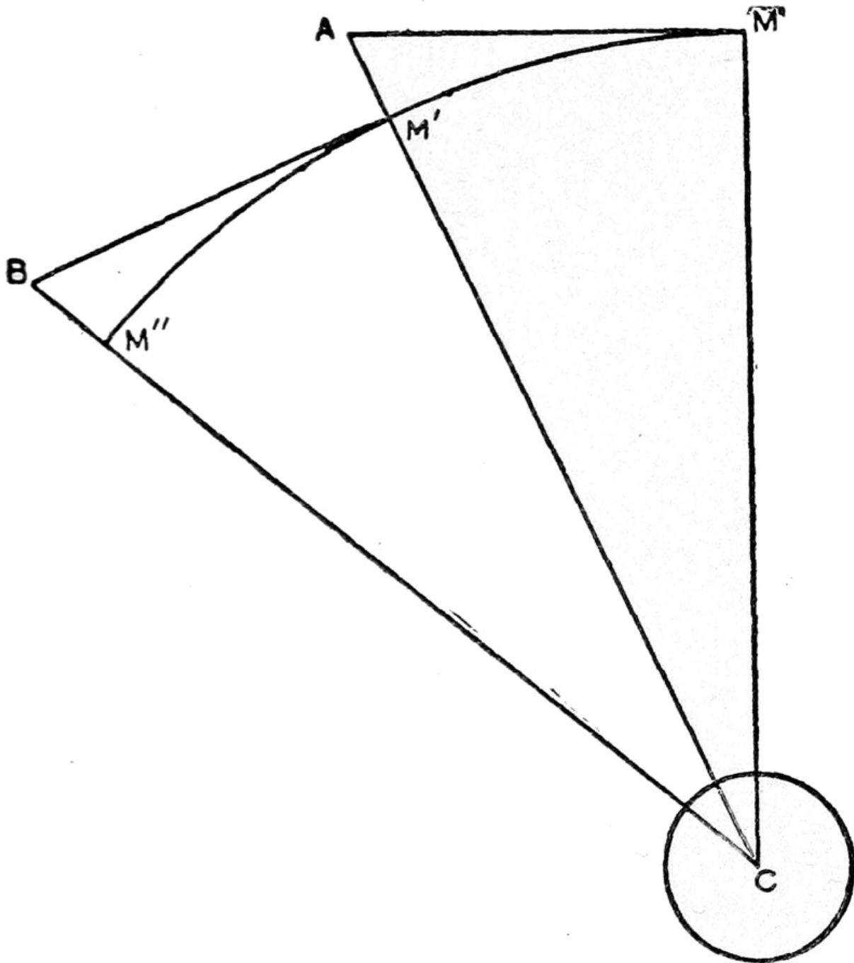
Fig. 5. How the Earth Controls the Moon.
