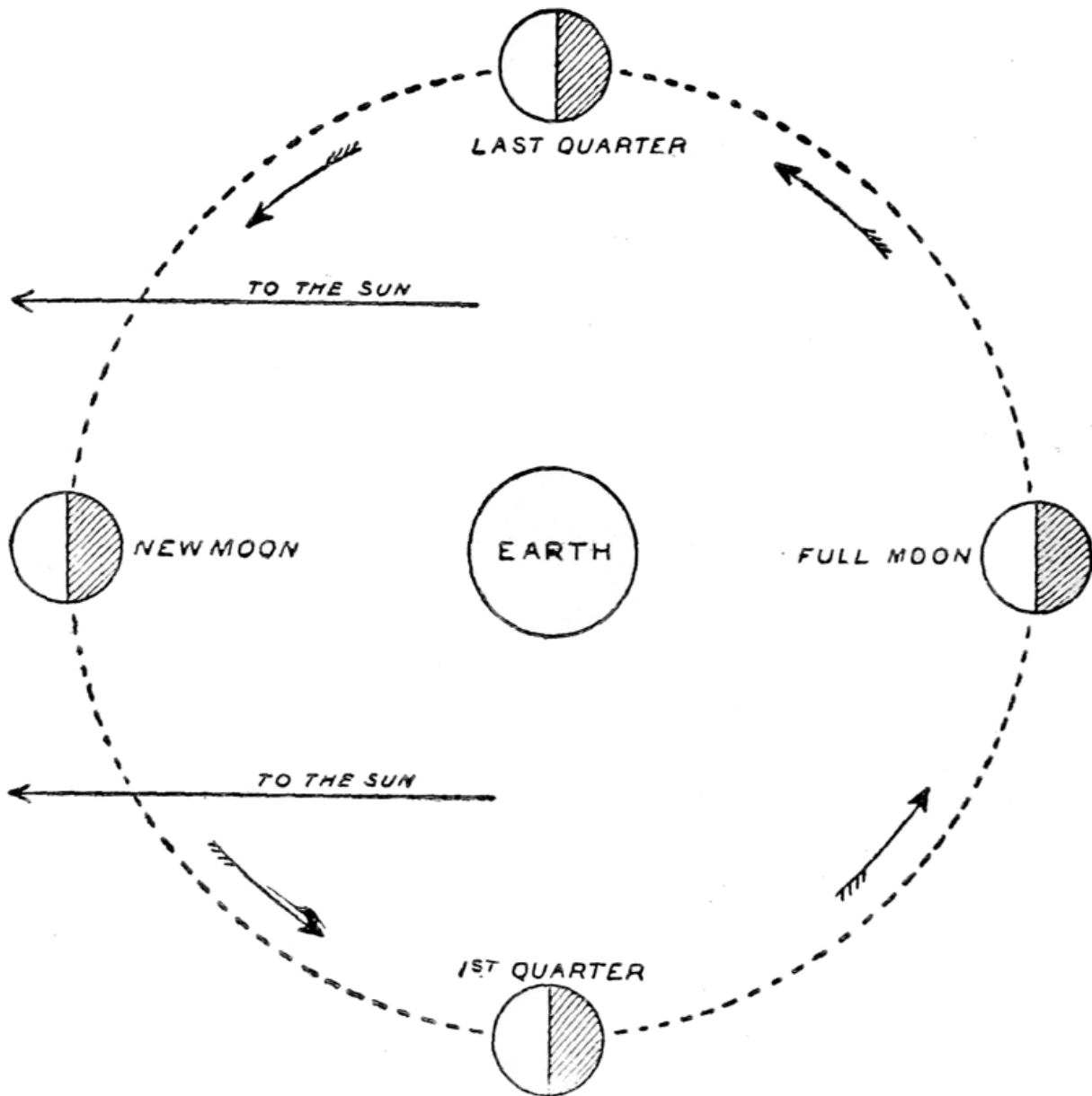
Fig. 15. The Phases of the Moon.
