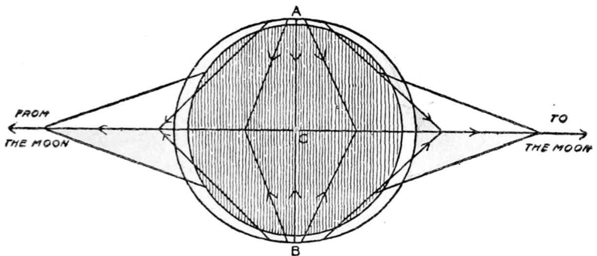
Fig. 6. The Tidal Force of the Moon.
