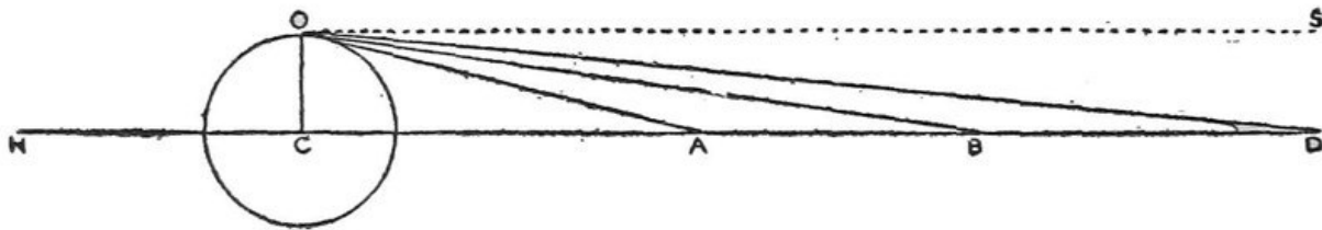
Fig. 1. The Rational and the Sensible Horizon.
