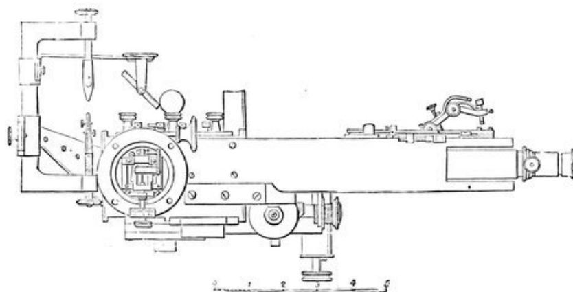
FIG. 197.—Cambridge Star Spectroscope Elevation.
