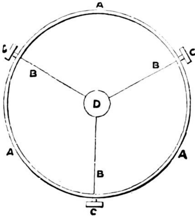
FIG. 77.—Support of diagonal plane mirror (Front view).
