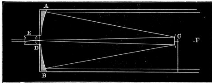
FIG. 56.—Reflecting Telescope (Cassegrain).
