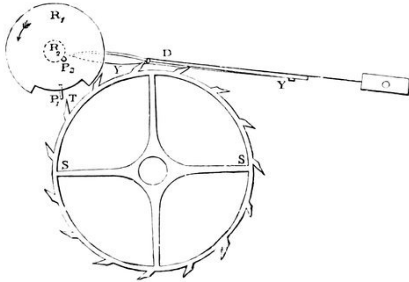
FIG. 99.—Chronometer Escapement.
