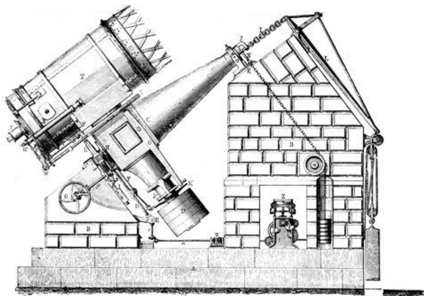
FIG. 144.—The mounting of the Melbourne Telescope. C, polar axis (cube 1 yard square, cone 8 feet long); D, Clock sector; U, Counterpoise weights ( 2\frac{1}{4} tons).
