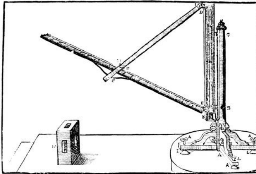
FIG. 14.—Instrument for Measuring Altitudes.
