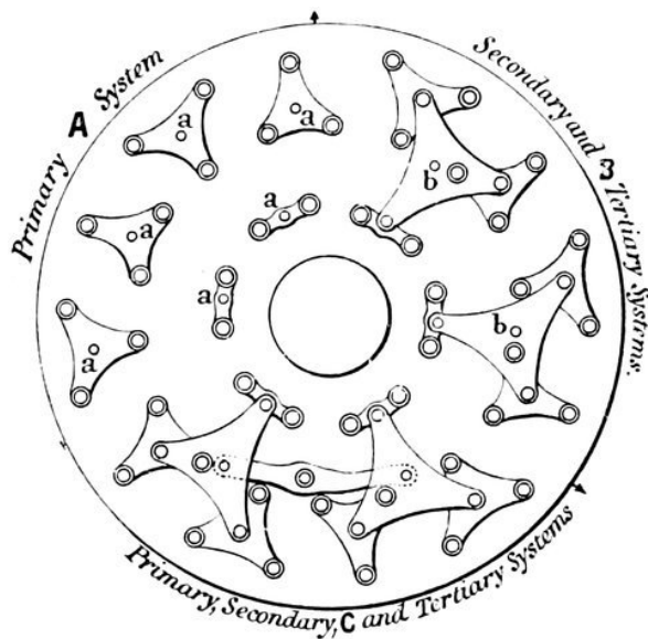
FIG. 75.—Primary, secondary, and tertiary systems of levers shown separately.
