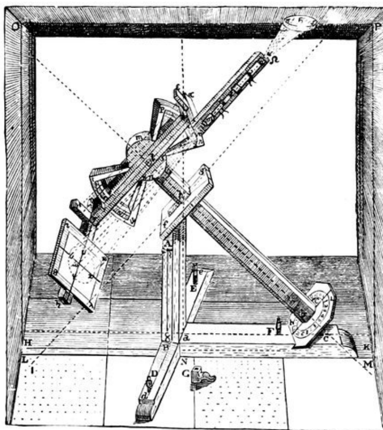
FIG. 40.—Scheiner's Telescope.
