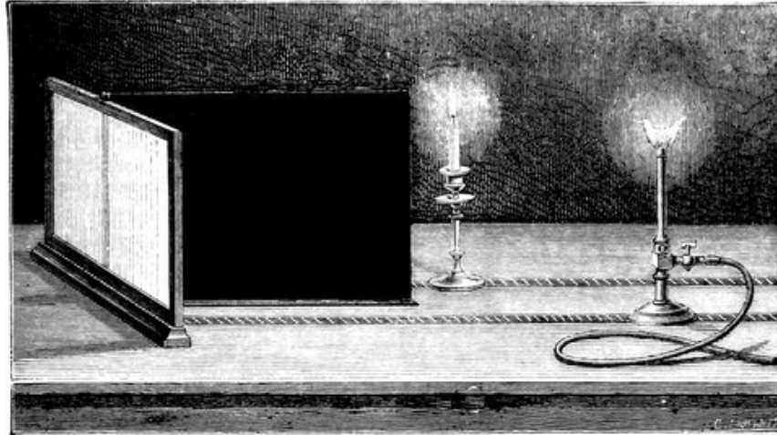
FIG. 166.—Bouguer's Photometer.
