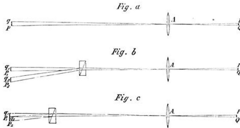
FIG. 111.—Double Image Micrometer. FIG. a , p\ q , single image formed by object-glass. FIG. b , p_1\ q_1, p_2\ q_2 , images separated by the double refracting prism. FIG. c , same, separated less, by the motion of the prism.
