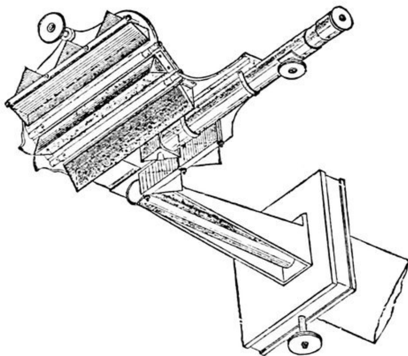
FIG. 194.—Solar Spectroscope (Grubb's form).
