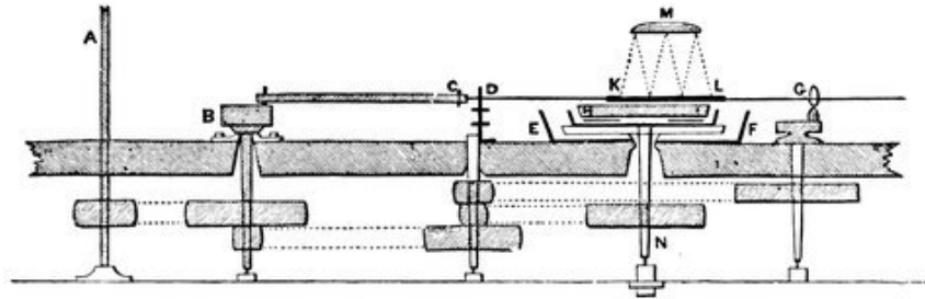
FIG. 65*.—Section of Lord Rosse's polishing machine.
