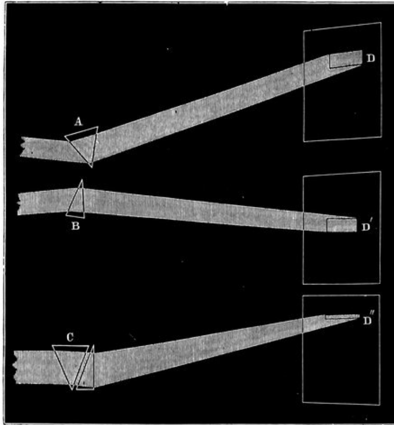
FIG. 44.—Diagram Explaining the Formation of an Achromatic Lens. A, crown-glass prism; B, flint-glass prism of less angle, but giving the same amount of colour; C, the two prisms combined, giving a colourless yet deviated band of light at D''.
