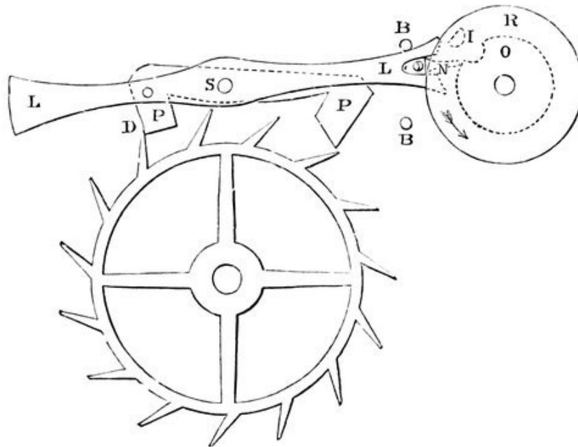
FIG. 98.—Detached Lever Escapement.
