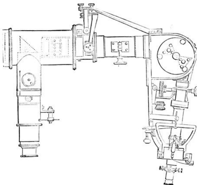
FIG. 198.—Cambridge Spectroscope Plan.
