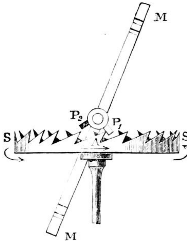
FIG. 86.—The Crown Wheel.
