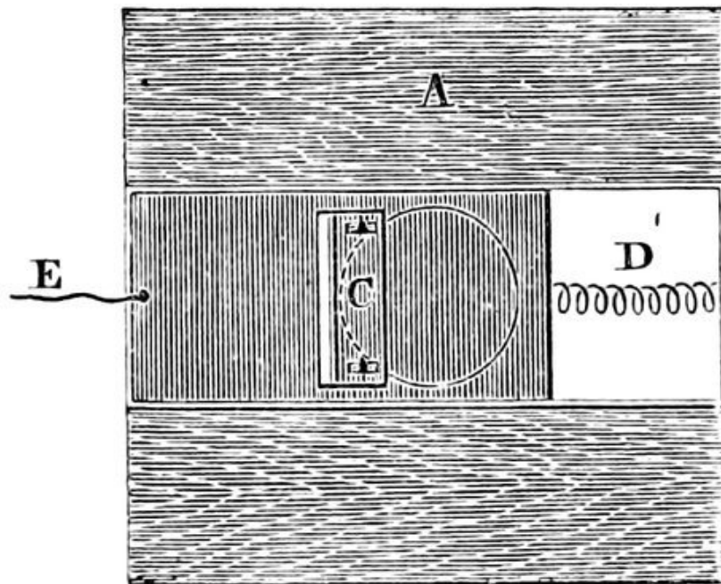
FIG. 210.—Instantaneous Shutter.
