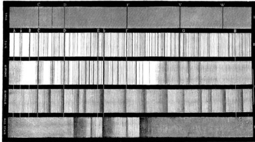
FIG. 200.—Types of Stellar Spectra (Secchi).
