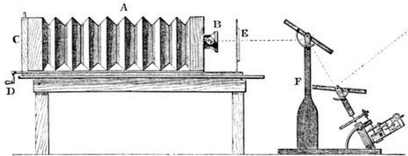
FIG. 209.—Enlarging Camera. F, heliostat for throwing beam of sunlight on the reflector, which throws it into the camera; E, negative; B, focussing-lens; C, plate- or paper-holder; D, focussing-screw.
