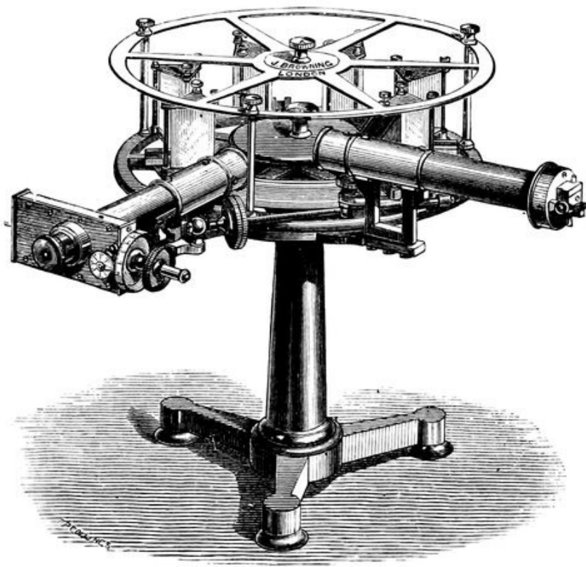
FIG. 177.—Spectroscope with returning Beam.
