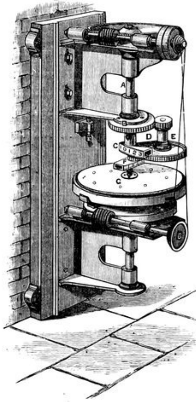
FIG. 66.—Mr. Lassell's polishing machine.
