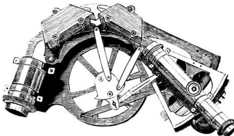
FIG. 174.—Automatic Spectroscope (Grubb's form).
