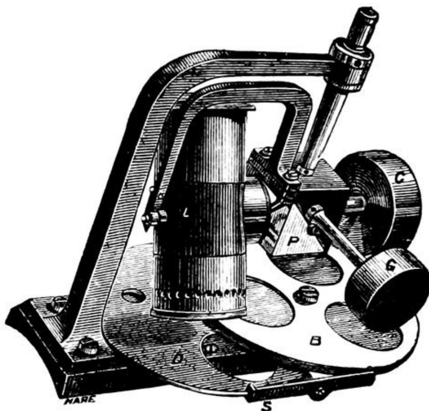
FIG. 150.—Cooke's illuminating lamp.
