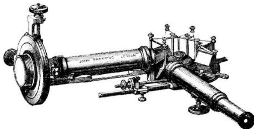
FIG. 193.—Solar Spectroscope (Browning's form).
