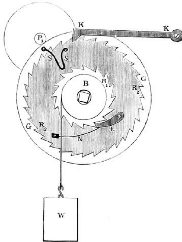
FIG. 88.—Winding Arrangements.
