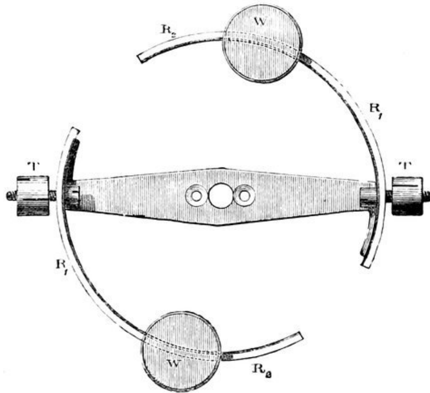
FIG. 97.—Compensating Balance.
