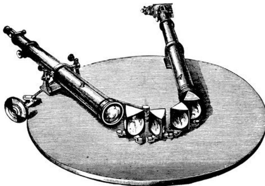
FIG. 173.—Spectroscope with Four Prisms.
