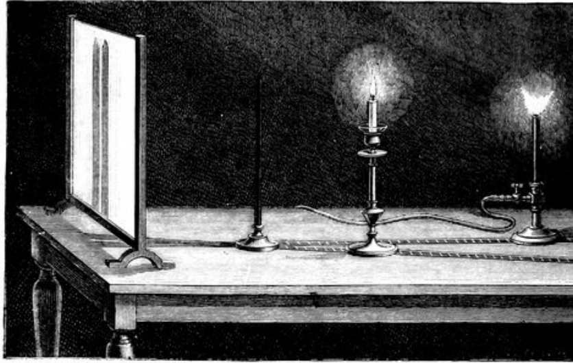
FIG. 165.—Rumford's Photometer.
