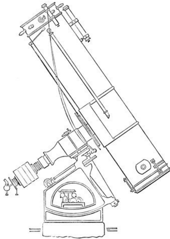
FIG. 140.—Grubb's form for Newtonians.
