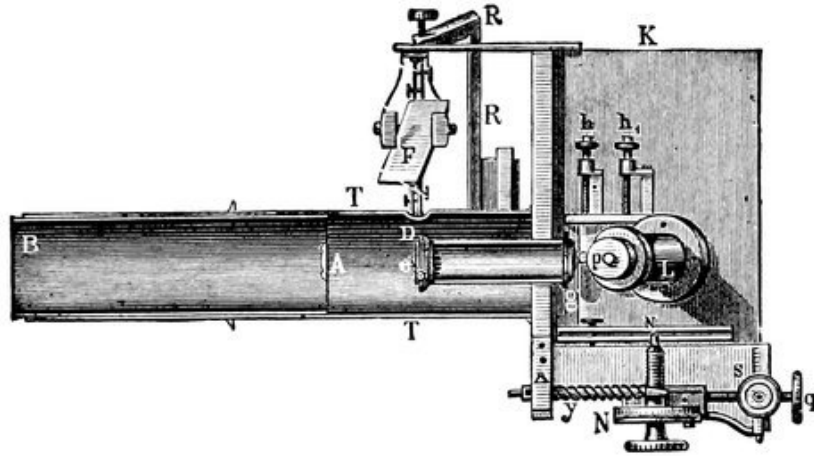
FIG. 195.—Side view of Spectroscope, showing the arrangement by which the light from a spark is thrown into the instrument by means of the reflecting prism, e , by a mirror F . (Huggins.)
