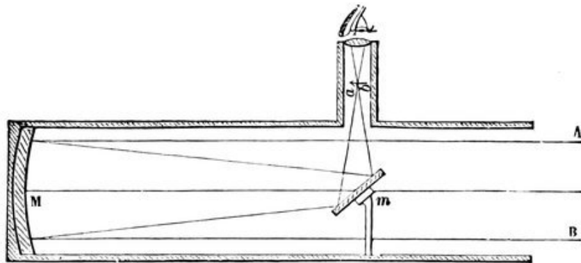
FIG. 55.—Newton's Telescope.
