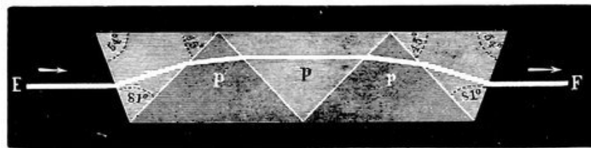
FIG. 178.—Direct Vision Prism.
