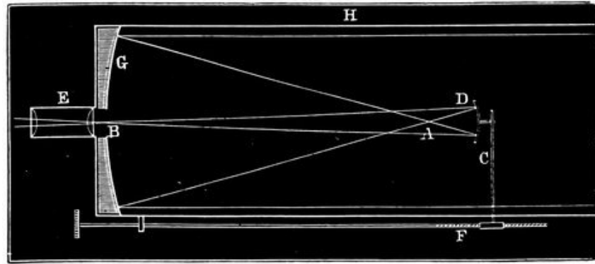
FIG. 54.—Reflecting Telescope (Gregorian).
