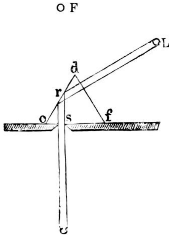
FIG. 188.—Comparison Prism, showing the path of the Ray.
