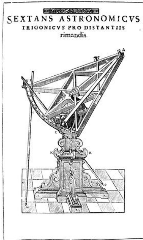
FIG. 19.—Tycho's Sextant.
