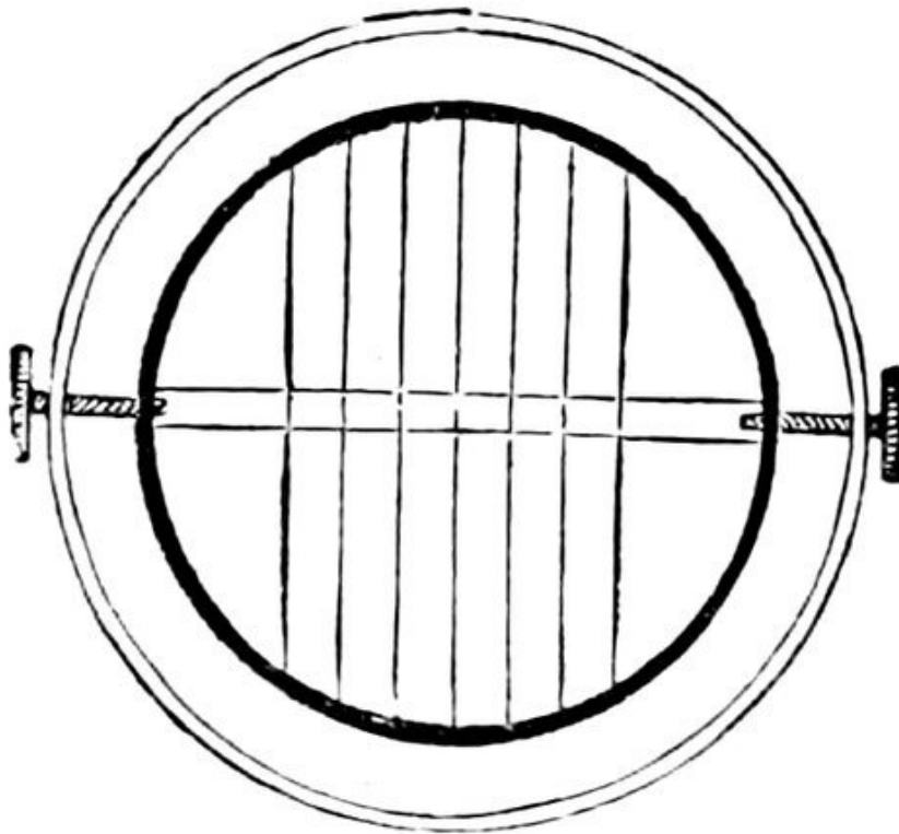
FIG. 123.—System of wires in transit eyepiece.
