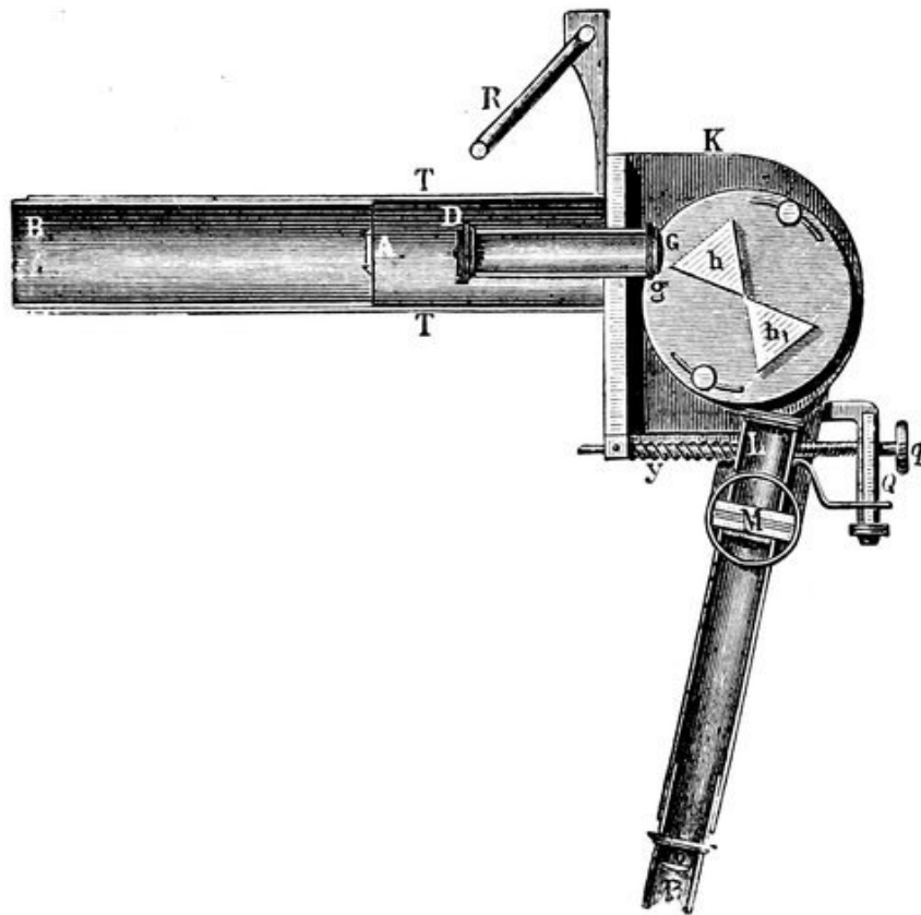
FIG. 196.—Plan of Spectroscope. T , eyepiece end of telescope, B interior tube, carrying A , cylindrical
