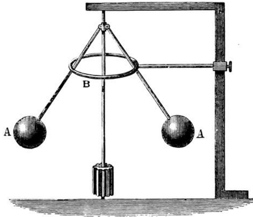
FIG. 146.—Clock Governor.
