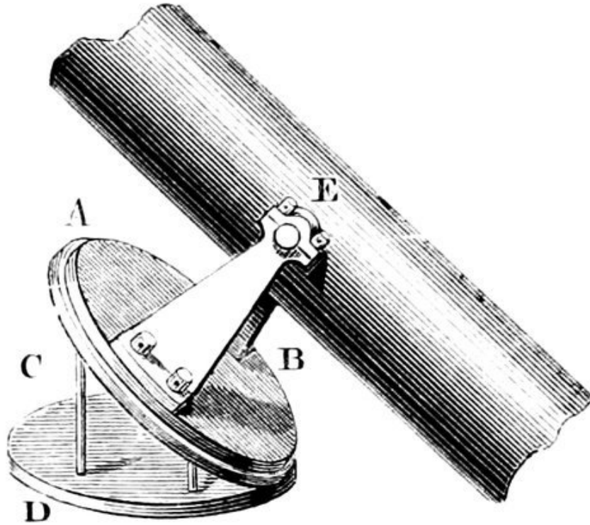
FIG. 137.—Simple Equatorial Mounting.
