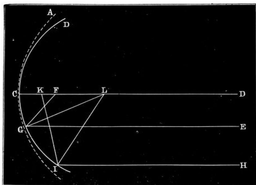
FIG. 58.—Diagram Illustrating Spherical Aberration.
