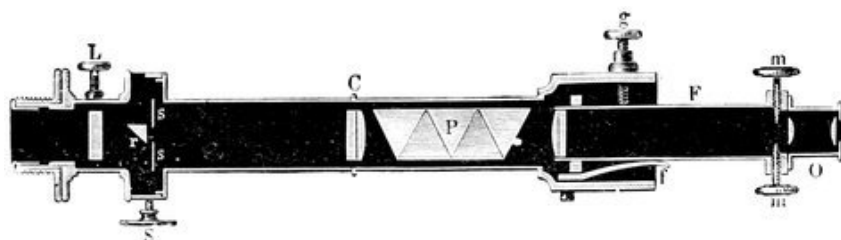
FIG. 199.—Direct-vision Star Spectroscope. (Secchi.)
