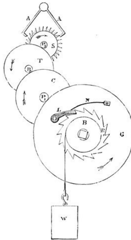
FIG. 87.—The Clock Train.
