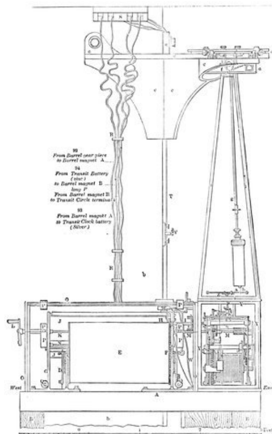
FIG. 124.—The Greenwich chronograph. General view.
