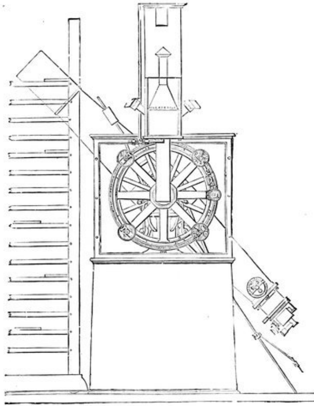
FIG. 120.—Cambridge (U.S.) meridian circle.
