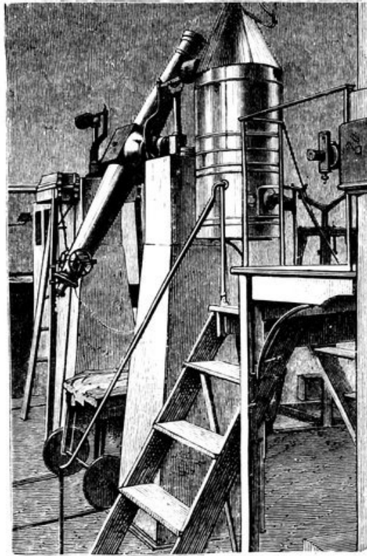
FIG. 114.—Transit Instalment in a fixed Observatory.
