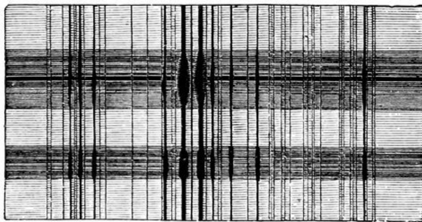
FIG. 185.—Spectrum of Sun-Spot.
