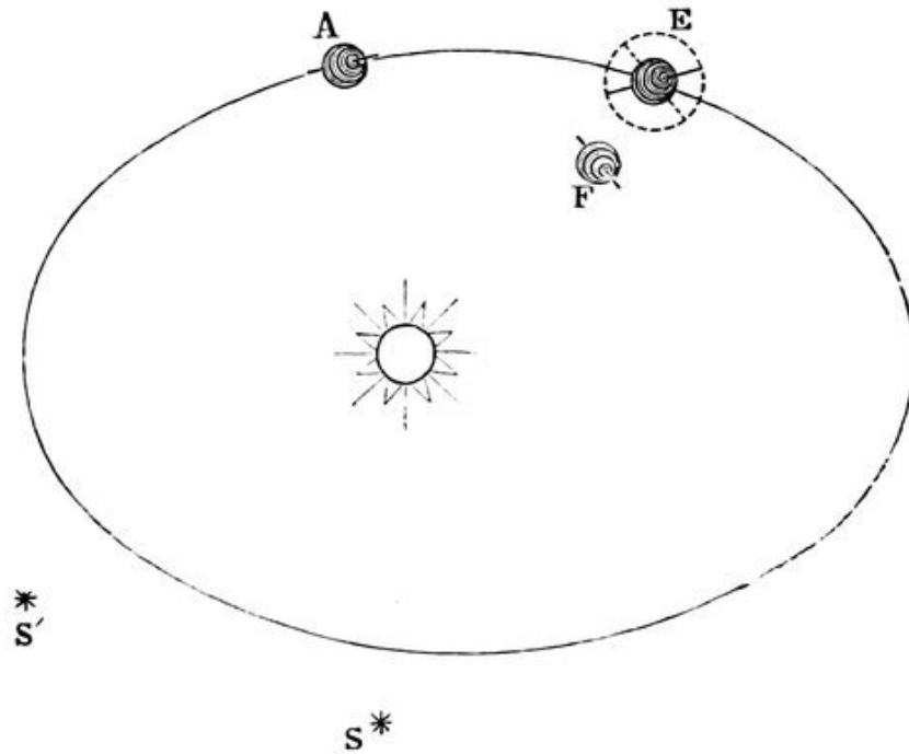
FIG. 10.—Diagram Illustrating the Precession of the Equinoxes.
