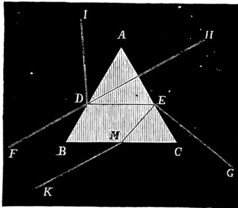
FIG. 167.—Kepler's Diagram.
