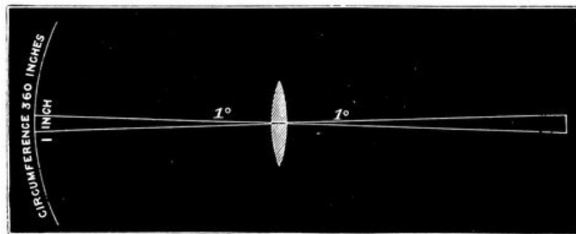
FIG. 39.—Diagram Explaining the Magnifying Power of Object-glass.
