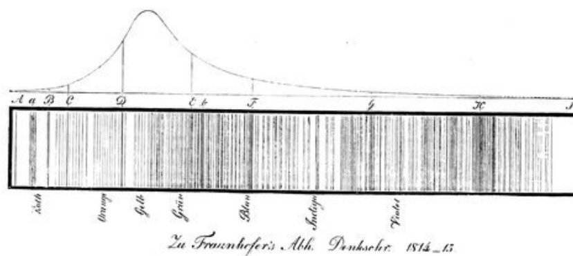
FIG. 170.—Copy of Fraunhofer's first Map of the Lines in the Solar Spectrum.
