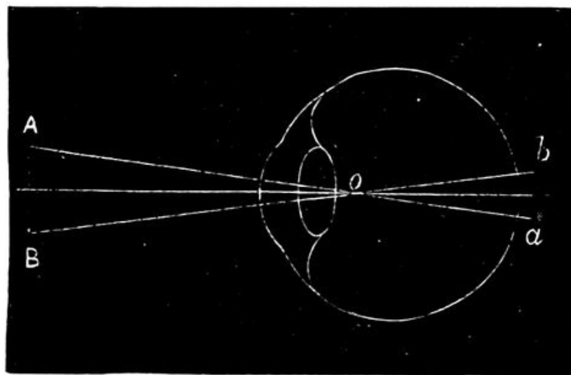
FIG. 34.—Action of a Long-sighted Eye.
