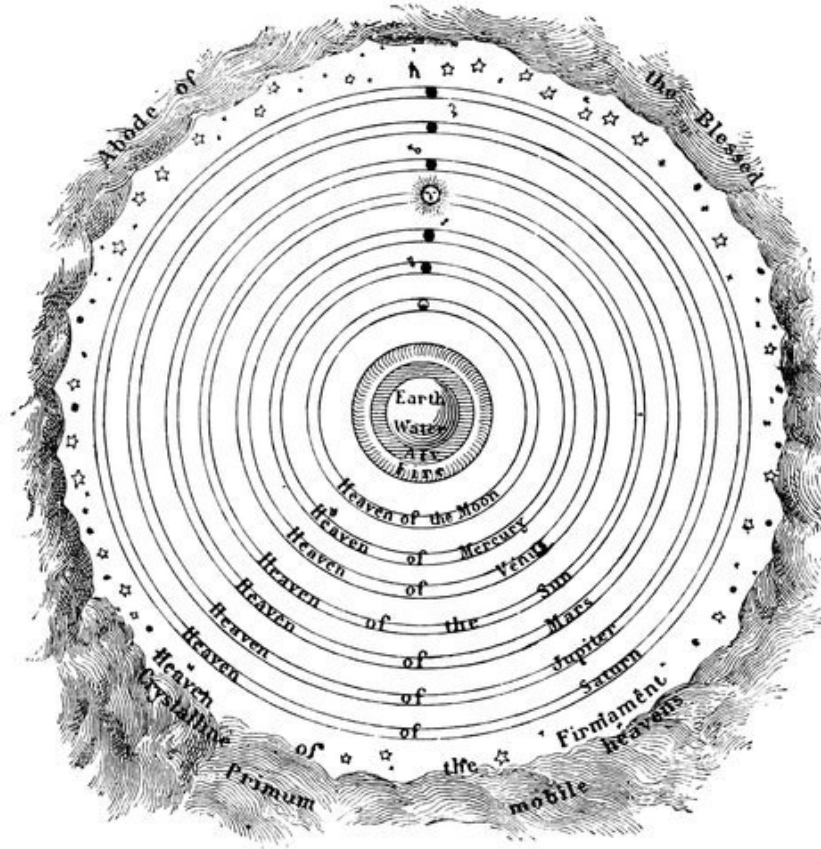
FIG. 1.—The Heavens according to Ptolemy.
