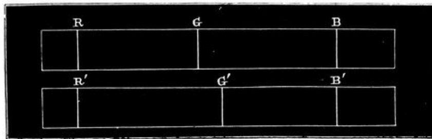
FIG. 46.—Diagram Illustrating the Irrationality of the Spectrum.
