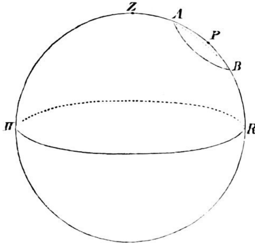
FIG. 121.—Diagram illustrating how the pole is found.
