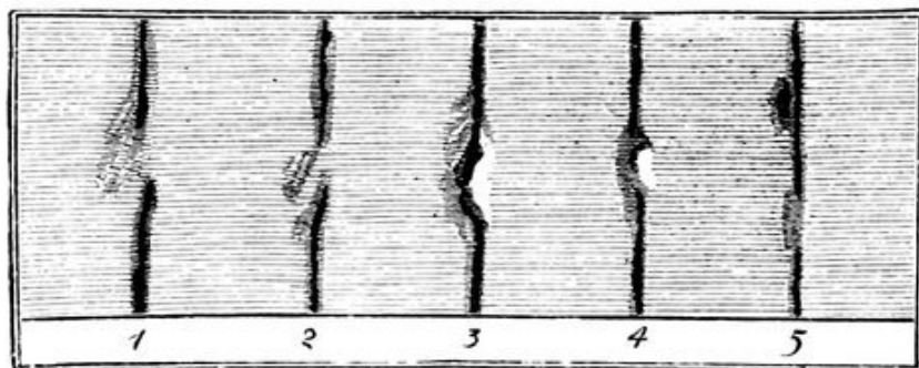
FIG. 202.—Distortions of F line on Sun.
