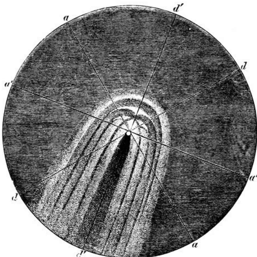
FIG. 161.—Measurement of the Angle of Position of the Axis of Figure of a Comet, a a , positions of fixed wire when the north vernier is at zero; d d position of movable wire under like conditions; a' a' , d' d' , positions of these wires which enable the angle of position of the comet's axis to be measured. The angle a a' or d d' is the angle required.
