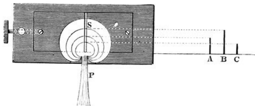
FIG. 186.—Diagram explaining Long and Short Lines.
