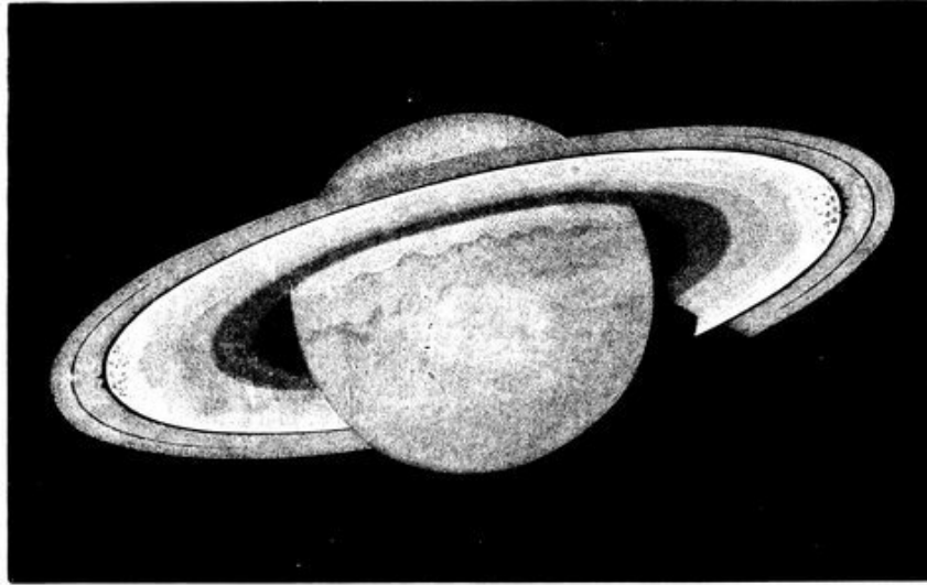
FIG. 84.—Details of the ring of Saturn observed by Trouvelot with the 26-inch Washington Refractor.
