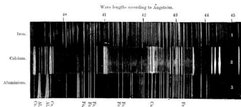
FIG. 181.—Comparison of the line spectra of Iron, Calcium, and Aluminium, with Common Impurities. Copy of a photograph, in which by dividing the slit of the spectroscope into sections, and admitting light from the various light sources through them in succession, spectra of different elements are recorded on the same photographic plate.
