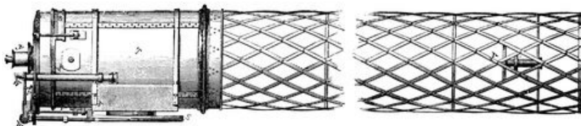
FIG. 71.—Optical part of Melbourne reflector, showing the lattice arrangement for supporting the convex mirror Y , T more solid part of tube fixed to declination axis, W finder.
