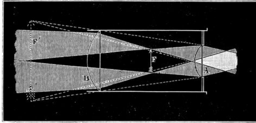
FIG. 60.—Huyghens' Eyepiece.
