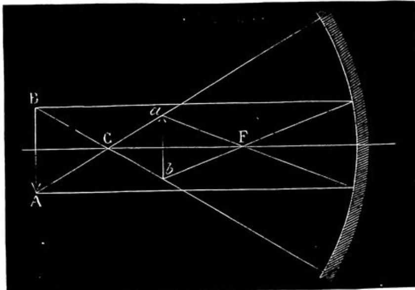
FIG. 52.—Diagram explaining Fig. 51 .
