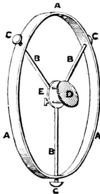
FIG. 78.—Support of diagonal plane mirror (Side view).
