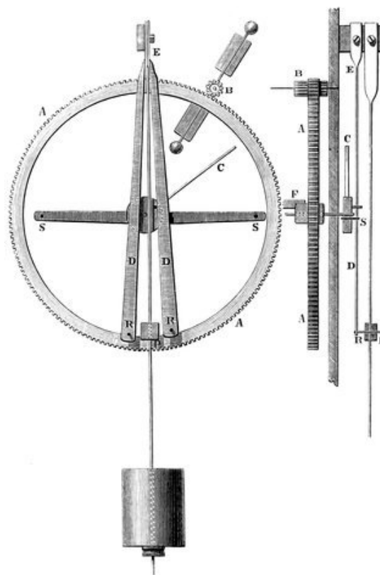
FIG. 146.—Clock Governor.
