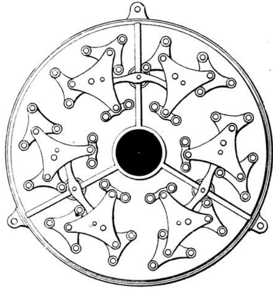
FIG. 76.—Complete system consolidated into three screws.
