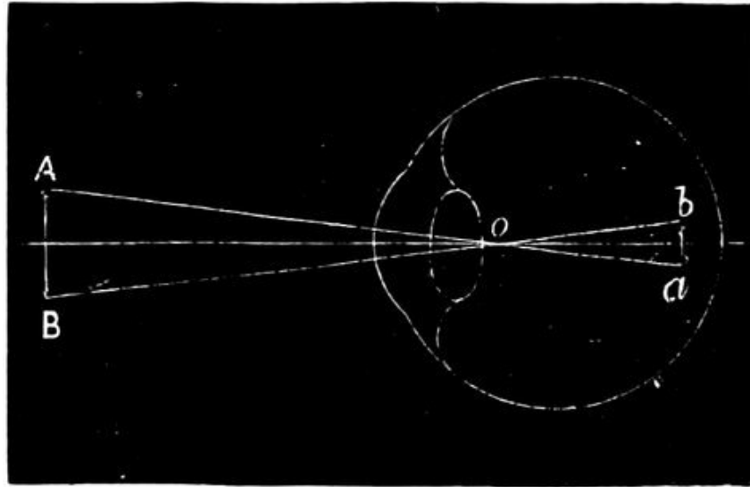
FIG. 36.—Action of Short-sighted Eye.
