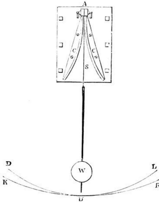
FIG. 89.—The Cycloidal Pendulum.
