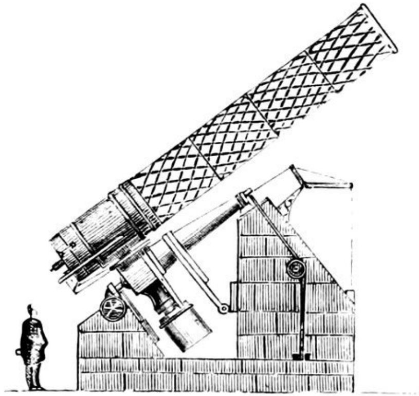
FIG. 143.—General view of the Melbourne Reflector.
