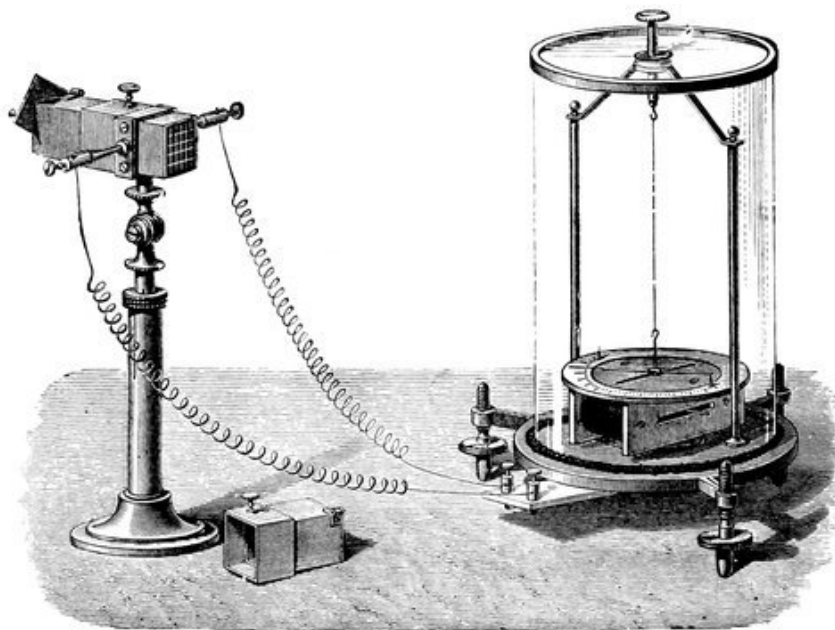
FIG. 164.—Thermopile and Galvanometer.
