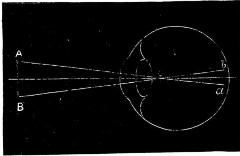
FIG. 33.—Action of Eye in Formation of Images.
