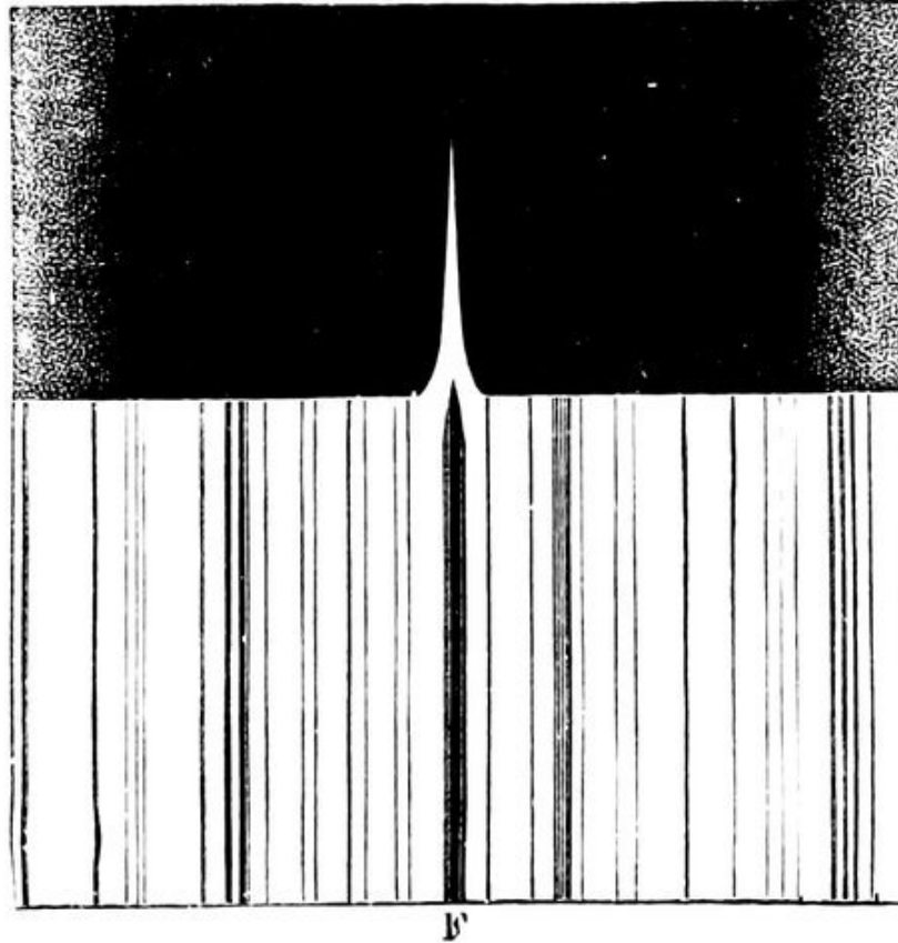
FIG. 201.—Part of Solar Spectrum near F.
