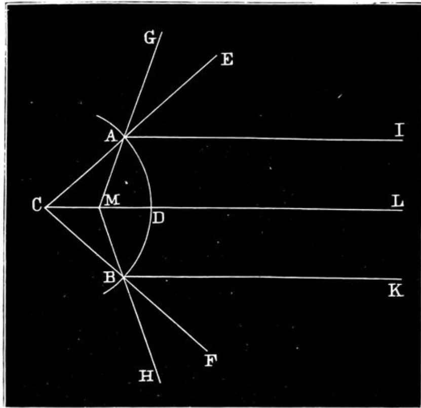
FIG. 53.—Reflection of Rays by Convex Mirror.
