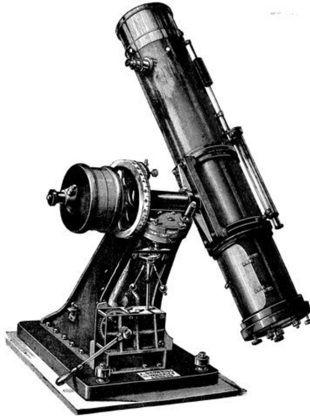
FIG. 141.—Browning's mounting for Newtonians.
