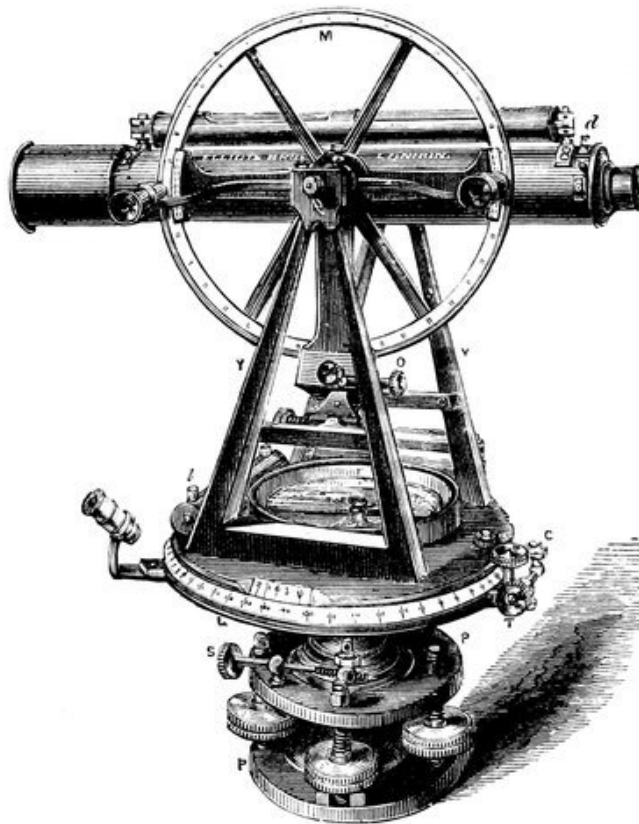
FIG. 132.—Theodolite.
