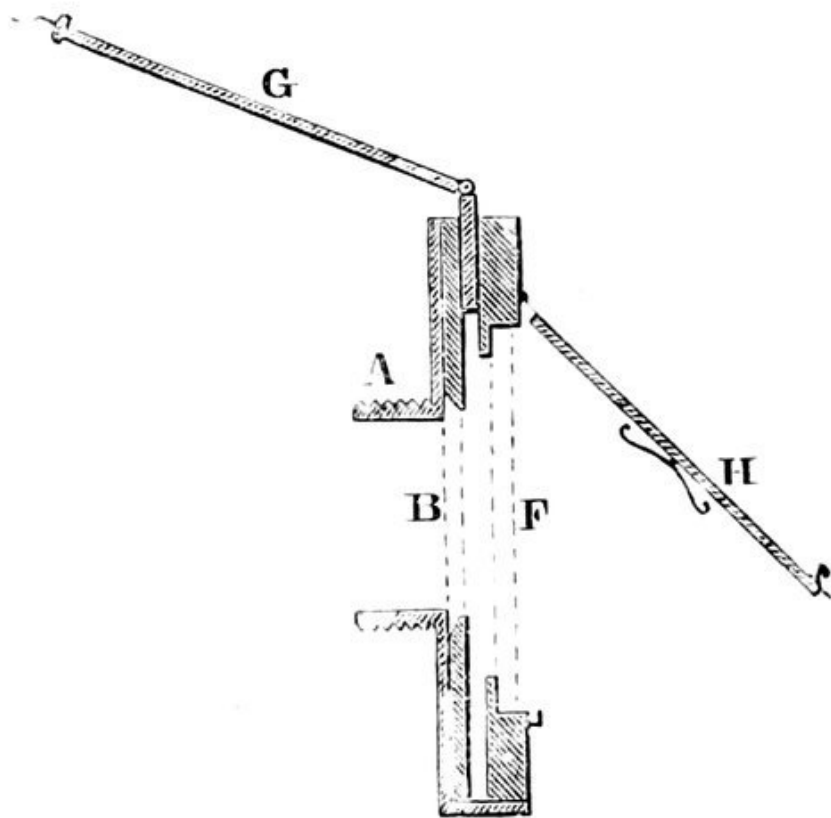
FIG. 208.—Section of Plate-holder.
