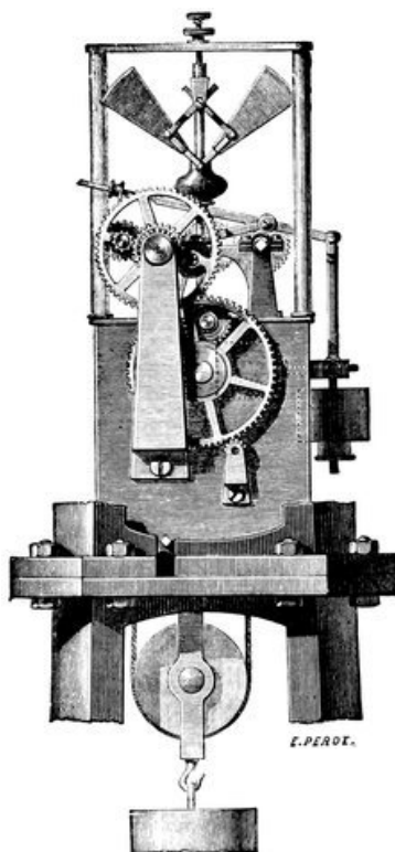
FIG. 148.—Foucault's governor.
