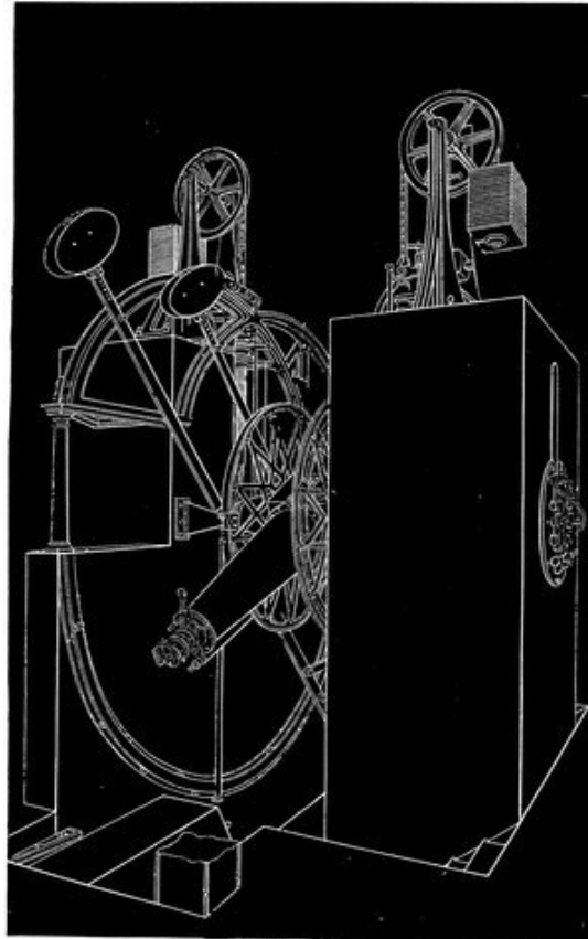
FIG. 118.—Perspective view of Greenwich Transit Circle.
