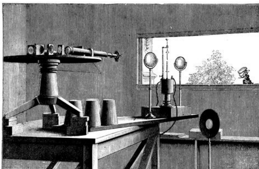
FIG. 216.—Arrangement for Photographically Determining the Coincidence of Solar and Metallic Lines.
