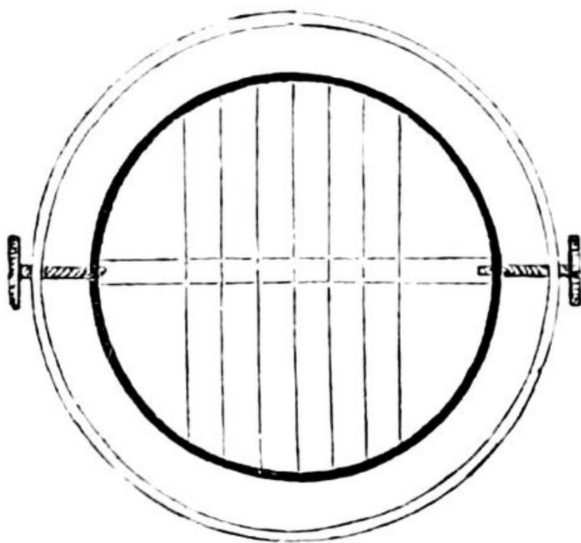
FIG. 103.—System of Wires in a Transit Eyepiece.
