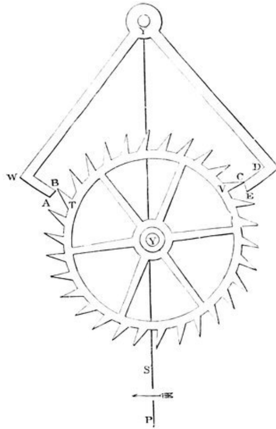
FIG. 93.—Graham's Dead Beat.
