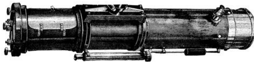
FIG. 70.—Optical part of a Newtonian reflector of ten inches aperture, showing eyepiece, adjusting screws for large speculum, finder, door for uncovering speculum, and counterpoise.
