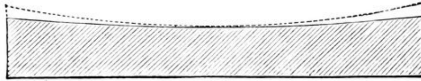
FIG. 65.—Showing in an exaggerated form how the edge of the speculum is worn down by polishing.
