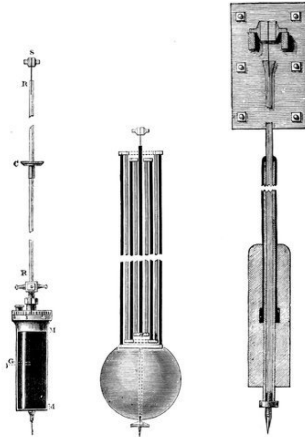
FIG. 90.—Graham's, Harrison's, and Greenwich Pendulums.
