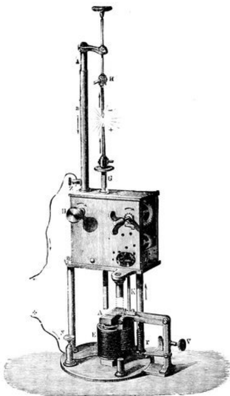
FIG. 179.—Electric Lamp. y, z, wires connecting battery of 50 Grove or Bunsen elements; G, H, carbon holders; K, rod, which stops a clockwork movement, which when going makes the poles approach until the current passes; A, armature of a magnet which by means of K frees the clockwork when not in contact; E, electro-magnet
