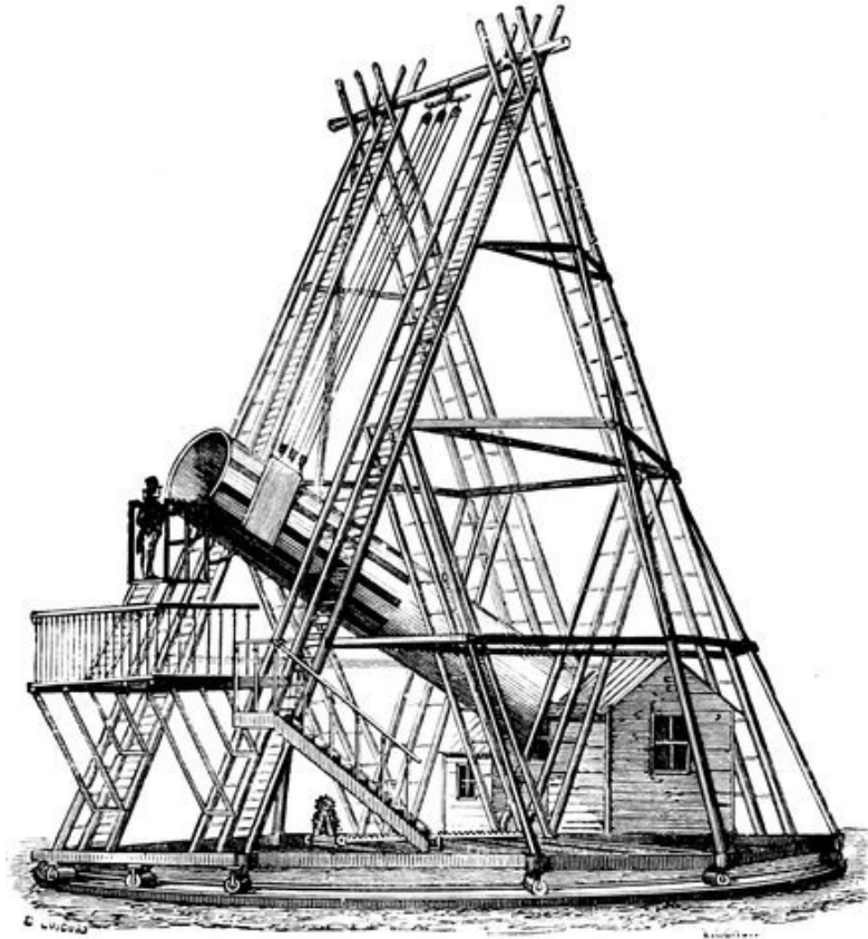
FIG. 134.—The 40-feet at Slough.
