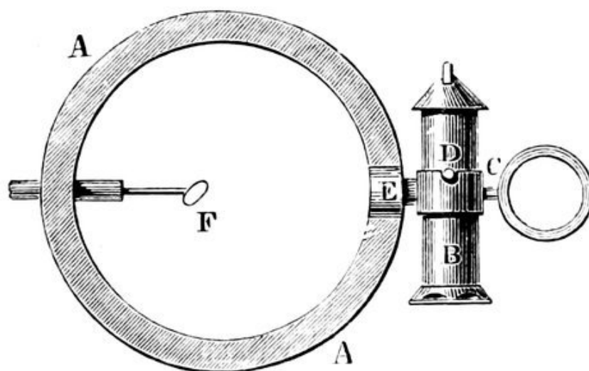
FIG. 149.—Illuminating lamp for equatorial.
