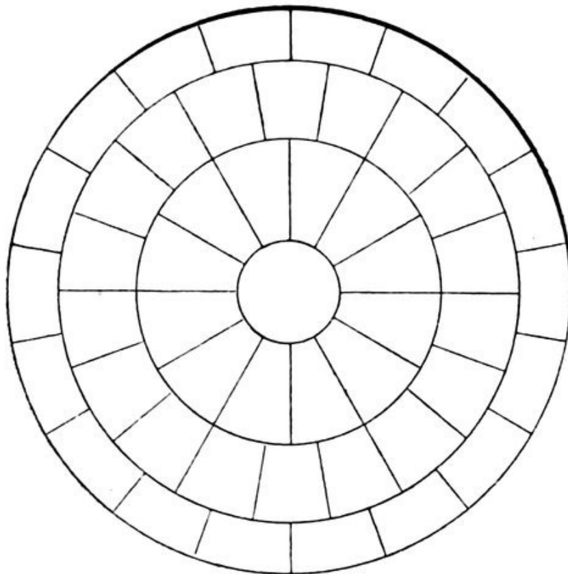
FIG. 74.—Division of the speculum into equal areas.
