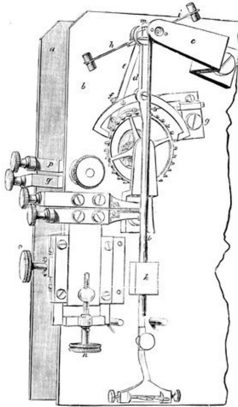
FIG. 96.—Greenwich Clock Escapement.
