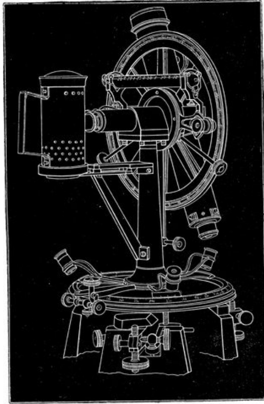
FIG. 133.—Portable Alt-azimuth.
