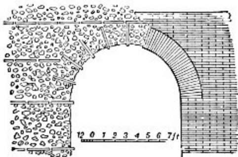
FIG. 189. CONCRETE ARCH; HALF WITH BRICK FACING REMOVED.
