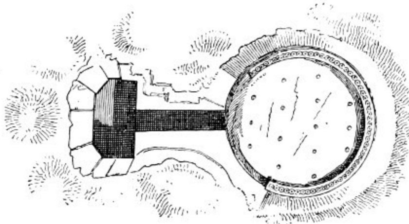
FIG. 214. PLAN OF KILN AT HEILIGENBERG.
