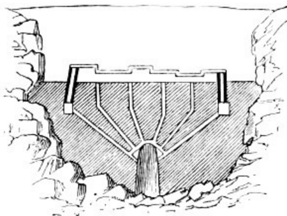
FIG. 215. SECTION OF KILN AT HEILIGENBERG.
