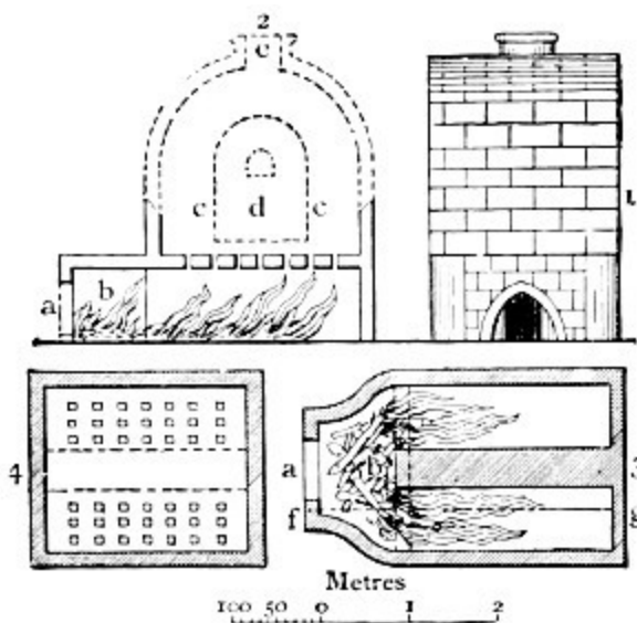
FIG. 212. ROMAN KILN FOUND AT HEDDERNHEIM, GERMANY.
