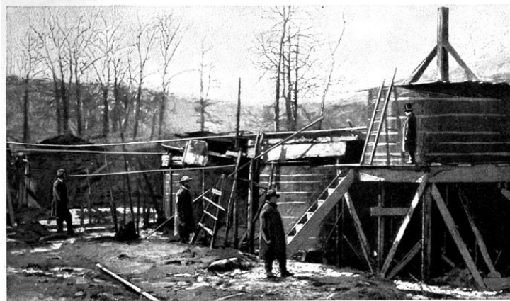
WOODEN TANKS FOR STORING OIL
