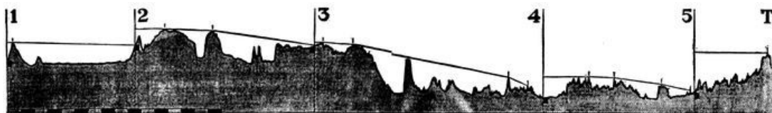
Scale—3 miles to each division. CONDENSED PROFILE OF TIDEWATER PIPE LINE BETWEEN RIXFORD AND TAMANEND, PENNSYLVANIA
