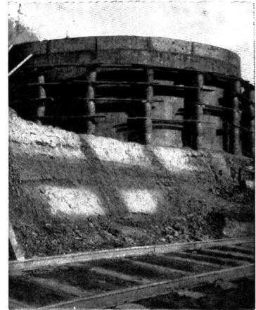
CONSTRUCTING AN IRON TANK FOR STORING OIL
