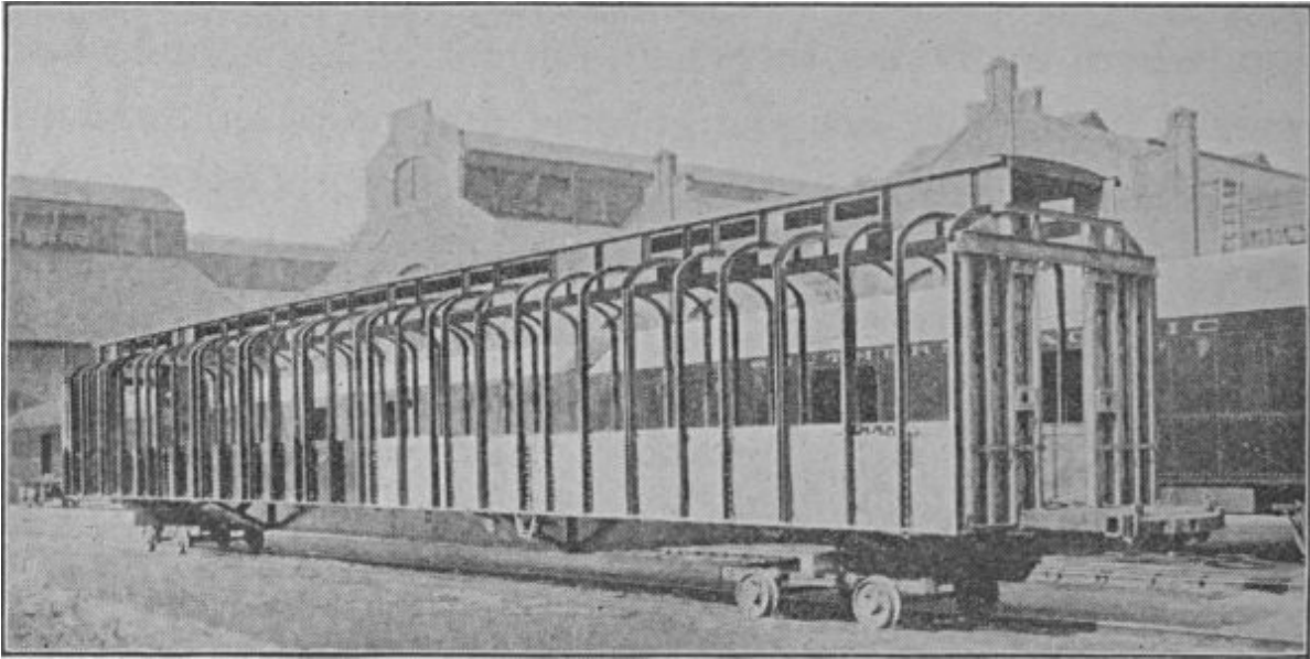
THE SKELETON OF A PULLMAN CAR
