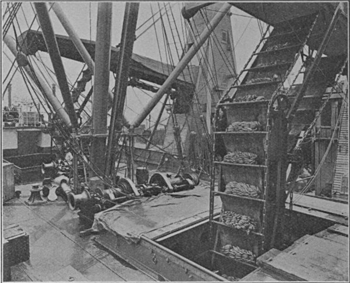
A BANANA CONVEYOR
