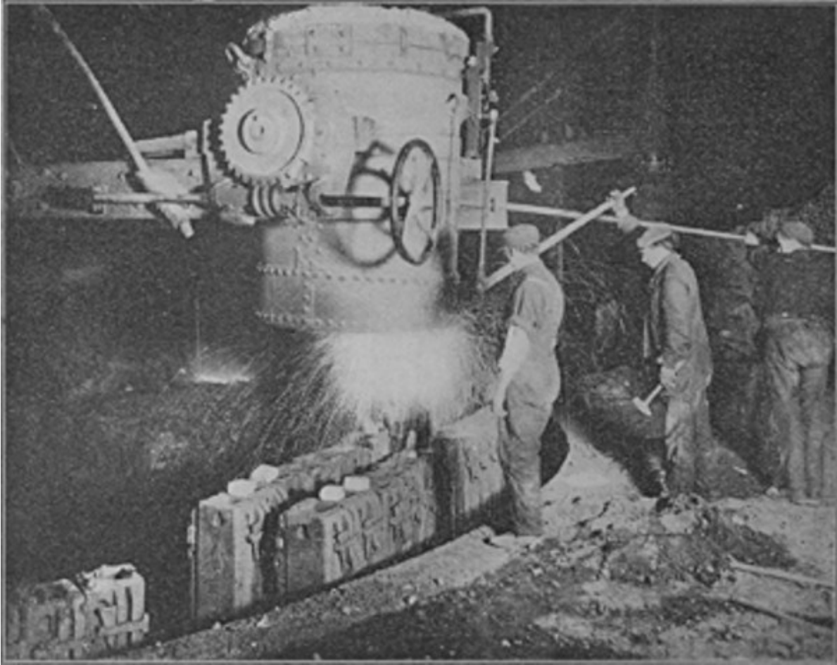
FILLING MOLDS WITH MOLTEN METAL
