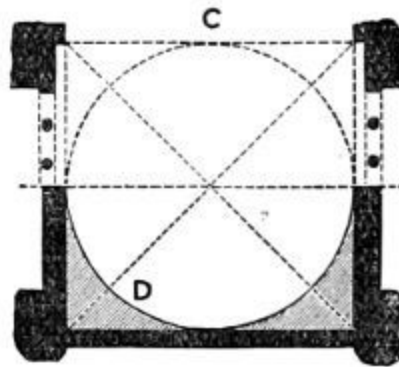
301. Diagram of Byzantine Pendentives.
