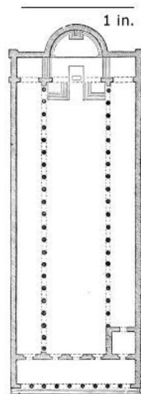
399. Plan of S. Maria Maggiore. Scale 100 ft. to 1 in.
