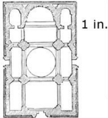
356. Plan of Cathedral at Ani. (From Texier.) Scale 100 ft. to 1 in.
