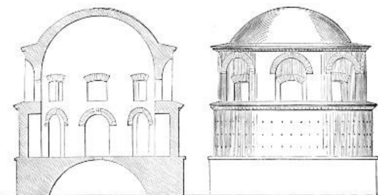
227. Section and Elevation of Tomb of Sta. Helena, Rome. No scale.
