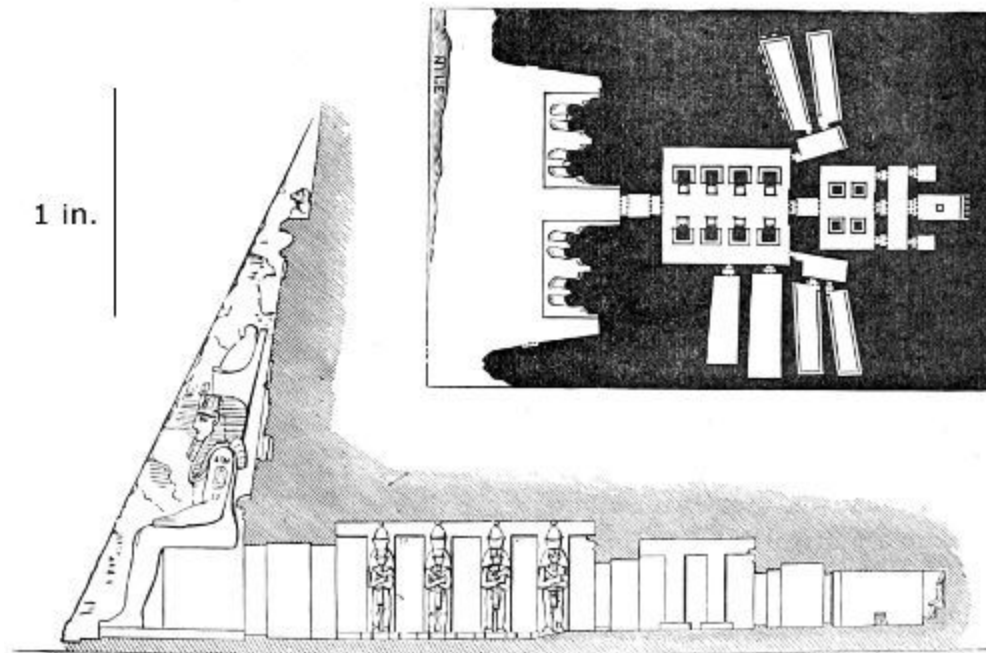
30. Plan and Section of Rock-cut Temple at Abû Simbel. Scale for plan 100 ft. to 1 in.; section 50 ft. to 1 in.
