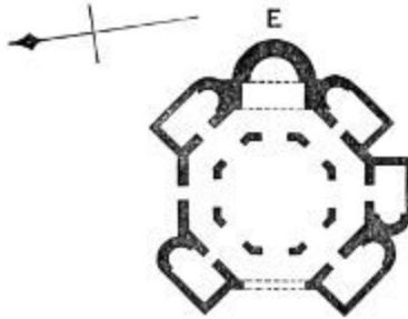
296. Church on Mount Gerizim.
