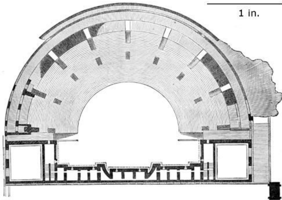
209. Plan of the Theatre at Orange. Scale 100 ft. to 1 in.
