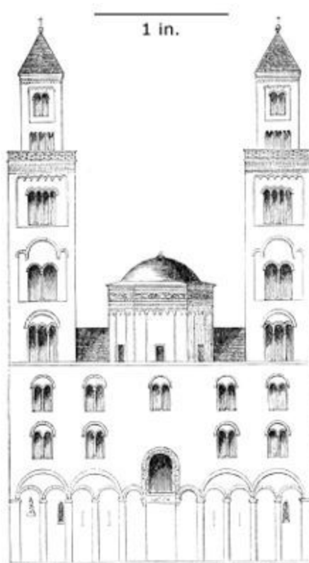
470. East End of Cathedral at Bari. (From Schultz.) Scale 50 ft. to 1 in.
