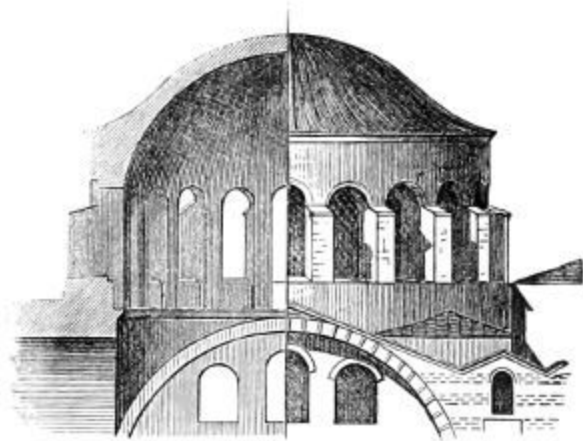
327. Half Section, half Elevation, of Dome of Sta. Irene at Constantinople.
