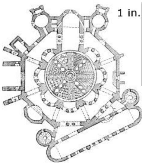
429. Plan of St. Vitale, Ravenna. (From Isabelle.) Scale 100 ft. to 1 in.
