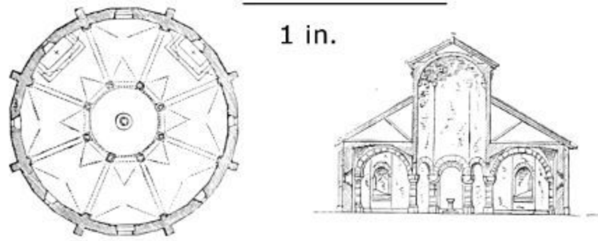
441. Plan and section of Baptistry at Asti. (From Osten.) Scale 50 ft. to 1 in.
