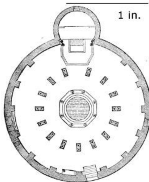
427. Plan of Baptistery at Nocera dei Pagani. Double the usual scale, or 50 ft. to 1 in.
