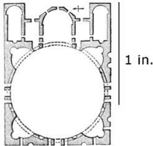
297. Cathedral at Bosra. Scale 100 ft. to 1 in.
