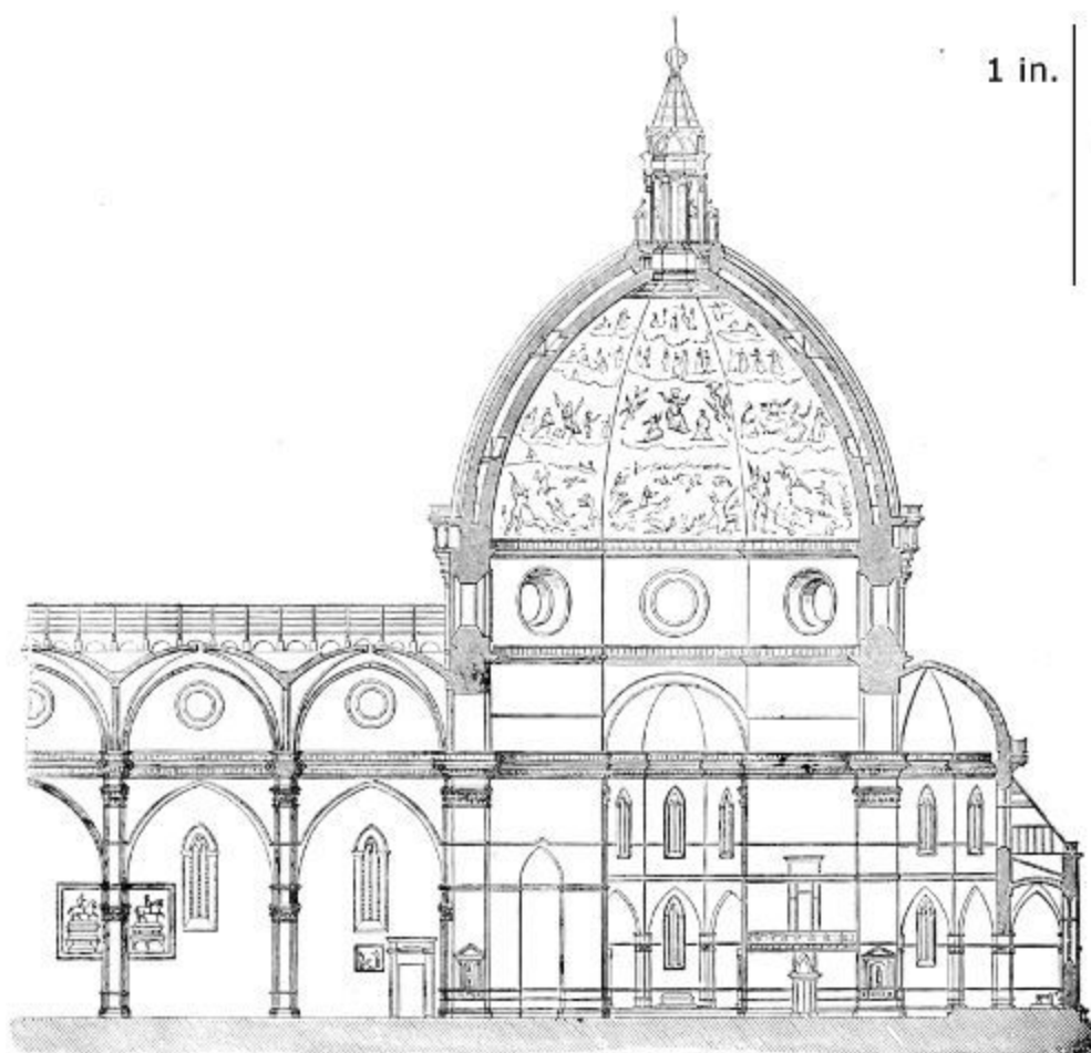
500. Section of Dome and part of Nave of the Cathedral at Florence. Scale 100 ft. to 1 in.
