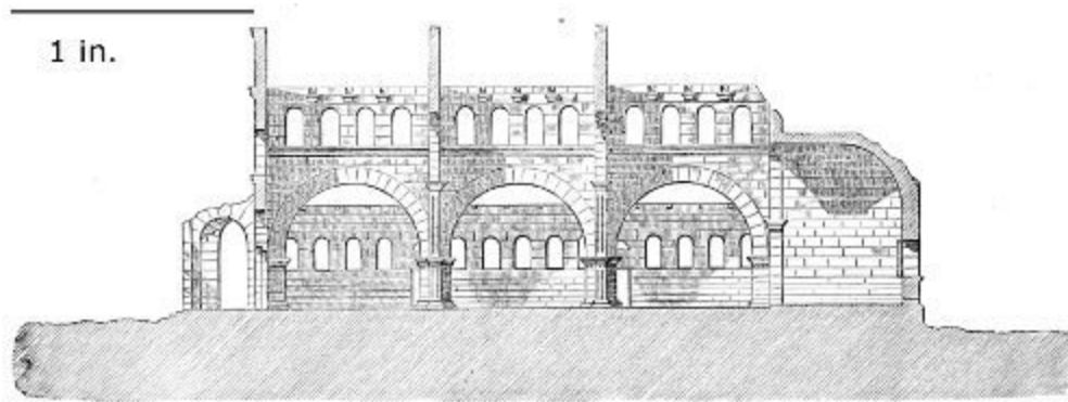
282. Section of Church at Roueiha. (From De Vogüé.) Scale 50 ft. to 1 in.
