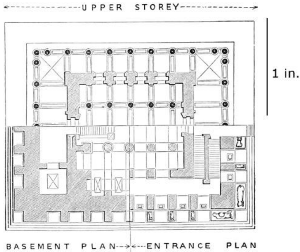
163. Plan of the Mausoleum at Halicarnassus, from a Drawing by the Author. Scale 50 ft. to 1 in.
