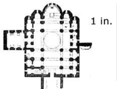
352. Plan of Church at Mokwi. Scale 100 feet to 1 in. [250]
