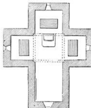
434. Tomb of Galla Placidia, Ravenna. (From Quast.) No scale.
