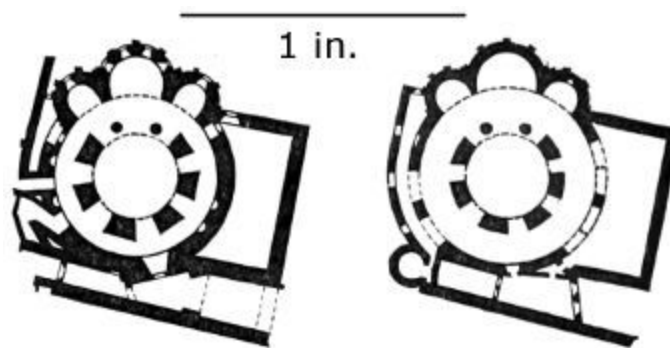
486. Ground and Upper Storey of San Donato, Zara. (From Jackson.) Scale 100 ft. to 1 in.
