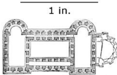
219. Plan of Porta Nigra at Trèves. Scale 100 ft. to 1 in.
