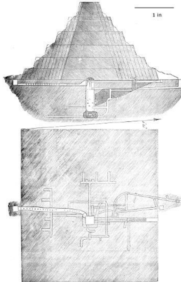
No. 10. Pyramid of Sakkara. (From Colonel Vyse's work.) Scale 100 ft to 1 in.
