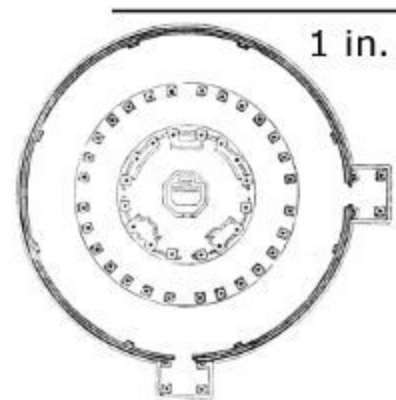
425. Plan of Sti. Angeli, Perugia. (From Isabelle.) Scale 100 ft. to 1 in.
