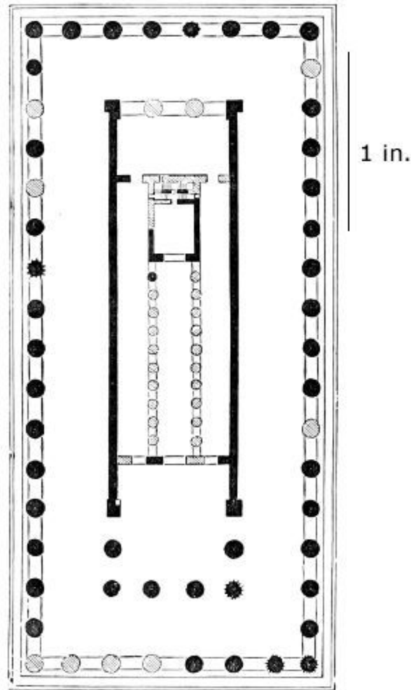
151. Plan of the great Temple at Selinus. (From Hittorff, 'Arch. Antique en Sicile.') Scale 100 ft. to 1 in.
