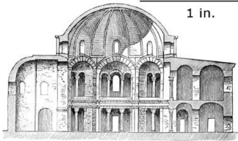
312. Section of Church of SS. Sergius and Bacchus. Scale 50 ft. to 1 in.
