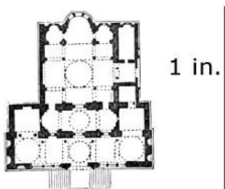
332. Plan of the Theotokos. Scale 100 ft. to 1 in.
