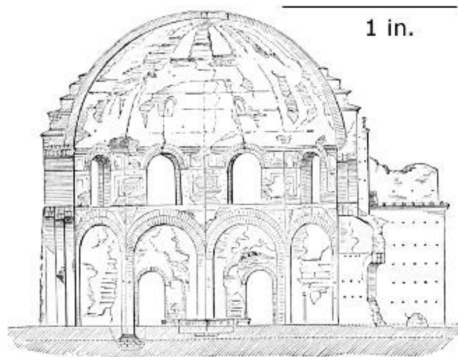
229. Section of Minerva Medica (from Isabelle.) Scale 50 ft. to 1 in.
