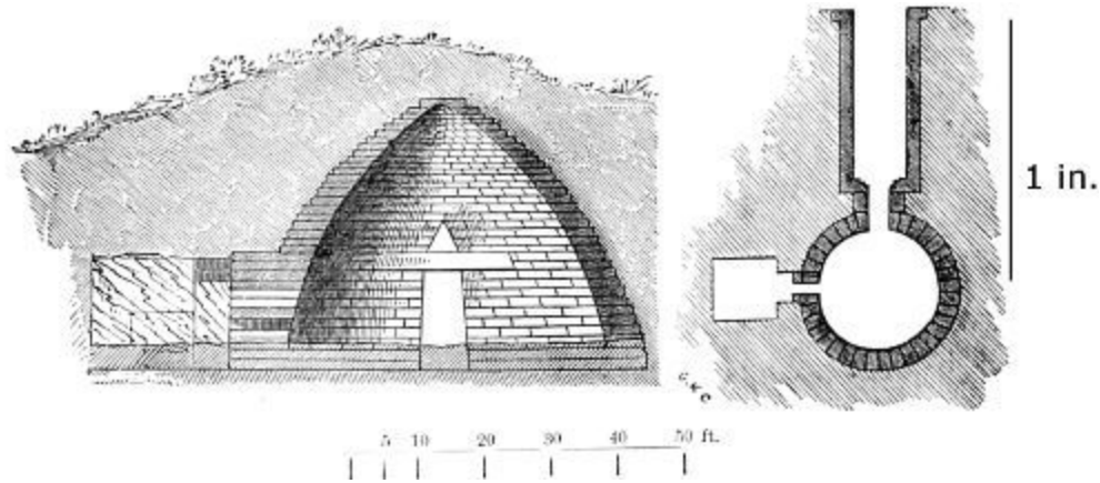
124. Section and Plan of Tomb of Atreus at Mycenæ. Scale of plan 100 ft. to 1 in.
