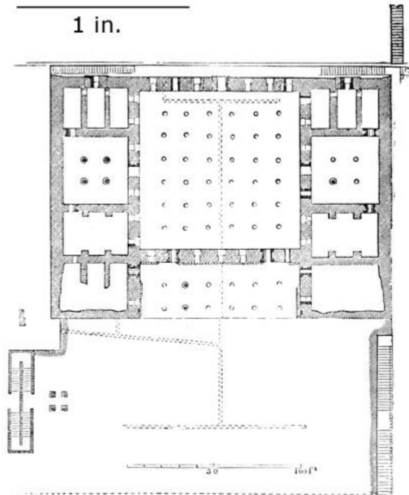
93. Palace of Xerxes. Scale 100 ft. to 1 in.
