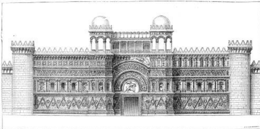
269. Elevation of External Façade of the Mashita, as restored by the Author.
