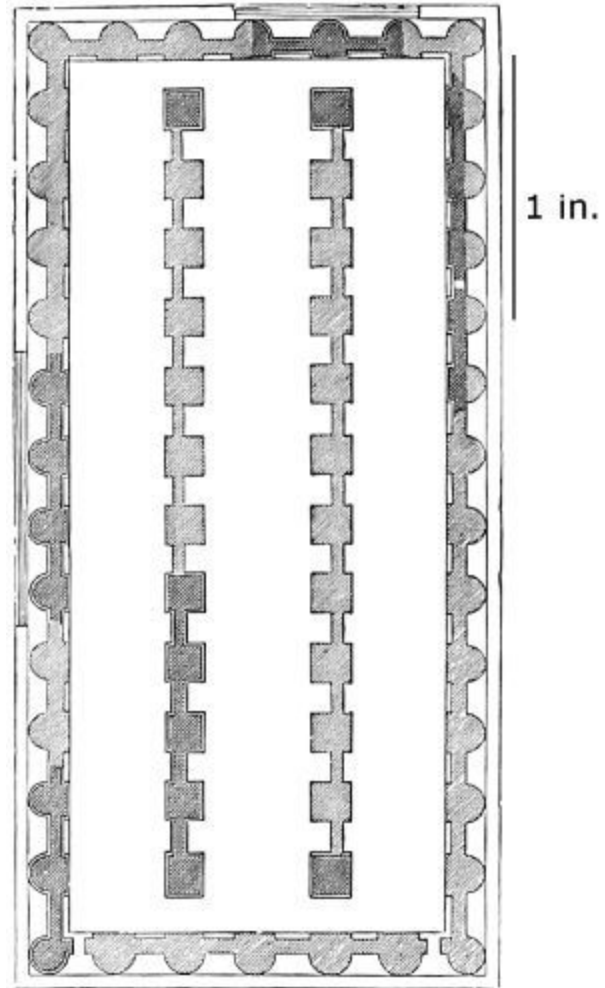
152. Plan of Great Temple at Agrigentum. Scale 100 ft. to 1 in.
