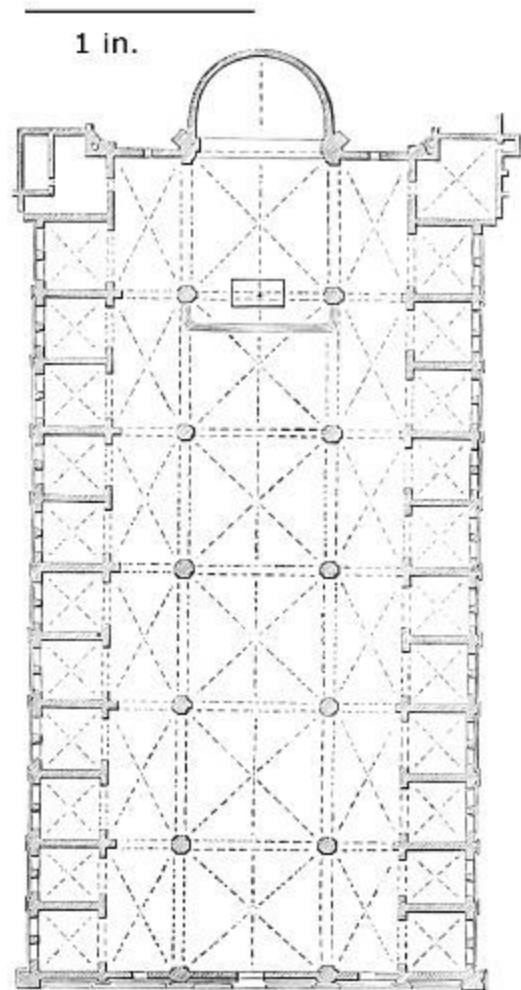
504. Plan of the part executed of St. Petronio, Bologna. (from Wiebeking.) Scale 100 ft. to 1 in.
