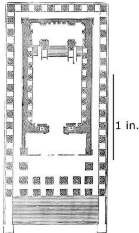
197. Plan of Small Temple at Baalbec. Scale 100 ft. to 1 in.
