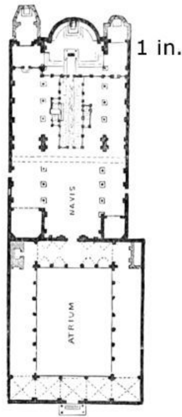
395. Plan of the Church of San Clemente at Rome. (From Gutensohn and Knapp. [263] ) Scale 100 ft. to 1 in
