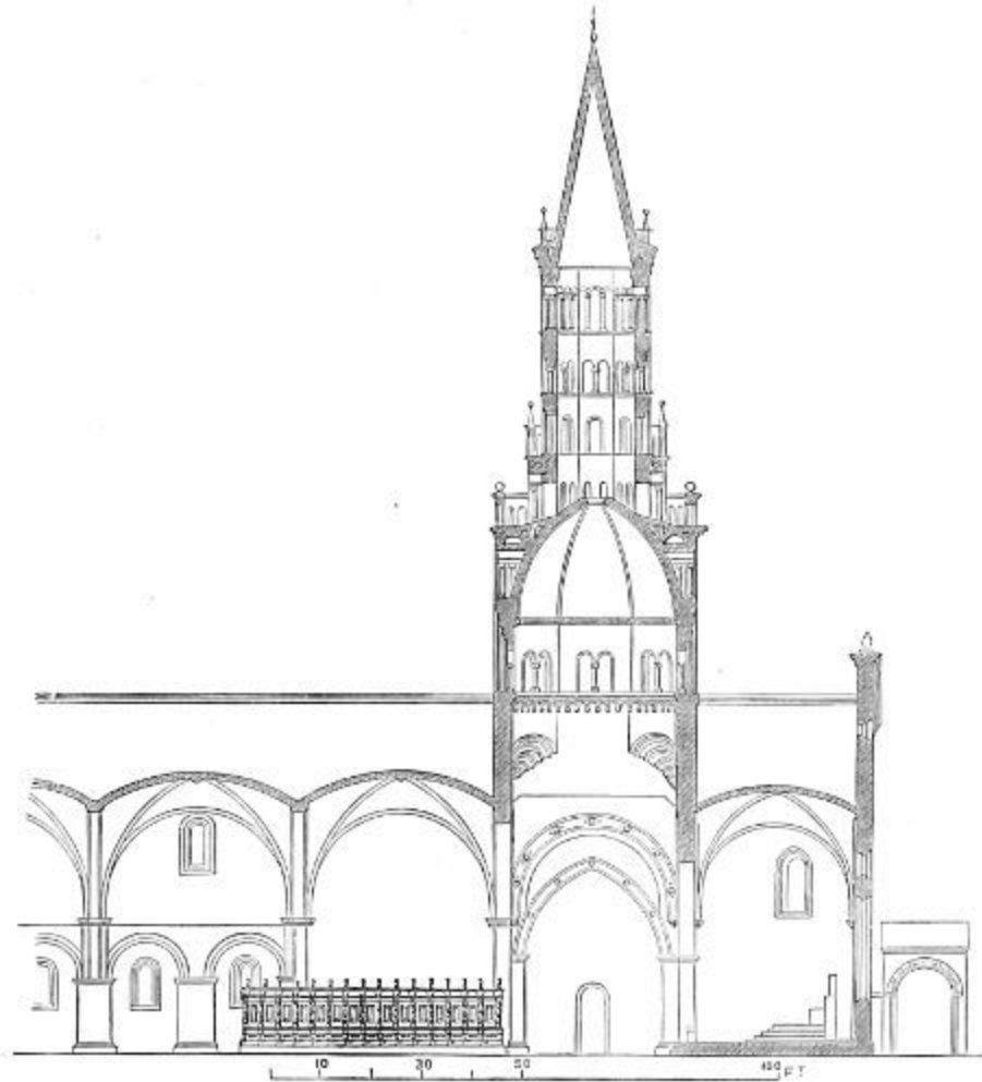
503. Section of Eastern portion of Church at Chiaravalle. (From Gruner's 'Terra Cotta Architecture in Italy.') Scale 50 ft. to 1 in.
