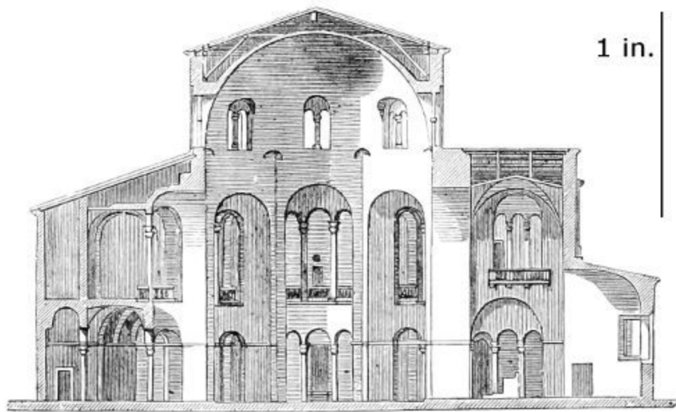
430. Section of St. Vitale, Ravenna. (From Isabelle.) Scale 50 ft. to 1 in.
