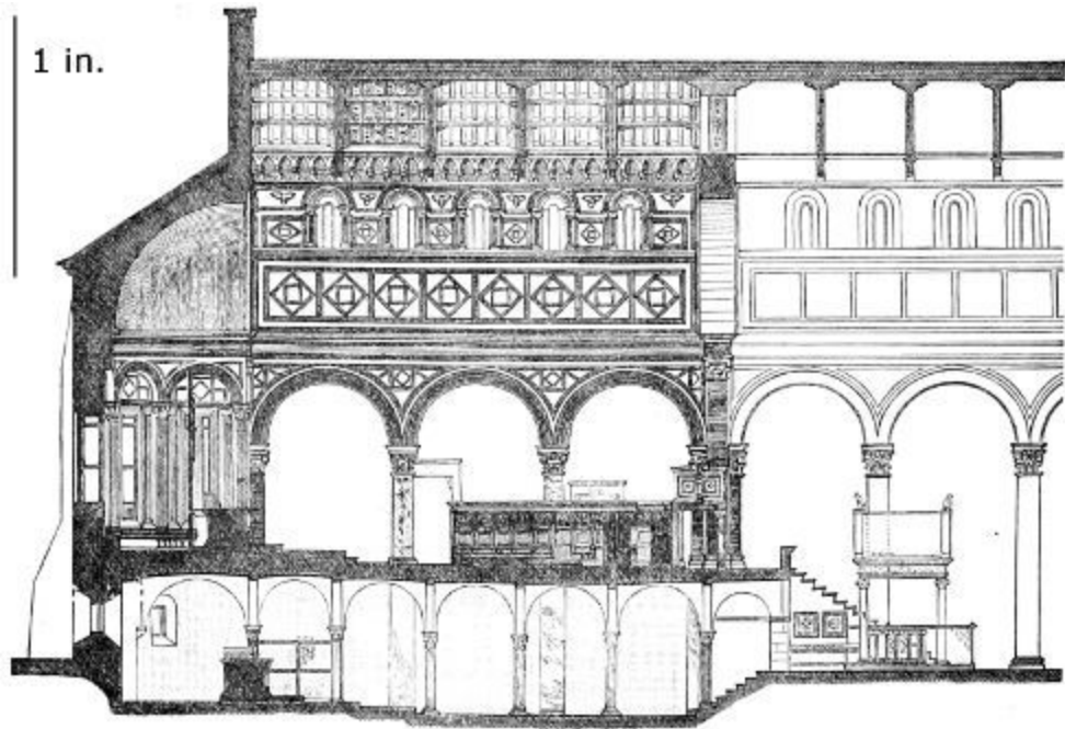
462. Section of San Miniato, near Florence. (From drawing by R. W. Schultz.) Scale 50 ft. to 1 in.
