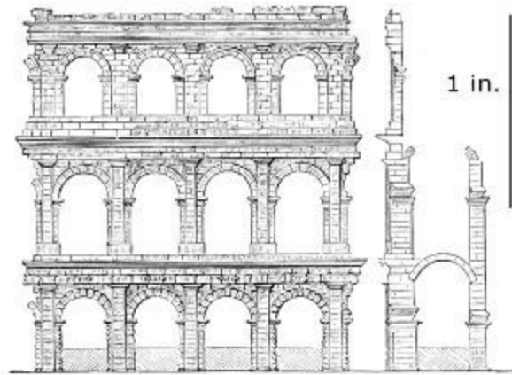
213. Elevation of the Amphitheatre at Verona. Scale 50 ft. to 1 in.
