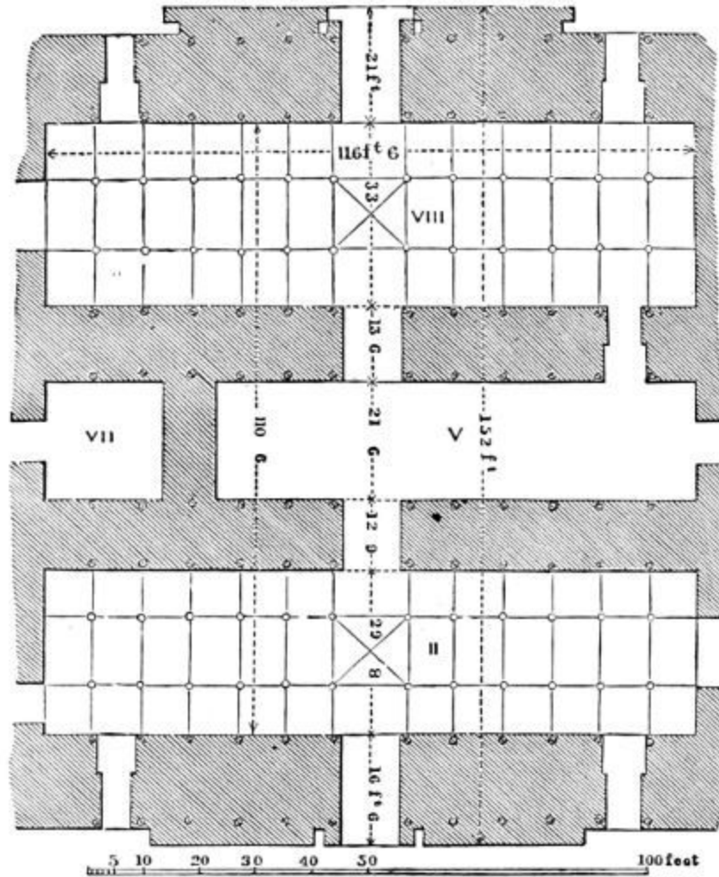
63. Enlarged Plan of the Three Principal Rooms at Khorsabad. Scale 50 ft. to 1 in.
