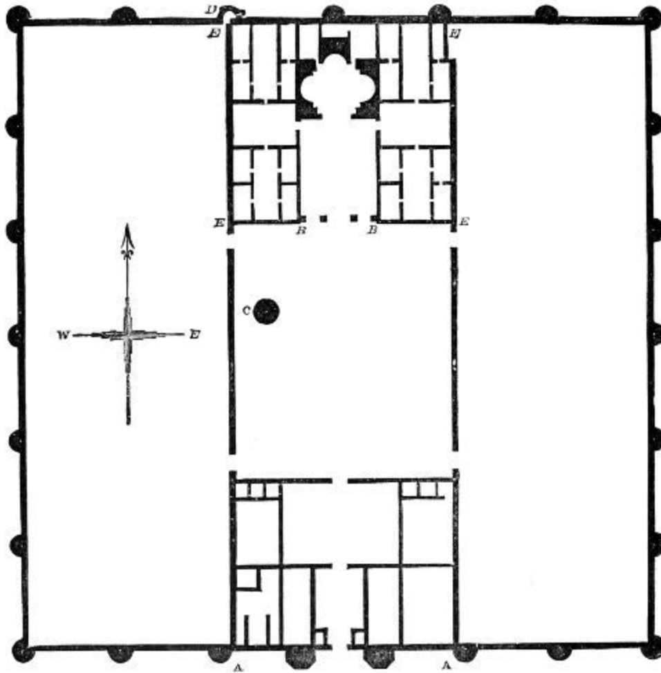
265. Sketch Plan of Palace at Mashita.
