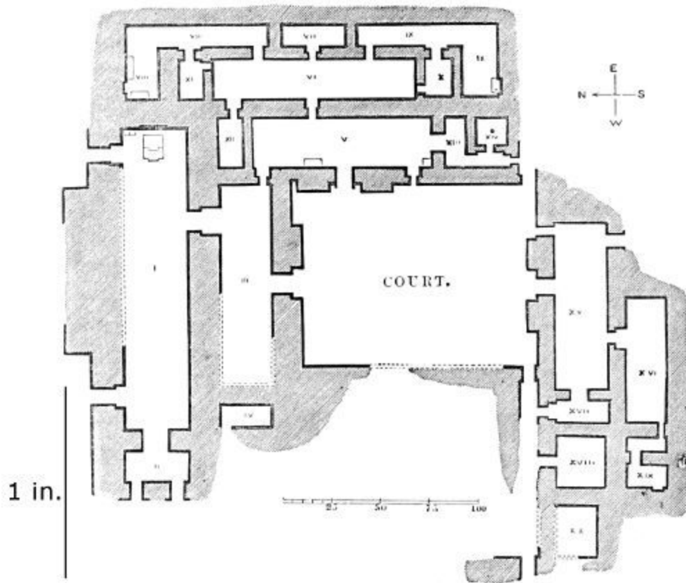
58. North-West Palace at. Nimroud. [79] Scale 100 ft. to 1 in.
