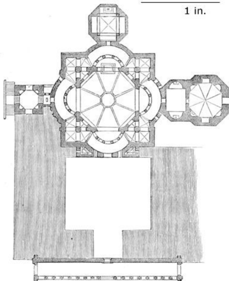
432. Plan of S. Lorenzo at Milan. (From Quast, 'Altchristlichen,' &c.) Scale 100 ft. to 1 in.
