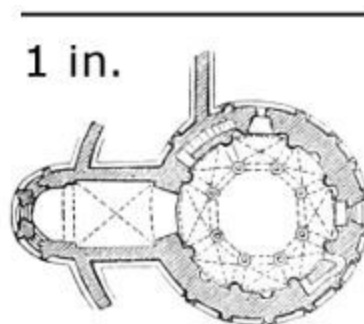
457. San Tomaso in Limine. Scale 100 ft. to 1 in.
