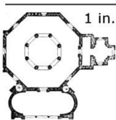
422. Baptistry of Constantine. (From Isabelle.) Scale 100 ft. to 1 in.
