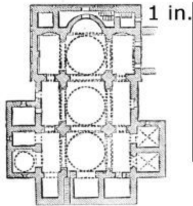
481. Plan of Church at Molfetta. Scale 100 ft. to 1 in.
