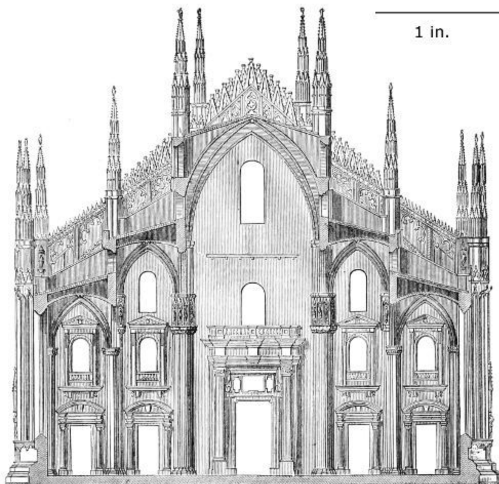
507. Section of the Cathedral of Milan. [313] (From Wiebeking.) Scale 50 ft. to 1 in.
