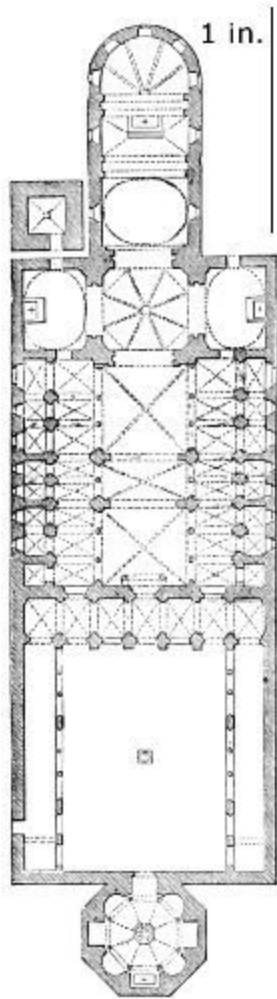
442. Plan of the Cathedral at Novara. Scale 100 ft. to 1 in.
