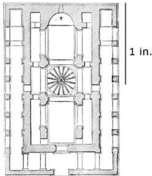
346. Plan of Church at Usunlar. (From Grimm.) Scale 50 ft. to 1 in.
