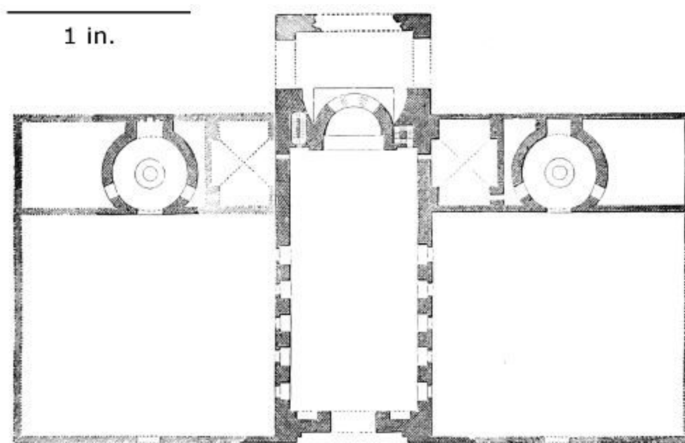
288. Church at Pergamus. (From a Plan by Ed. Falkener, Esq.) Scale 100 ft. to 1 in.
