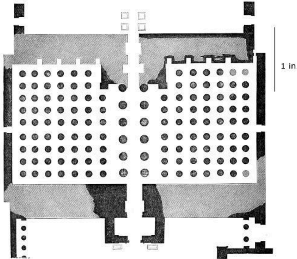
22. Plan of Hypostyle Hall at Karnac. Scale 100 ft. to 1 in.
