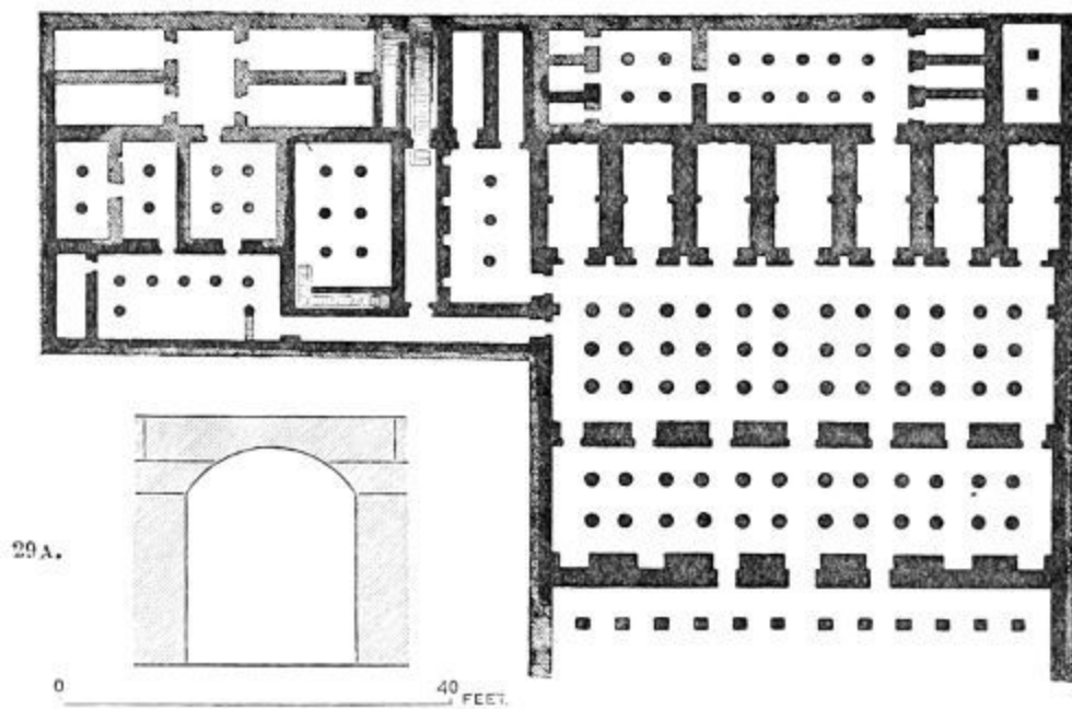
29. Plan of Temple of Abydos.
