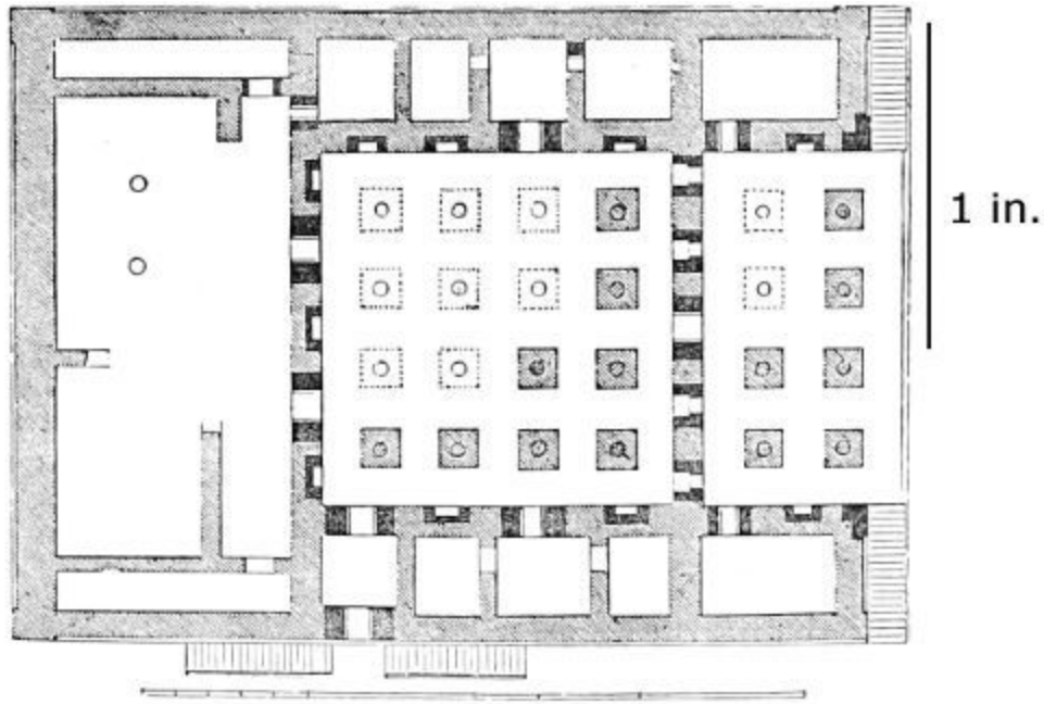
90. Palace of Darius. Scale 50 ft. to 1 in.
