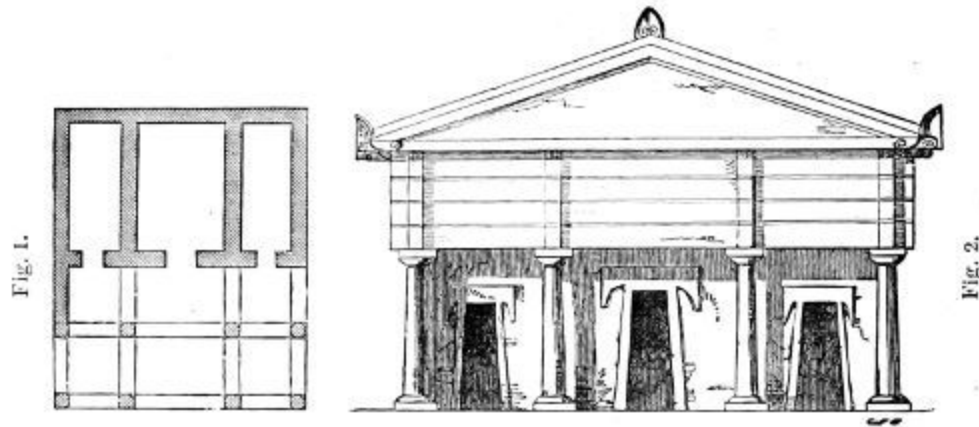
167. Plan and Elevation of an Etruscan Temple.
