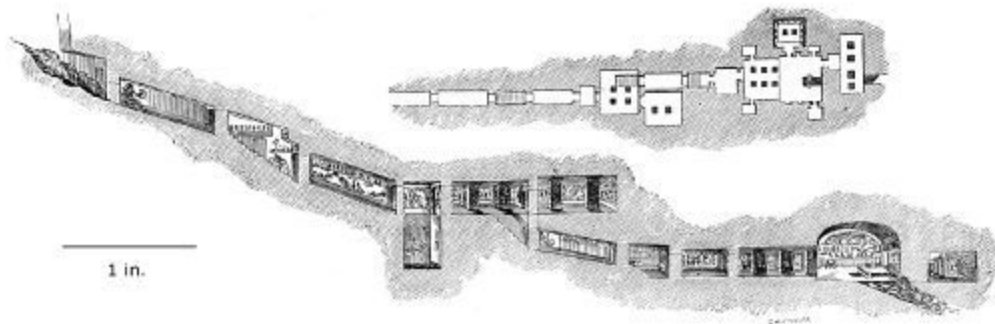
32. Plan and Section of Tomb of Meneptah at Thebes. Scale for plan 100 ft. to 1 in.; section 50 ft. to 1 in.
