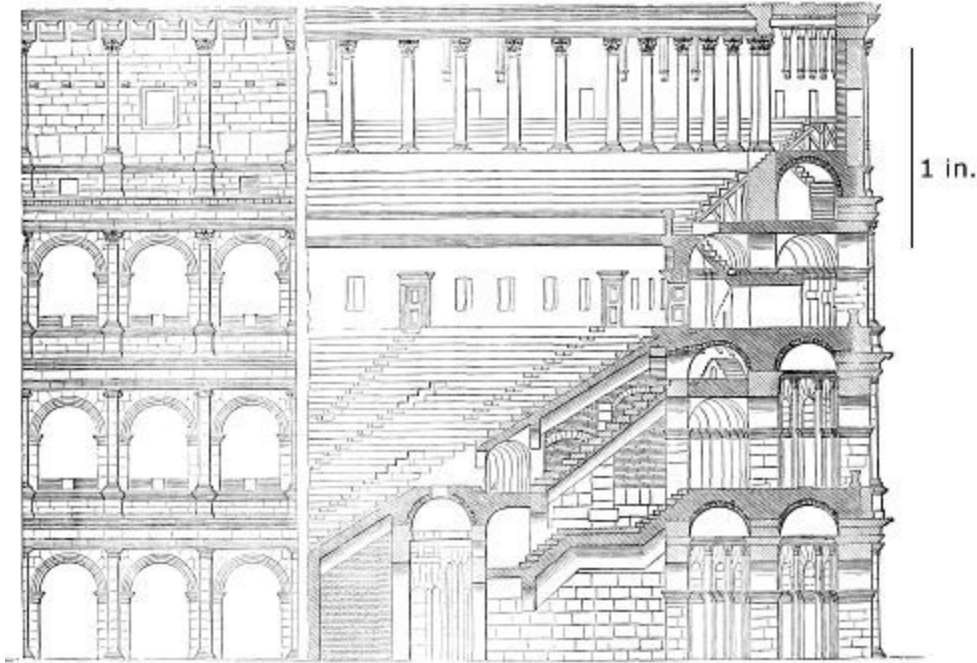
211. Elevation and Section of part of the Flavian Amphitheatre at Rome. Scale 50 ft. to 1 in.
