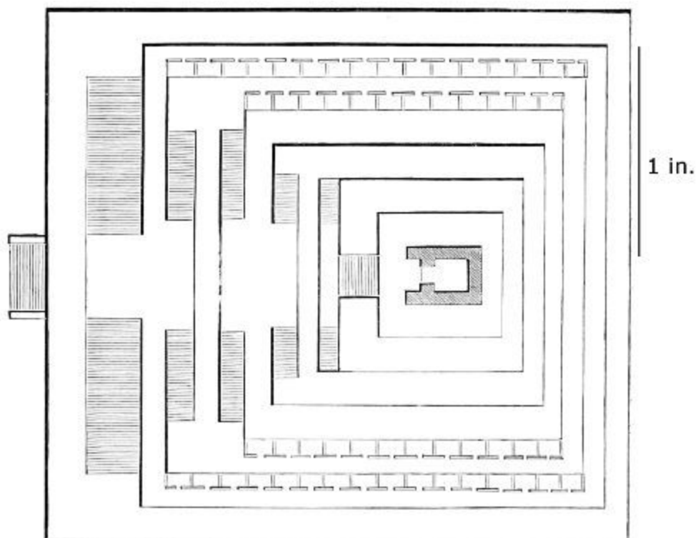
51. Diagram Plan of Birs Nimroud. Scale 100 ft. to 1 in.
