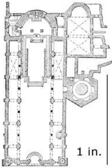
466. Plan of Zara Cathedral. Scale 100 ft. to 1 in.
