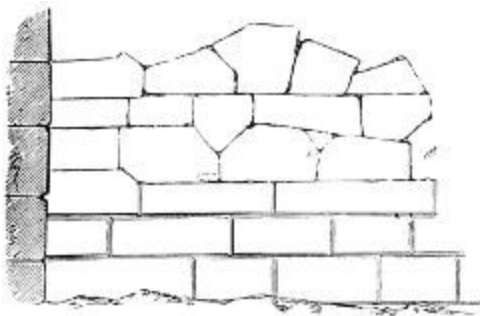
128. Wall in Peloponnesus. (From Blouet's 'Voyage en Grèce.')
