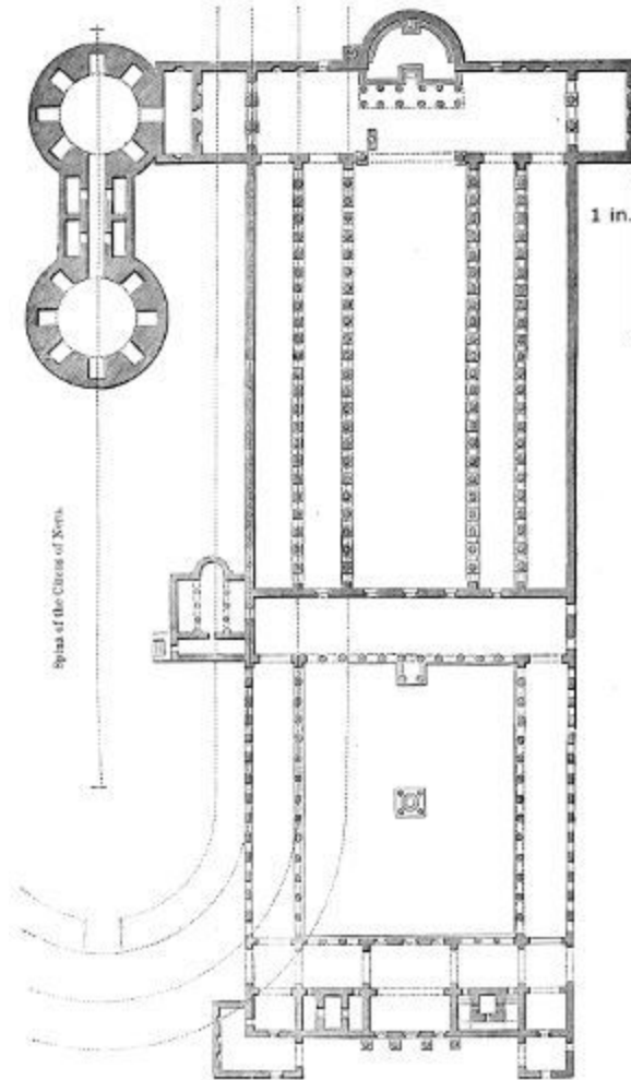
396. Plan of the original Basilica of St. Peter at Rome. (From Gutensohn and Knapp.) Scale 100 ft. to 1 in.
