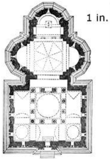
386. Plan of Church at Kurtea d'Argyisch. Scale 50 ft. to 1 in.
