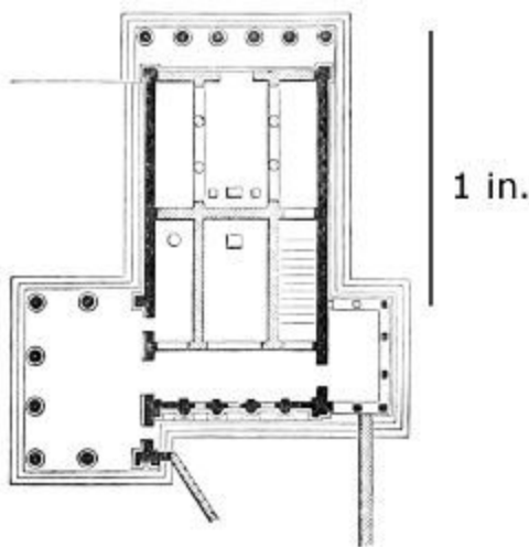
158. Restored Plan of Erechtheum. Scale 50 ft. to 1 in.
