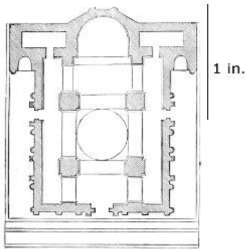
344. Plan of Church at Dighour. (From Texier.) Scale 50 ft. to 1 in.
