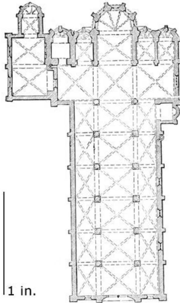
494. Plan of Sta. Anastasia, Verona. Scale 100 ft. to 1 in.
