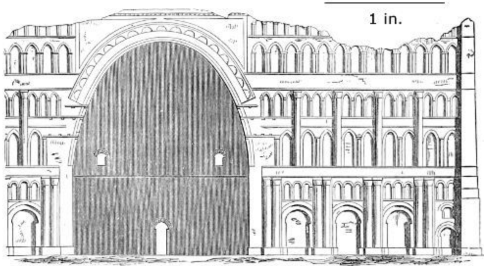
264. Elevation of Great Arch of Tâk Kesra at Ctesiphon. Scale 50 ft. to 1 in.
