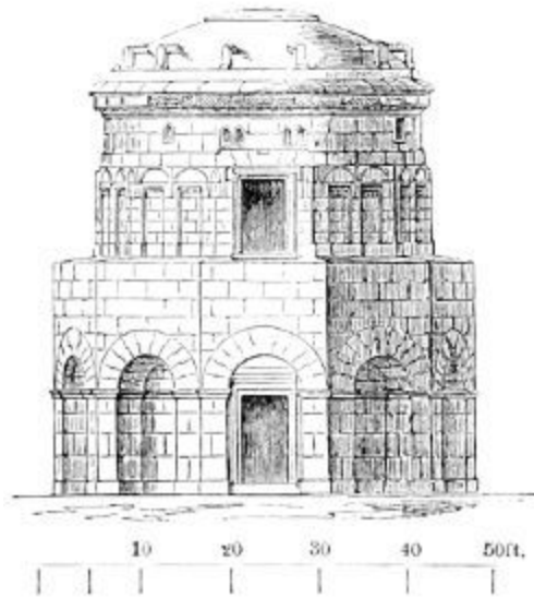
437. Elevation of Tomb of Theodoric, Ravenna. (From Isabelle, 'Édifices Circulaires.')
