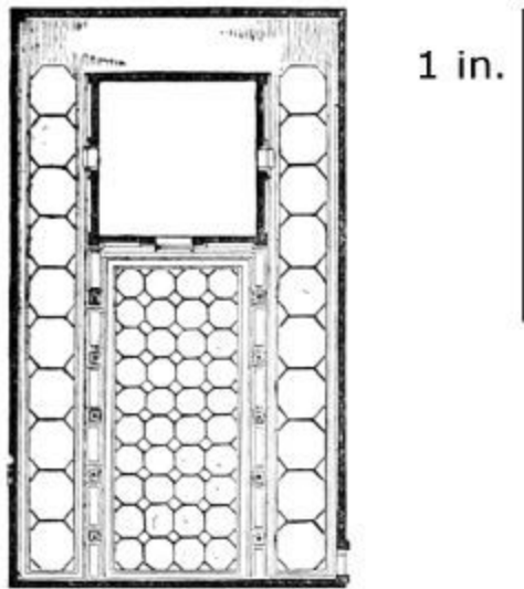
390. Plan of Church at Djemla. Scale 50 ft. to 1 in.
