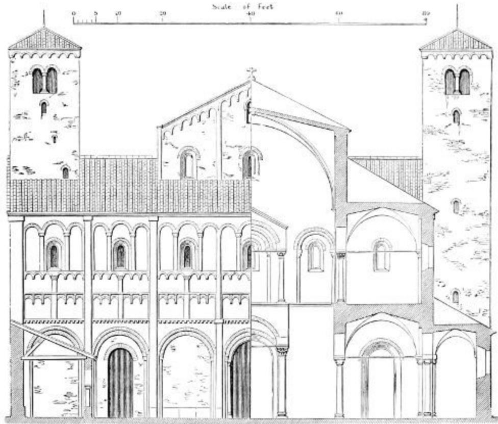
443. Elevation and Section of the Façade of the Cathedral at Novara. (From Osten.)
