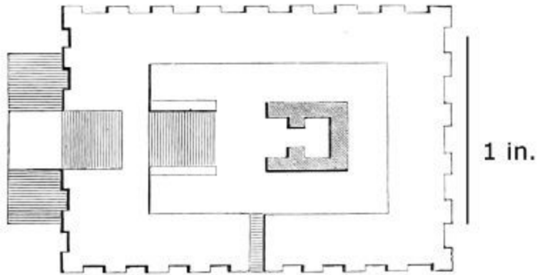
49. Plan of Temple at Mugheyr. Scale 100 ft. to 1 in.
