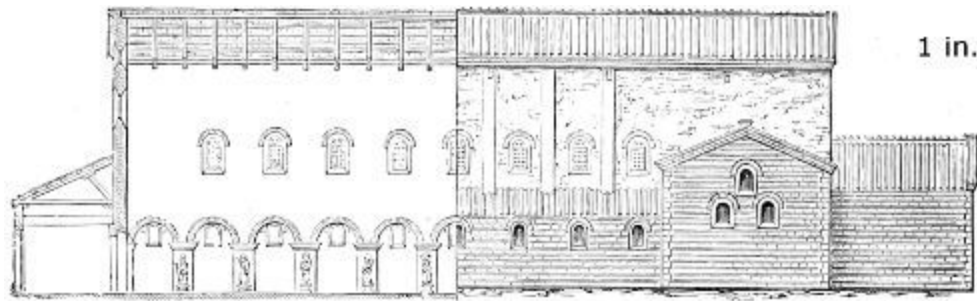
408. Half Section, half Elevation, of the Church of San Vincenzo alle Tre Fontane. (From Guttensohn and Knapp.) Scale 50 ft. to 1 in.
