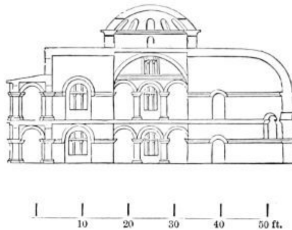
328. St Clement, Ancyra. (From a Drawing by Ed. Falkener.)
