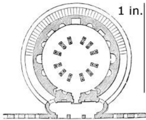
423. Plan of the Tomb of Sta. Costanza, Rome. (From Isabelle, 'Édifices Circulaires.') Scale 100 ft. to 1 in.
