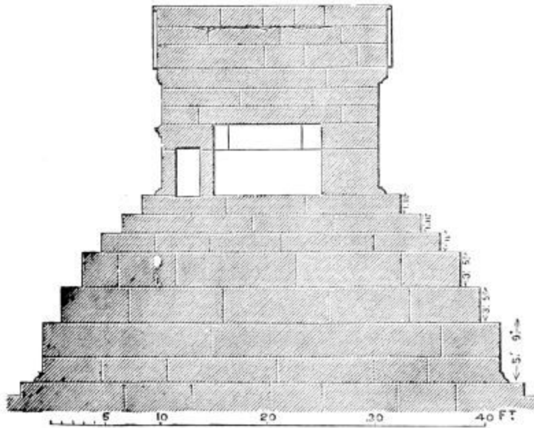
86. Section of Tomb of Cyrus. (From Texier.)
