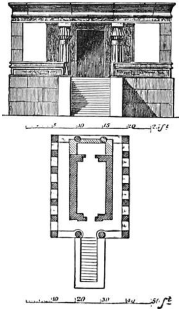
31. Mammeisi at Elephantine.
