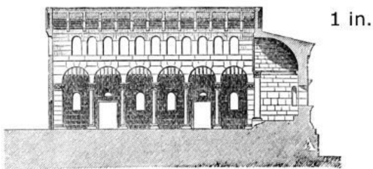
279. Section of Church in Baquoza. (From De Vogüé.) Scale 50 ft. to 1 in.
