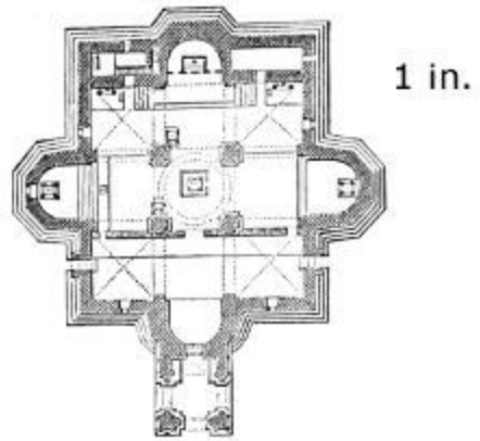
353. Plan of Church at Etchmiasdin. (From Brosset.) Scale 100 ft. to 1 in.
