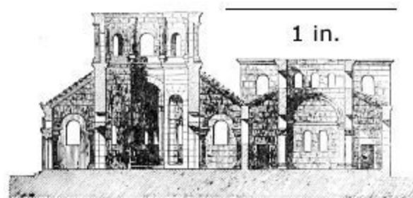
298. Section of Double Church at Kalat Sema'n. (From De Vogüé.) Scale 50 ft. to 1 in.
