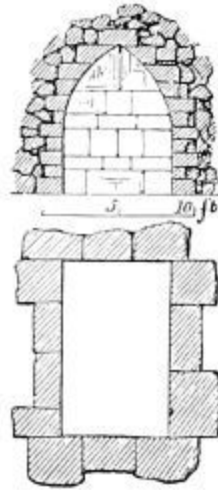
114. Plan and Section of Chamber in Tumulus at Tantalais.
