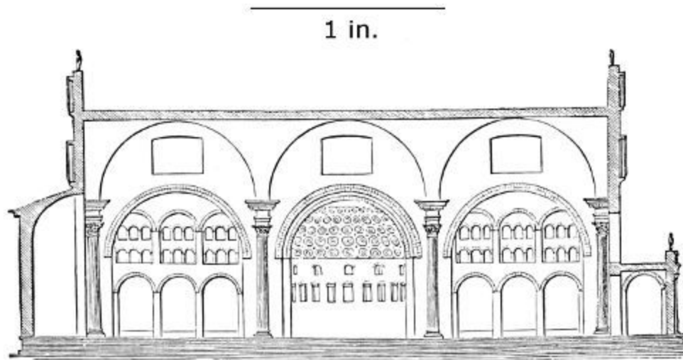
202. Longitudinal Section of Basilica of Maxentius. Scale 100 ft. to 1 in.
