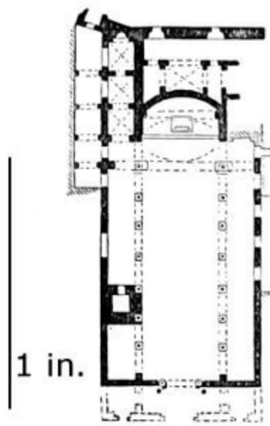
405. Plan of Sta. Pudentiana. Scale 100 ft. to 1 in.
