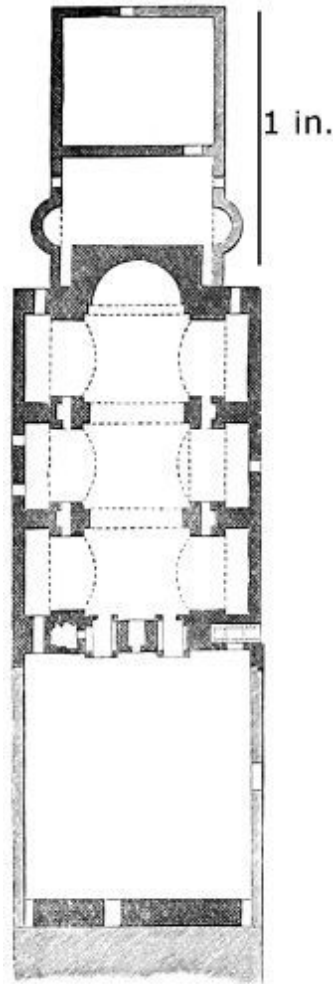
294. Church at Hierapolis. Scale 100 ft. to 1 in. (E. F. del.)
