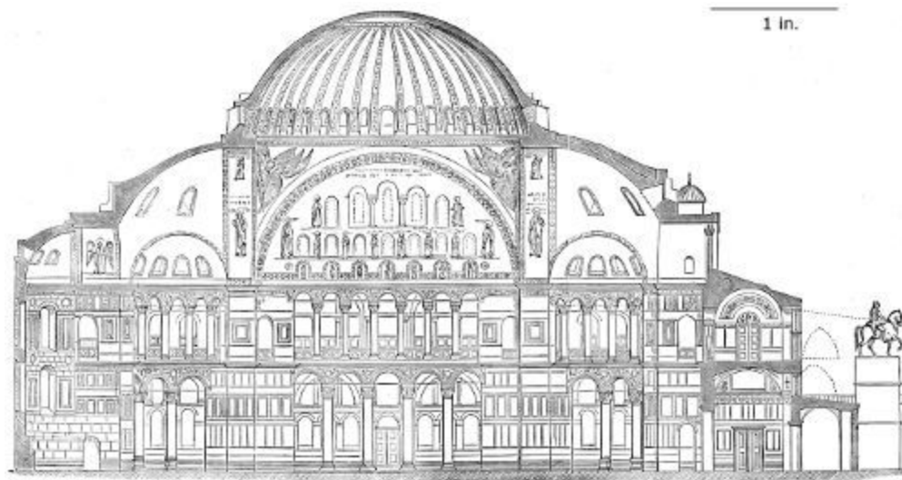
317. Section of Sta. Sophia from E. to W. Scale 100 ft. to 1 in.
