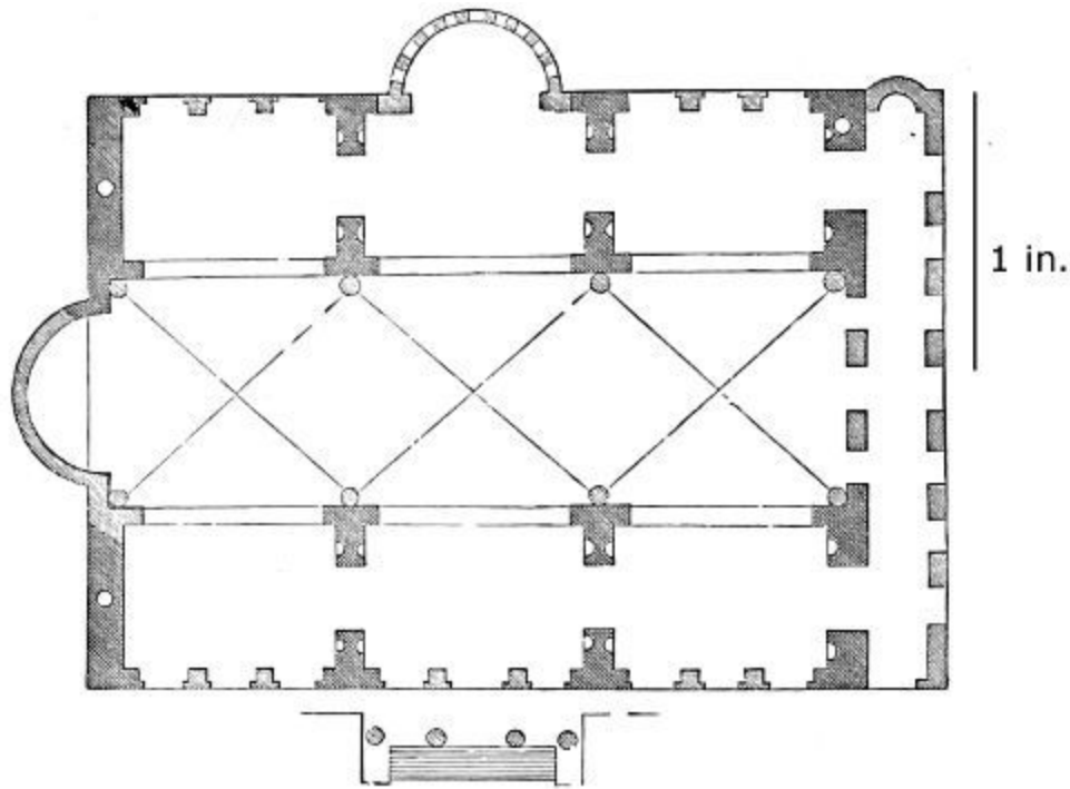
201. Plan of Basilica of Maxentius. Scale 100 ft. to 1 in.
