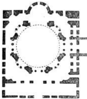
311. Church of SS. Sergius and Bacchus.
