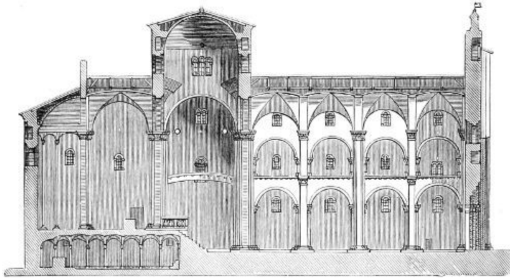
444. Section of San Michele, Pavia. (From Agincourt.) No scale.
