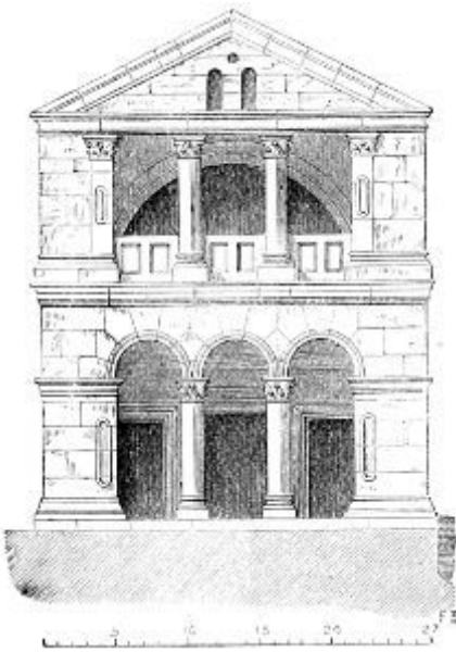
286. Elevation of Chapel at Babouda. (From De Vogüé.)
