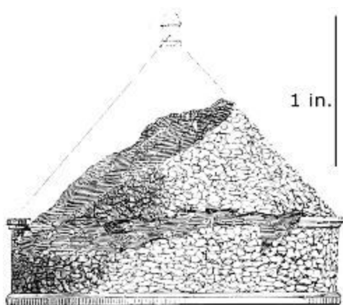
113. Elevation of Tumulus at Tantalais. (From Texier's 'Asie Mineure.') 100 ft. to 1 in.
