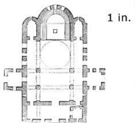
348. Plan of Church at Pitzounda. Scale 100 ft. to 1 in.
