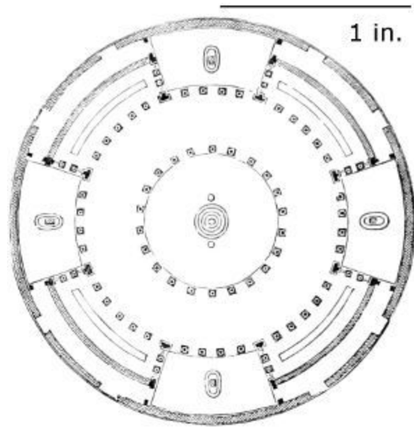
424. Plan of San Stefano Rotondo. (From Gutensohn and Knapp.) Scale 100 ft. to 1 in.
