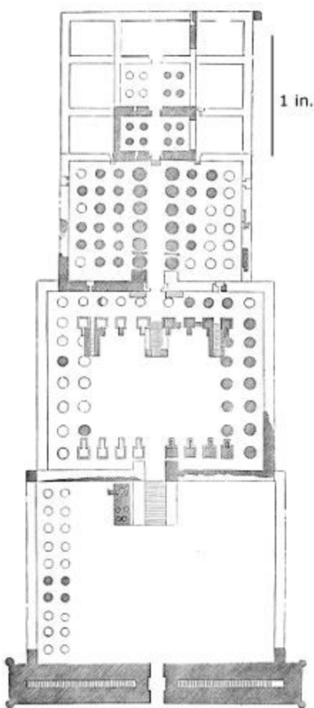
19. Ramesseum at Thebes. Scale 100 ft. to 1 in.
