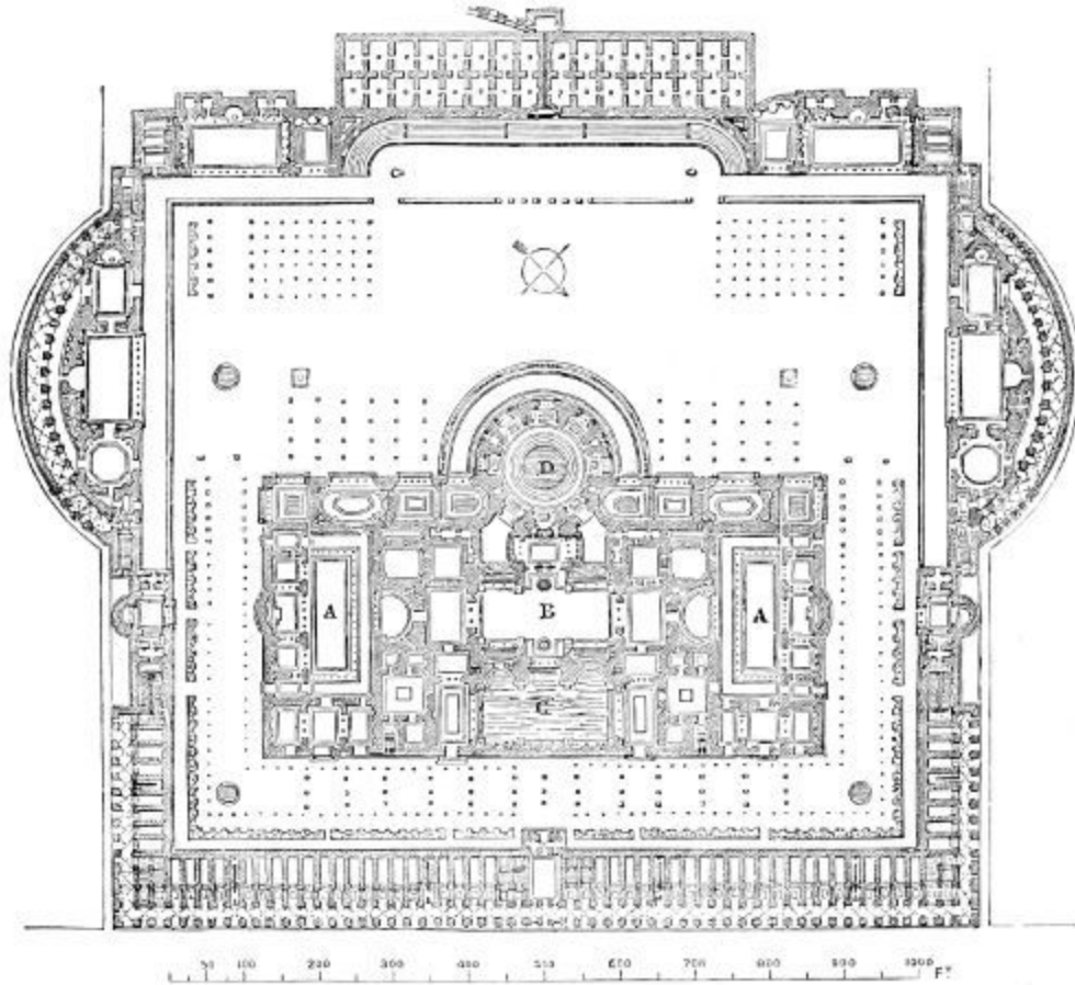
214. Baths of Caracalla, as restored by A. Blouet.
