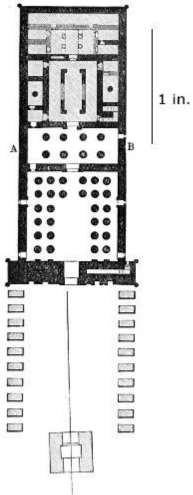
25. South Temple of Karnac. Scale 100 ft. to 1 in.
