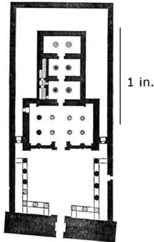
42. Plan of Temple at Kalábsheh. Scale 100 ft. 1 in.
