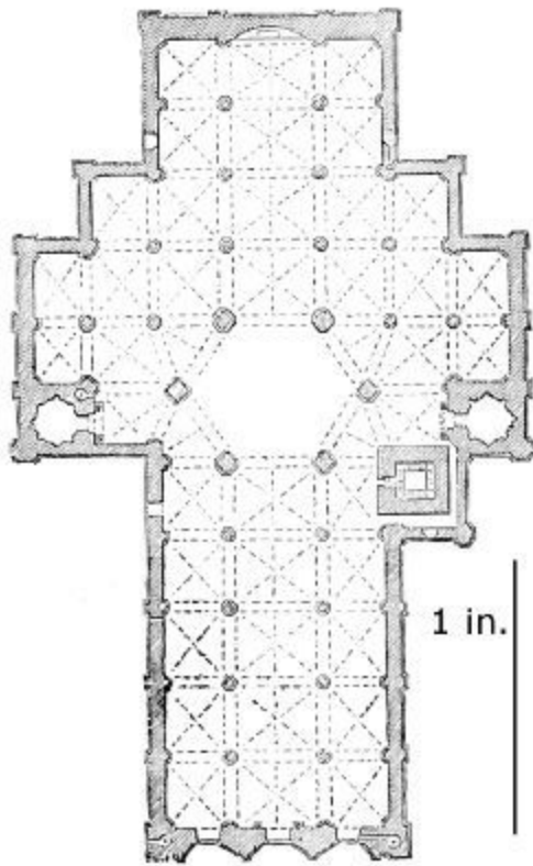
497. Plan of the Cathedral at Siena. (From the 'Églises principales d'Europe.') Scale 100 ft. to 1 in.
