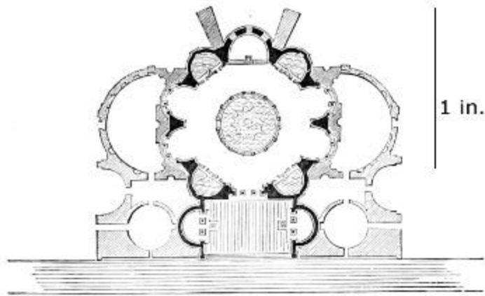
228. Plan of Minerva Medica at Rome, as restored in Isabelle's 'Édifices Circulaires,' on the theory of its being a Bath. Scale 100 ft. to 1 in.
