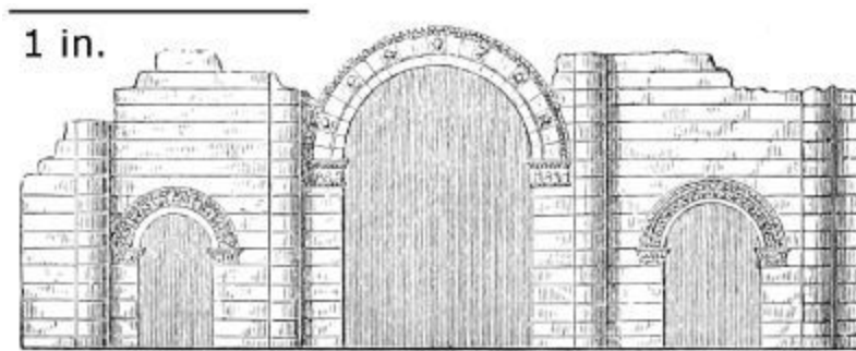
254. Elevation of part of the Palace of Al Hadhr. Scale 50 ft. to 1 in.
