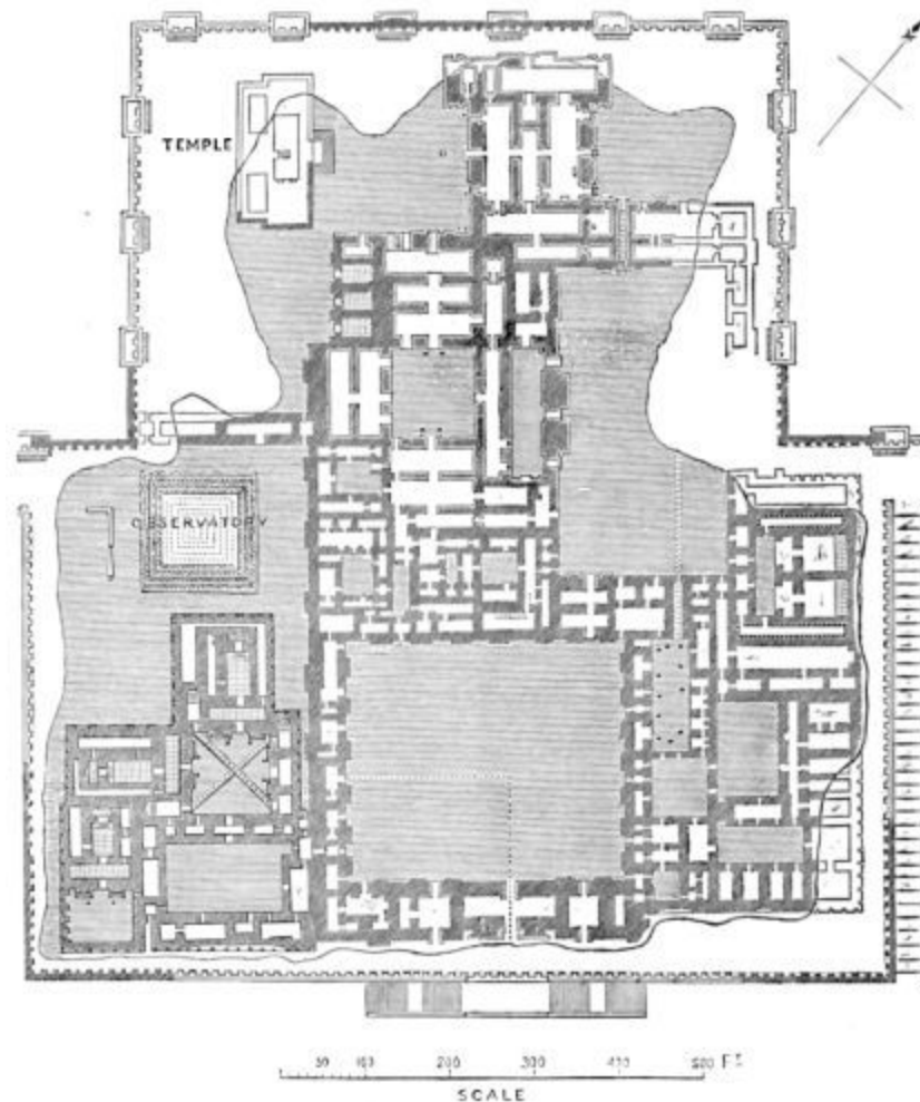
61. Plan of Palace at Khorsabad, as completely excavated by M. Place. The parts tinted were actually found. Those in outline are conjectural.
