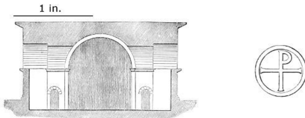
295. Section of Church at Hierapolis. Scale 50 ft. to 1 in. With monogram found on its walls. (From a Drawing by E. Falkener.)
