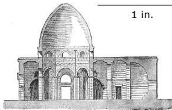
310. Section of Church at Ezra. Scale 50 ft. to 1 in.
