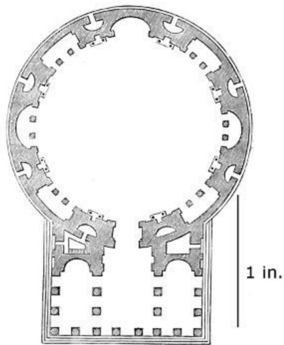
190. Plan of Pantheon at Rome. Scale 100 ft. to 1 in.
