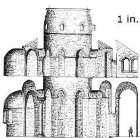
487. Section San Donato, Zara. Scale 50 ft. to 1 in.
