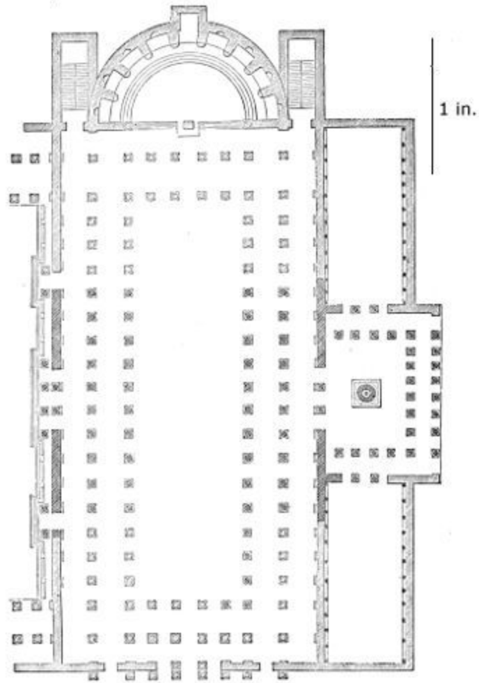
199. Plan of Trajan's Basilica at Rome. Scale 100 ft. to 1 in.
