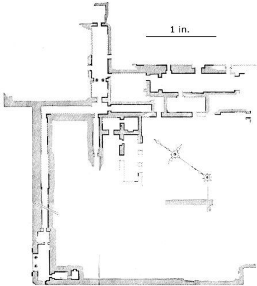
70. Central Palace, Koyunjik. Scale 100 ft. to 1 in.
