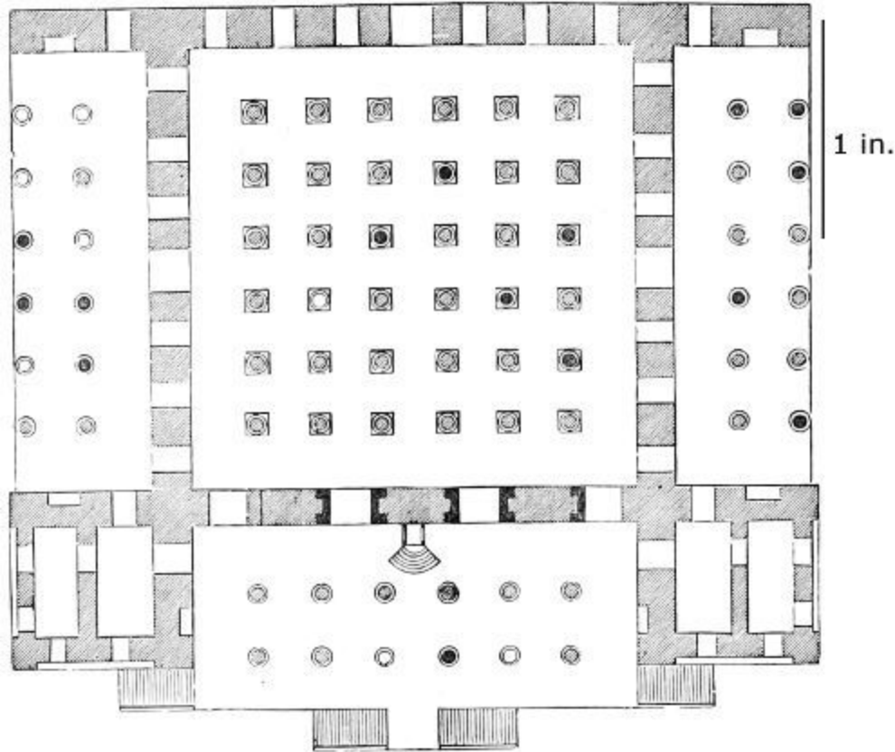
94. Restored Plan of Great Hall of Xerxes at Persepolis. Scale 100 ft. to 1 in.
