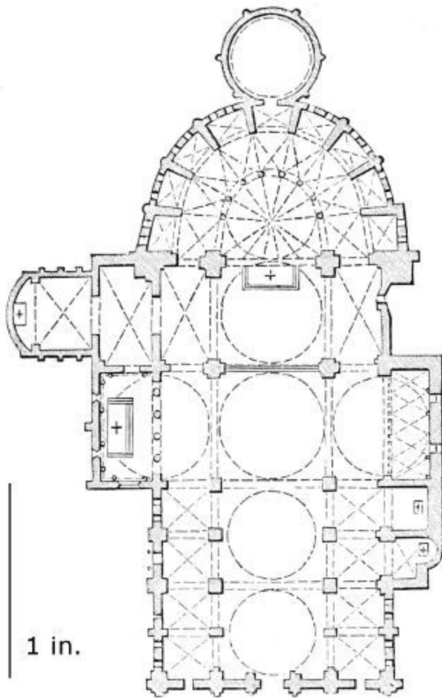
417. Plan of St. Antonio, Padua. (From Wiebeking.) Scale 100 ft. to 1 in.
