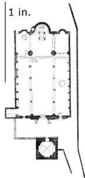
451. Plan of Sta. Maria, Toscanella. (From Gailhabaud.) Scale 100 ft. to 1 in.
