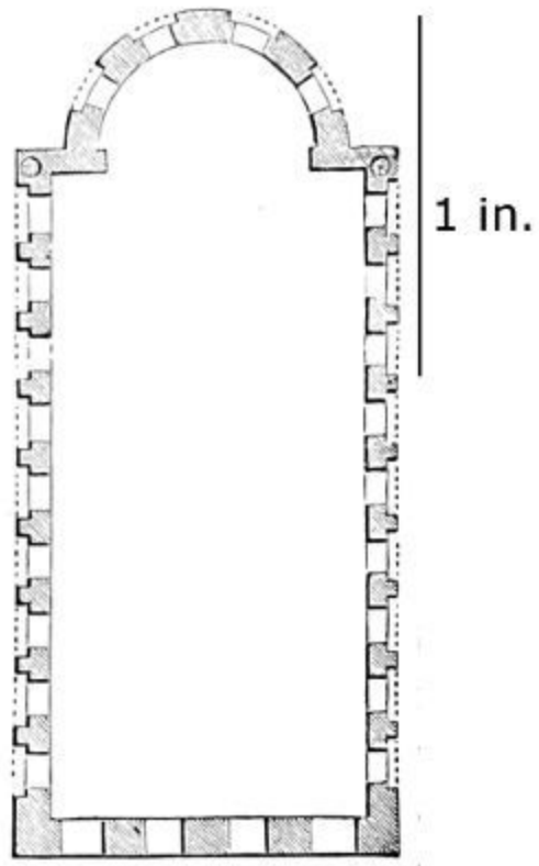
205. Plan of the Basilica at Trèves. Scale 100 ft. to 1 in.
