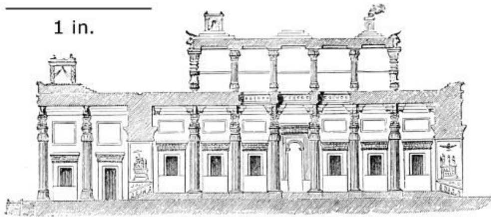
97. Restored Section of Hall of Xerxes. Scale 100 ft. to 1 in.
