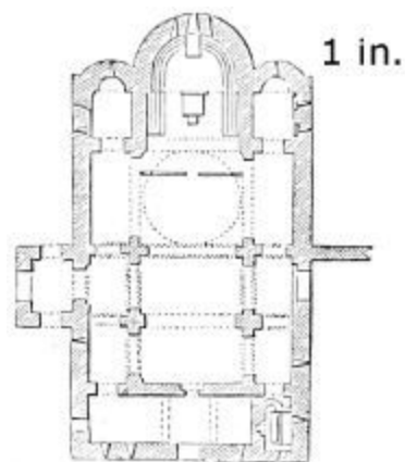
351. Church at Bedochwinta. (From Brosset.) Scale 100 ft. to 1 in.
