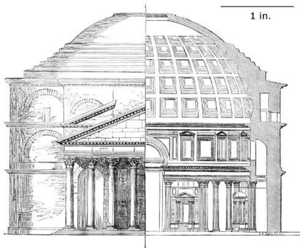
191. Half Elevation, half Section, of the Pantheon at Rome. Scale 50 ft. to 1 in.
