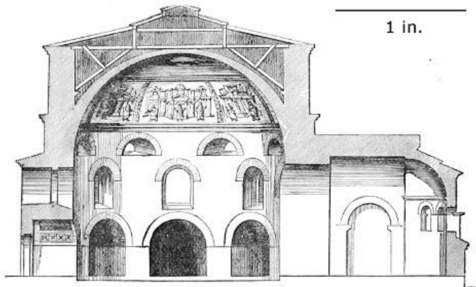
305. Section of Church of St. George at Thessalonica. (From Texier and Pullan.) Scale 50 ft. to 1 in.
