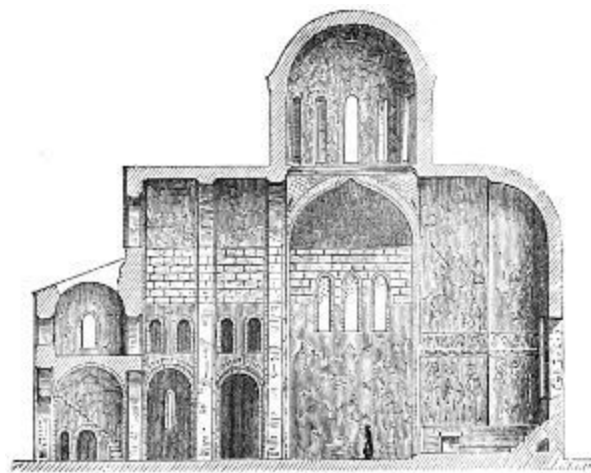
349. Section of Church at Pitzounda. (From Dubois.) No scale.
