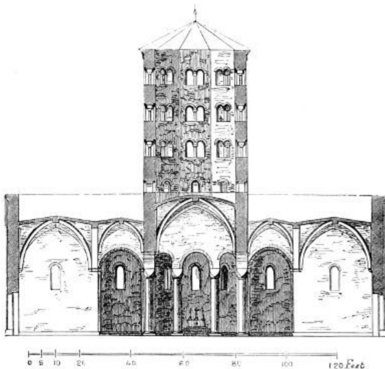
440a. Section of Church of San Antonio at Piacenza. (From Osten.)
