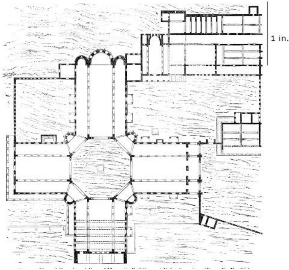
280. Plan of Church and Part of Monastic Buildings at Kalat Sema'n. (From De Vogüé.) Scale 100 ft. to 1 in.
