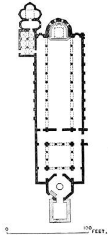
418. Church at Parenzo in Istria. (From Jackson.) Scale 100 ft. to 1 in.
