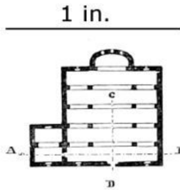
290. Plan, Tafkha. Scale 100 ft. to 1 in.
