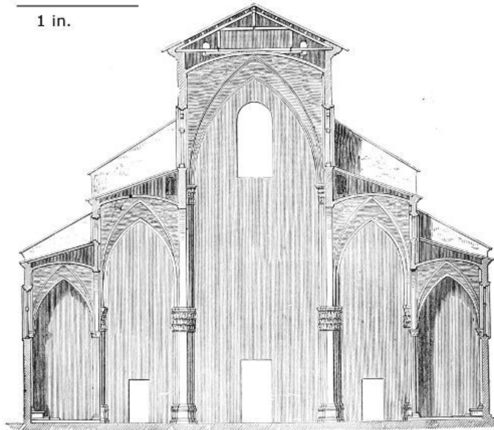
505. Section of San Petronio, Bologna. (From Wiebeking.) Scale 50 ft. to 1 in.
