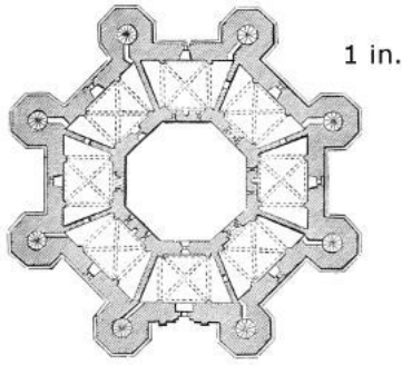
490. Plan of Castel del Monte. (From Schultz.) Scale 100 ft. to 1 in.
