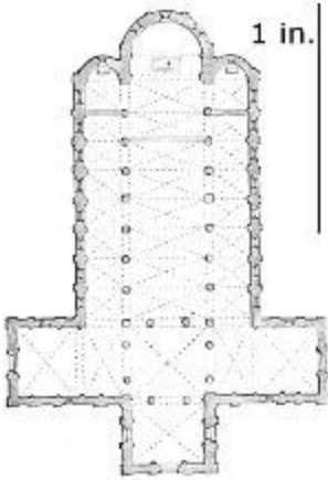
440. Plan of San Antonio, Piacenza. (From Osten. [293] ) Scale 100 ft. to 1 in. [294]
