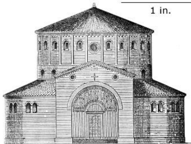
455. Elevation of Duomo at Brescia. (From Hübsch.) Scale 50 ft. to 1 in.
