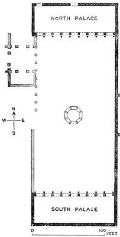
255. Plan of Mosque at Diarbekr.
