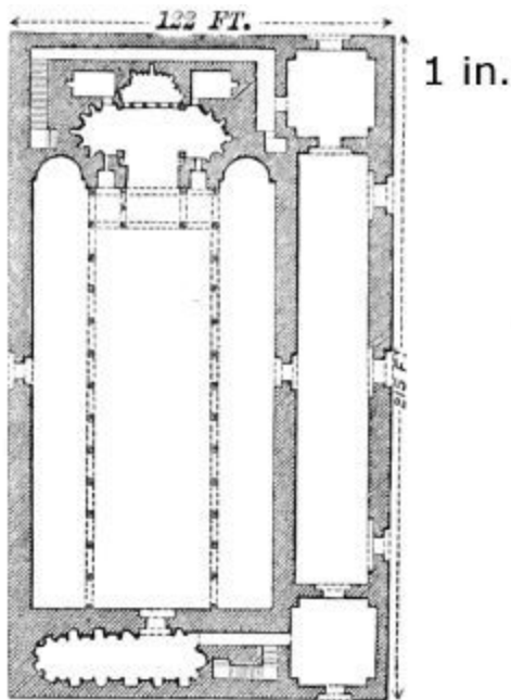
394. White Convent near Siout. (From a Plan by the Hon. Sir Arthur Gordon.) Scale 100 ft. to 1 in.
