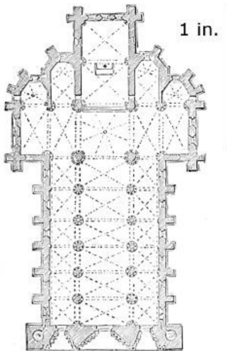
492. Plan of the Church at Vercelli. (From Osten's 'Baukunst in Lombardei.') Scale 100 ft. to 1 in.
