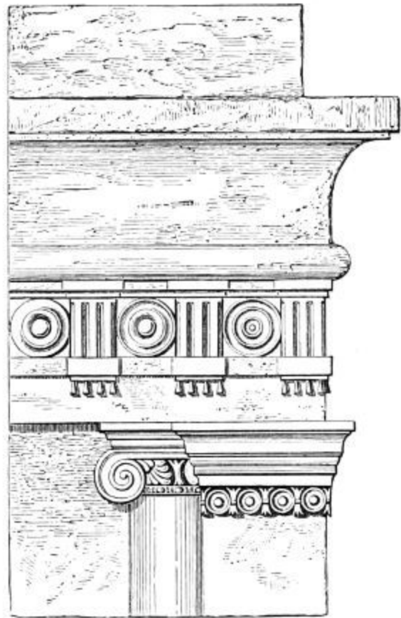
240. Angle of Tomb of Absalom. (From De Saulcy.)
