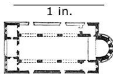
283. Plan of Church at Qalb Louzeh. Scale 100 ft. to 1 in.
