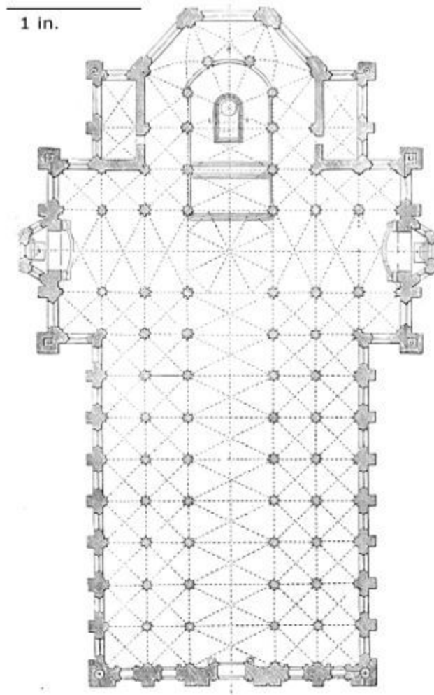
506. Plan of the Cathedral of Milan. (From 'Chiesi Principali d'Europa.') Scale 100 ft. to 1 in.
