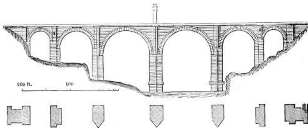
252. Bridge of Trajan, at Alcantara, in Spain.
