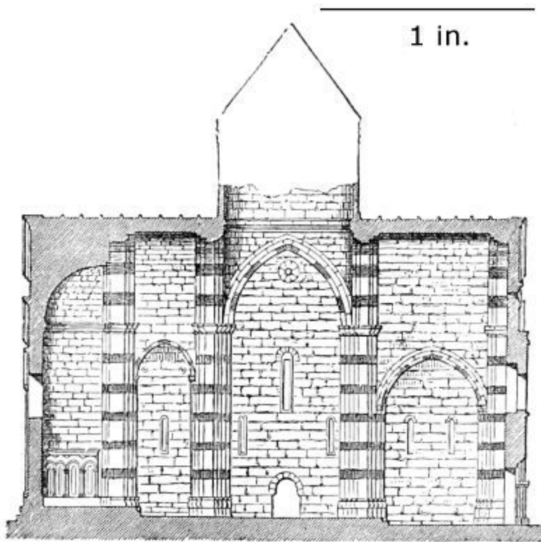
357. Section of Cathedral at Ani. Scale 50 ft. to 1 in.
