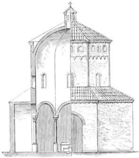
433. Half Section, half Elevation, of the Baptistery at Novara. (From Osten.) No scale.
