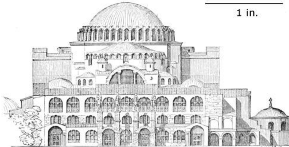
316. Elevation Façade of Sta. Sophia at Constantinople. (From Salzenberg.) Scale 100 ft. to 1 in.
