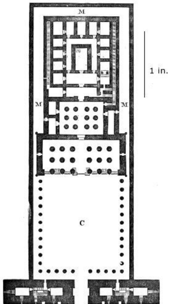
37. Plan of Temple at Edfû, Apollinopolis Magna. Scale 100 ft. to 1 in.
