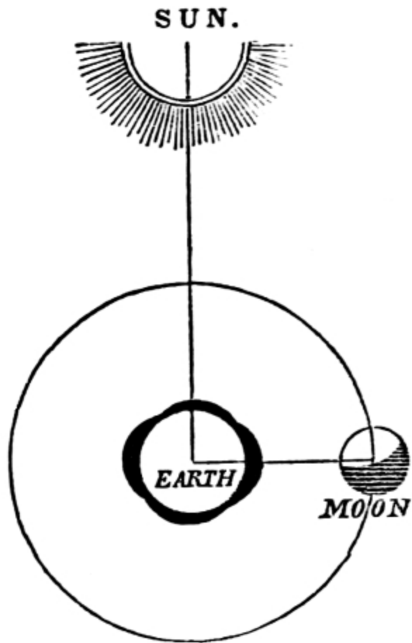
MOON'S ORBIT.
