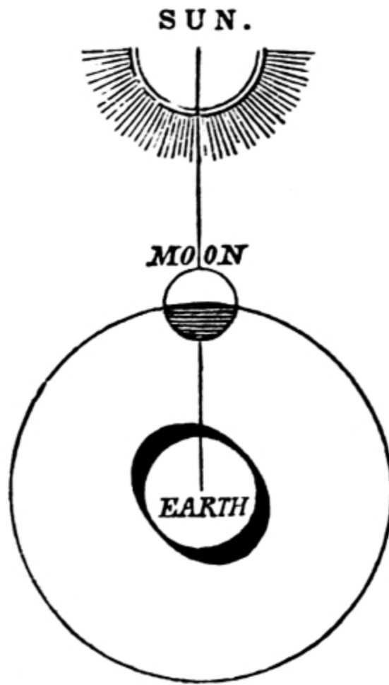
MOON'S ORBIT.
