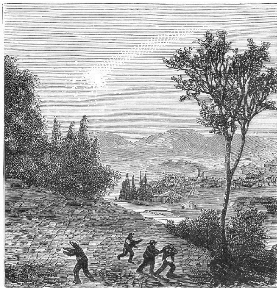
Fig. 48.—Explosion of a Bolide.
