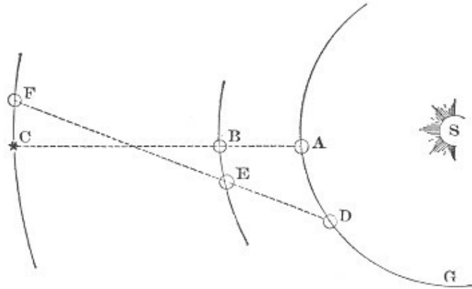
Fig. 47.—Illustrating Movements of a Superior Planet.
