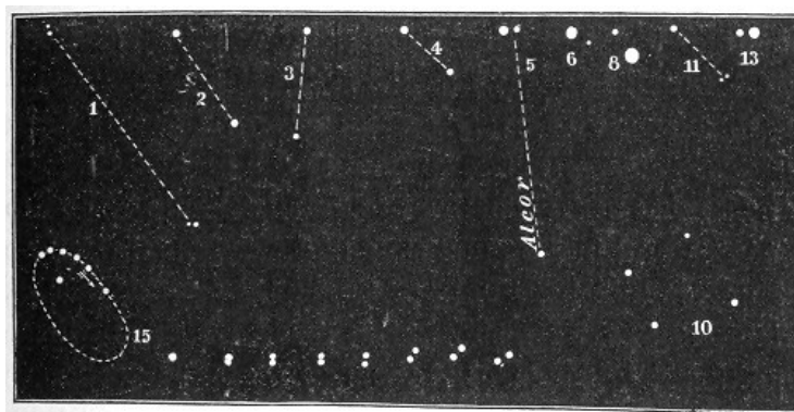
Fig. 75.—Aspects and Revolution of Double Stars.
