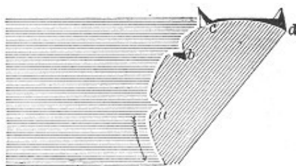
Fig. 59.—Illumination of Craters and Peaks.
