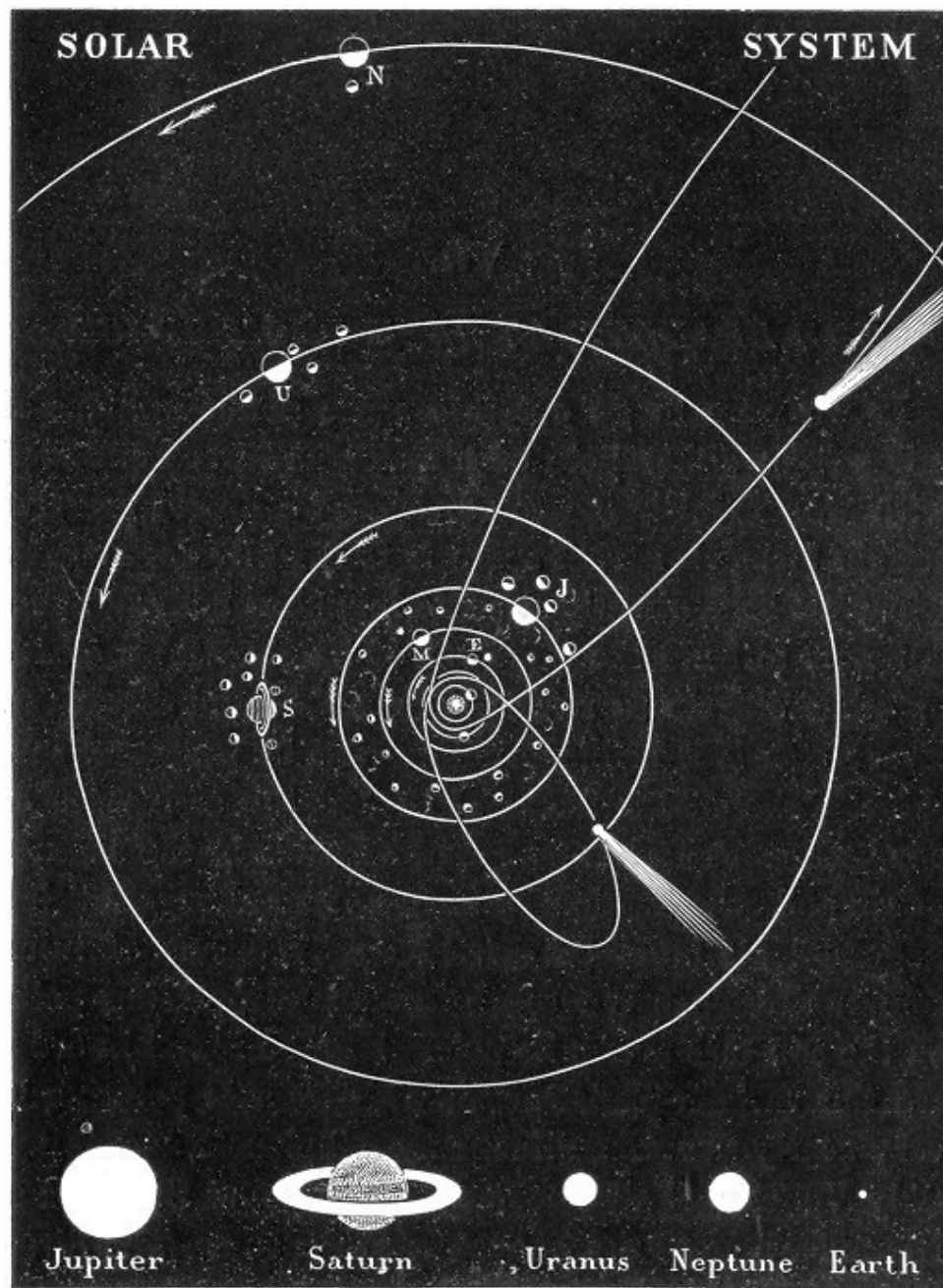
Fig. 38.—Orbits and Comparative Sizes of the Planets.
