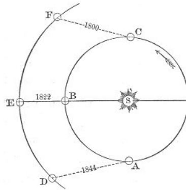
Fig. 66.—Perturbation of Uranus.
