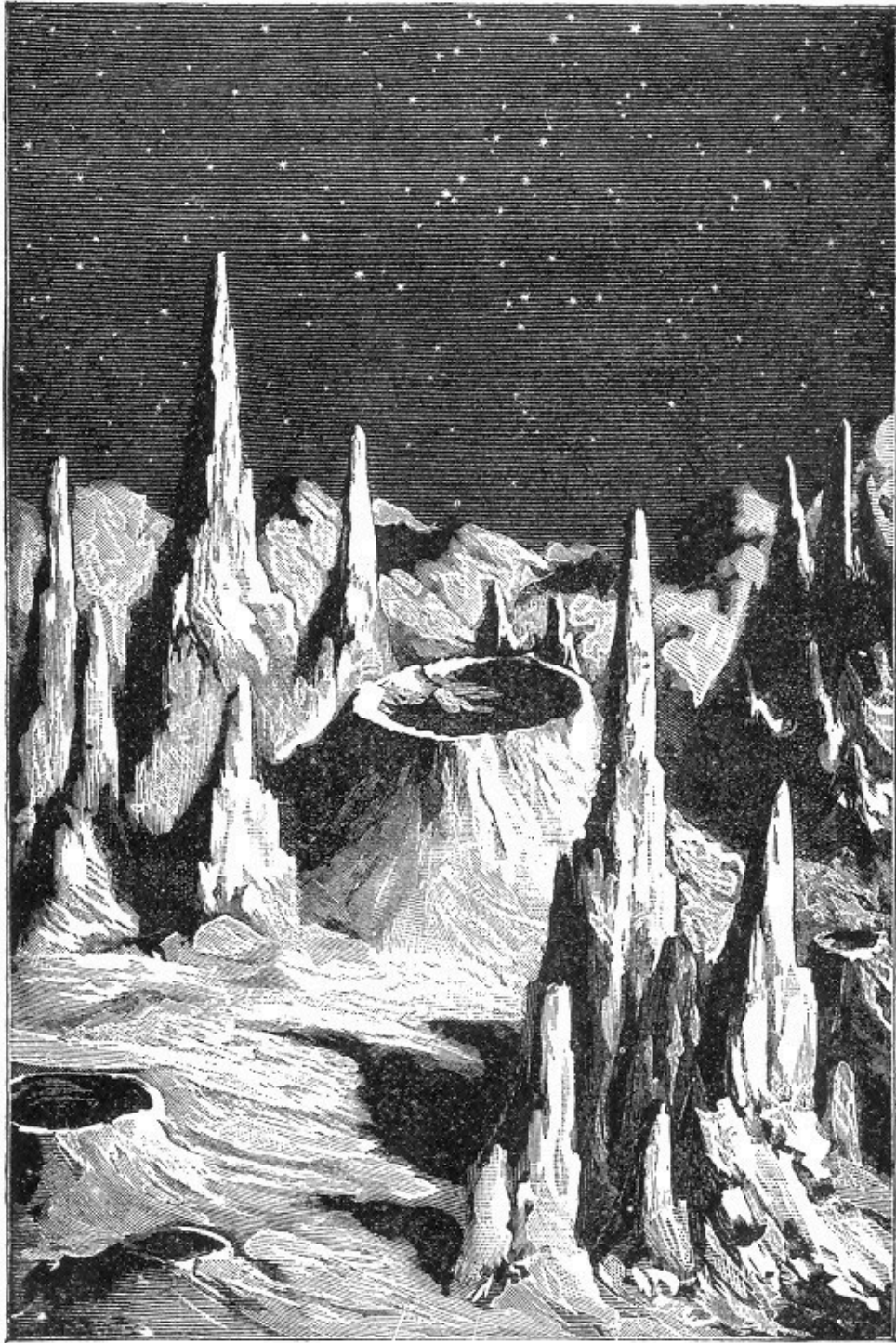
Fig. 57.—Lunar Day.
