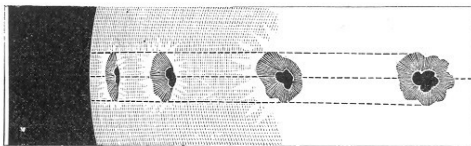
Fig. 35.—Change in Spots as rotated across the Disk, showing Cavities.
