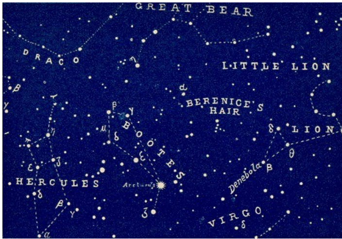
Fig. 71.—Arcturus comes to the Meridian, 70^\circ from the Pole, at 10 o'clock May 25th, 9 o'clock June 9th, and at 8 o'clock June 25th.
