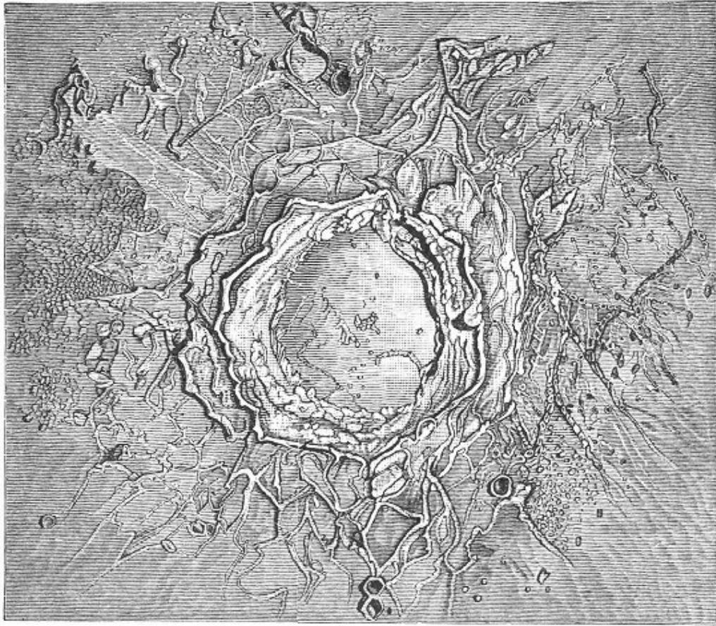
Fig. 60.—Lunar Crater "Copernicus," after Secchi.
