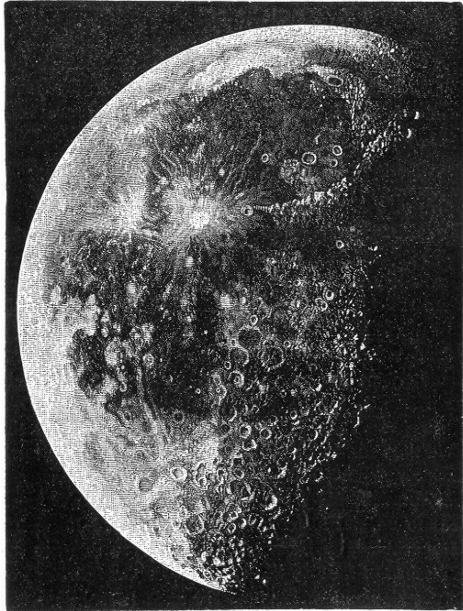
Fig. 58.—View of the Moon near the Third Quarter. From a Photograph by Professor Henry Draper.
