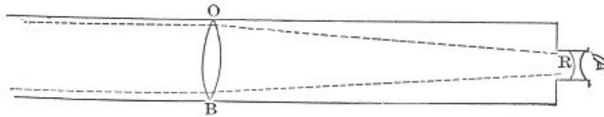
Fig. 13.—Refracting Telescope.
