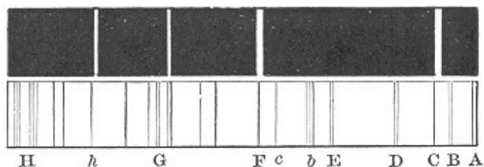
Fig. 18.—Spectra of glowing Hydrogen and the Sun.
