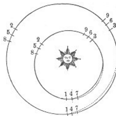
Fig. 3.—Changes of orbit by mutual attraction.
