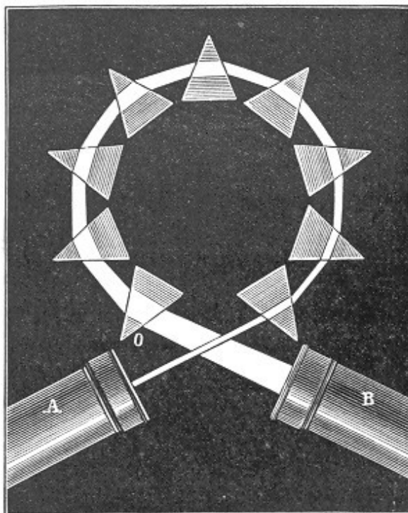
Fig. 17.—Spectroscope, with Battery of Prisms.
