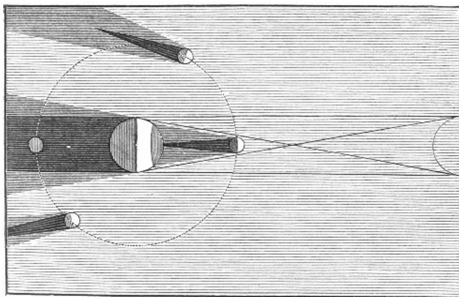
Fig. 61.—Eclipses; Shadows of Earth and Moon.
