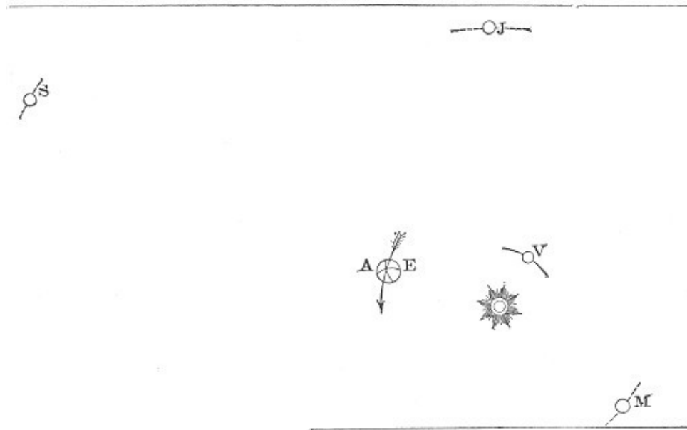
Fig. 45. Showing Position of Planets.
