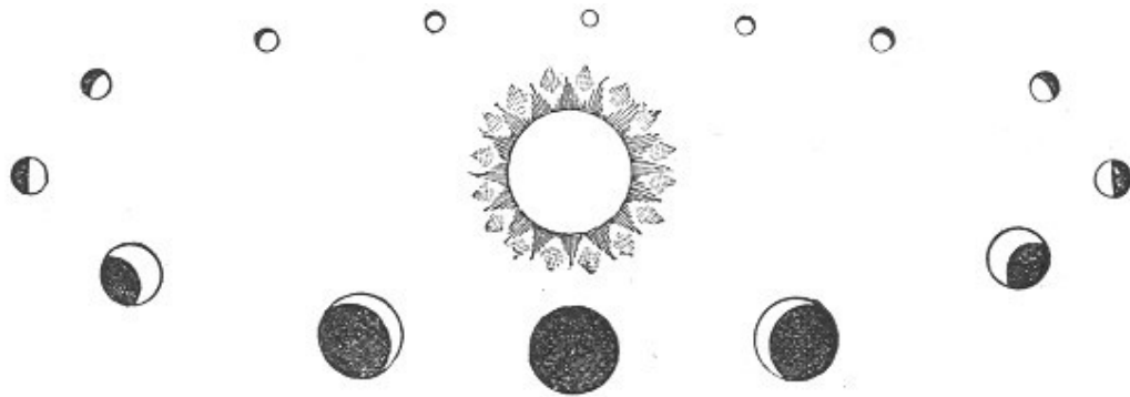
Fig. 53.—Phases of Venus, and Various Apparent Dimensions.
