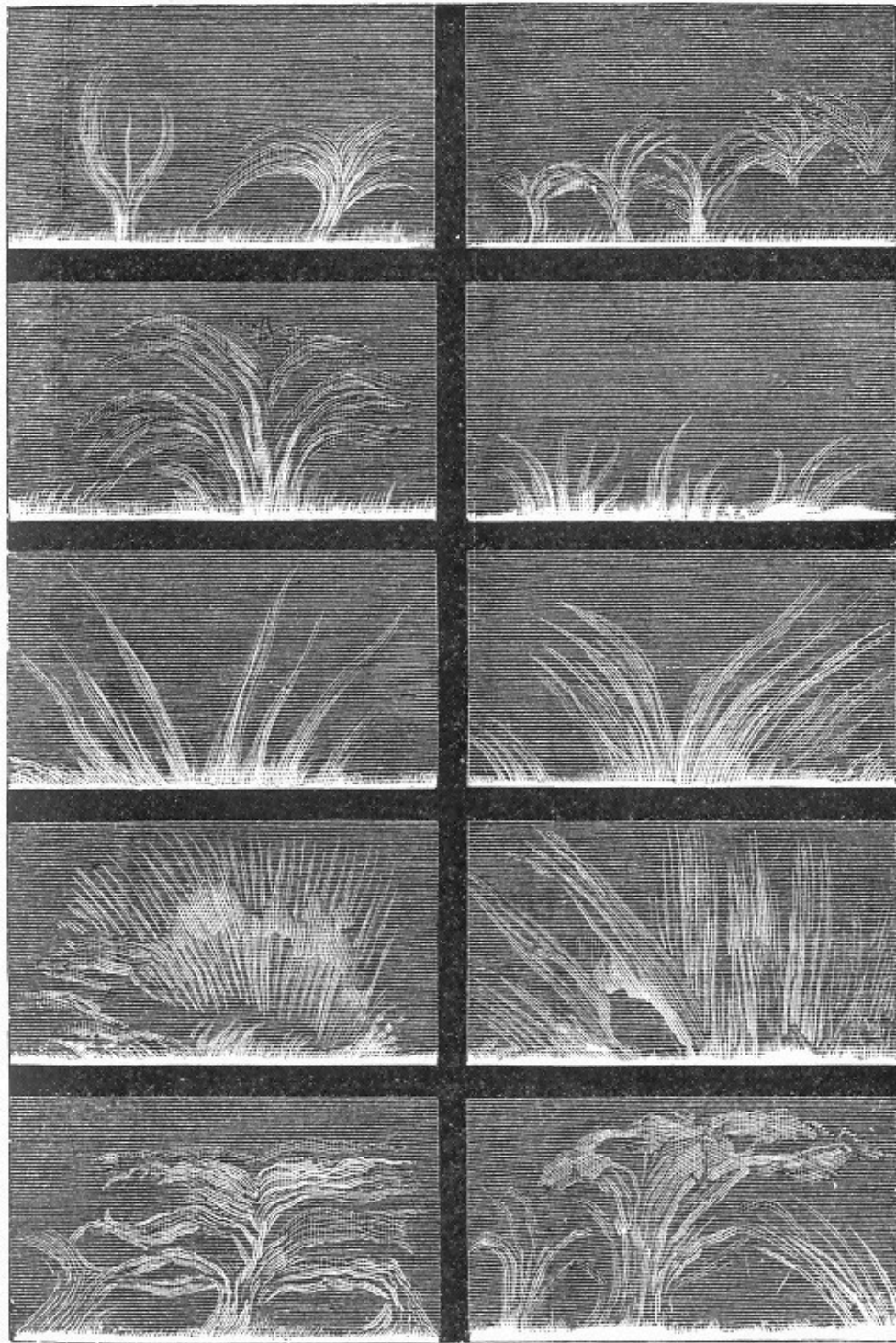
Fig. 34.—Solar Prominences of Flaming Hydrogen.
