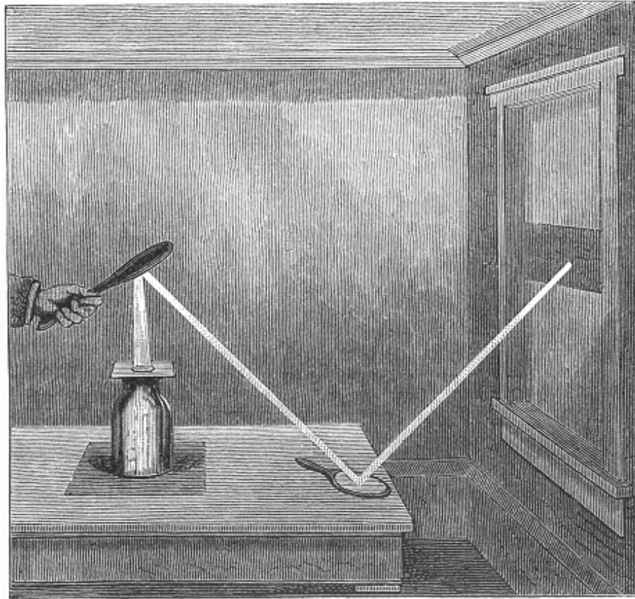
Fig. 9.—Reflection and Diffusion of Light.
