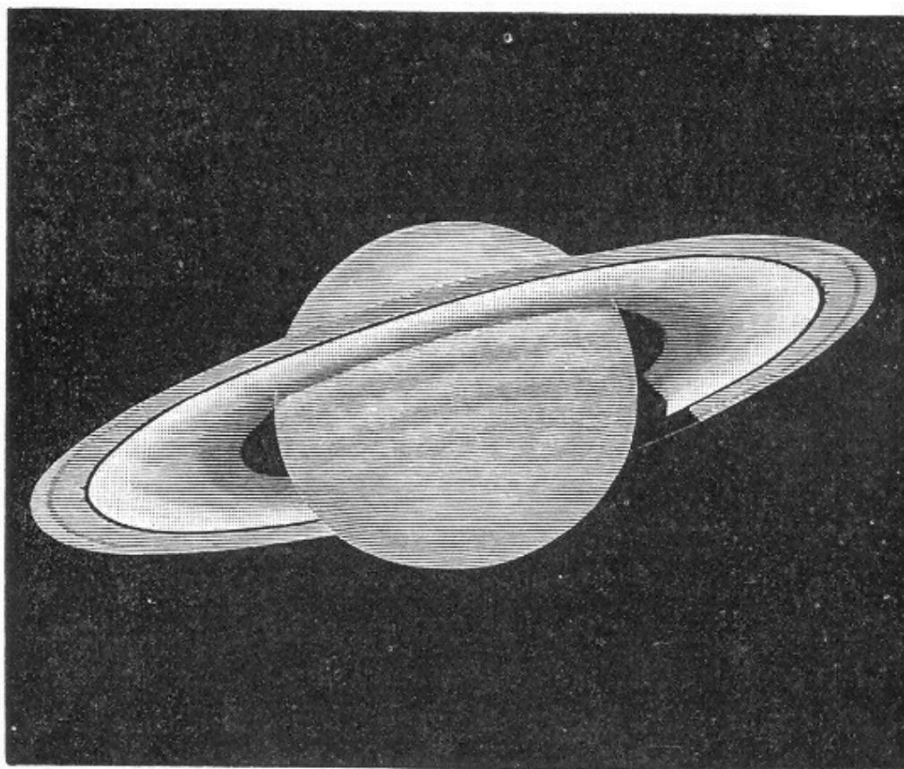
Fig. 65.—View of Saturn and his Rings.
