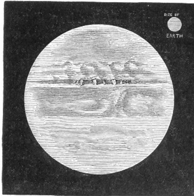
Fig. 63.—Jupiter as seen by the great Washington Telescope. Drawn by Mr. Holden.
