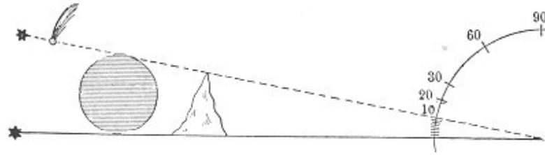
Fig. 20.—Illustration of Angles.
