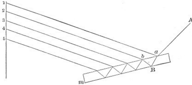
Fig. 10.—Manifold Reflections.
