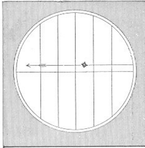
Fig. 23.—Transit of a Star noted.
