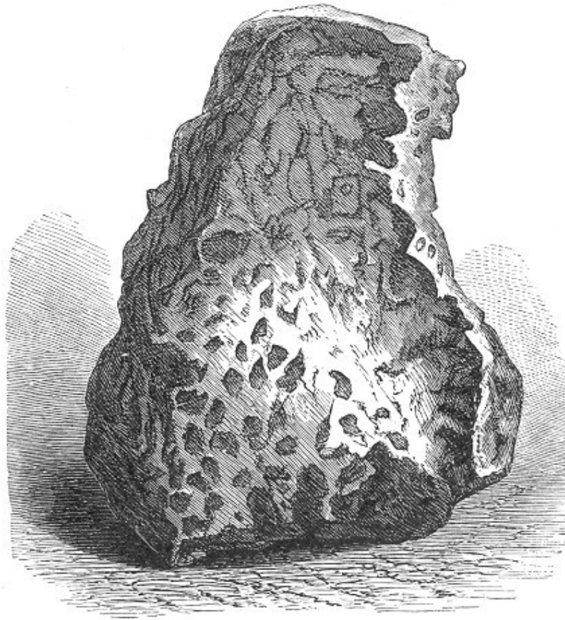
Fig. 50.—Santa Rosa Aerolite.
