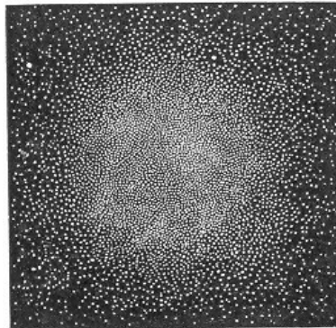
Fig. 77.—Globular Cluster.
