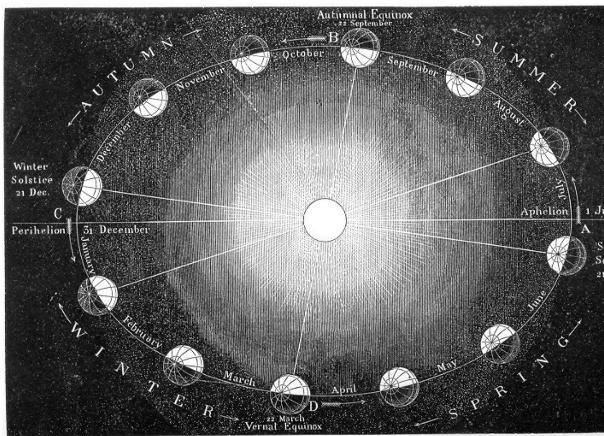
Fig. 39.—Orbit of Earth, showing Parallelism of Axis and Seasons.
