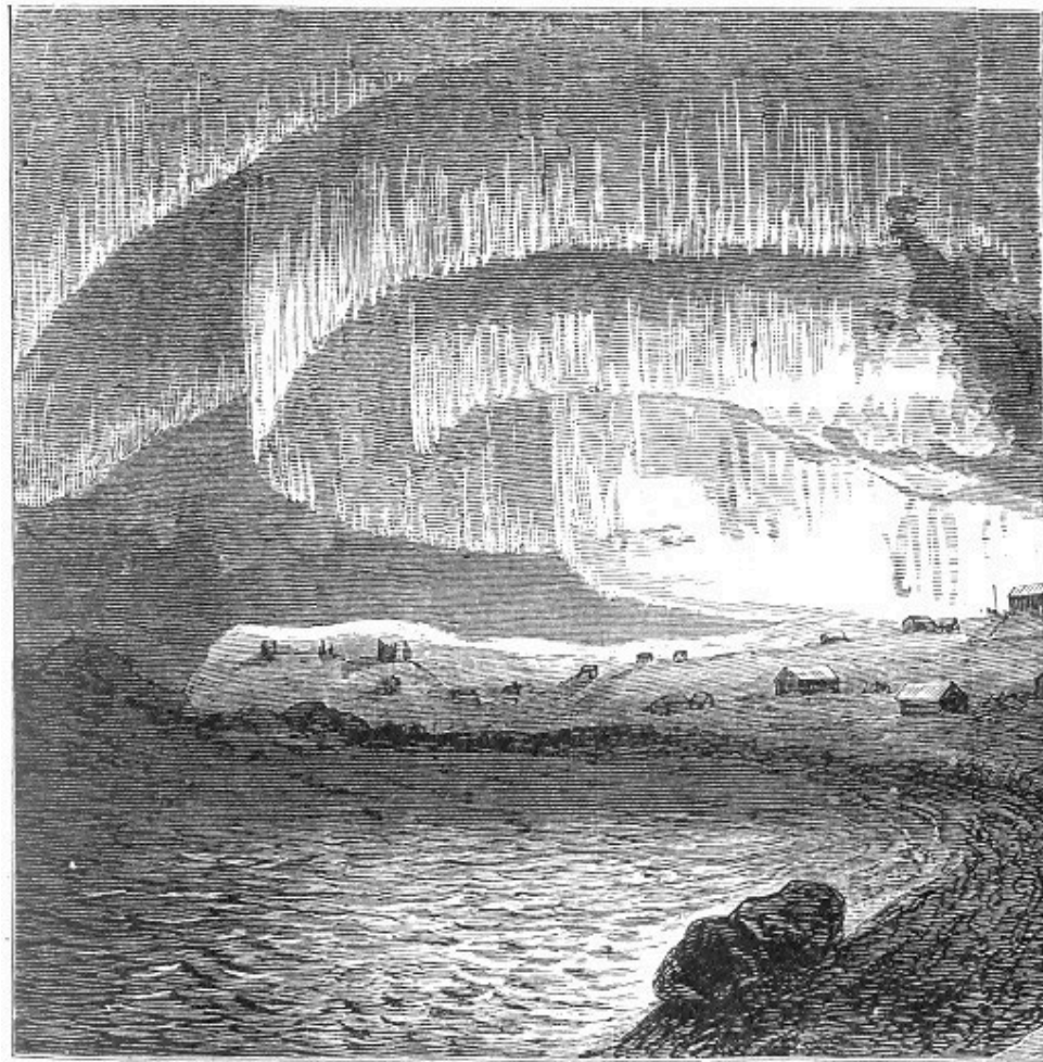
Fig. 55.—The Aurora as Waving Curtains.
