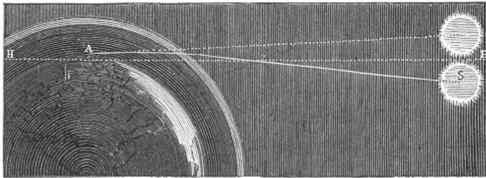
Fig. 12.—Atmospherical Refraction.
