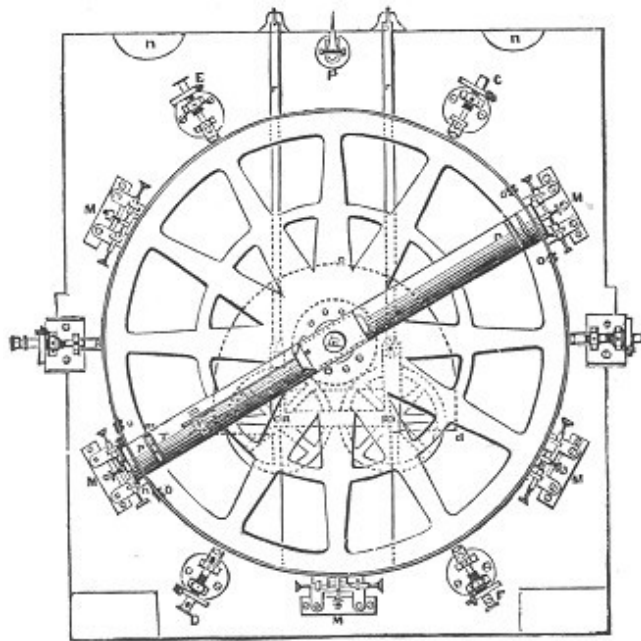
Fig. 21.—Mural Circle.
