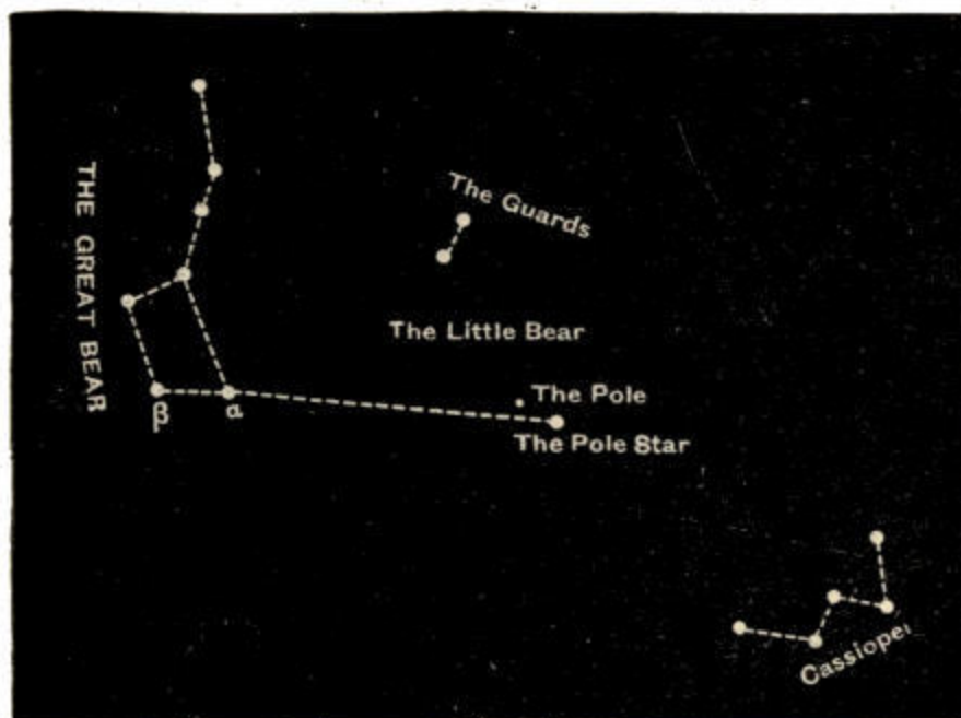
Fig. 81.—The Great Bear and Cassiopeia.
