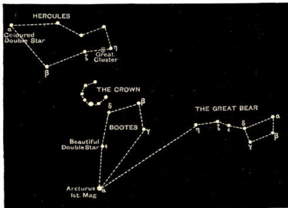
Fig. 88.—Boötes and the Crown.
