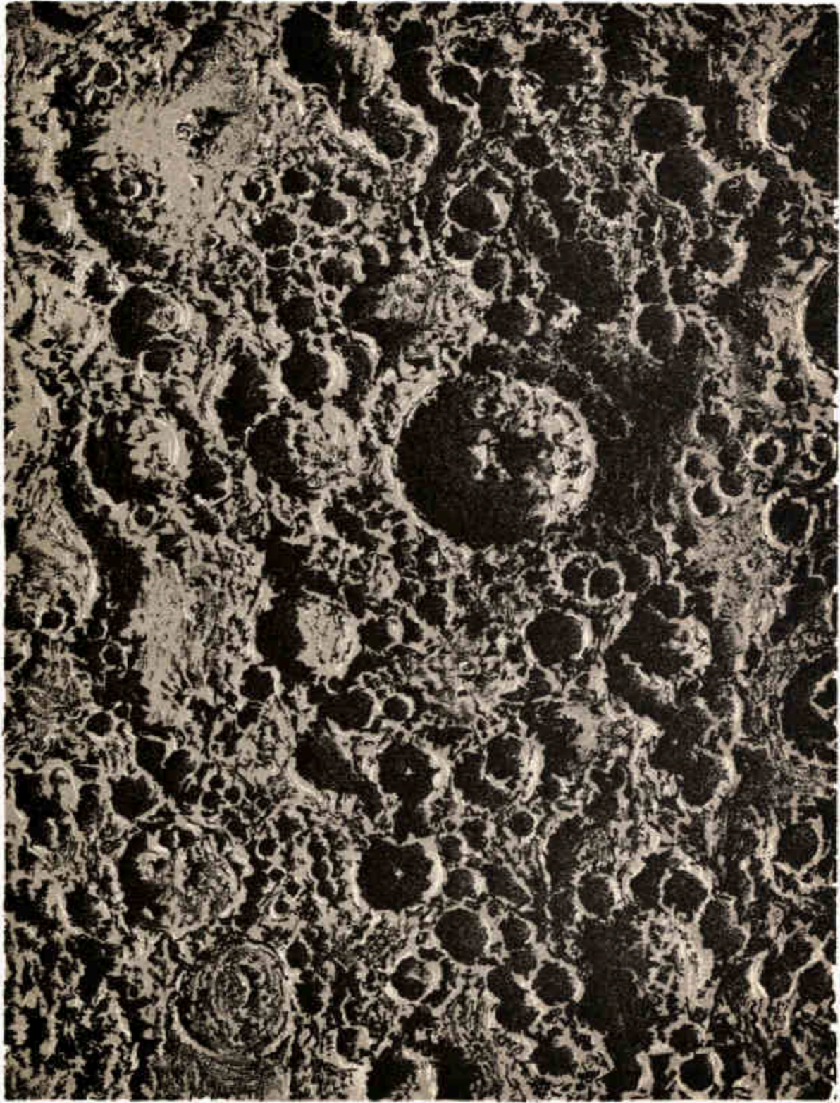
PLATE X. TYCHO AND ITS SURROUNDINGS. (AFTER NASMYTH.)
