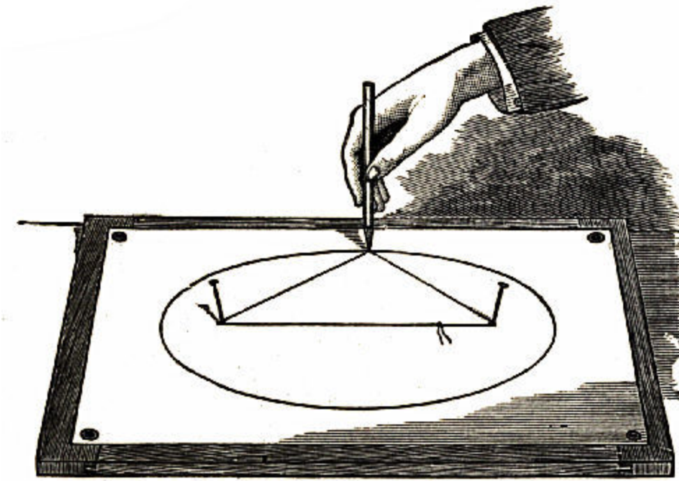
Fig. 37.—Drawing an Ellipse.
