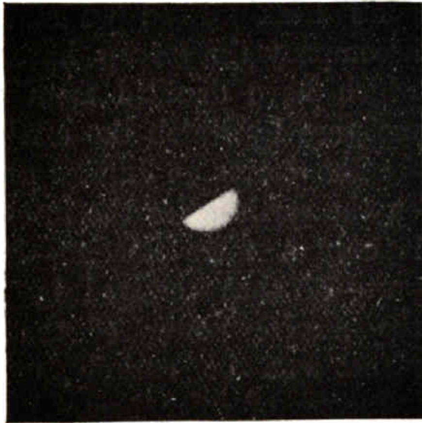
Fig. 60.—The Occultation of Jupiter (4).
