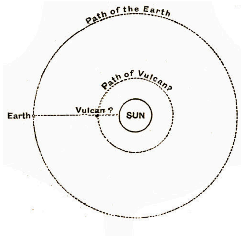
Fig. 40.—The Transit of the Planet of Romance.
