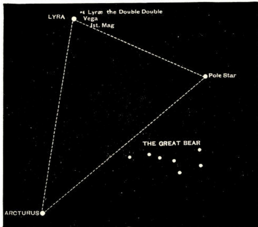
Fig. 90.—The Constellation of Lyra.
