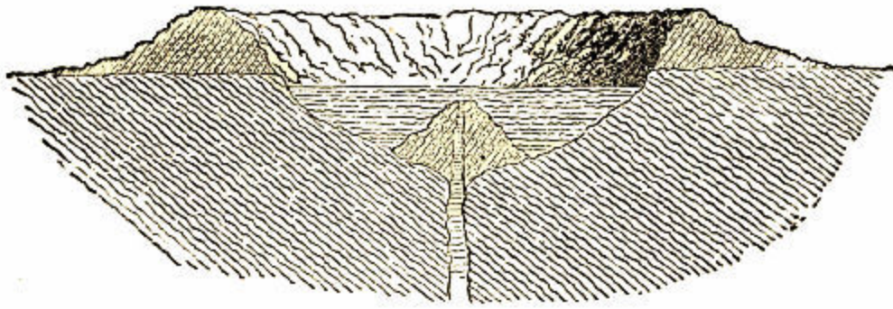
Fig. 30.—Formation of the Level Floor by Lava.
