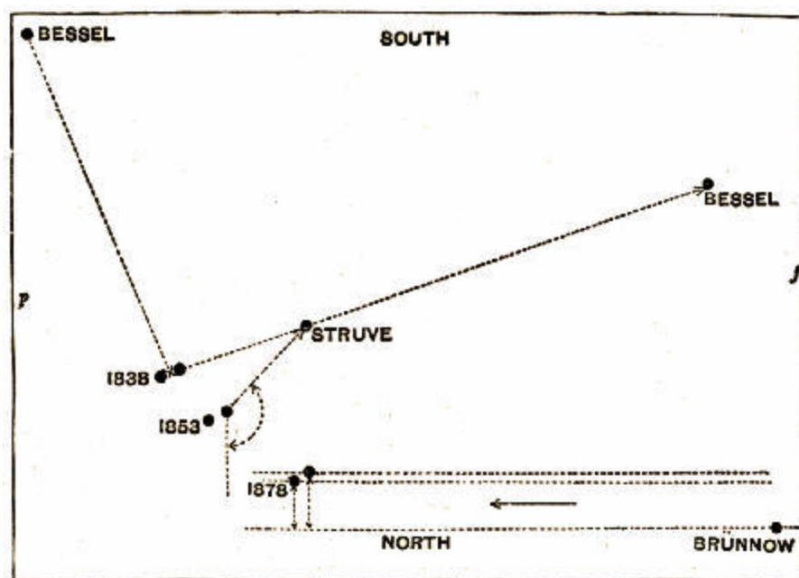
Fig. 94.—61 Cygni and the Comparison Stars.
