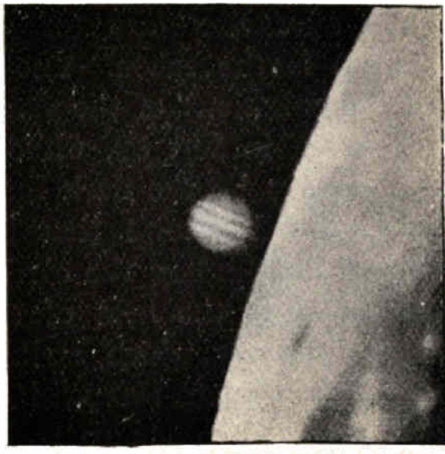
Fig. 58.—The Occultation of Jupiter (2).
