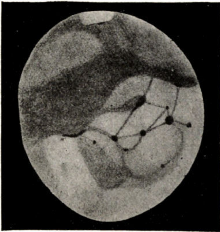
Fig. 51.—Drawing of Mars (July 30th, 1894).
