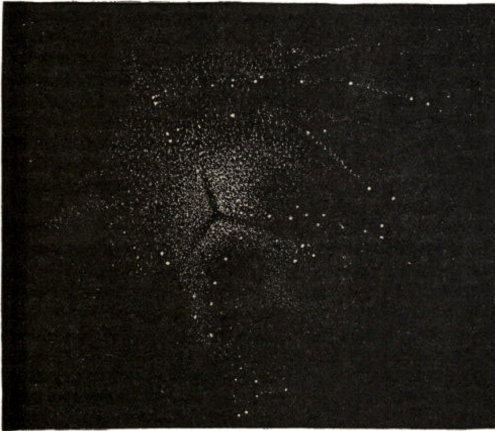
Fig. 96.—The Globular Cluster in Hercules.
