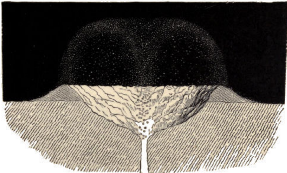
Fig. 28.—Volcano in Activity.
