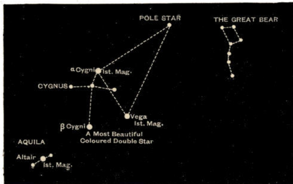
Fig. 91.—Vega, the Swan, and the Eagle.
