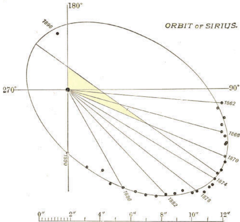
Fig. 92.—The Orbit of Sirius (Professor Burnham).
