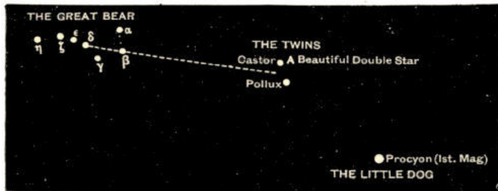
Fig. 86.—Castor and Pollux.
