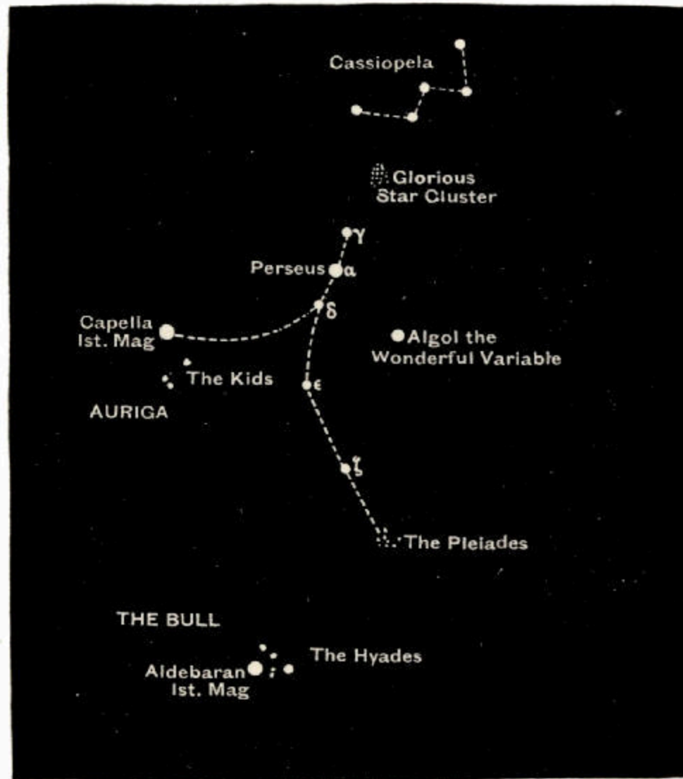
Fig. 83.—Perseus and its Neighbouring Stars.
