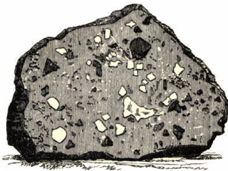
Fig. 79.—Section of the Chaco Meteorite.
