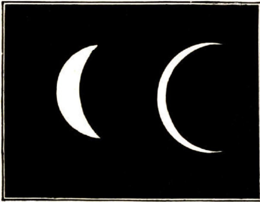
Fig. 42.—Mercury as a Crescent.
