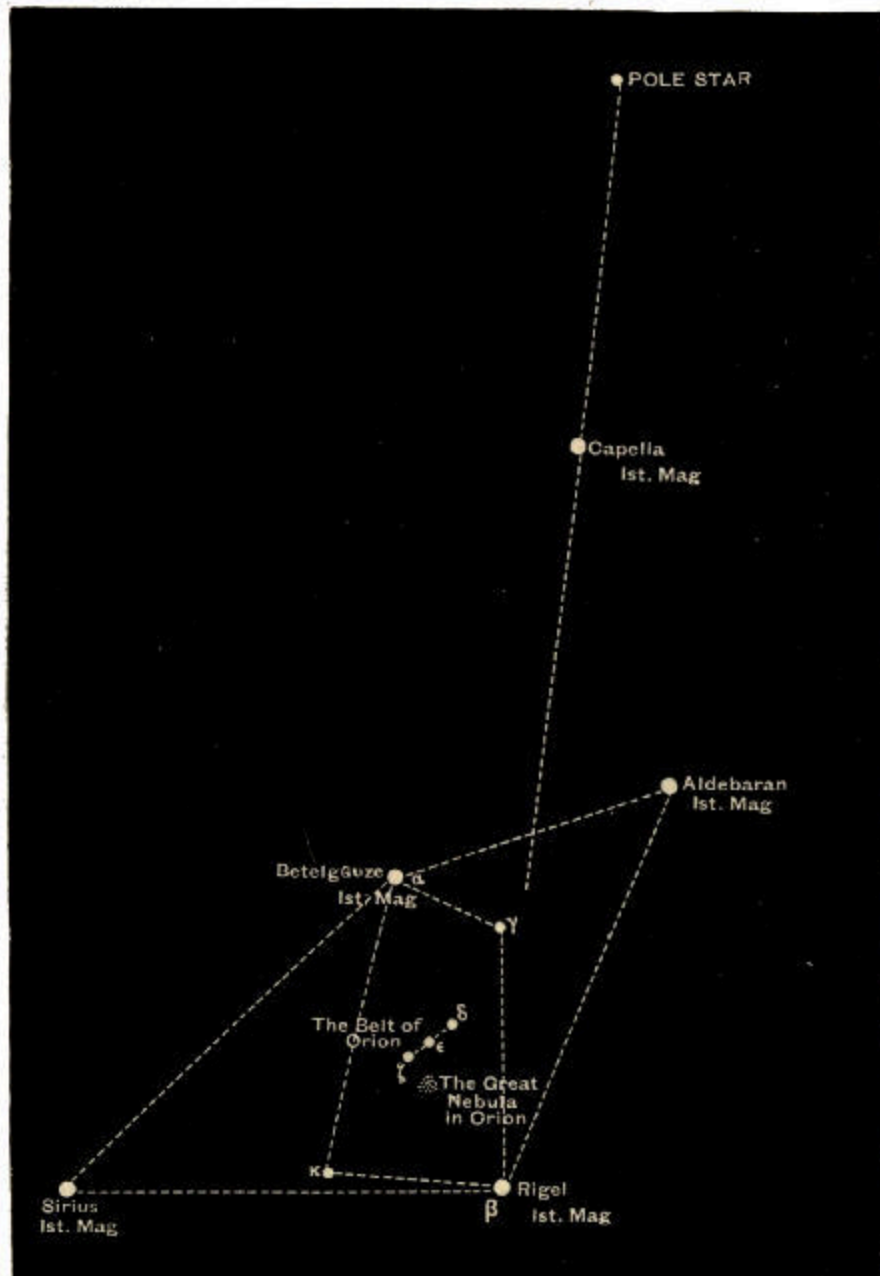
Fig. 85.—Orion, Sirius, and the Neighbouring Stars.
