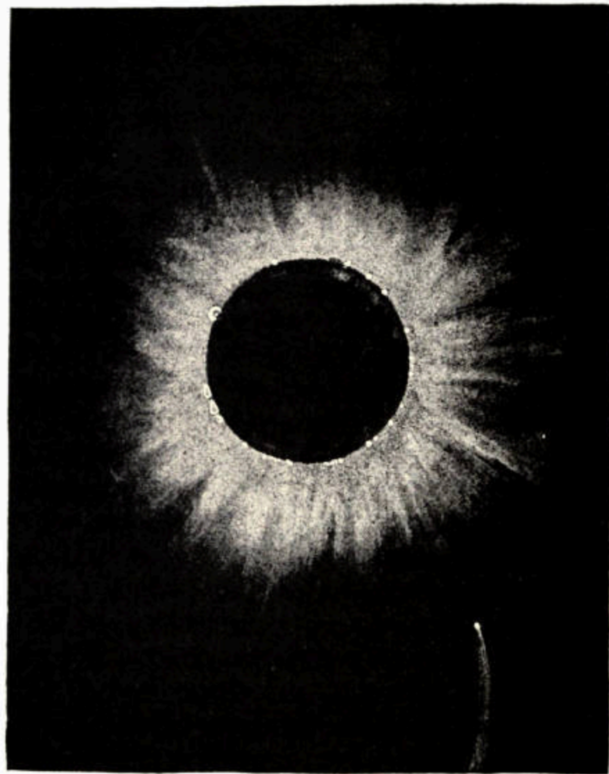
Fig. 20.—View of the Corona (and a Comet) in a Total Eclipse.
