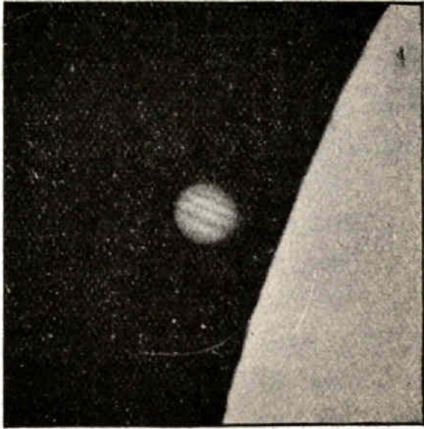
Fig. 57.—The Occultation of Jupiter (1).
