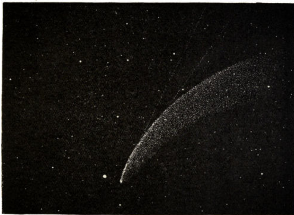
Fig. 73.—Tails of the Comet of 1858.
