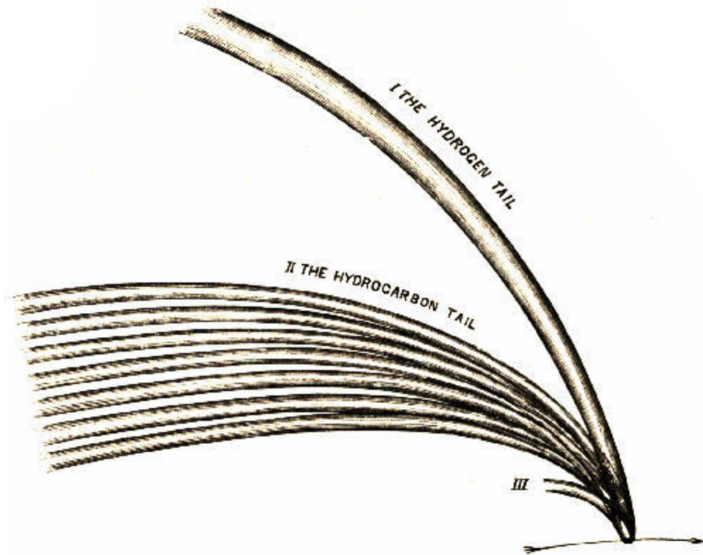
Fig. 72.—Bredichin's Theory of Comets' Tails.
