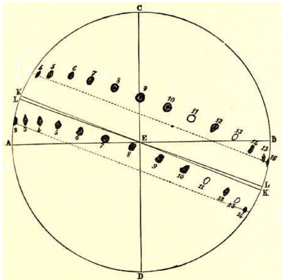
Fig. 14.—Scheiner's Observations on Sun-spots.
