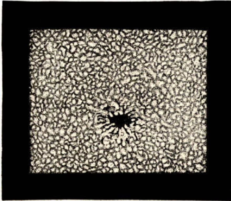
Fig. 16.—The Texture of the Sun and a small Spot.
