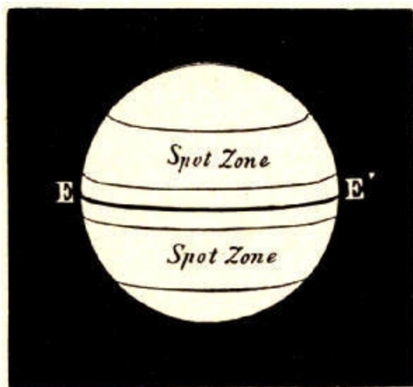
Fig. 15.—Zones on the Sun's Surface
