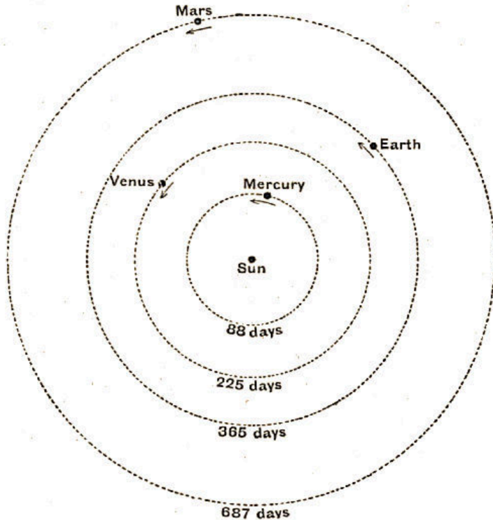
Fig. 31.—The Orbits of the Four Interior Planets.
