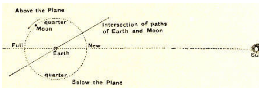
Fig. 24.—The Moon's Path around the Sun.
