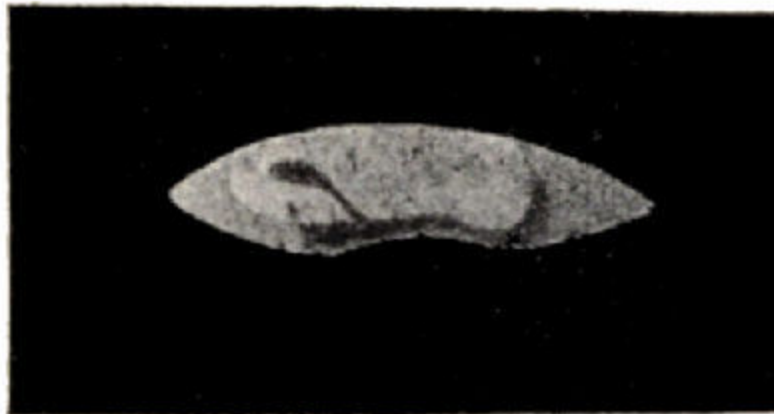
Fig. 54.—The Southern Polar Cap on Mars (July 1, 1894).
