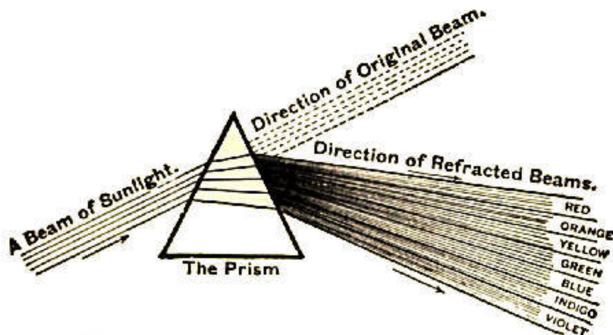
Fig. 18.—Dispersion of Light by the Prism.
