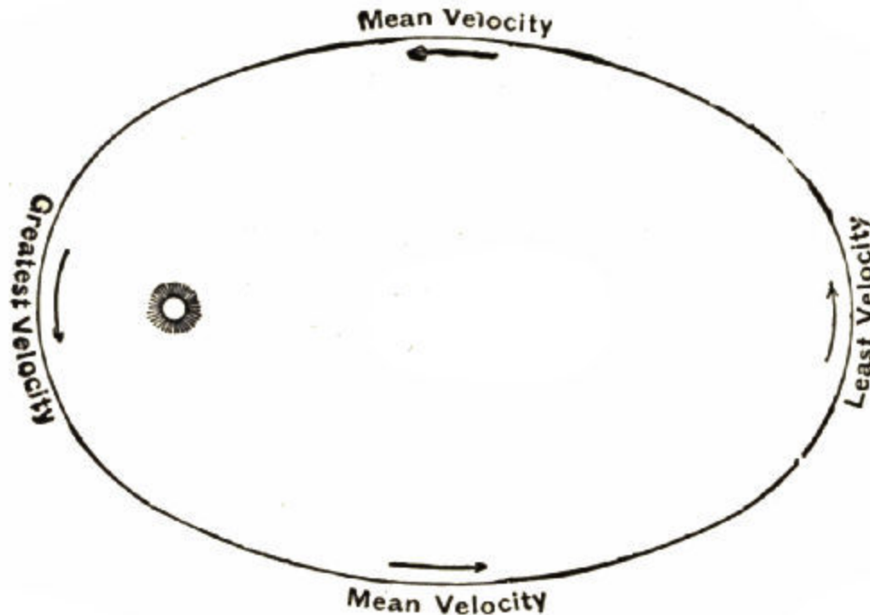
Fig. 38.—Varying Velocity of Elliptic Motion.
