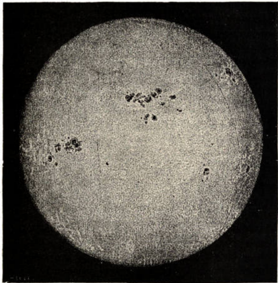
Fig. 11.—The Sun, photographed on September 22, 1870.
