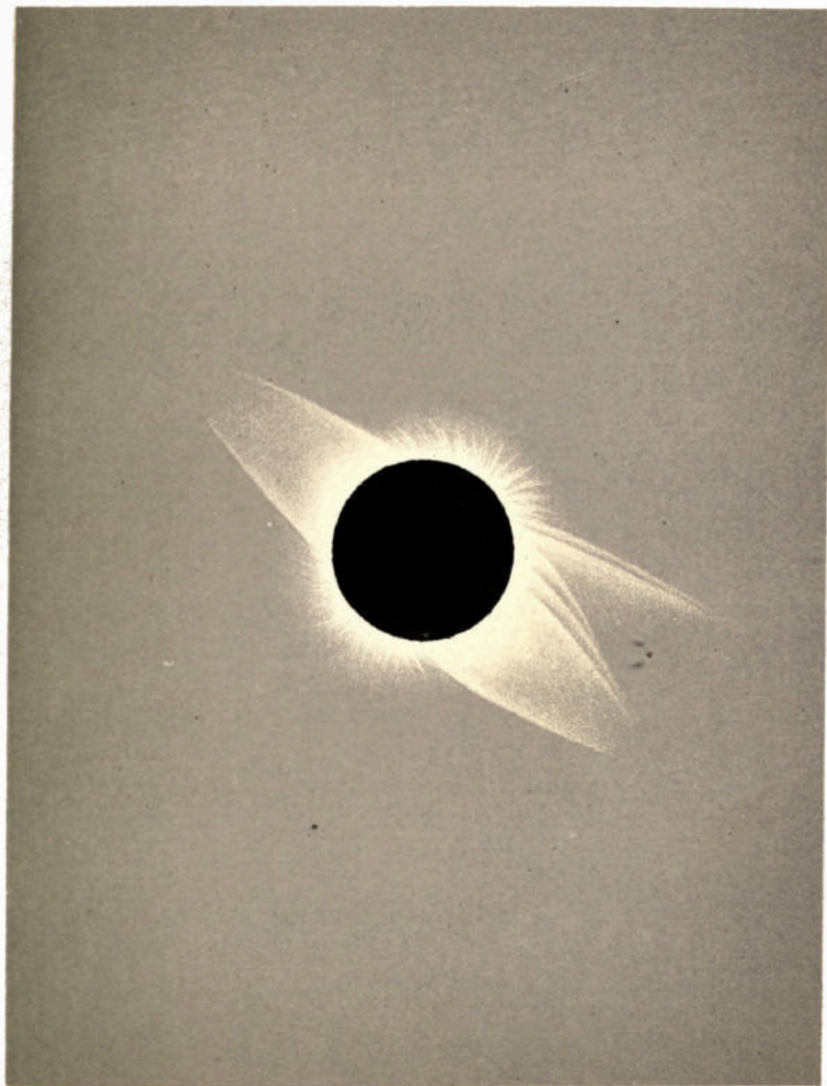
PLATE V. TOTAL SOLAR ECLIPSE, JULY 29TH, 1878.
