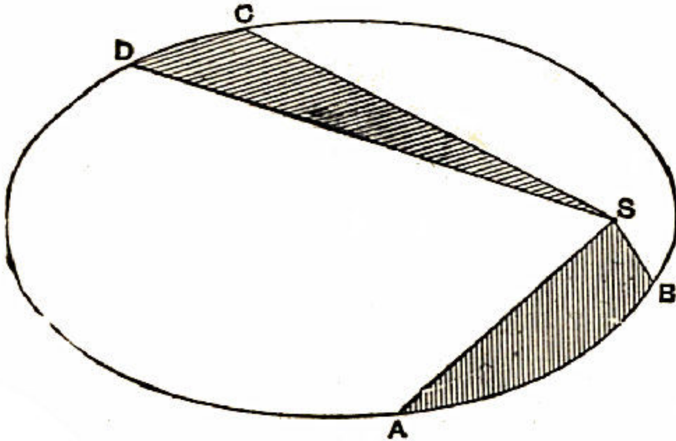
Fig. 39.—Equal Areas in Equal Times.
