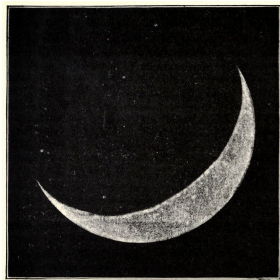
Fig. 43. Venus, May 29th, 1889.
