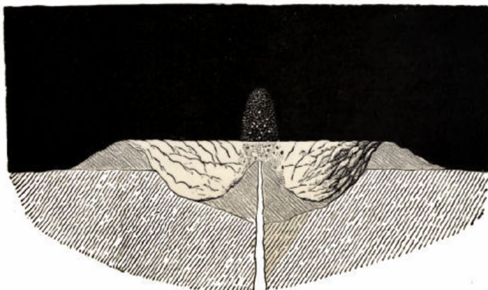
Fig. 29.—Subsequent Feeble Activity.
