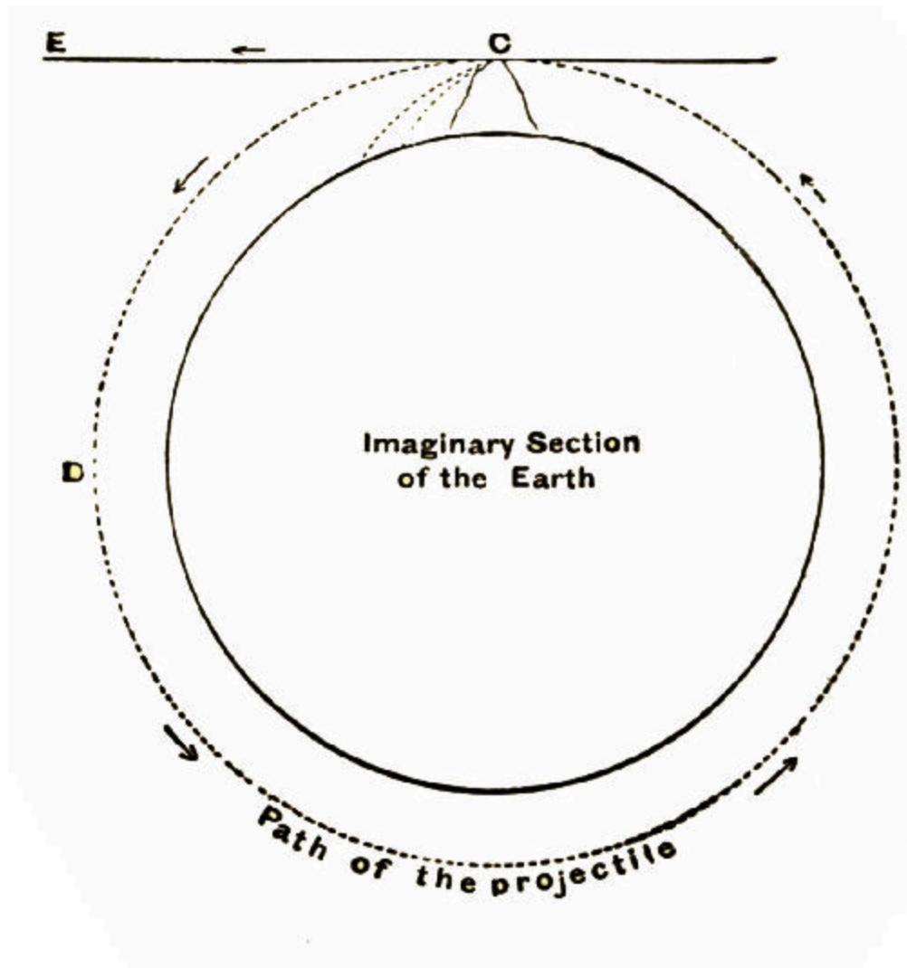
Fig. 36.—Illustration of the Moon's Motion.
