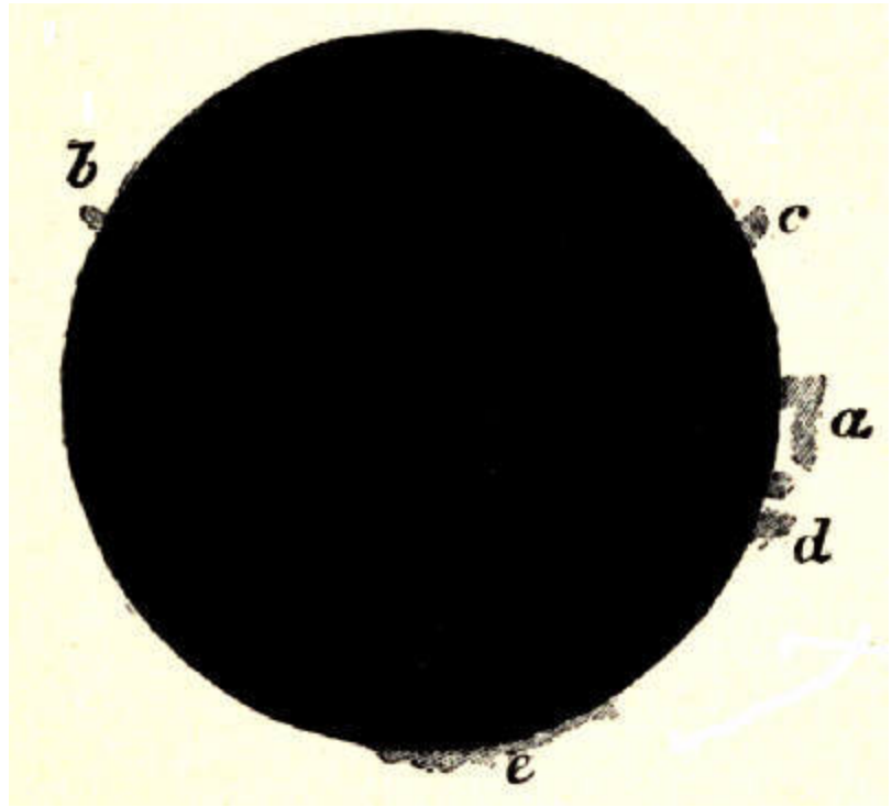
Fig. 19.—Prominences seen in Total Eclipse.
