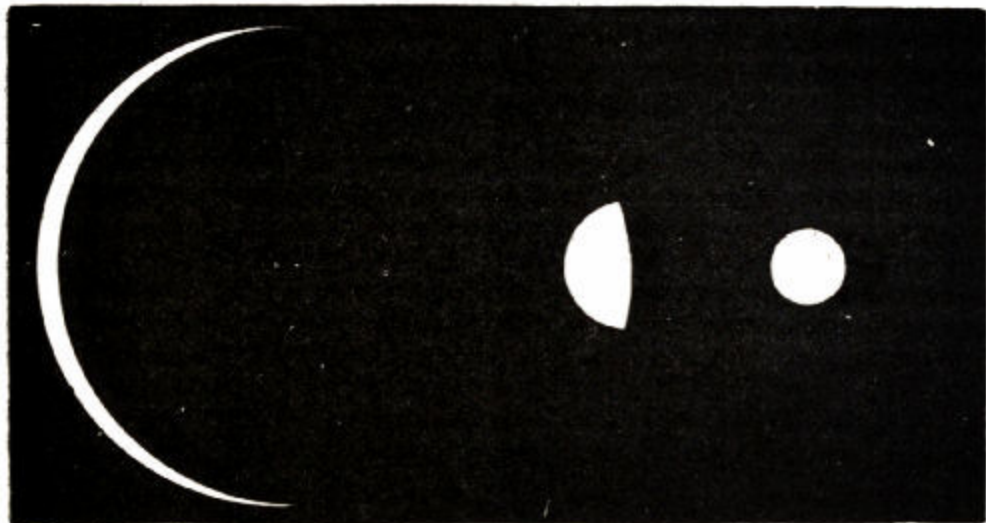
Fig. 44.—Different Aspects of Venus in the Telescope.
