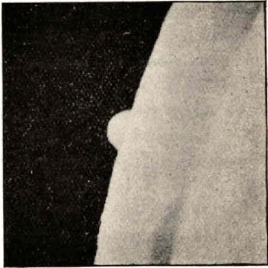
Fig. 59.—The Occultation of Jupiter (3).
