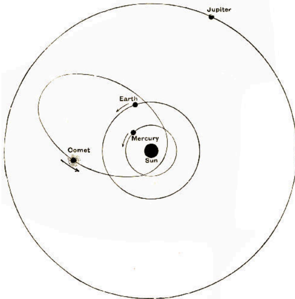
Fig. 70.—The Orbit of Encke's Comet.
