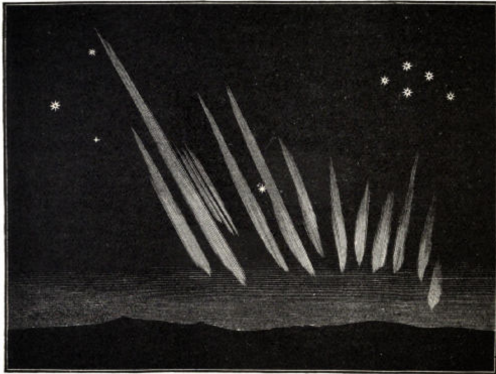
Fig. 74.—The Comet of 1744.
