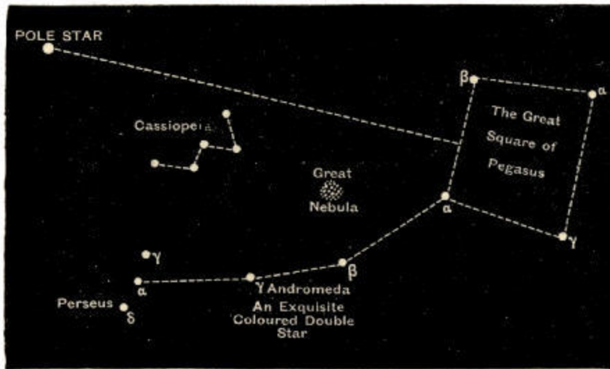
Fig. 82.—The Great Square of Pegasus.
