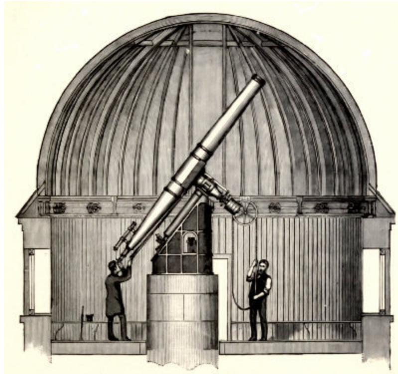
Fig. 3.—Section of the Dome of Dunsink Observatory.
