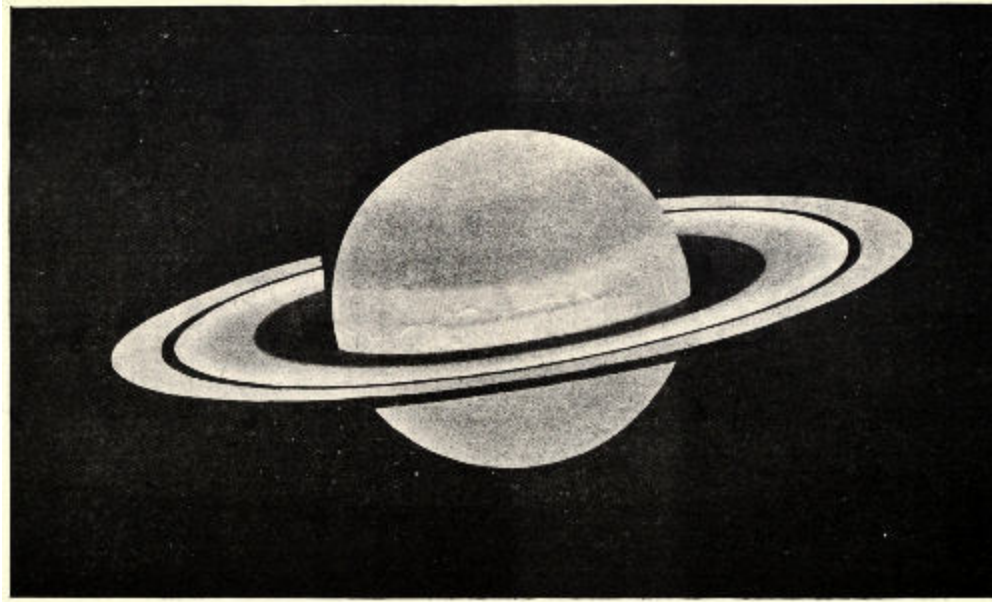
Fig. 64. Saturn. (July 2nd, 1894. 36-in. equatorial.) (Prof. E.E. Barnard.)
