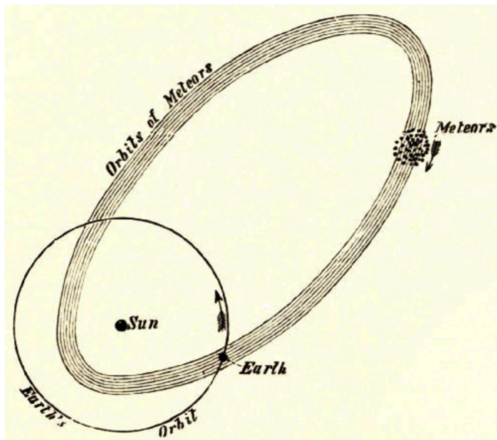
Fig. 76.—The Orbit of a Shoal of Meteors.
