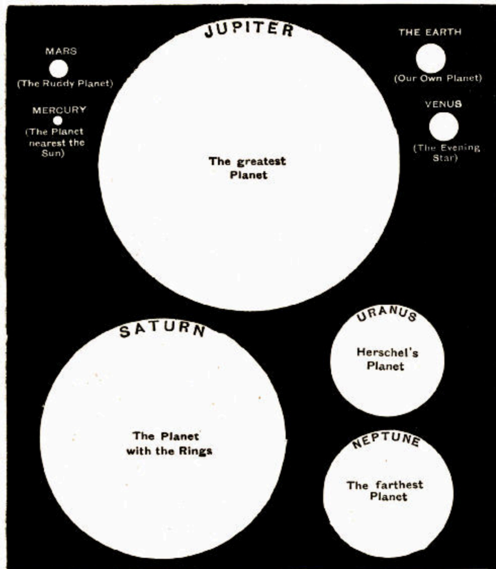
Fig. 35.—Comparative Sizes of the Planets.
