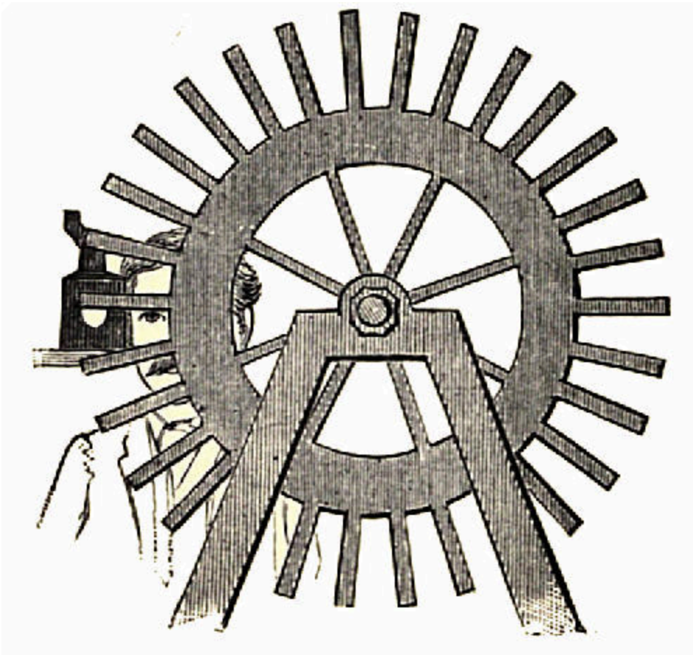
Fig. 63.—Mode of Measuring the Velocity of Light.
