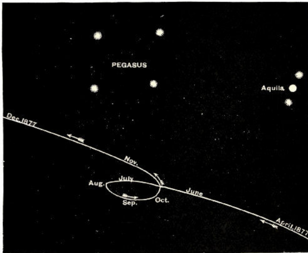
Fig. 49.—The Apparent Movements of Mars In 1877.
