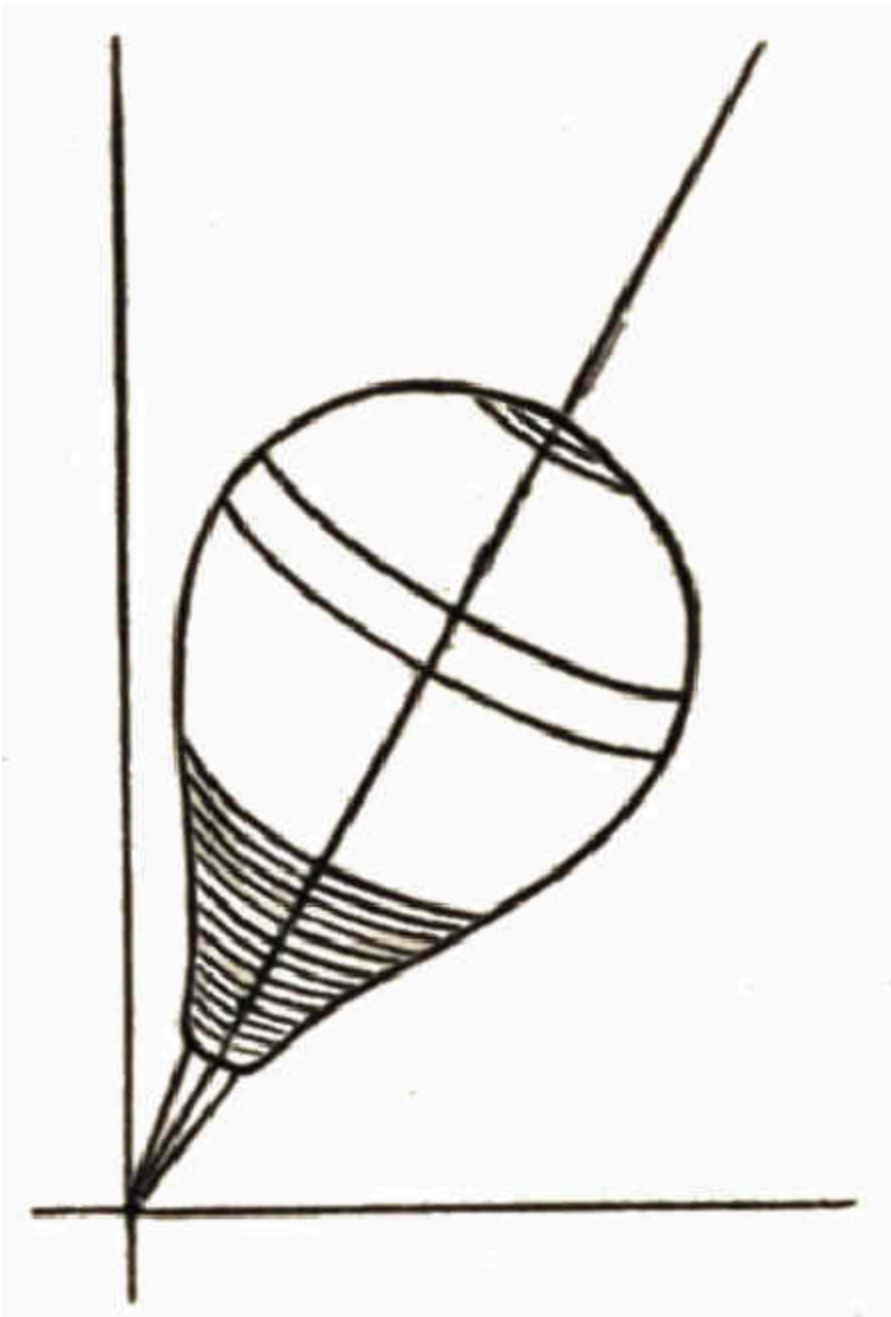
Fig. 101.—Illustration of the Motion of Precession.
