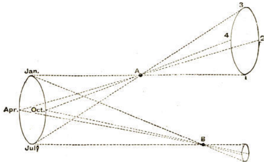
Fig. 93.—The Parallaxic Ellipse.
