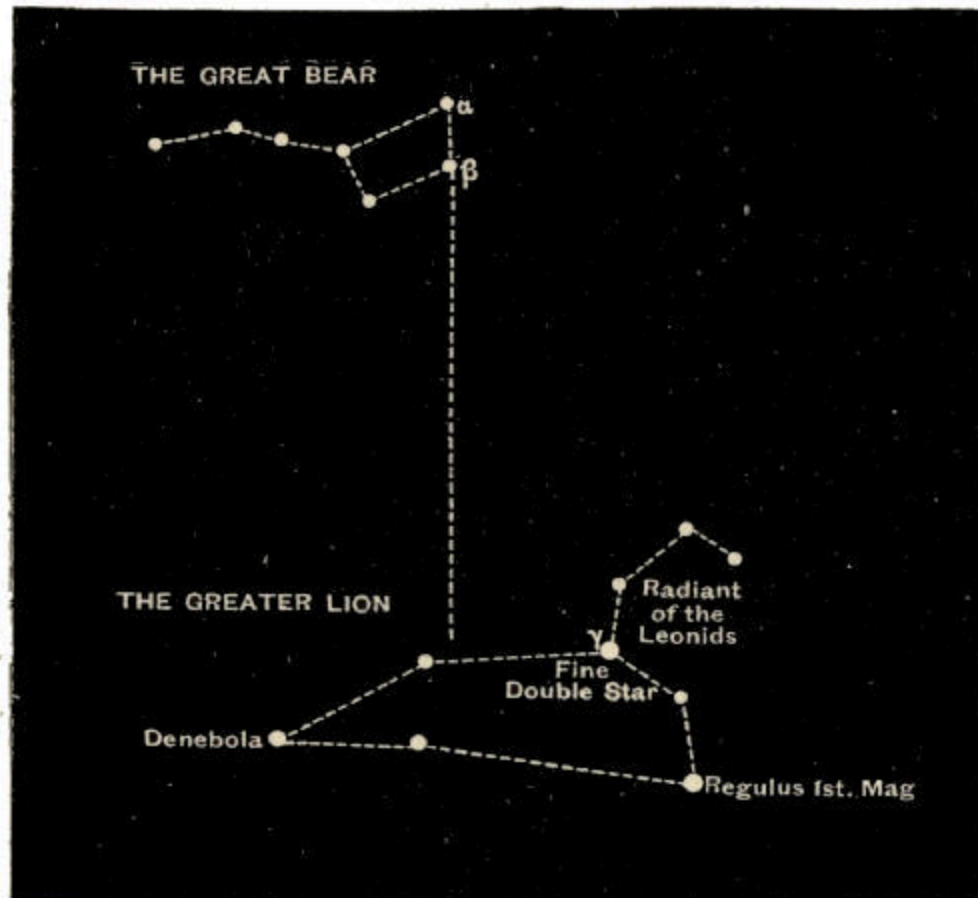
Fig. 87.—The Great Bear and the Lion.
