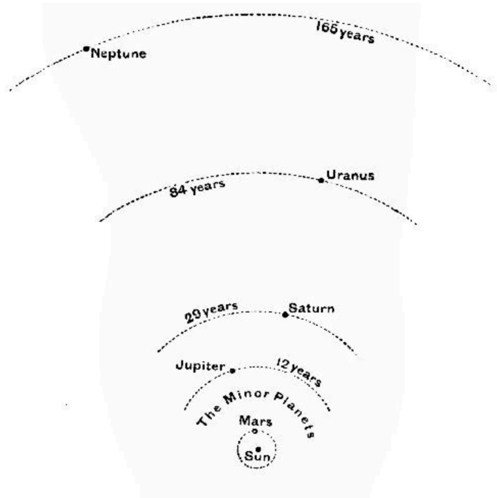
Fig. 33.—The Orbits of the Four Giant Planets.
