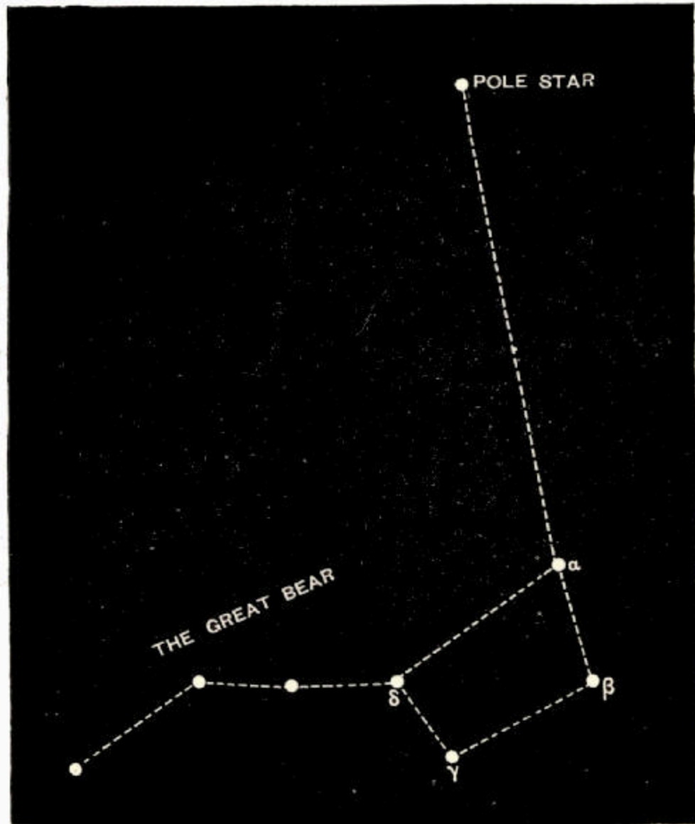
Fig. 80.—The Great Bear and Pole Star.
