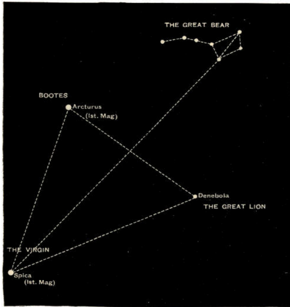
Fig. 89.—Virgo and the neighbouring Constellations.
