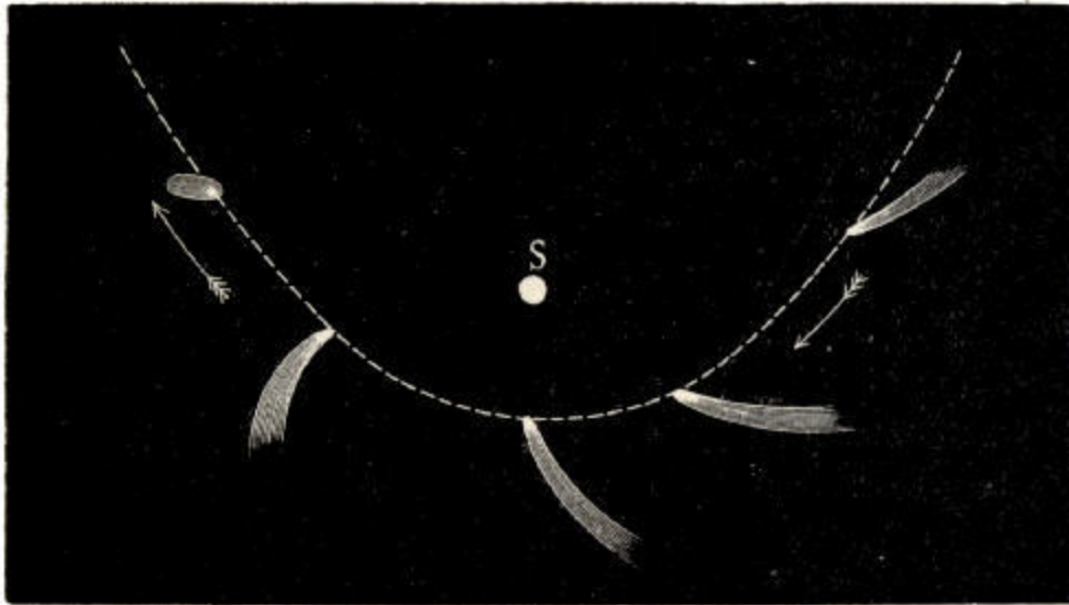
Fig. 71.—The Tail of a Comet directed from the Sun.
