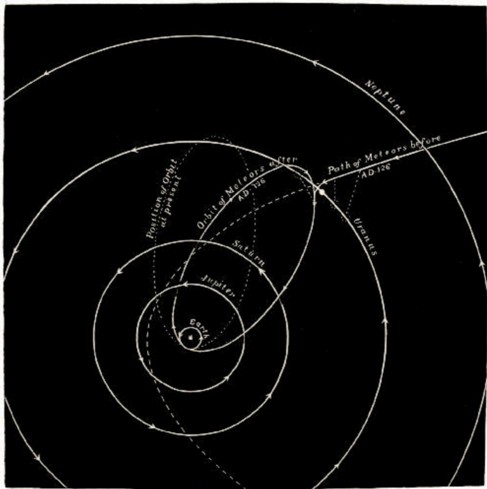
Fig. 78.—The History of the Leonids.
