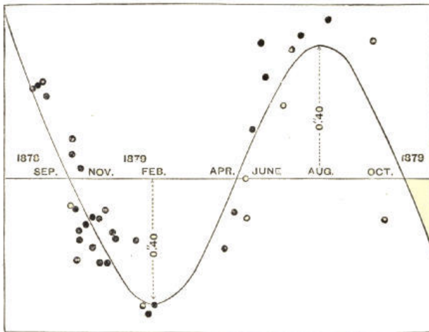
Fig. 95.—Parallax in Declination of 61 Cygni.
