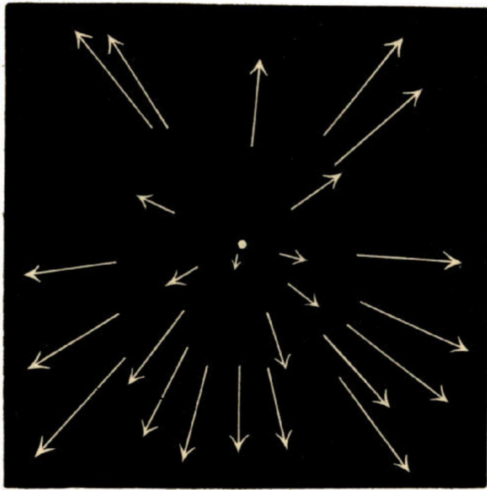
Fig. 77.—The Radiant Point of Shooting Stars.
