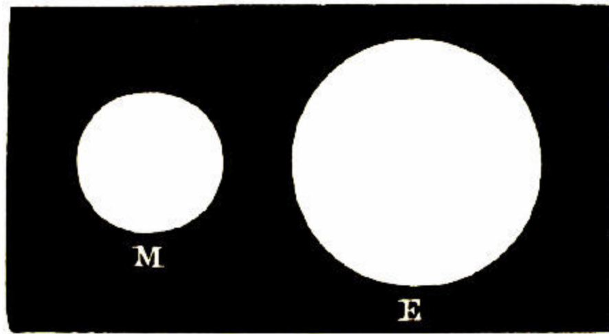
Fig. 50.—Relative Sizes of Mars and the Earth.
