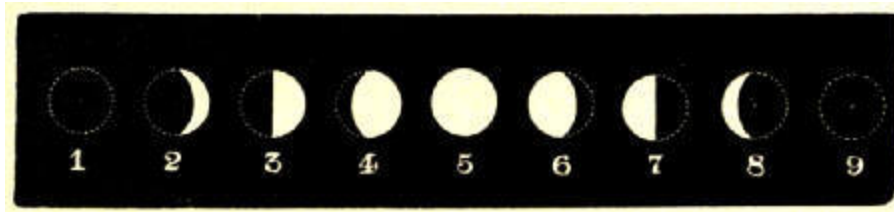
Fig. 25.—The Phases of the Moon.
