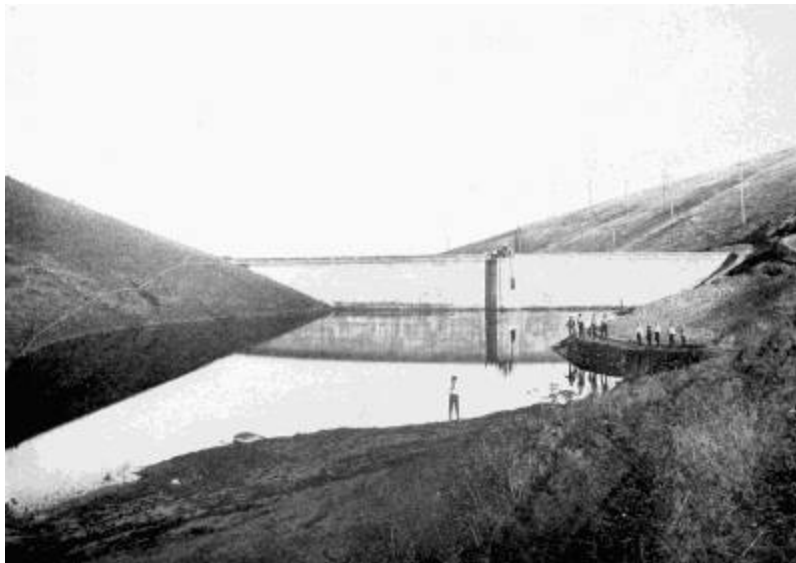
ONE VIEW OF THE PARTIALLY COMPLETED TWENTY MILLION GALLON POMEROY GULCH RESERVOIR. A LINK IN THE PRESSURE WATER SERVICE FOR THE IRRIGATION AND DOMESTIC SUPPLY OF CLARKSTON-VINELAND
