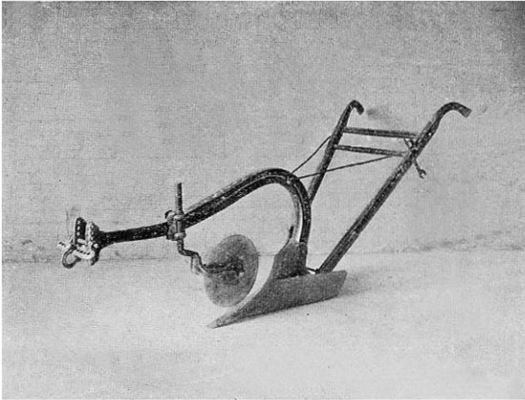
FIG. 53. An iron beam-plow, with rolling coulter and double clevis. To List
