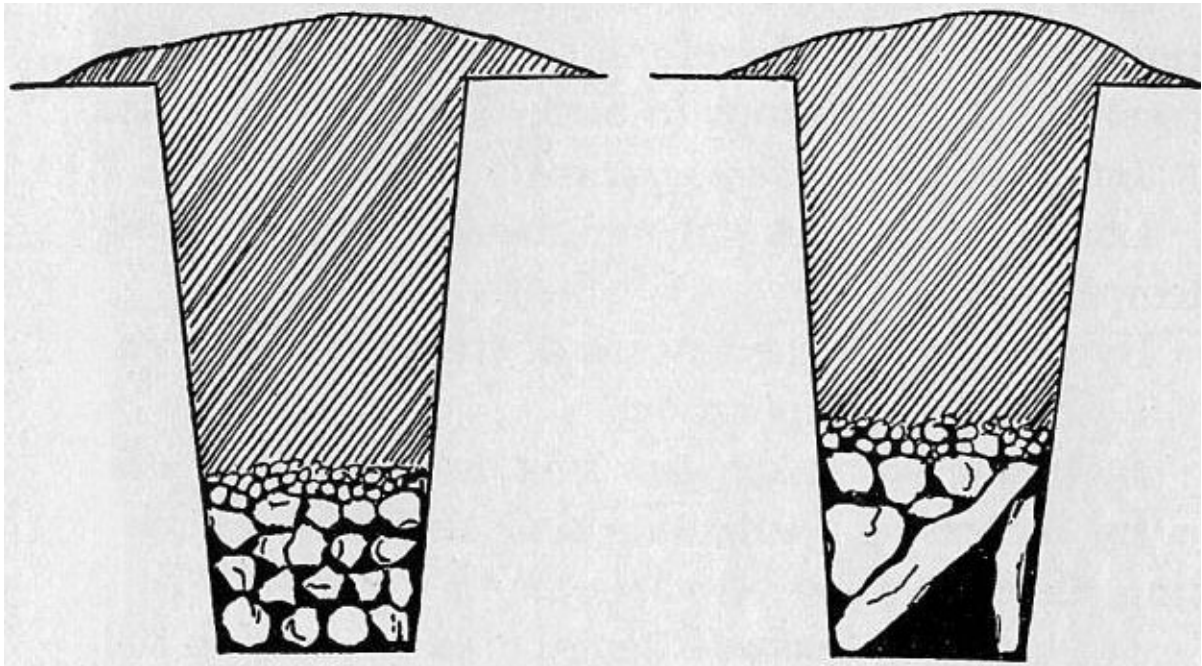
FIG. 83.—CROSS-SECTIONS OF STONE-DRAINS. ToList
