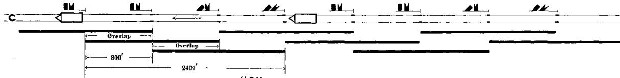
"C" Block System, With Overlaps. The Block Section Equal to Two Overlaps.
