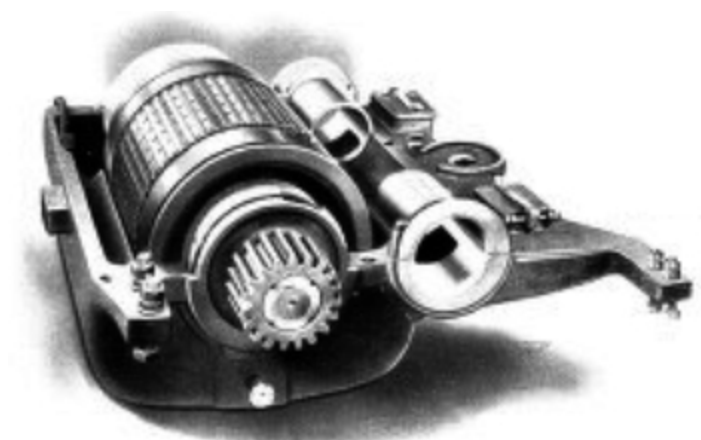
200 H. P. RAILWAY MOTOR
