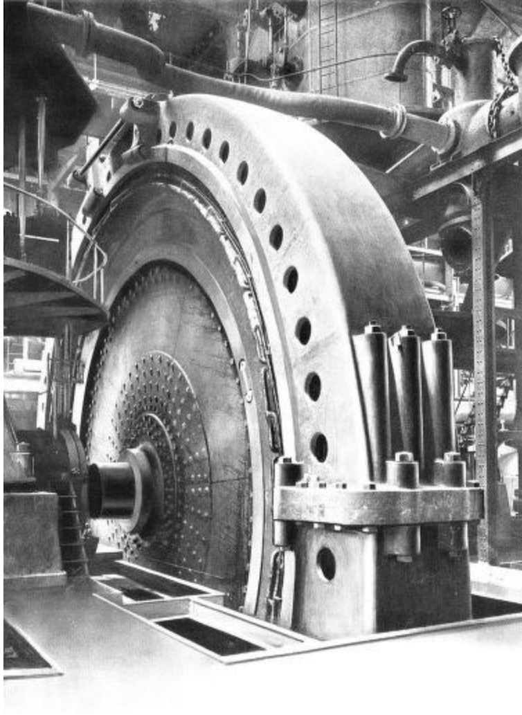
5,000 K. W. ALTERNATOR—MAIN POWER HOUSE
