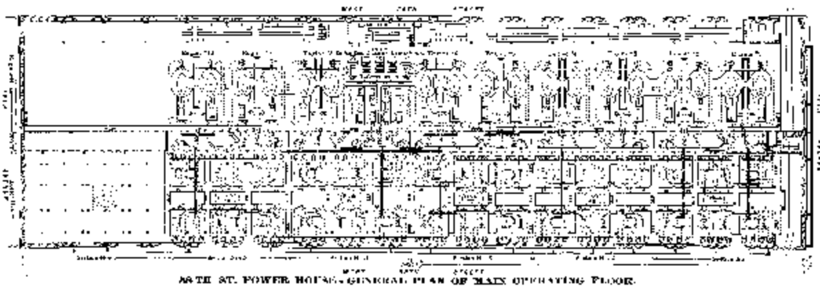
58TH ST. POWER HOUSE—GENERAL PLAN OF MAIN OPERATING FLOOR.
