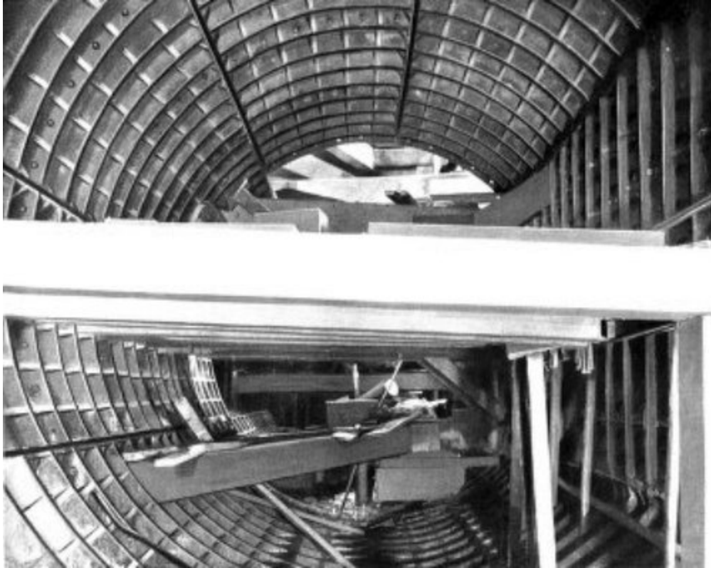
SECTION OF HARLEM RIVER TUNNEL DURING CONSTRUCTION
