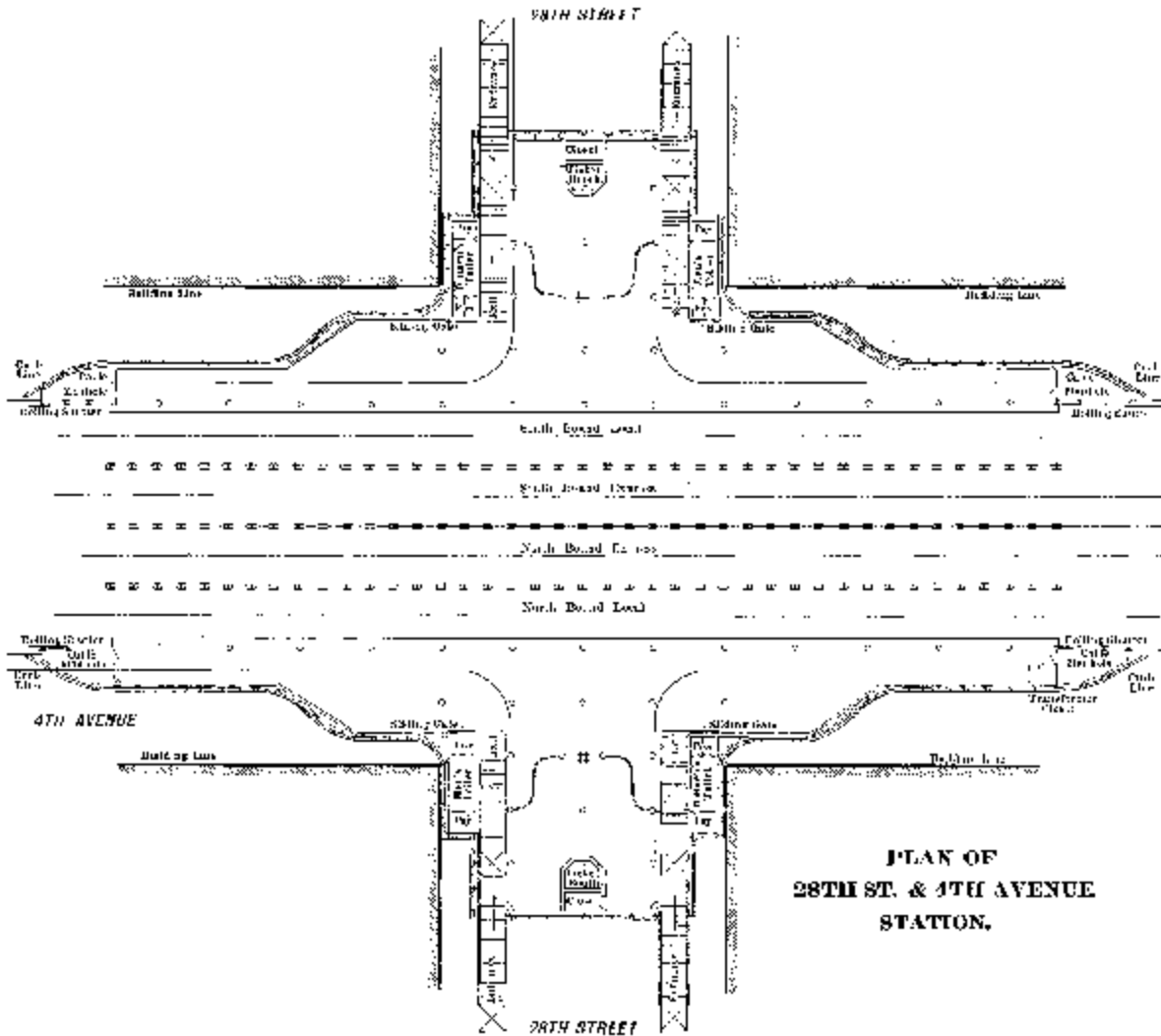
PLAN OF 28TH ST. & 4TH AVENUE STATION.
