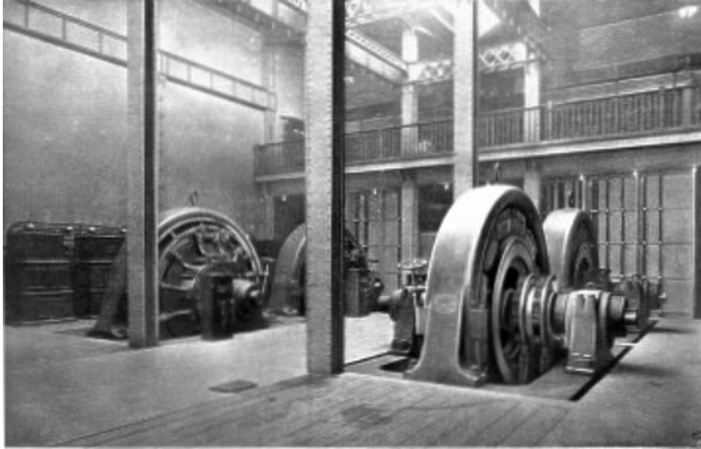
INTERIOR OF SUB-STATION NO. 11
