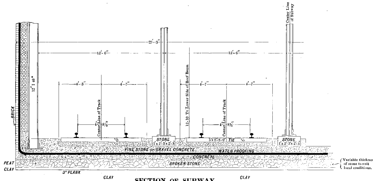
SECTION OF SUBWAY AT PEARL STREET
