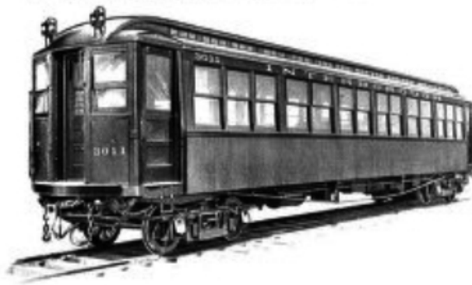
EXTERIOR VIEW—PROTECTED WOODEN CAR, SHOWING COPPER SIDES
