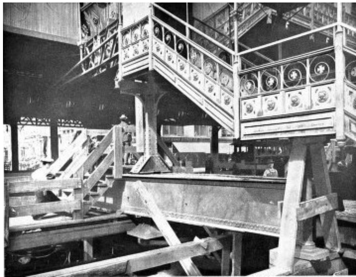
SUPPORT OF ELEVATED RAILWAY STATION AT 42D STREET AND SIXTH AVENUE
