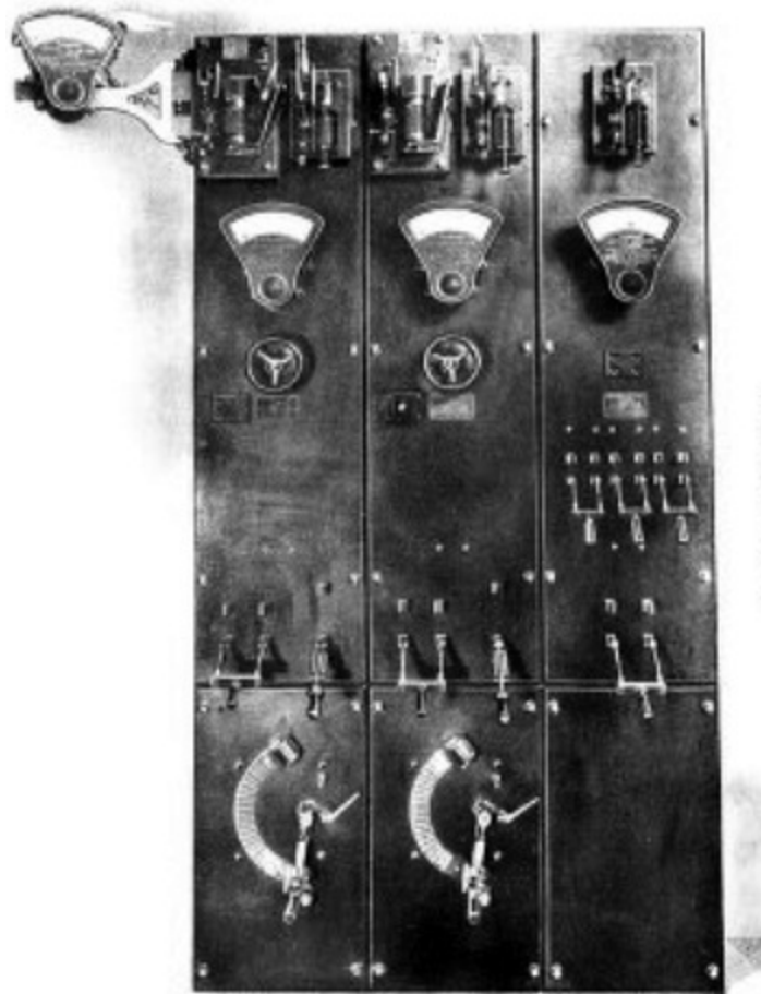
MOTOR-GENERATORS AND BATTERY BOARD FOR CONTROL CIRCUITS—SUB-STATION
