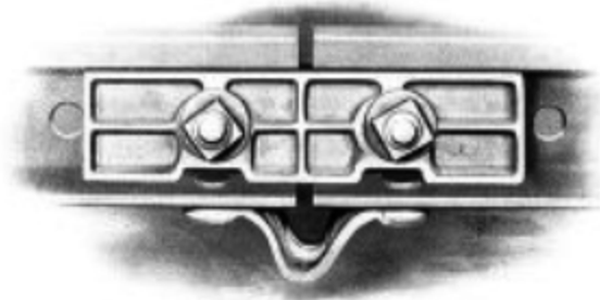
CONTACT RAIL JOINT WITH FISH PLATE
