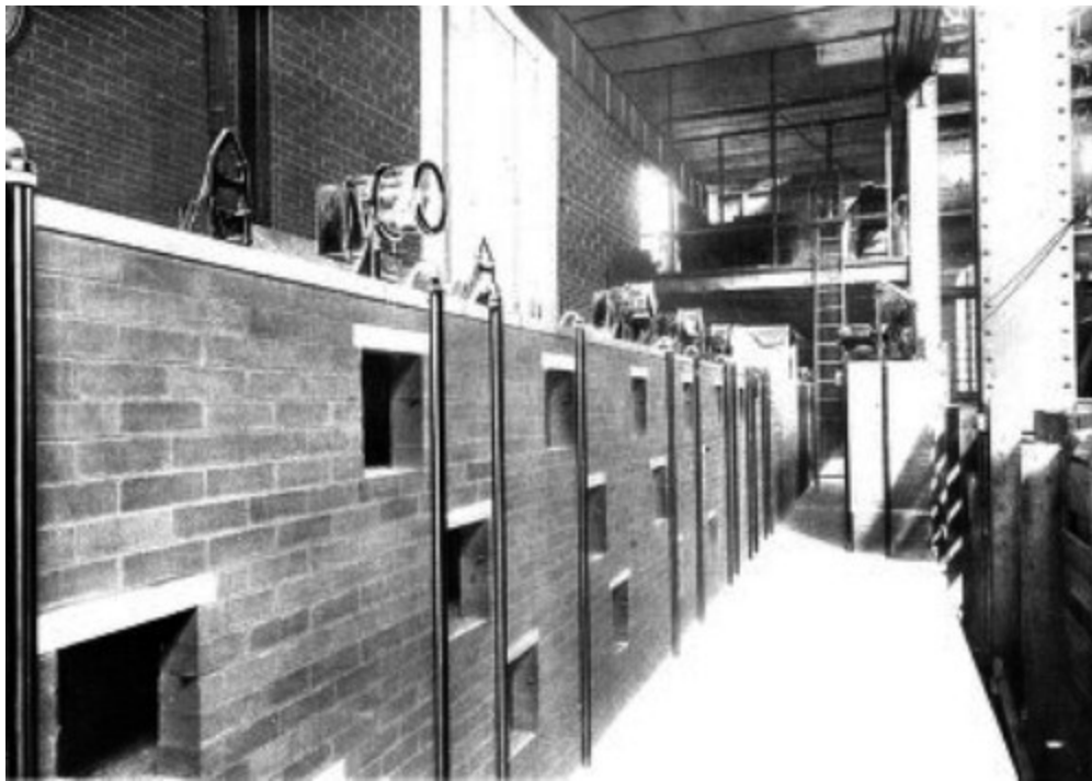
PART OF BUS BAR COMPARTMENTS—MAIN POWER STATION
