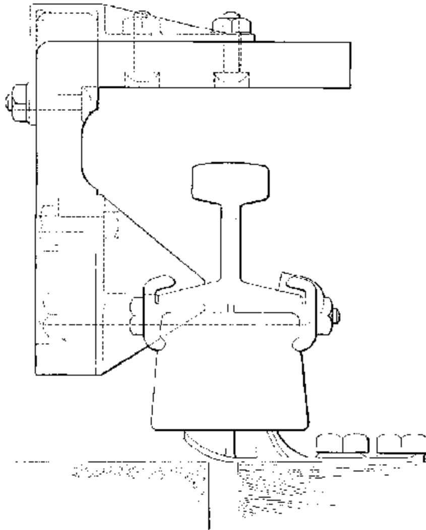
ASSEMBLY OF CONTACT RAIL AND
