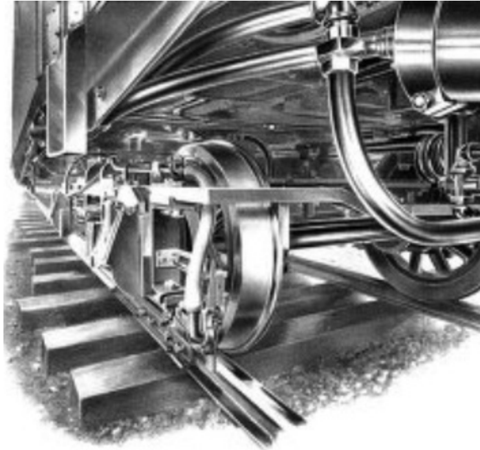
VIEW UNDER CAR, SHOWING TRIGGER ON TRUCK IN POSITION TO ENGAGE WITH TRACK STOP
