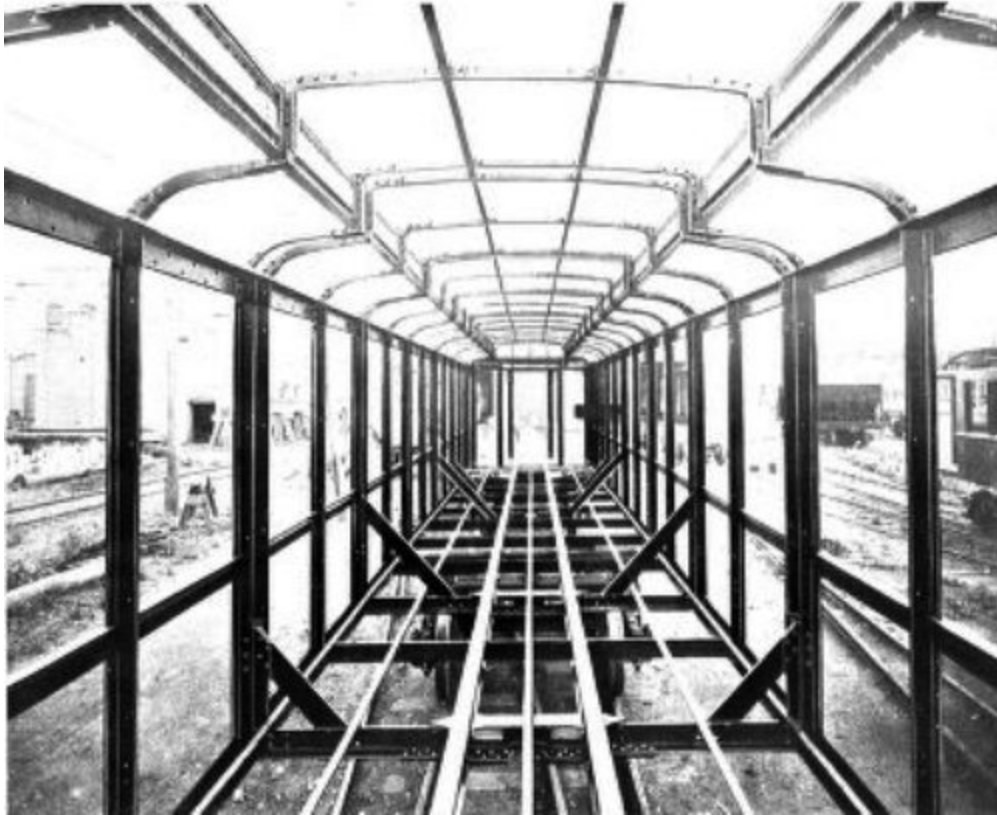
INTERIOR VIEW—SKELETON FRAMING OF STEEL CAR
