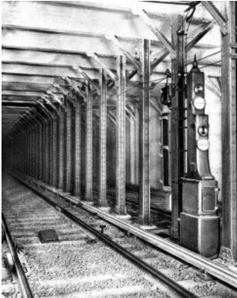
FRONT VIEW OF BLOCK SIGNAL POST, SHOWING LIGHTS, INDICATORS AND TRACK STOP
