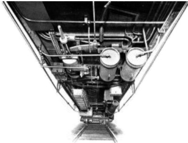
APPARATUS UNDER COMPOSITE MOTOR CAR
