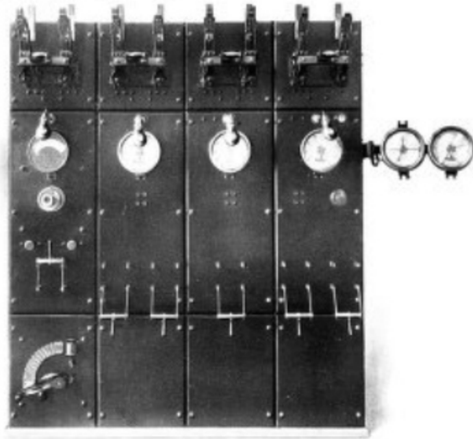
SWITCHBOARD FOR ALTERNATING CURRENT BLOCK SIGNAL CIRCUITS—IN SUB- STATION
