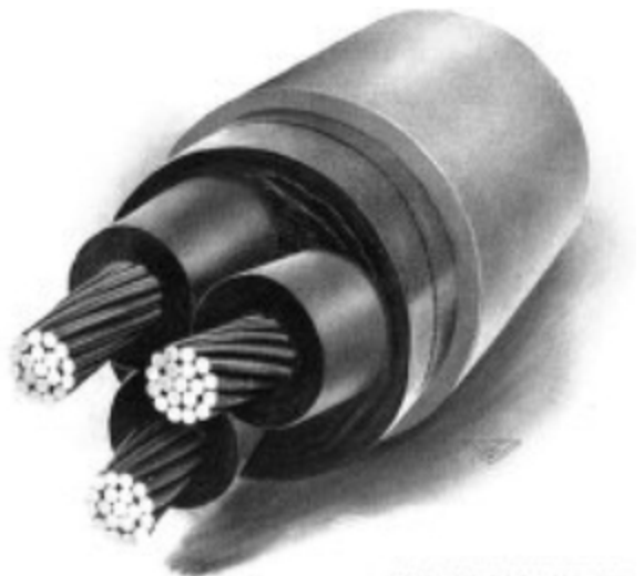
THREE-CONDUCTOR NO. 000 CABLE FOR 11,000 VOLT DISTRIBUTION
