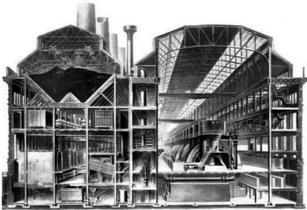
CROSS SECTION OF POWER HOUSE IN PERSPECTIVE
