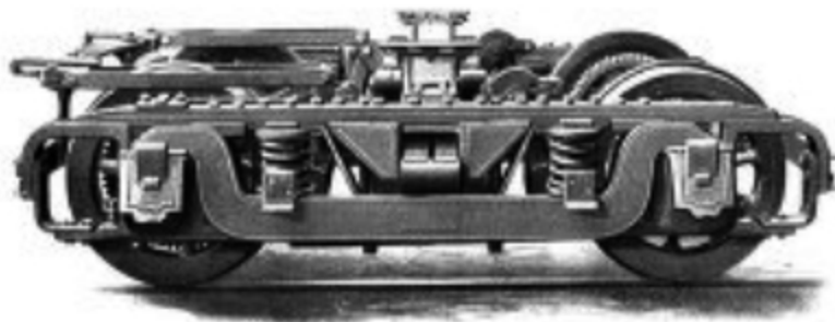
SIDE VIEW OF MOTOR TRUCK
