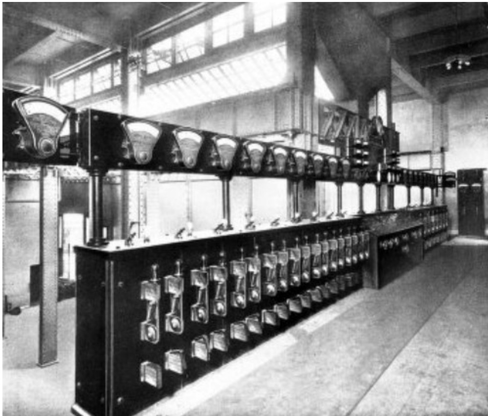
OPERATING BOARD—SUB-STATION NO. 11
