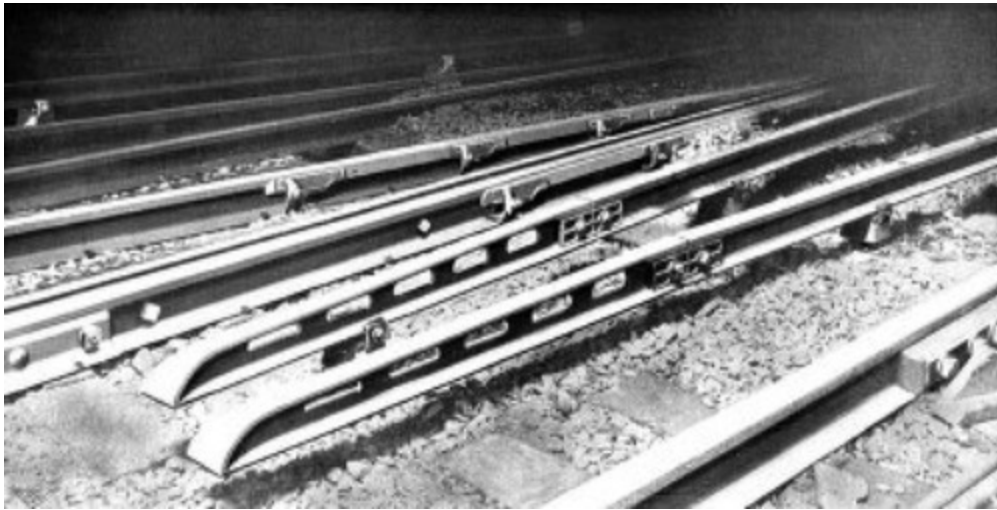
CONTACT RAILS, SHOWING END INCLINES
