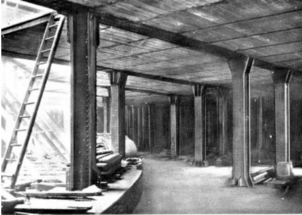
COLUMNS OF HOTEL BELMONT, PASSING THROUGH SUBWAY AT 42D STREET AND PARK AVENUE
