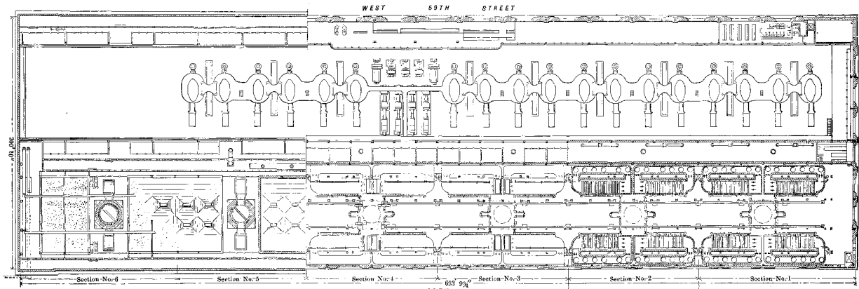
58 TH ST. POWER HOUSE - GENERAL PLAN OF COAL BUNKERS AND ECONOMIZERS.
