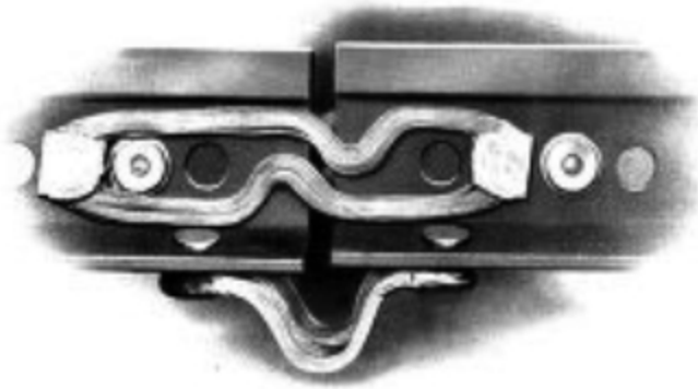
CONTACT RAIL BANDS
