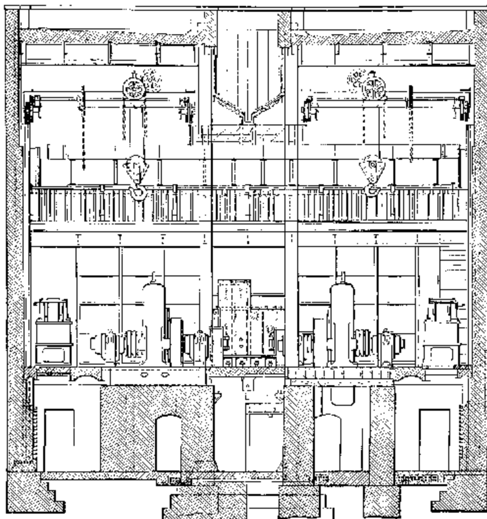
CROSS SECTION SUB-STATION NO. 14
