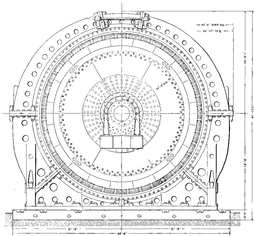
SIDE AND END ELEVATIONS OF ALTERNATOR.
