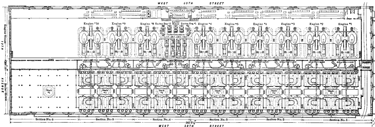
58 TH ST. POWER HOUSE - GENERAL PLAN OF MAIN OPERATING FLOOR.
