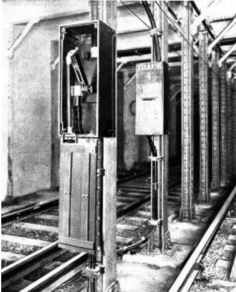
SWITCH CONNECTING FEEDER TO CONTACT RAIL
