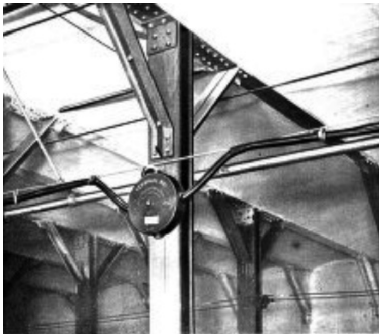
MAIN LINE, PIPING AND WIRING FOR BLOCK AND INTERLOCKING SYSTEM, SHOWING JUNCTION BOX
