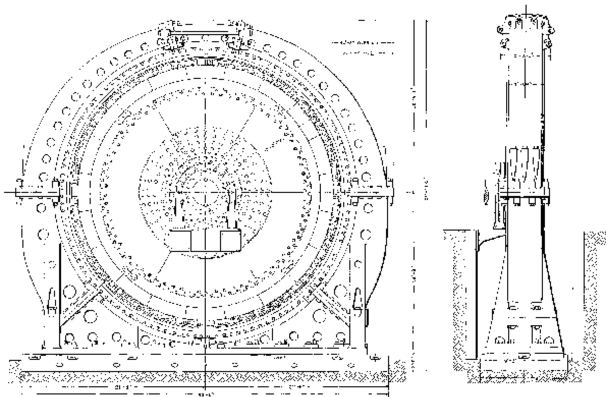
SIDE AND END ELEVATIONS OF ALTERNATOR.
