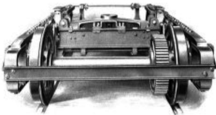
END VIEW OF MOTOR TRUCK
