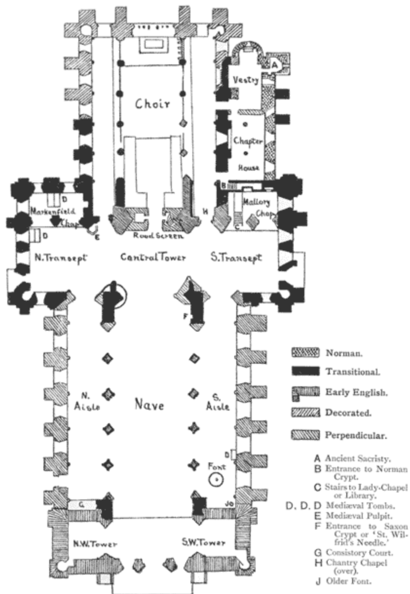
GROUND PLAN OF RIPON CATHEDRAL.
