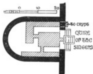
CONJECTURAL PLAN OF THE CRYPT AND PRESBYTERY IN THE TIME OF WILFRID, BY MR. J. T. MICKLETHWAITE, V.P.S.A.
