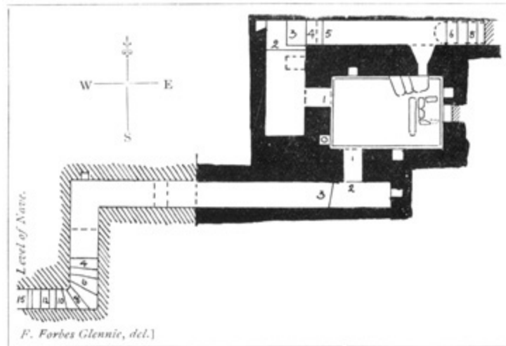
PLAN OF THE SAXON CRYPT.
