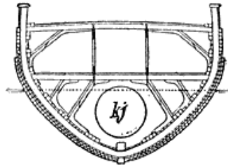
Fig. 4. Transverse section at the engine-room.
