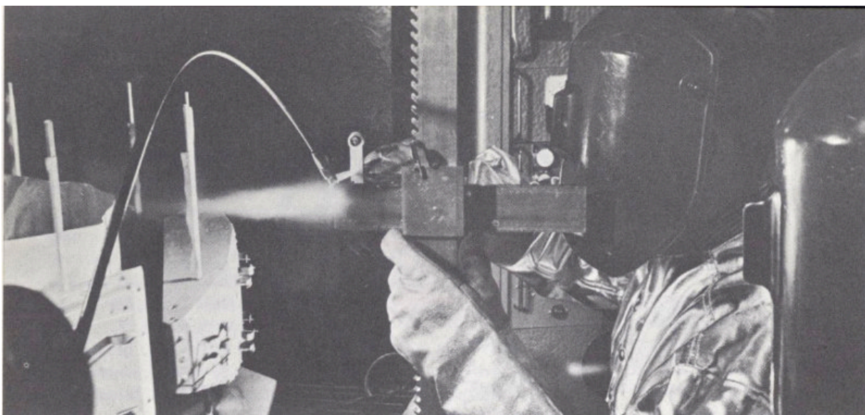
Partially molten aluminum oxide particles being sprayed onto aluminum outer surface panels.
