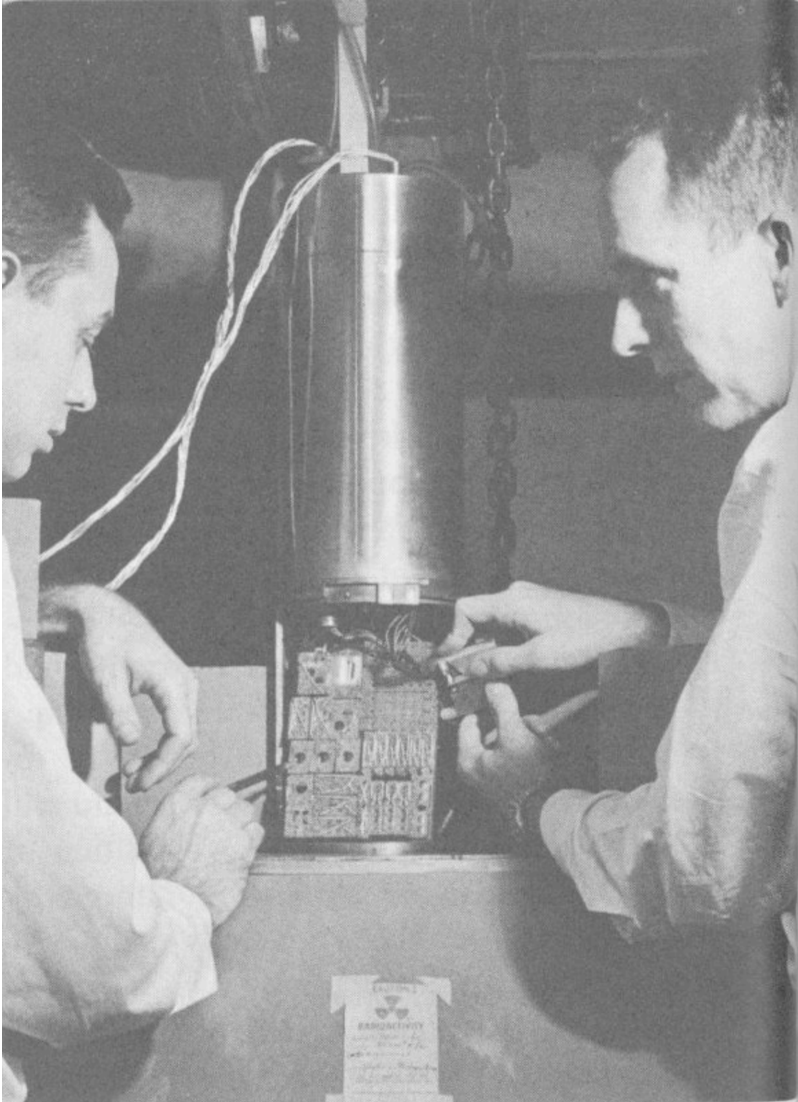
A duplicate of one of Telstar I's command decoders, containing 37 transistors and 191 diodes, being placed in a small elevator that will
