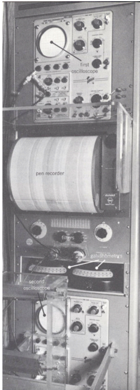
General view of amplifying, monitoring, and recording gear that picks up glints of sunlight at the Crawford's Hill observation station.
