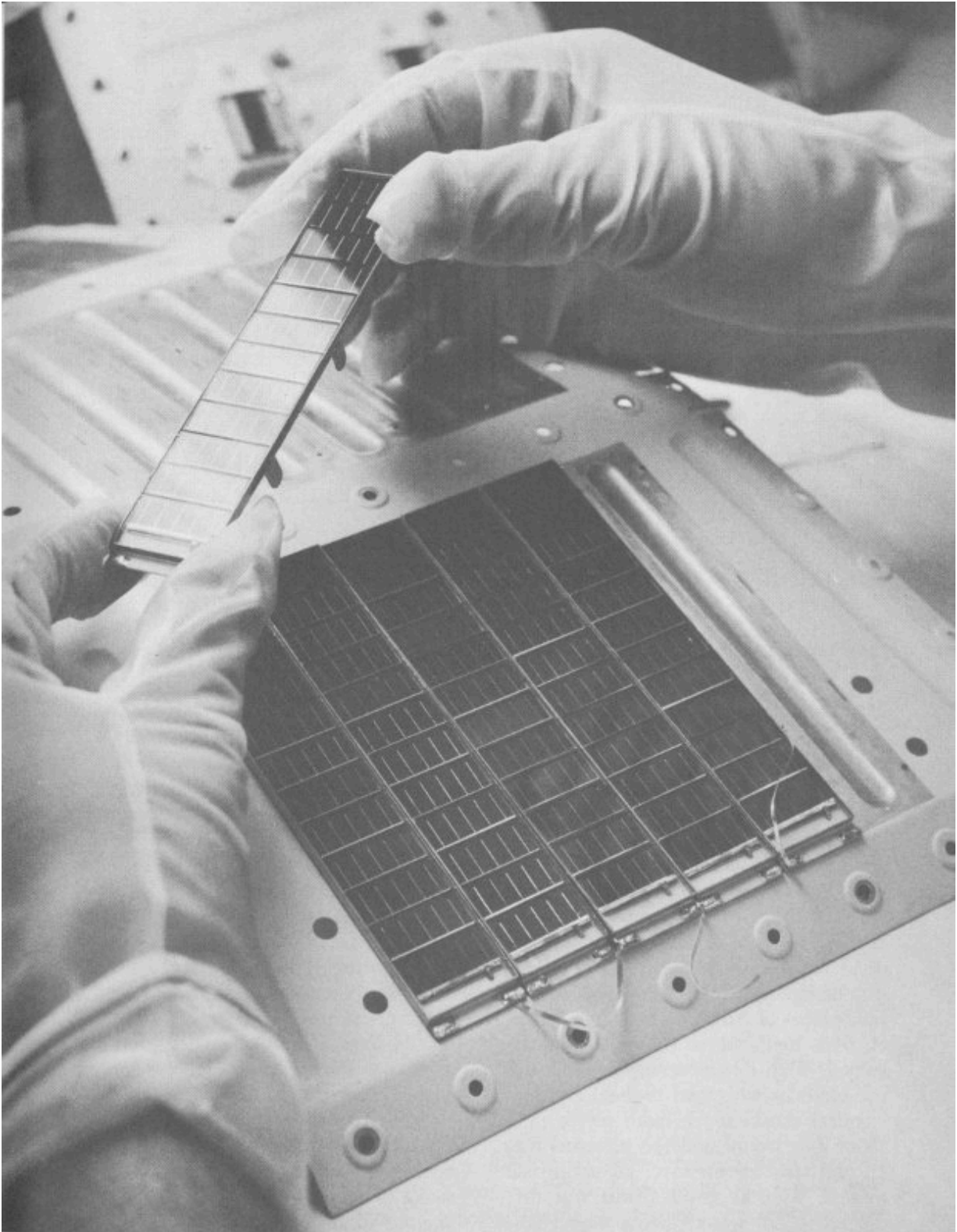
The satellite uses 300 modules of twelve solar cells, in groups of six or three modules per facet.
