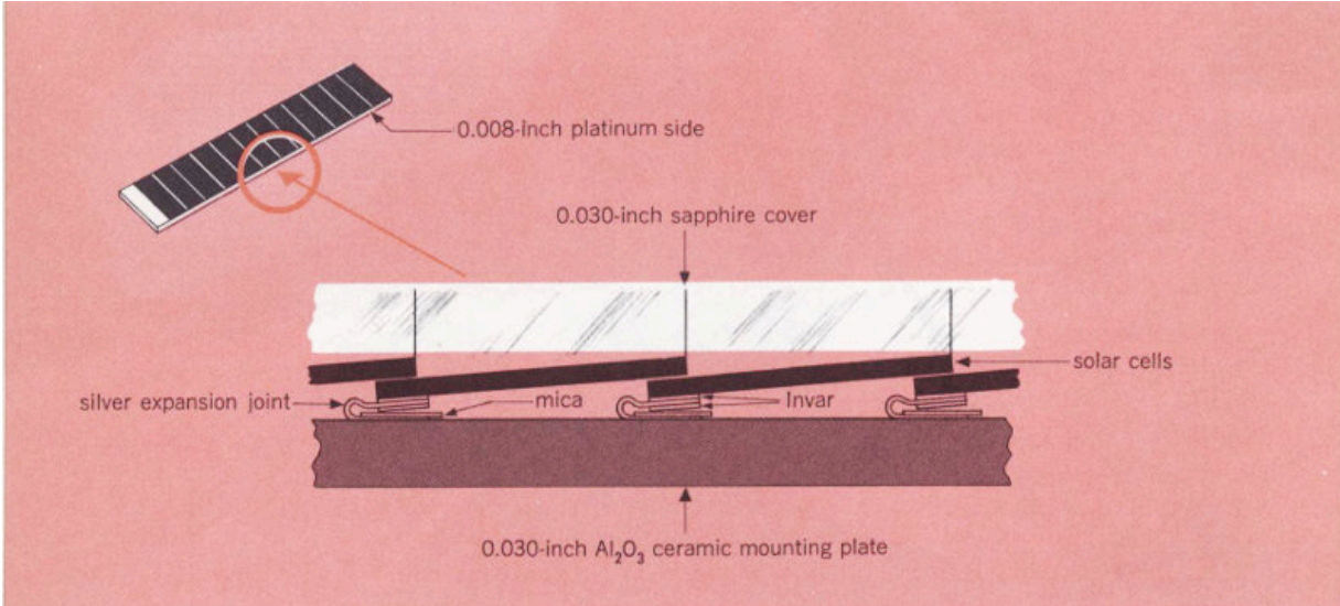
Lengthwise diagram of a solar cell module, showing how individual cells were fixed in place.
