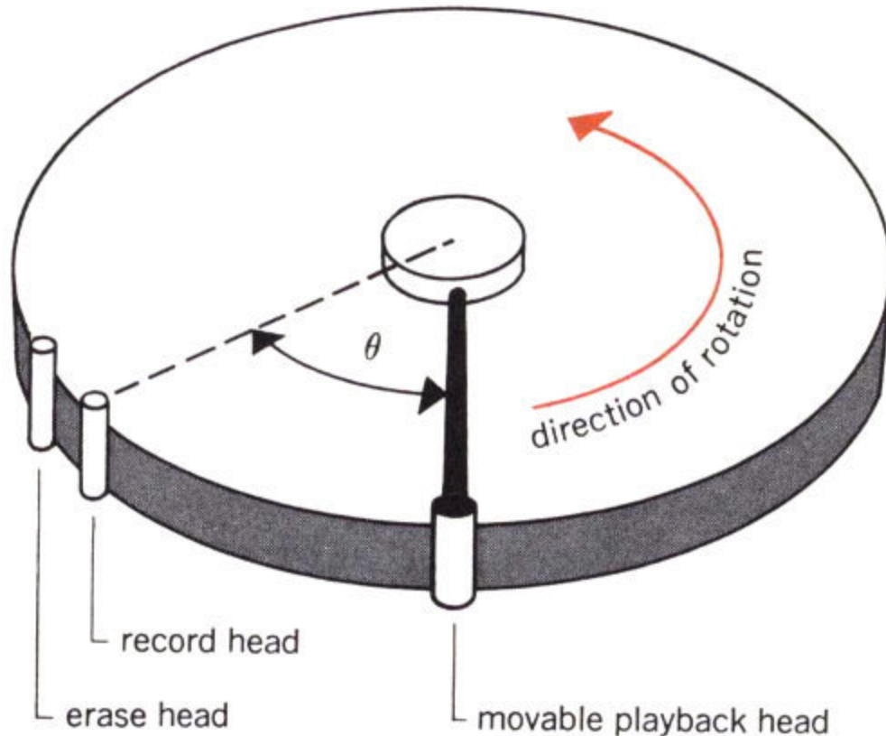
Recording equipment used in the experiment.
