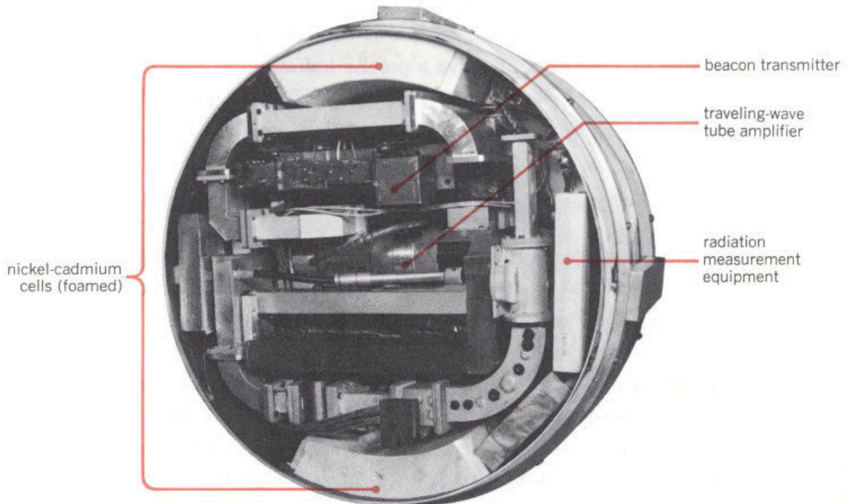
The Telstar I satellite—inside (looking at the electronics canister from the top down)
