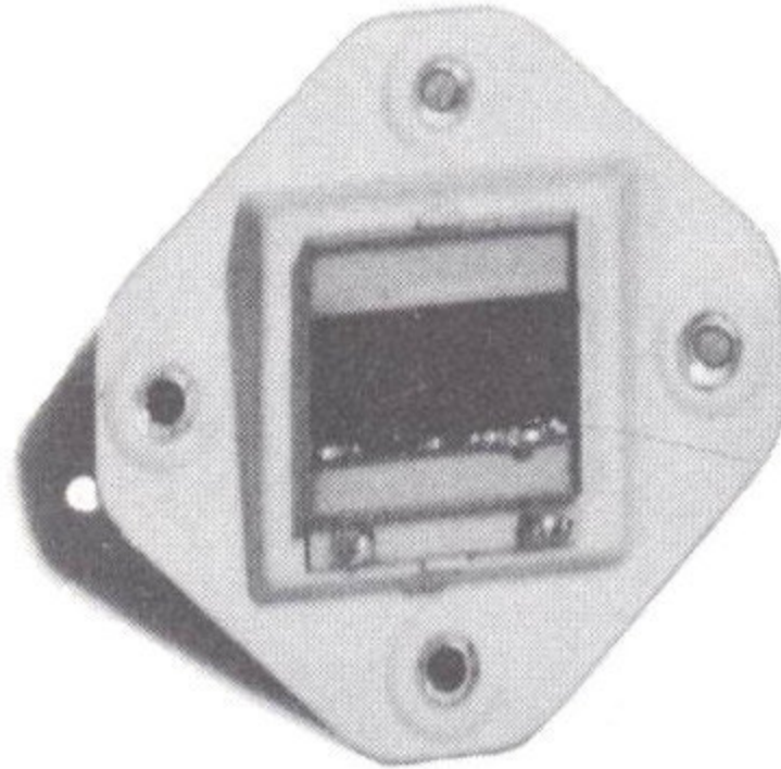
solar cells used to measure radiation damage and as solar aspect indicators
