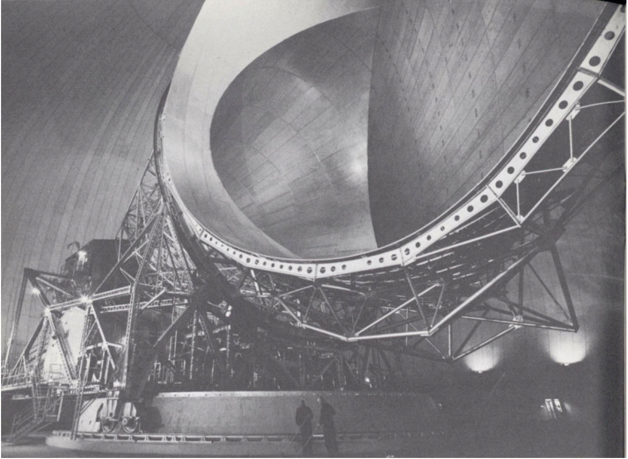
The giant horn antenna at Andover, Maine
