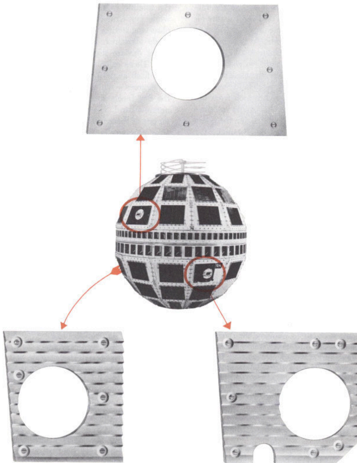
Sketches of three reflecting mirrors and their locations on the Telstar satellite. The upper plane mirror is set at 68^\circ to the spin axis; the lower ones are faceted to give reflecting surfaces at 95^\circ . Two of the satellite's
