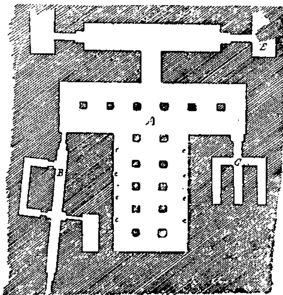
Fig 74. --Plan of temple of the Sphinx.
