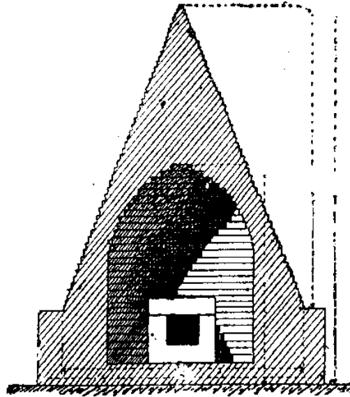
Fig 144.--Section of "vaulted" brick pyramid, Abydos.
