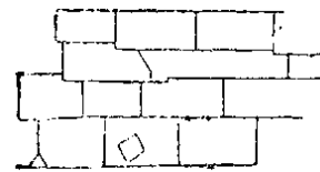
Fig 52 .--Masonry in temple of Seti I. at Abydos.
