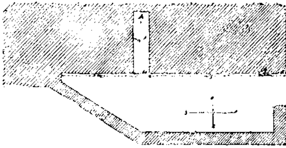
Fig 116. --Plan of forecourt, mastaba of Neferhotep.
