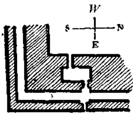
Fig. 30. --Plan of south-east gate, second fortress of Abydos.
