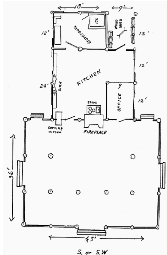
A. Floor Plan for Mess Hall for Camp of 150 to 200 Girls
