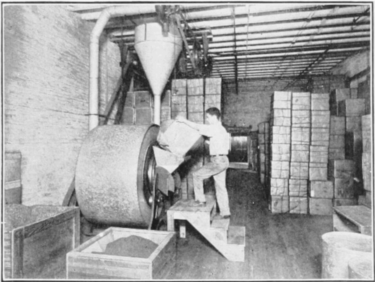
Vacuum Tea Cleaner
