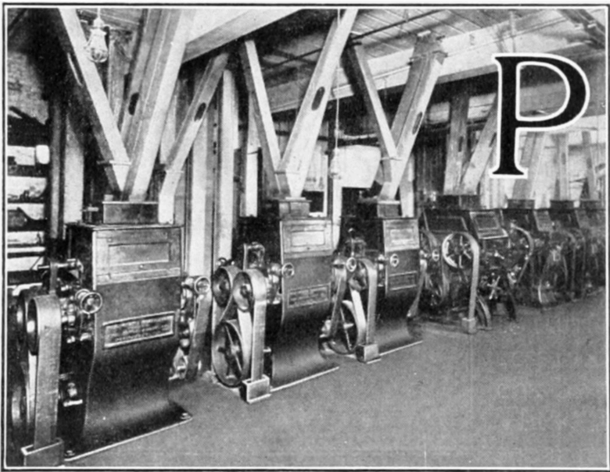
A Group of Pepper Mills
