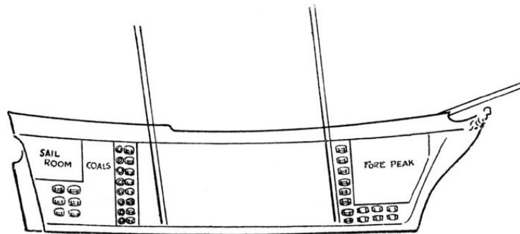
Plan of the Schooner Good Intent showing Method of Smuggling Casks. To List
