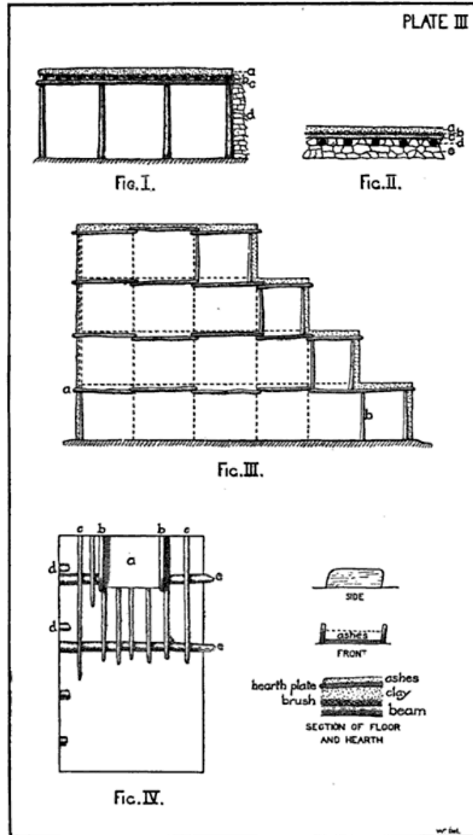
PLATE III: SECTIONS OF BUILDING B.
