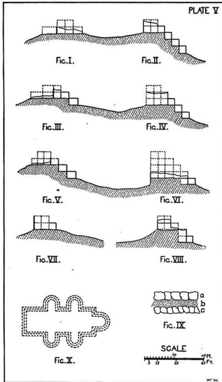
PLATE V: SECTIONS OF BUILDING A.
