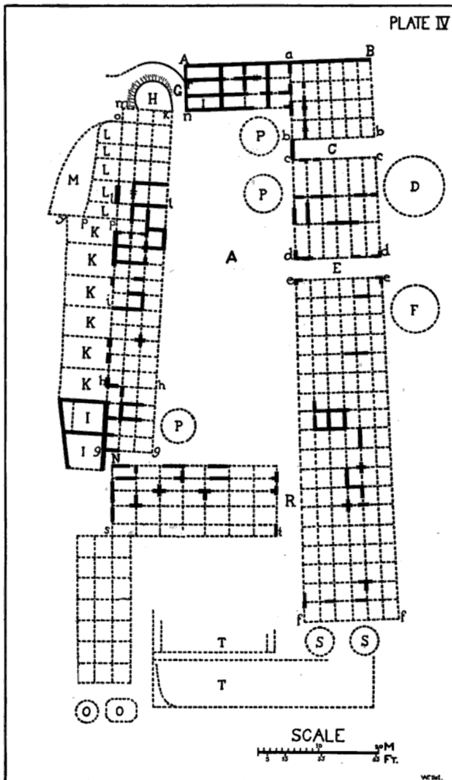
PLAN OF BUILDING A.
