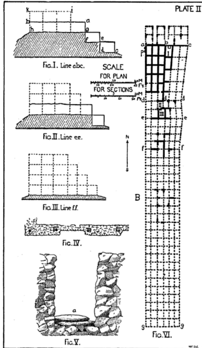
PLATE II: PLAN OF SECTIONS OF BUILDING B.
