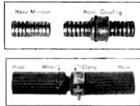
Figure 14.—Hose menders: Above, hose mender and hose coupling; below, two pieces of hose joined with a mender. The left-hand piece is fastened with wire twisted with a pair of pliers, and the right-hand piece is clamped.
