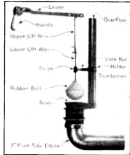
Figure 8.—Flush valve for low tank.
