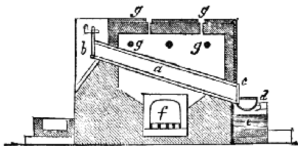
Bismuth furnace in section.
