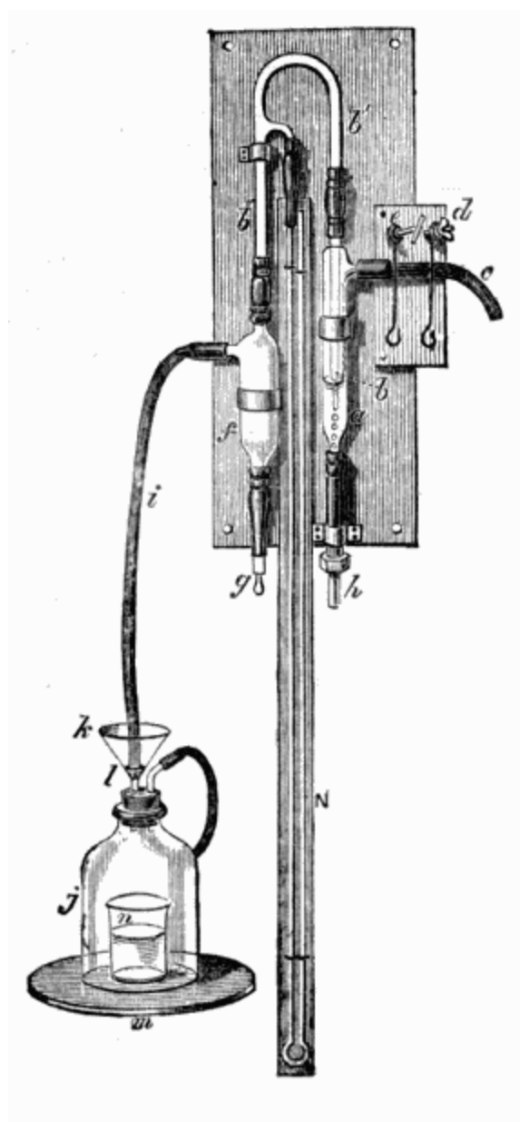
Bunsen's water-air-pump.
