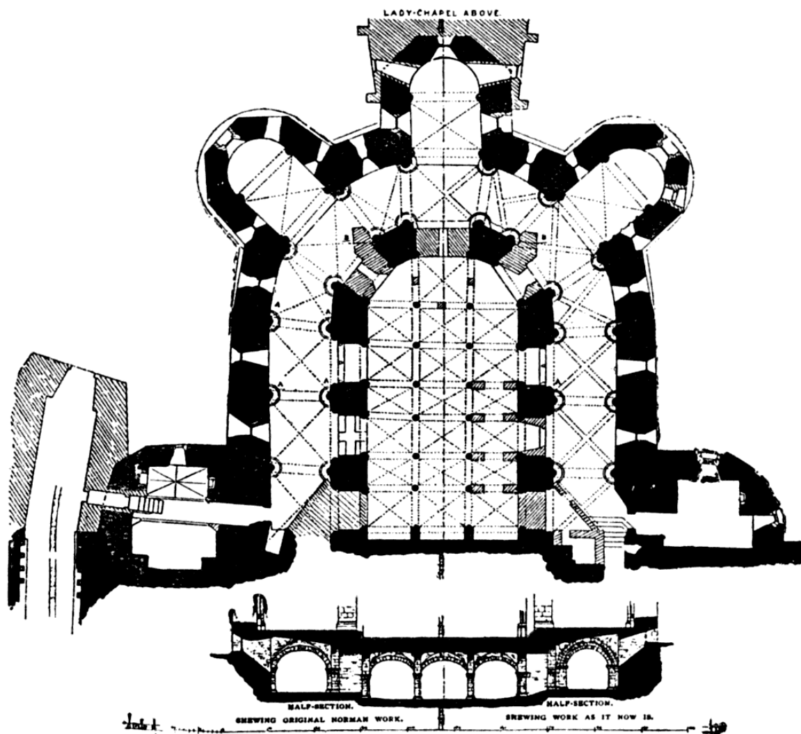
PLAN OF THE CRYPT.
