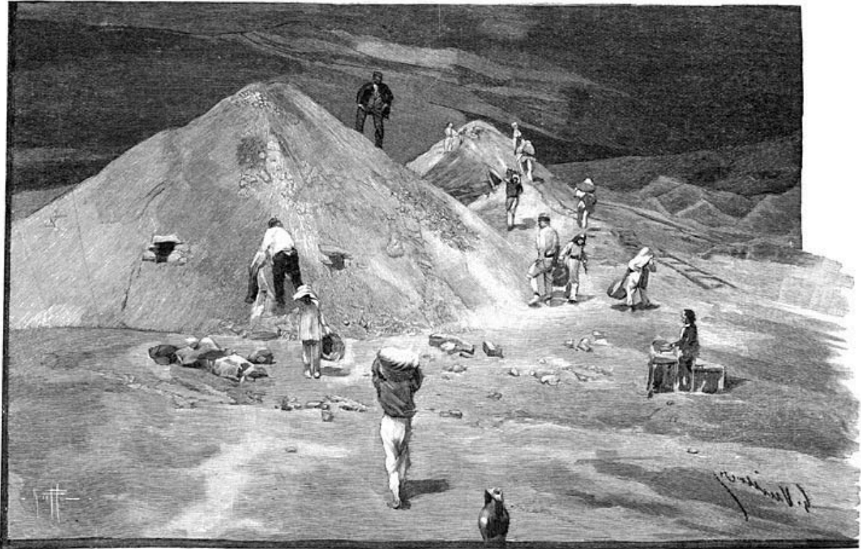
Calcarone of zwavelhoopen.
