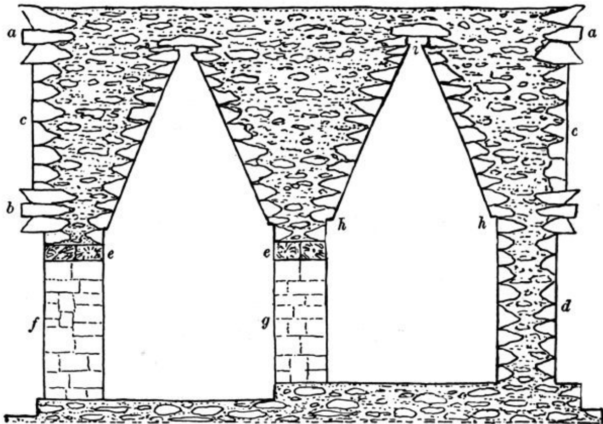
Fig. 21. Cross-section of Typical Mayan Temple in Northern Yucatan: a, upper cornice; b, medial cornice; c, upper zone; d, lower zone; e, wooden lintels; f, exterior doorway; g, interior doorway; h, offset at spring of vault; i, cap stone.
