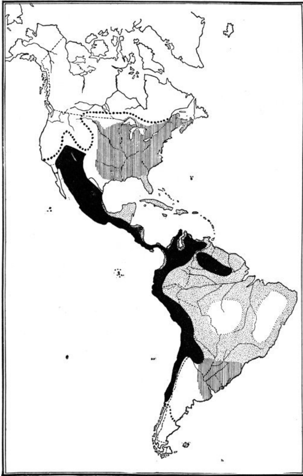
Distribution of Agriculture in the New World. The dotted line gives the limits of pottery; solid black, agriculture in arid regions of considerable altitude, mostly with irrigation; dotted areas, agriculture under humid lowland conditions; lined area, agriculture under temperate conditions.
