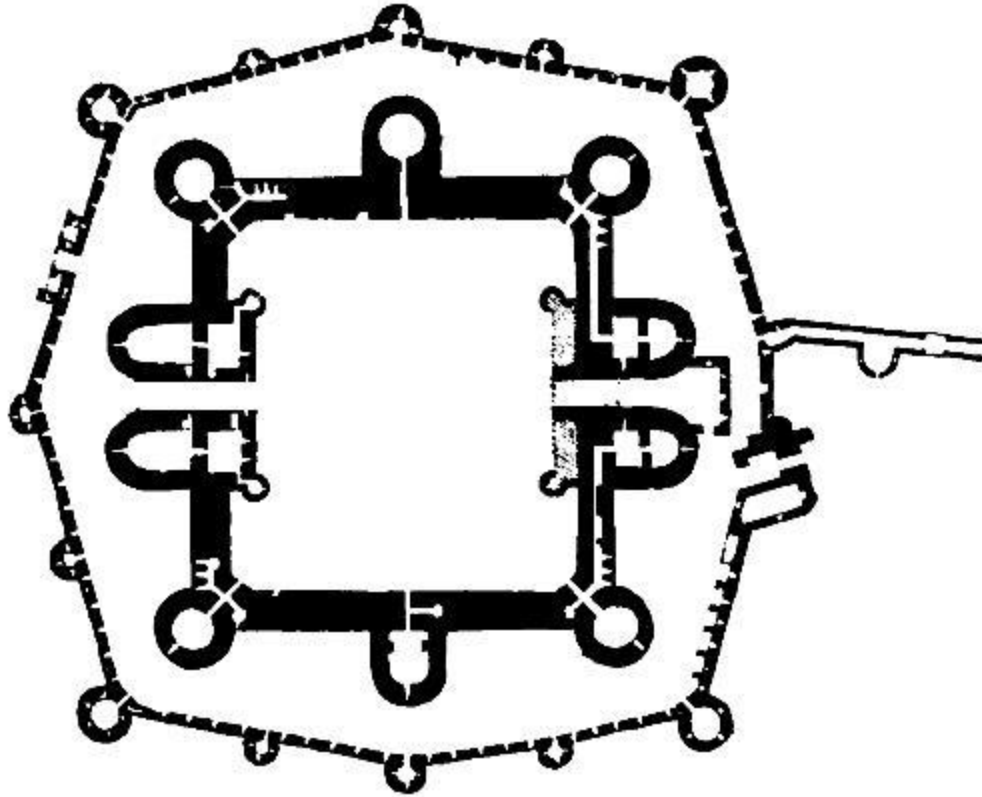
Beaumaris Castle; Plan
