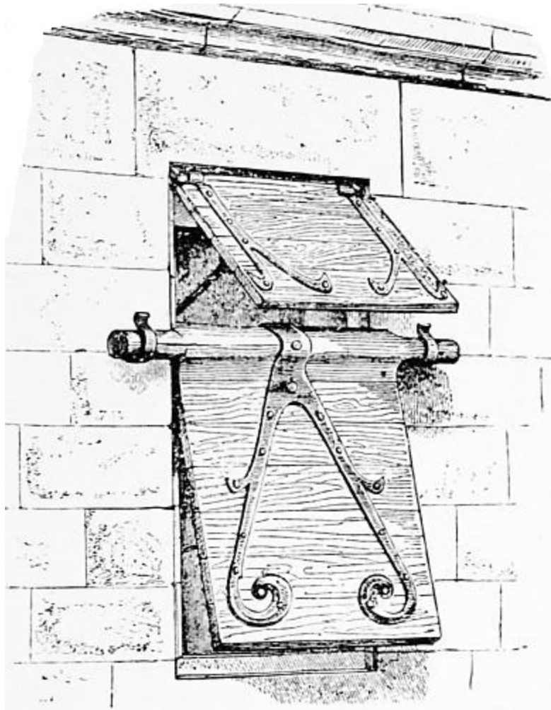
Shutter closing opening in wall or parapet
