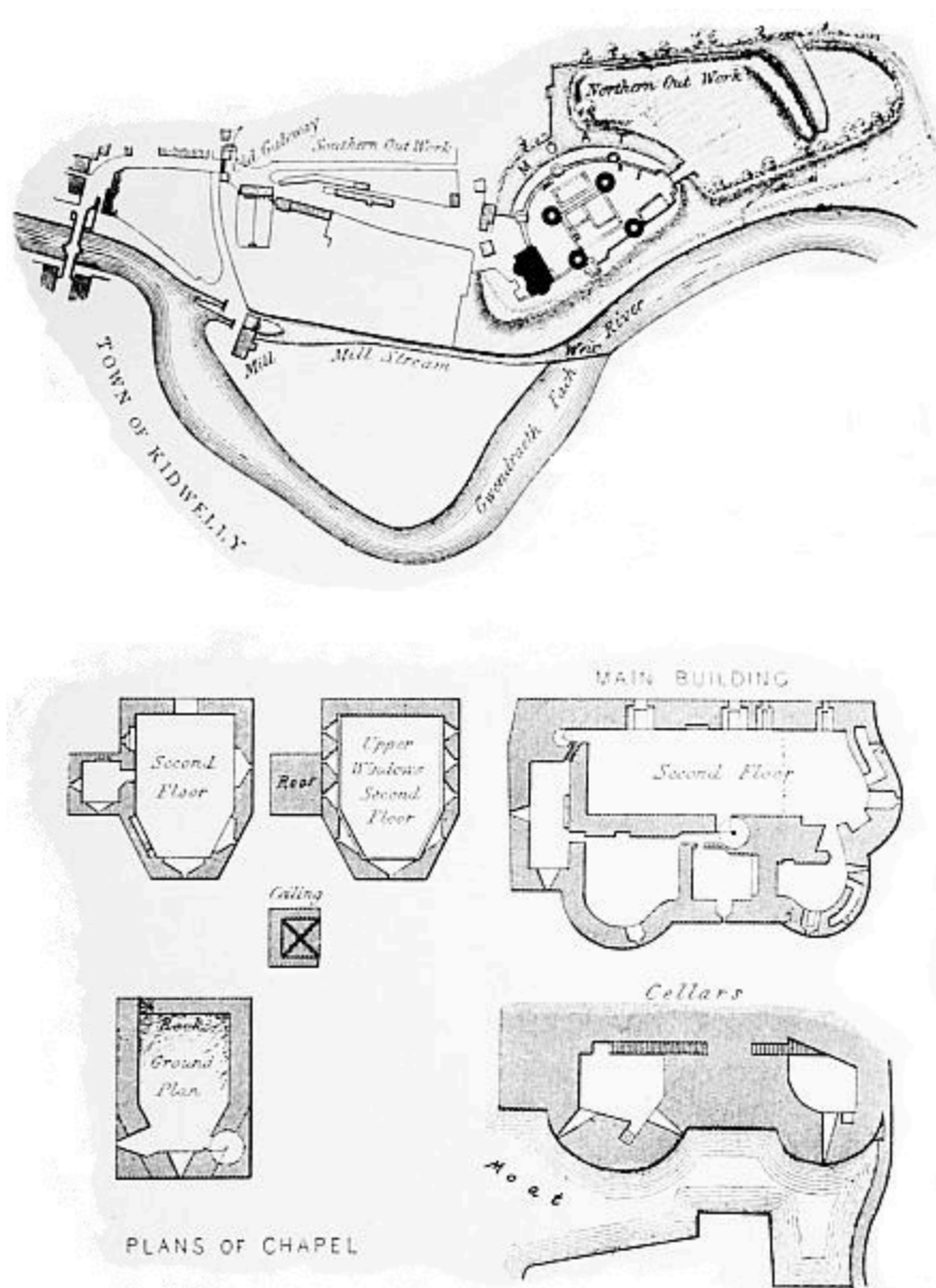
Kidwelly Castle; Plan
