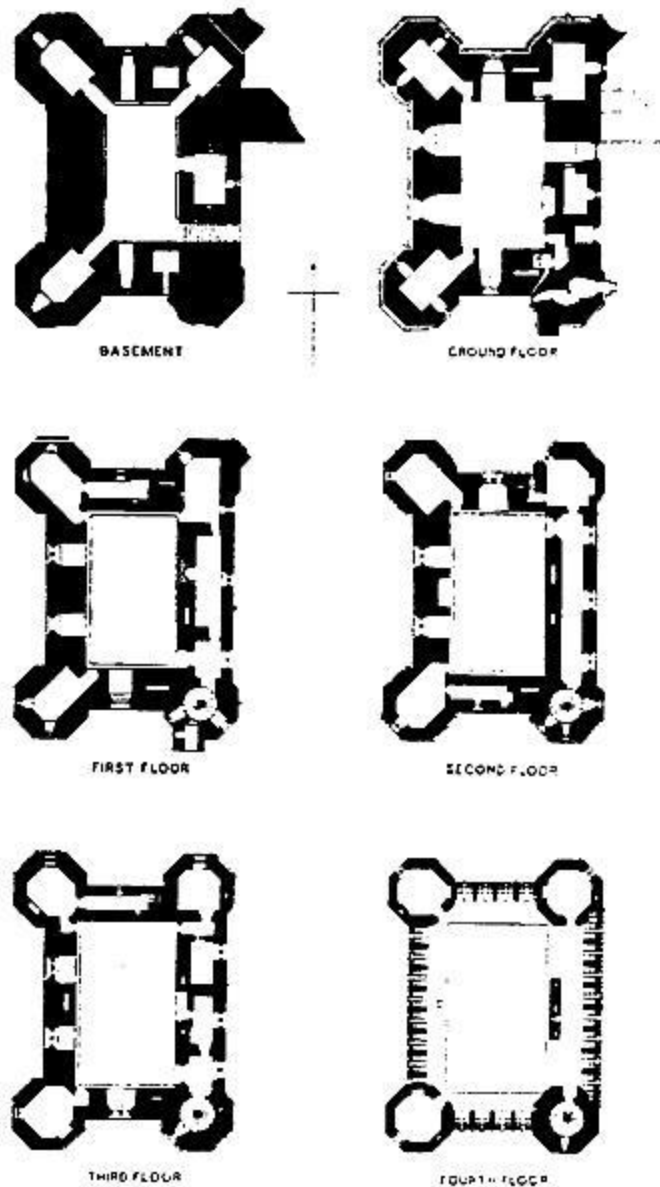
Tattershall Castle; Plan
