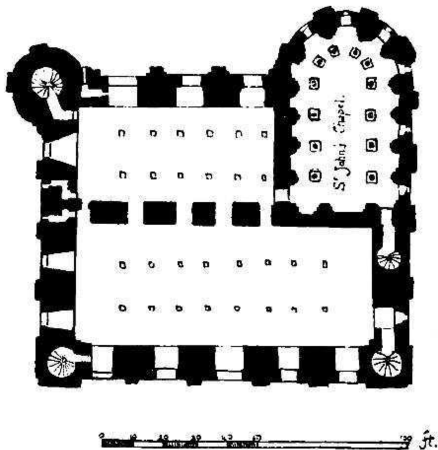
White Tower; Plan of Second Floor
