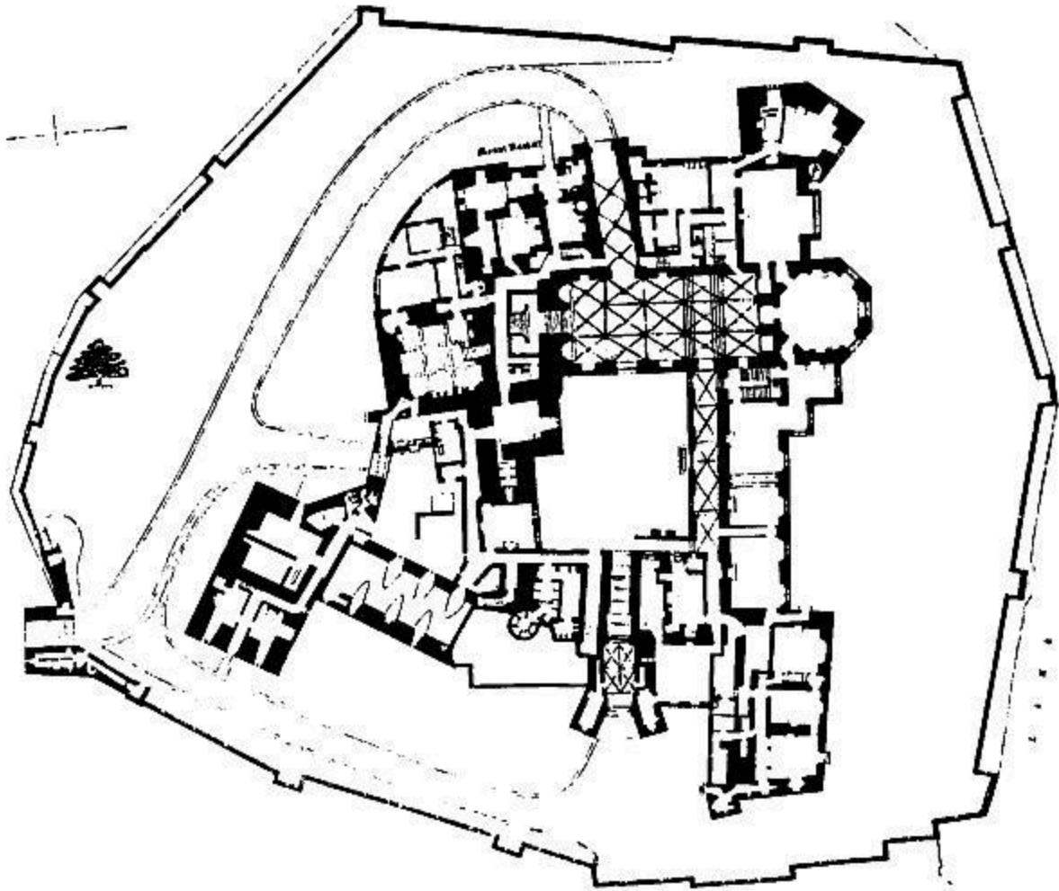
RABY CASTLE, DURHAM GROUND PLAN.
