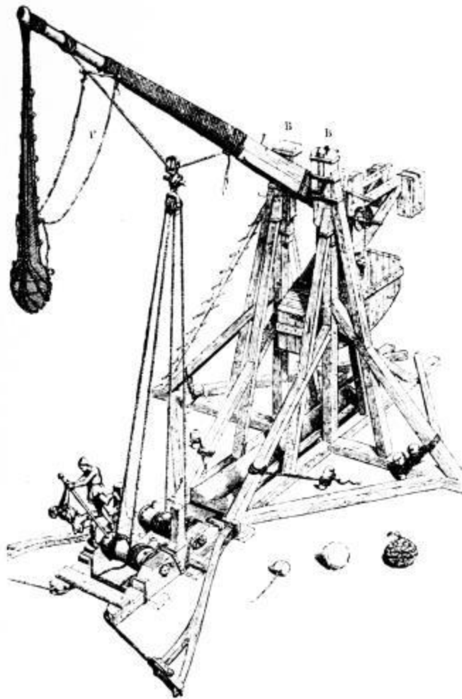
Trébuchet or Slinging machine
