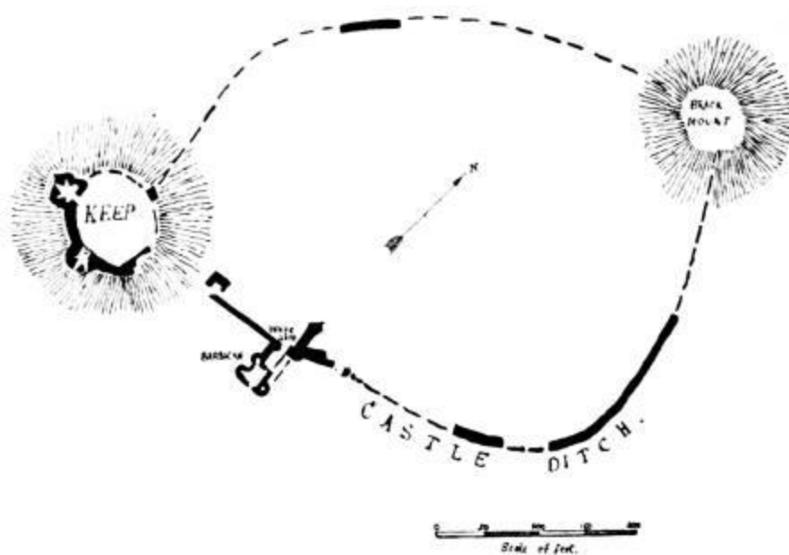
Lewes; Plan
