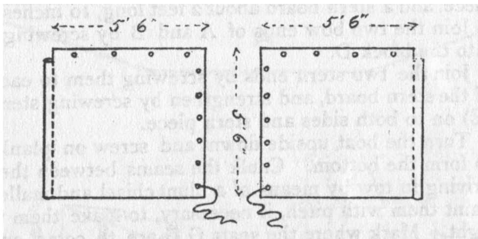
Six squares of canvas, 5ft. 6in. square, with eyelets and hemmed tube on one side. Each Scout carries one, and can pack his kit in it if necessary, or use it as a cape in rain.
