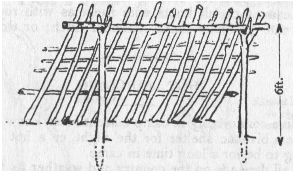
Framework of a Bivouac Shelter, to be thatched with brushwood or grass. A second lean-to roof on opposite side of ridge pole will then make a hut.
