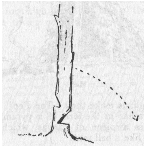
How to Fell a Tree.
