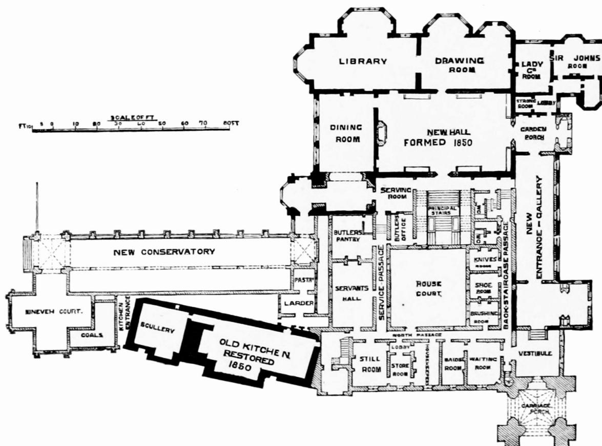
CANFORD MANOR HOUSE, DORSET. GENERAL PLAN, SHEWING THE IMPROVEMENTS AS EXECUTED. ALTERATIONS ARE ETCHED IN LIGHT TINT.
