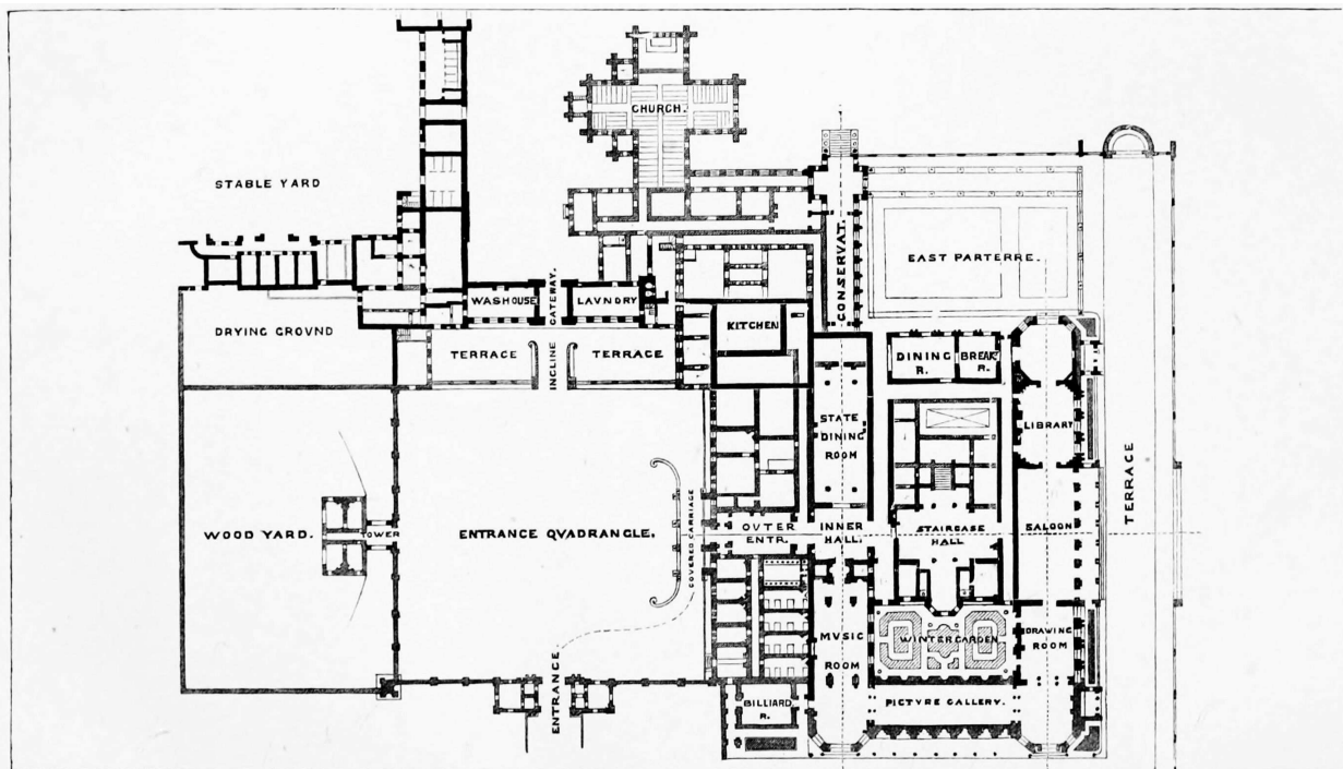
CLUMBER HOUSE, NOTTINGHAMSHIRE. BLOCK PLAN SHEWING SUGGESTED IMPROVEMENT.
