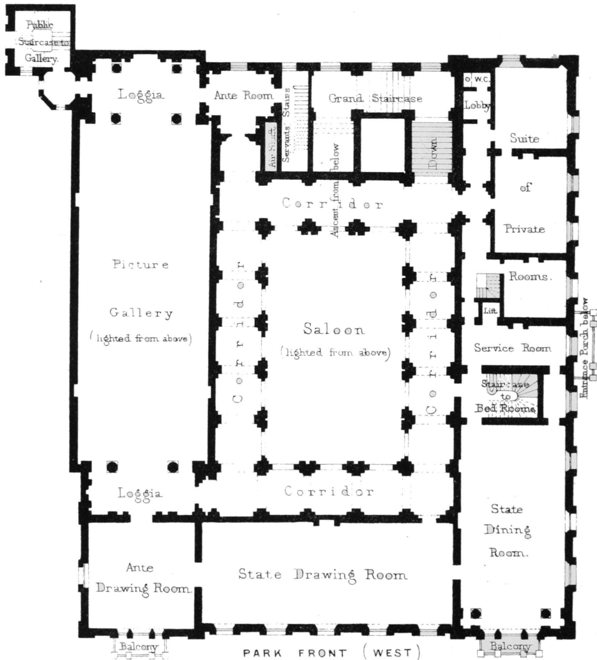
BRIDGEWATER HOUSE. LONDON. PRINCIPAL FLOOR.
