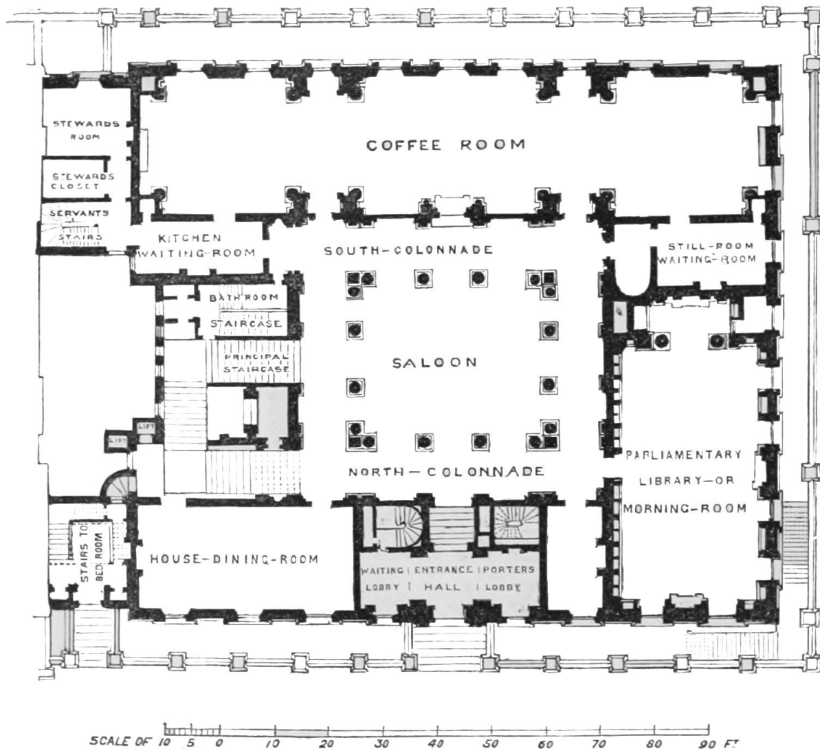
REFORM CLUB HOUSE, PALL MALL, LONDON. PLAN OF THE GROUND FLOOR.
