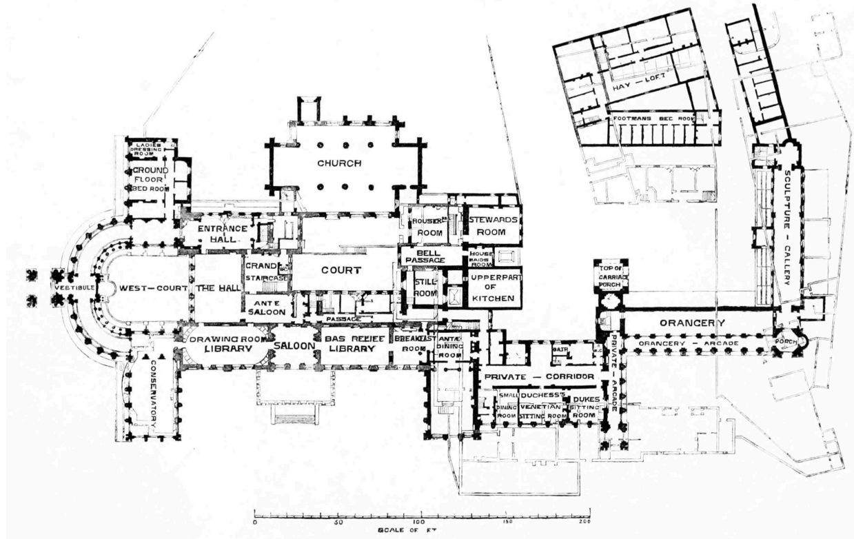
TRENTHAM HALL, STAFFORDSHIRE. THE SEAT OF THE RIGHT HON. THE DUKE OF SUTHERLAND.
