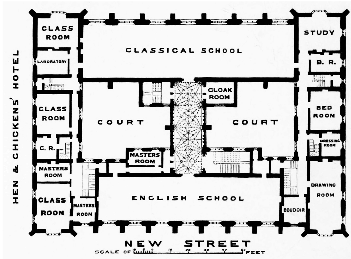
BIRMINGHAM FREE GRAMMAR SCHOOL. PLAN OF ONE PAIR FLOOR.
