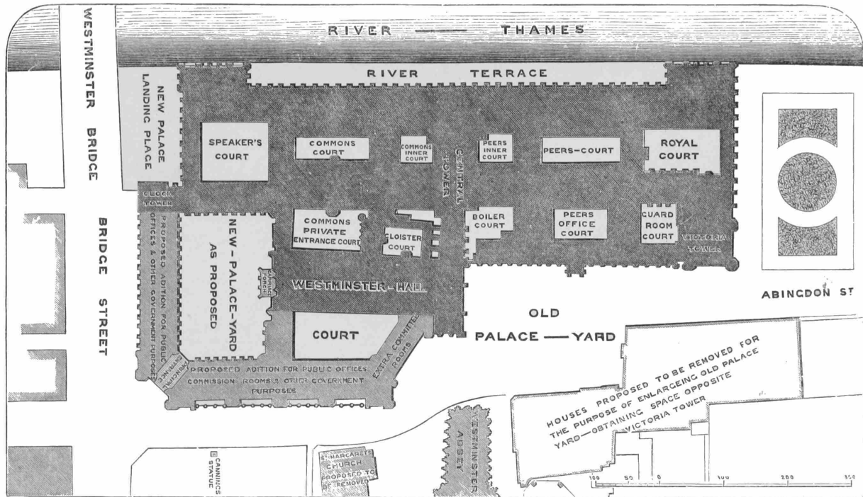
NEW PALACE AT WESTMINSTER. BLOCK PLAN SHOWING SIR CHARLES BARRY'S PROPOSAL FOR ENCLOSING NEW PALACE YARD AND FOR NEW BUILDINGS ON SITE OF THE COURTS OF LAW. THE BUILDING AS EXECUTED IS SHOWN BY THE DARK TINT.
