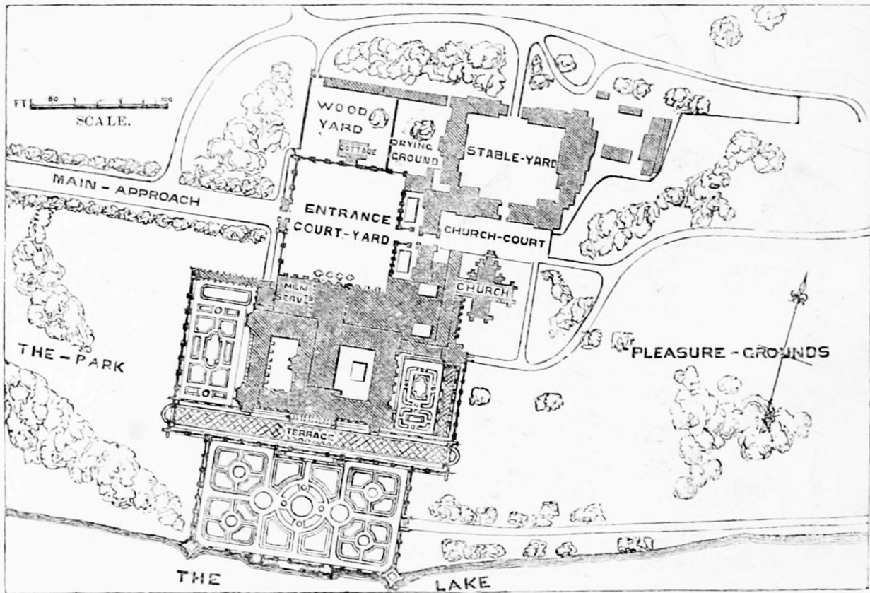
CLUMBER HOUSE, NOTTINGHAMSHIRE. BLOCK PLAN SHEWING SUGGESTED IMPROVEMENT.
