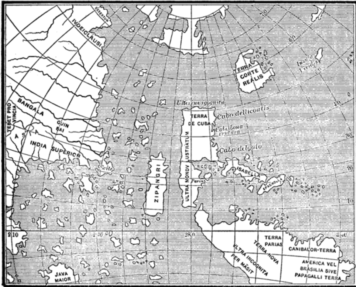
SCHÖNER'S GLOBE, 1520.
