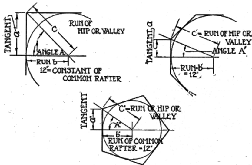
Fig. 68. Tangents
