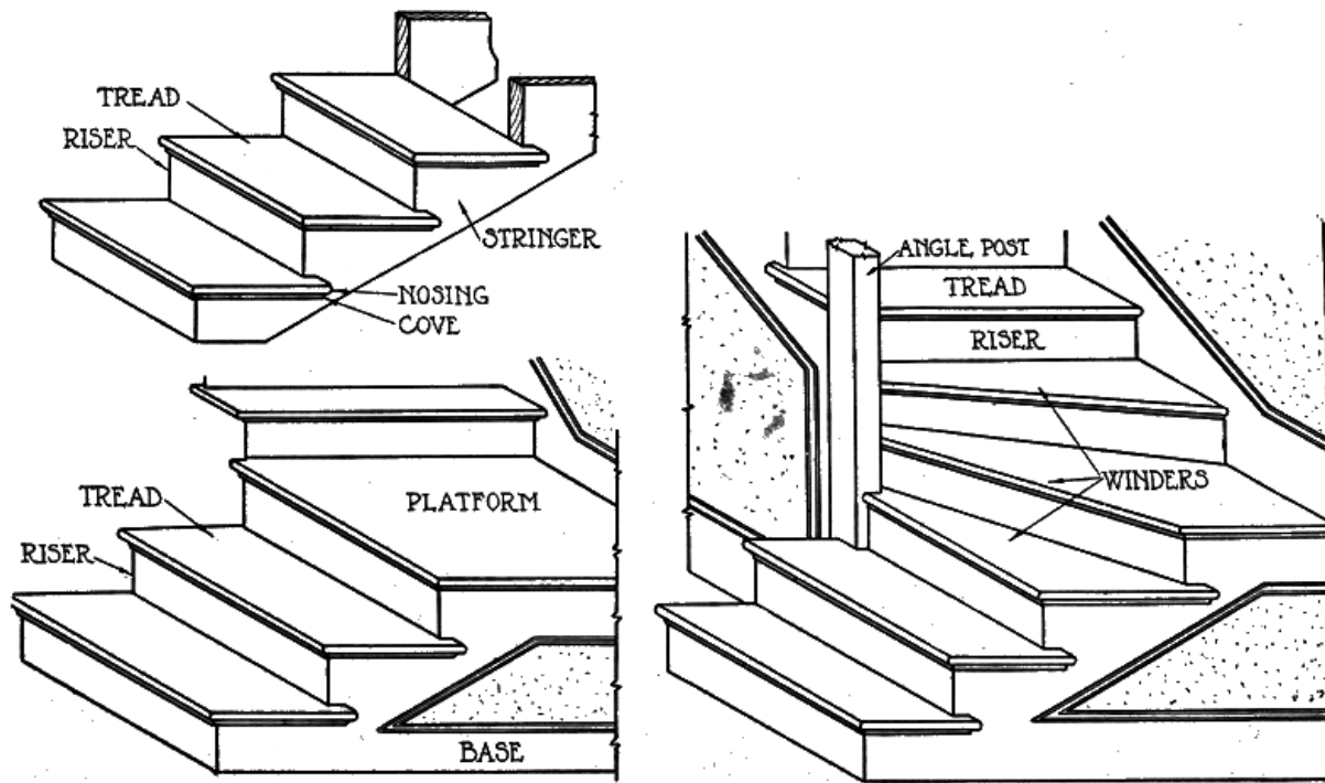
Fig. 120-a-b Types of Stairs Fig. 120-c
