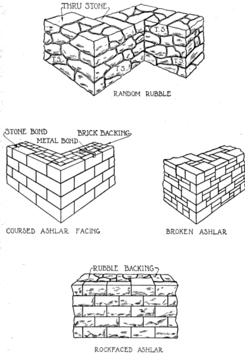
Fig. 11. Types of Stone Work
