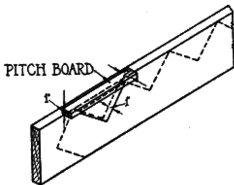
Fig. 123. Pitch Board.
