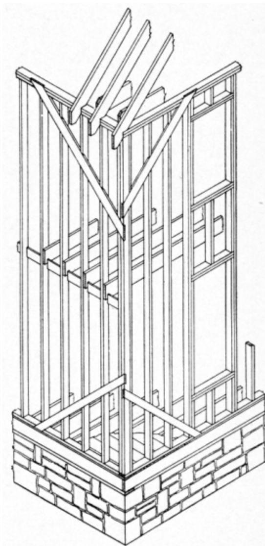
Fig. 19. Balloon Frame House
