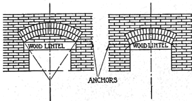
Fig. 150. Lintels
