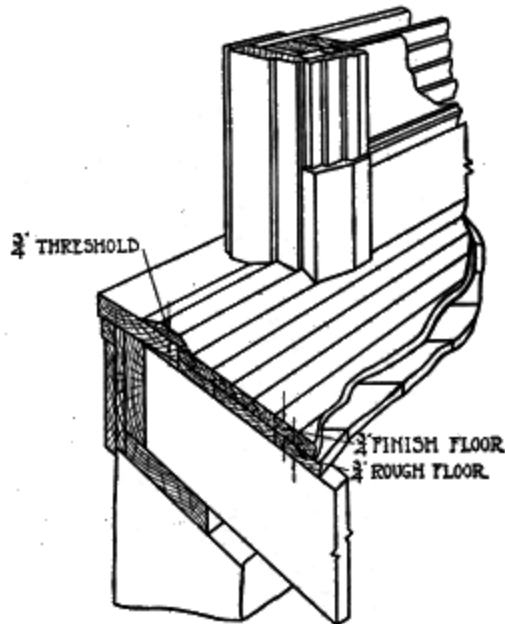
Fig. 38. Threshold Detail
