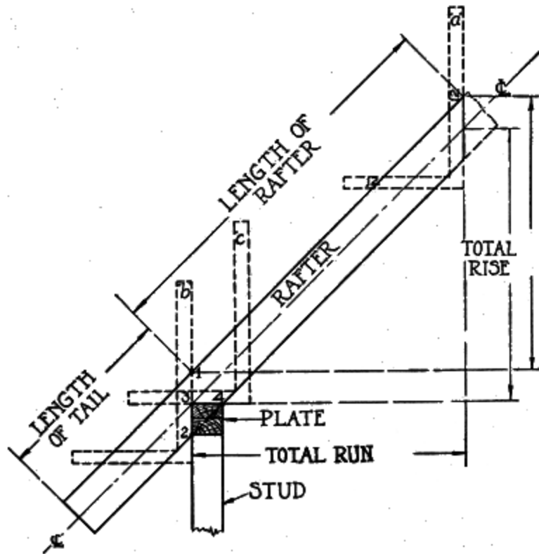
Fig. 52. Laying out Rafter
