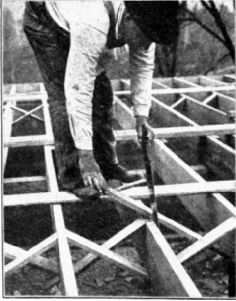
Fig. 23. Cutting Bridging
