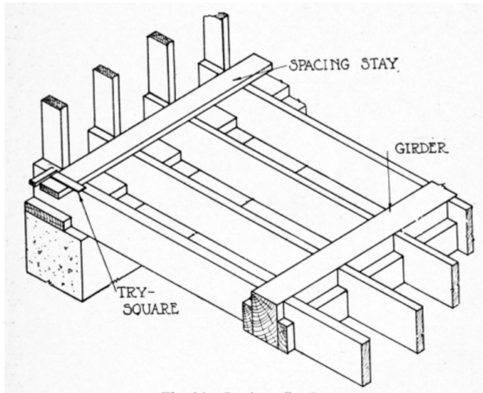
Fig. 24. Laying off a Stay
