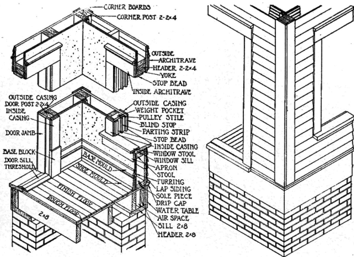
Fig. 110-a. Interior Wall Detail
