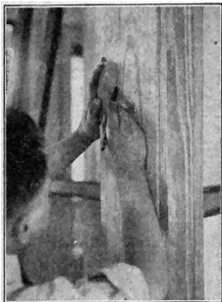
Fig. 131. Using Block to Locate Door Stop Position on Jamb
