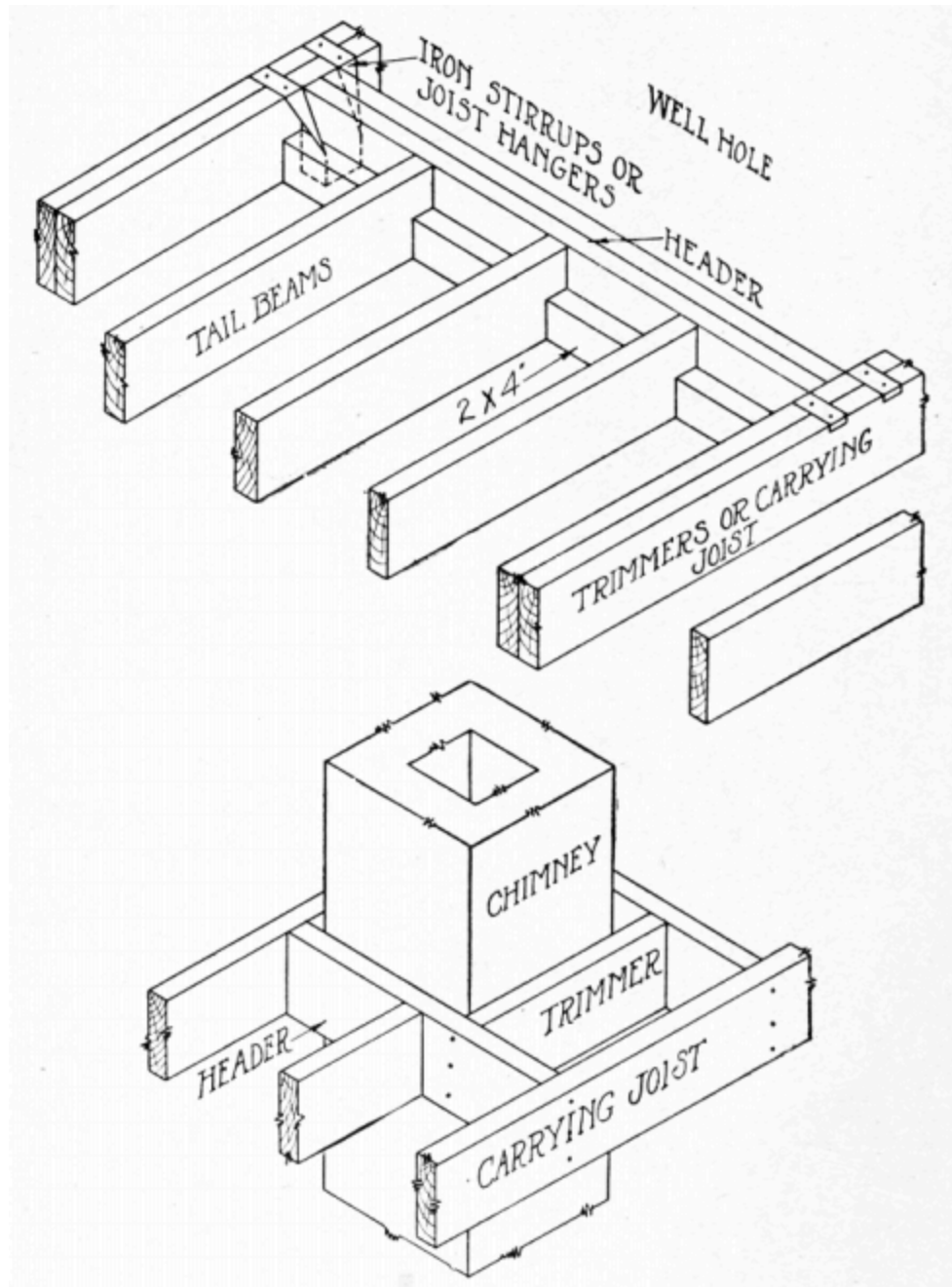
Fig. 25-a-b. Headers and Trimmers in Floor Frame
