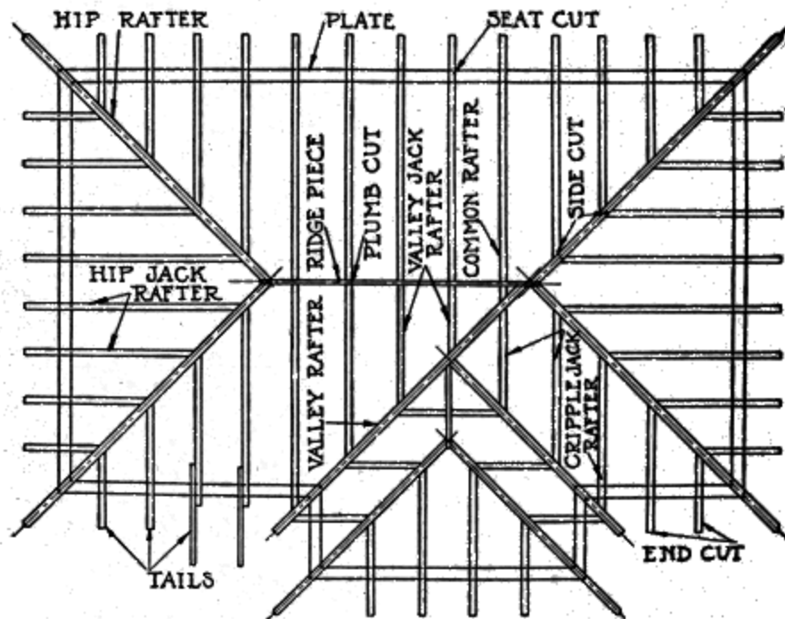
Fig. 41. Plan of Roof Rafters
