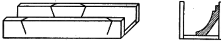
Fig. 99. Miter Box for Raked Gable Moulding Cut at Eaves
