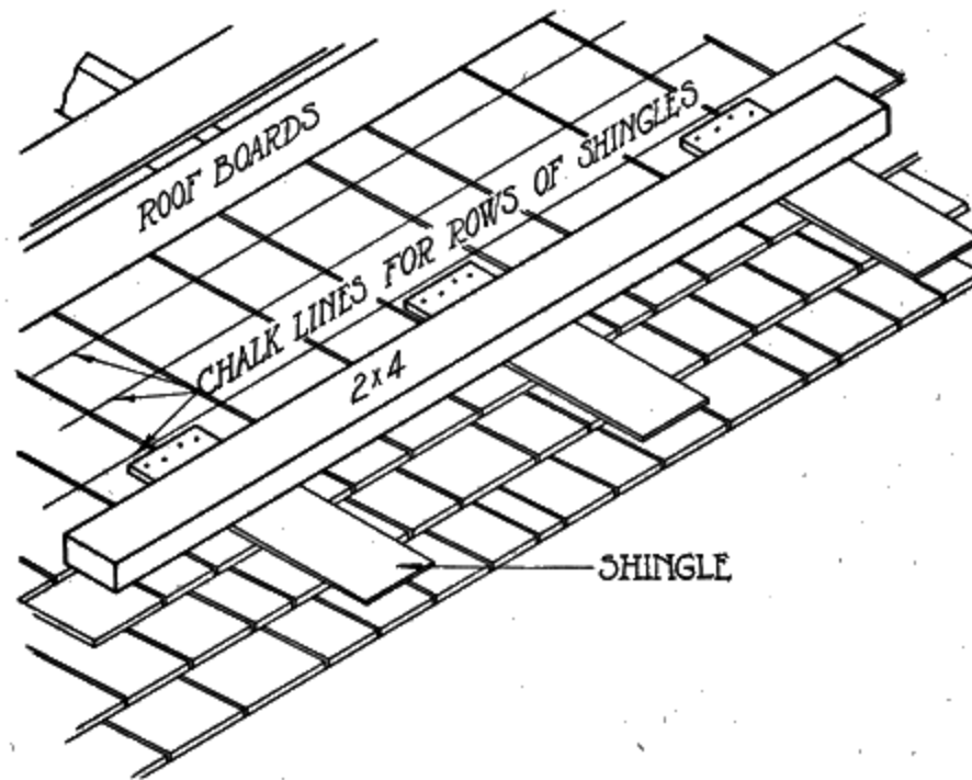
Fig. 103. Shingling. Toe Hold
