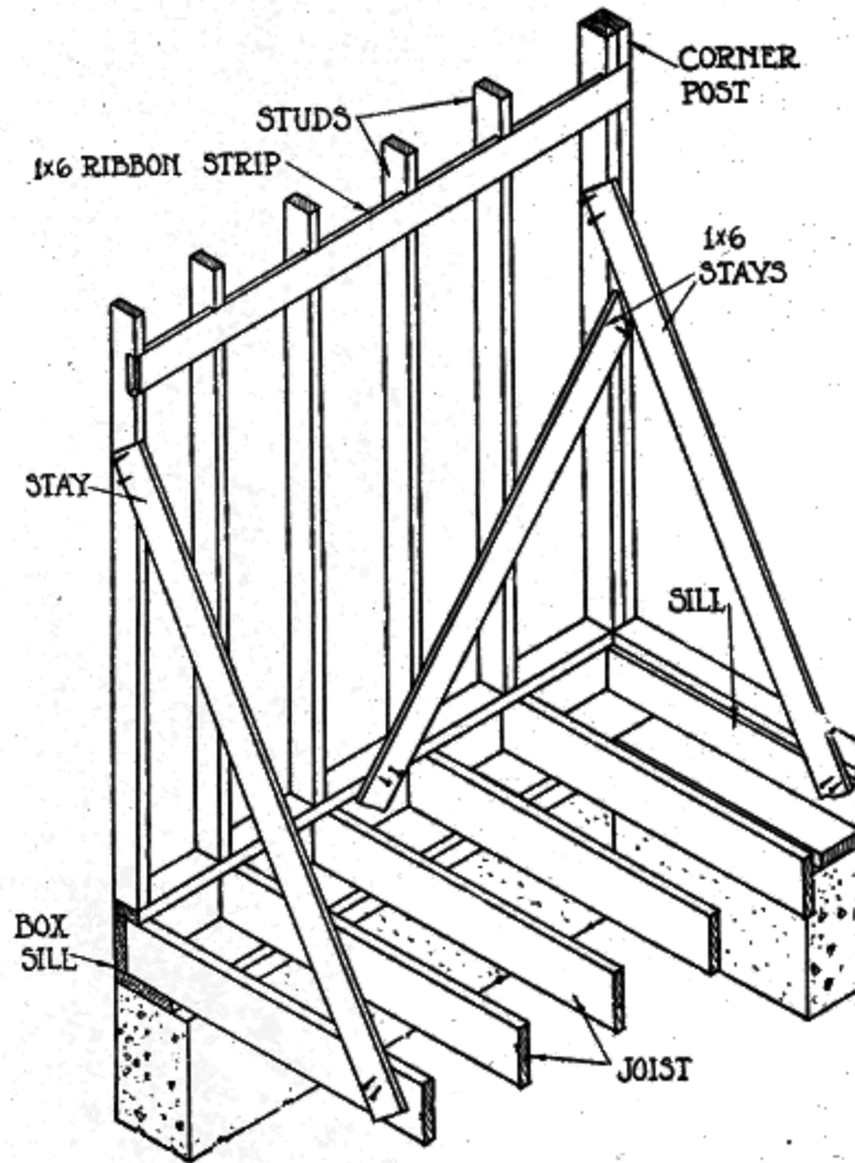
Fig. 34. Side Wall Stayed
