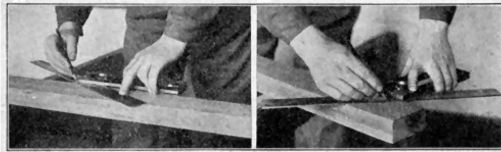
Fig. 79. Laying off Seat Cut with Fig. 80 . Laying off Plumb Cut with Framing Tool Framing Tool
