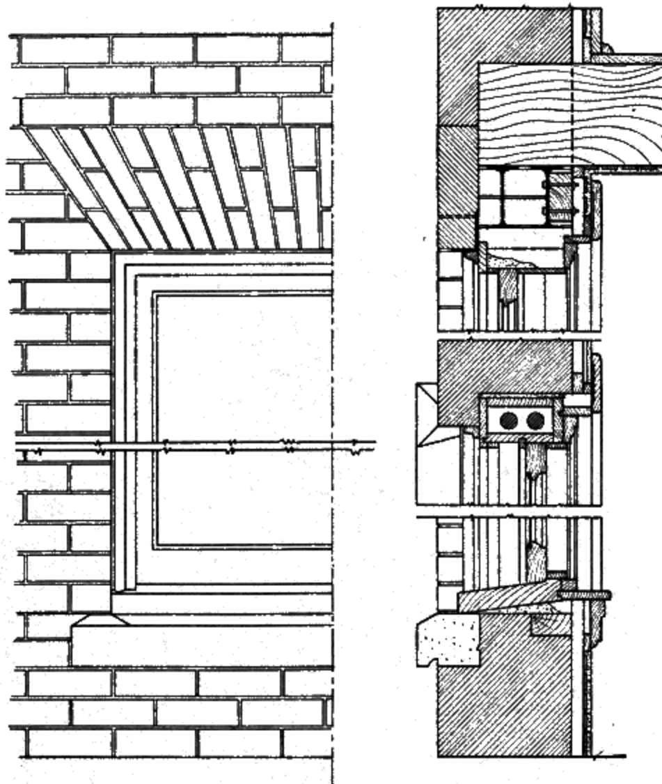
Fig. 149. Window Detail for Brick Wall
