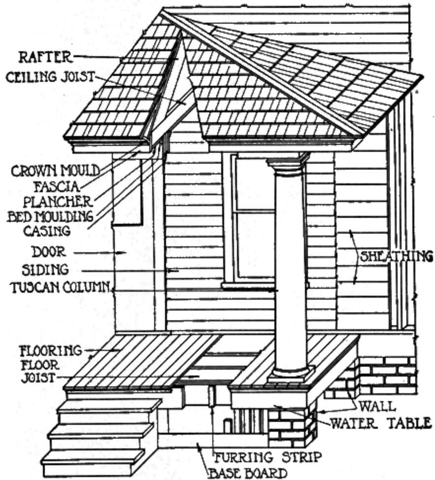
Fig. 128. Detail of Porch Finish
