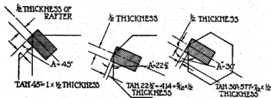
Fig. 78. Backing for Hip of any Polygon
