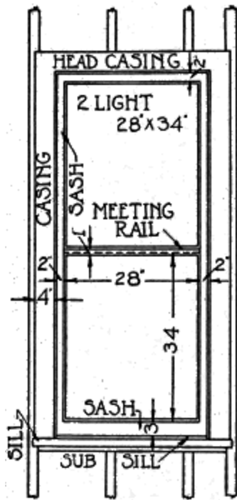
Fig. 36. Estimating Window Openings
