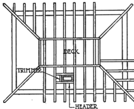
Fig. 89. Deck Frame
