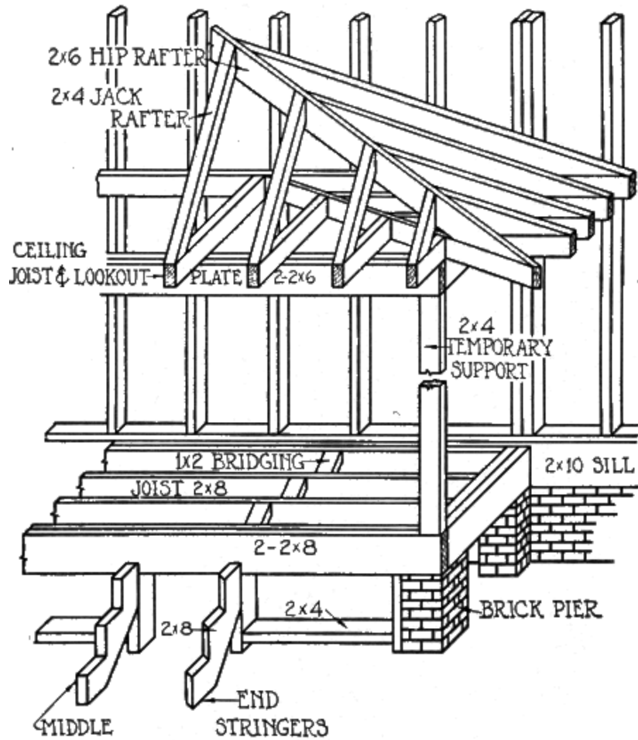
Fig. 127. Detail of Porch Framing
