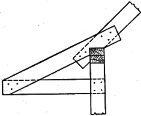
Fig. 53. Independent Rafter Tail
