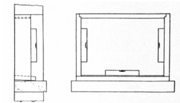
Fig. 15. Plumbing and Leveling Cellar Frame
