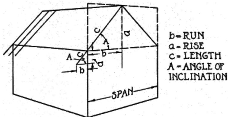
Fig. 43. Run, Rise and Length
