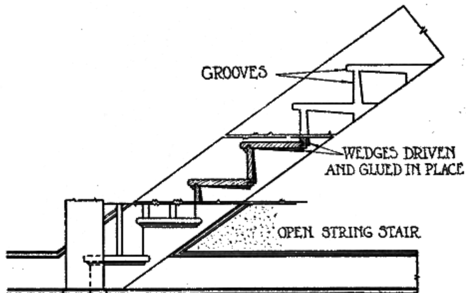
Fig. 126. Main Stair Detail
