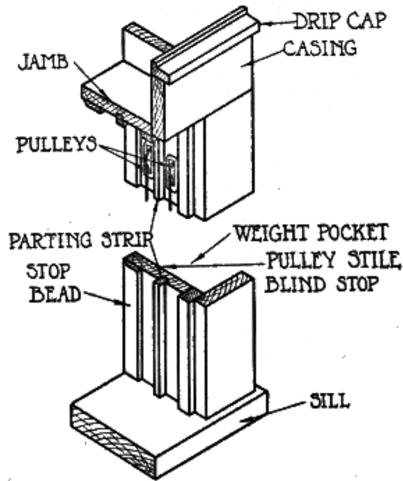
Fig. 146. Detail of Window Frame
