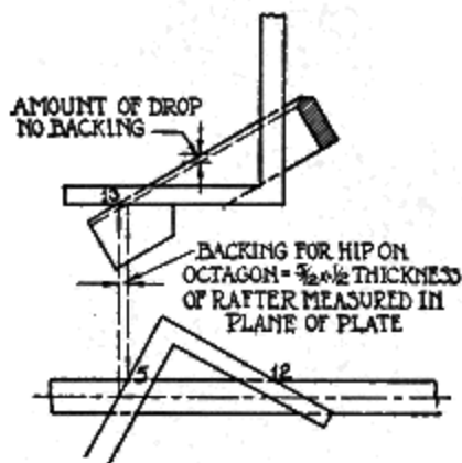
Fig. 77. Laying out Backing for Octagon Hip
