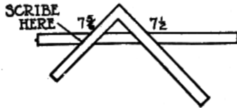
Fig. 88-b. Fig. 88-c. Side Cuts of Jacks for Uneven Pitches
