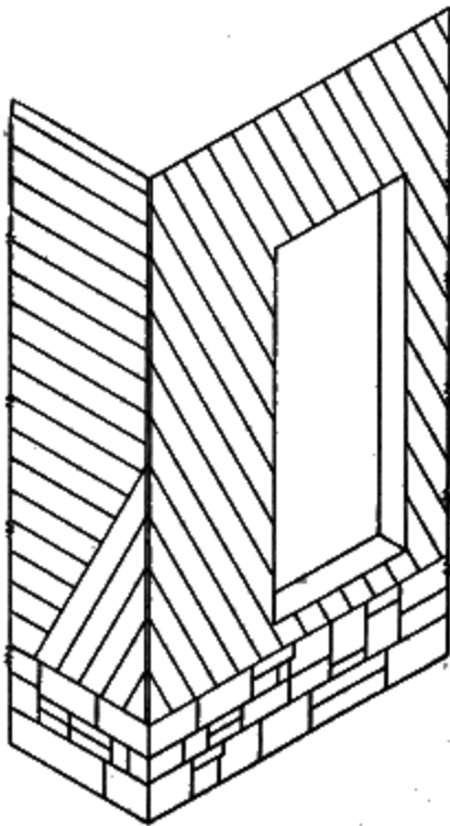
Fig. 90. Sheathing
