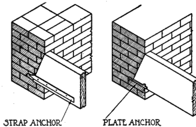
Fig. 147-a Fig. 147-b Joist Framed into Brick Wall
