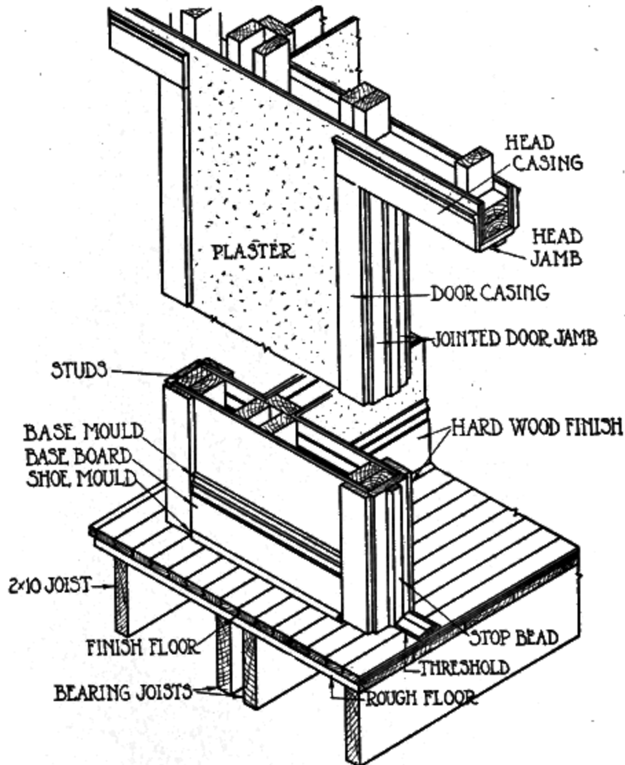
Fig. 119. Detail of Partition Wall
