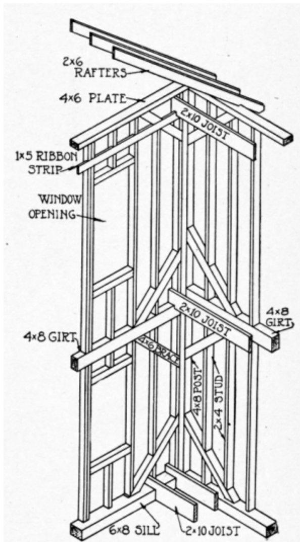
Fig. 16. Full Frame House
