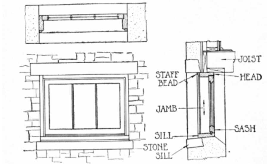
Fig. 13. Cellar Frame with Sash
