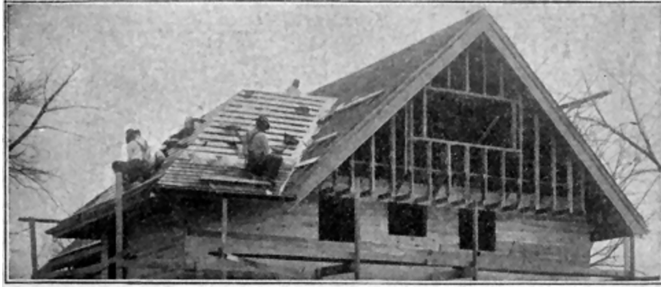
Fig. 107. Shingling Valley
