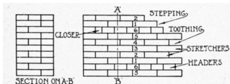
Fig. 8. American Bond
