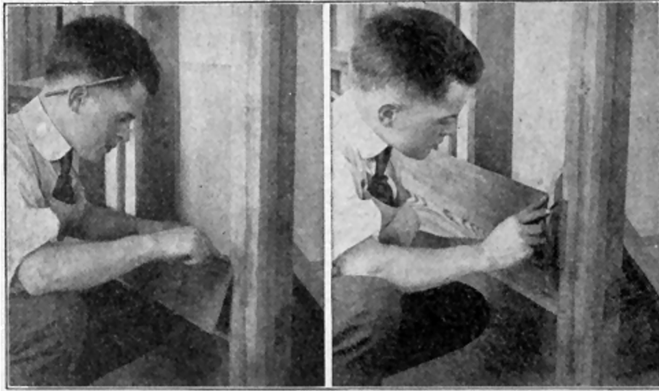
Fig. 114. Marking Length of Siding
