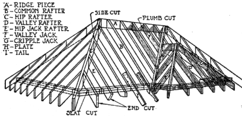
Fig. 40. Roof Details
