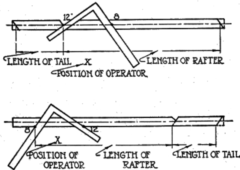
Fig. 45-a-b. Laying off Common Rafter
