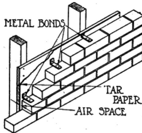
Fig. 148. Brick Veneer
