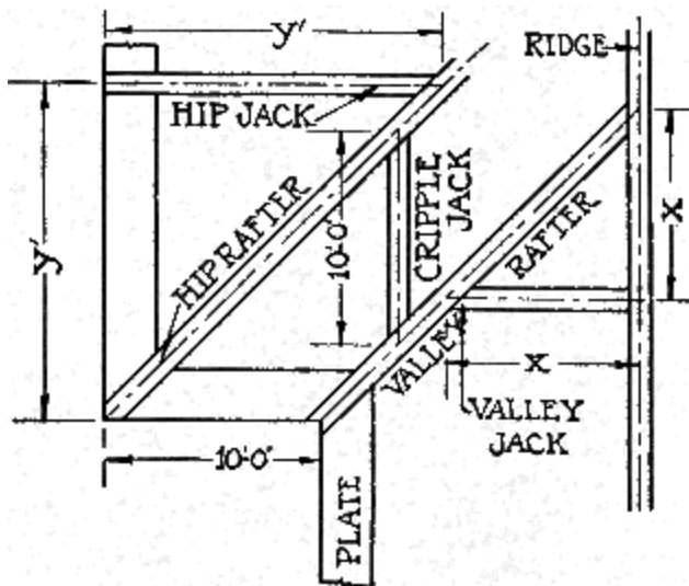
Fig. 66. Lengths of Jack Rafters.
