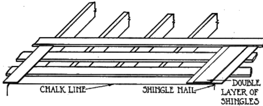
Fig. 102. Beginning Course
