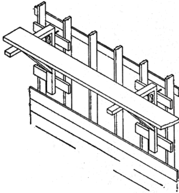
Fig. 94. Scaffold Bracket
