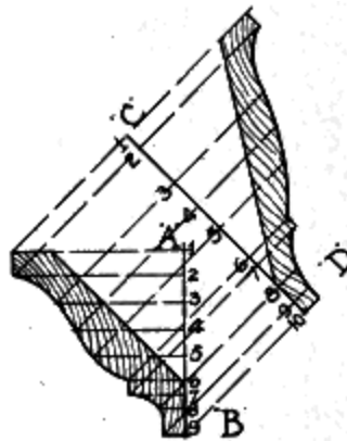
Fig. 98. Laying out Gable or Raked Moulding
