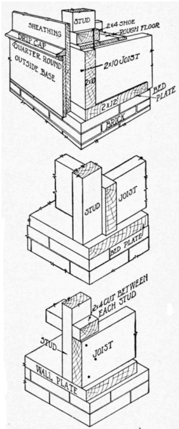
Fig. 21. Three Types of Box Sills
