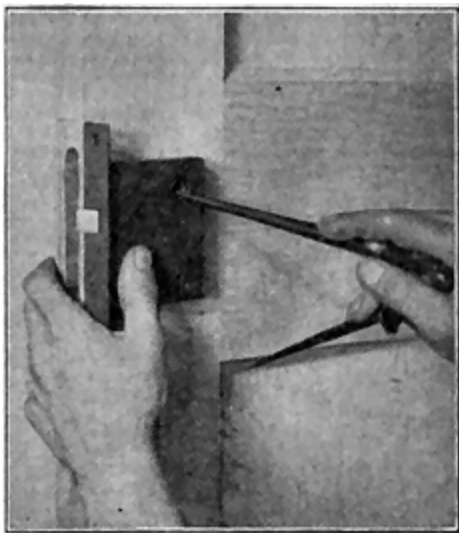
Fig. 142. Locating Knob Spindle Hole
