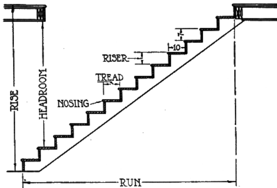
Fig. 121. Rise and Run of Stair
