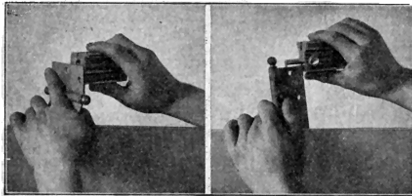
Fig. 137. Setting Gage for Depth of Gain
