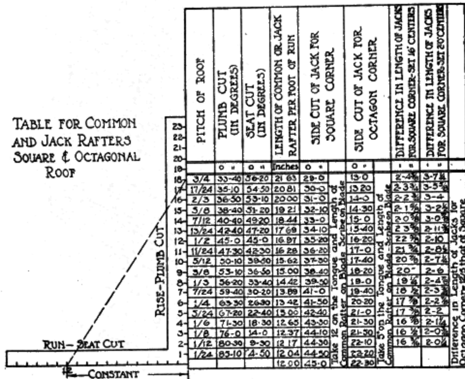
Fig. 49. Framing Table for Common Rafter
