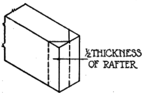
Fig. 63. Miter Cut of Hip Rafter End
