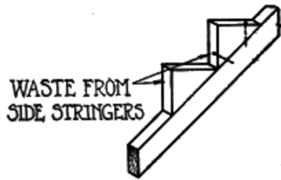
Fig. 124. Economical Center Stringer
