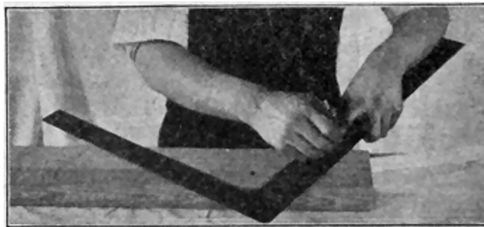
Fig. 46. Position in Laying off Plumb Cut when Laid off before Seat Cut
