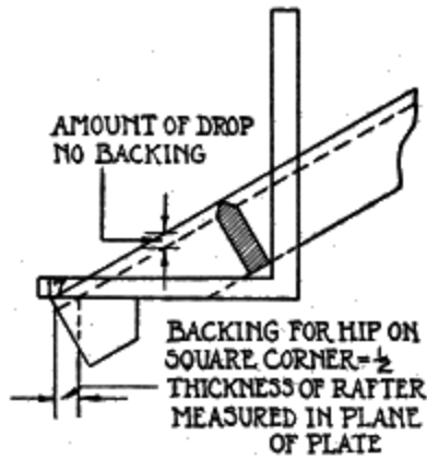
Fig. 64. Backing the Hip Rafter
