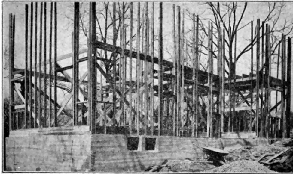
Fig. 29. Headers and Trimmers in Wall Frame
