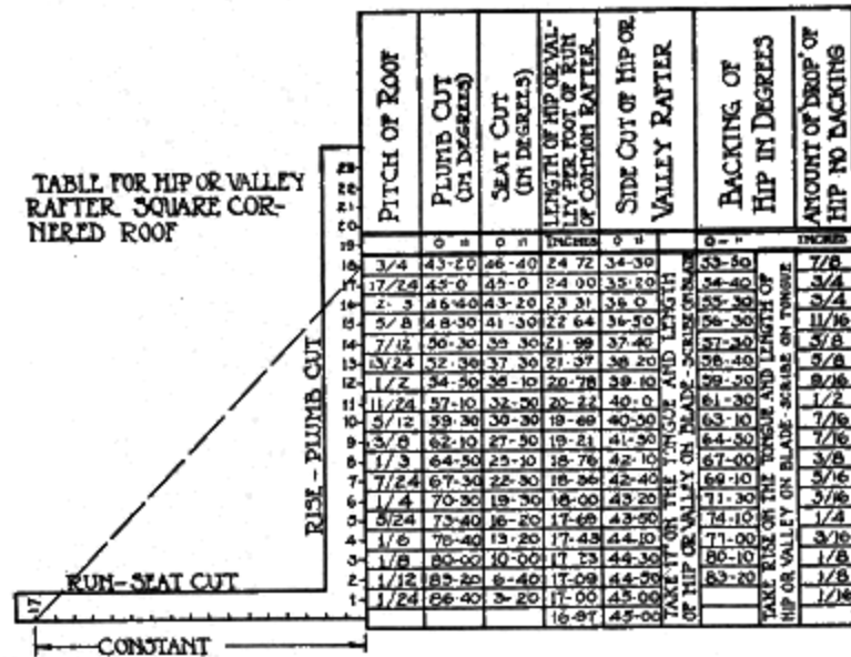
Fig. 60. Framing Table for Hip or Valley Rafters
