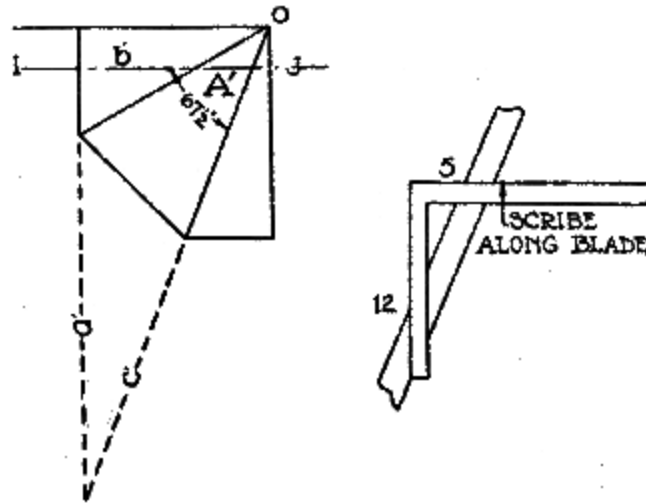
Fig. 84-a. Fig. 84-b. Framing Octagon Hip Intercepted at 67\frac{1}{2}^\circ
