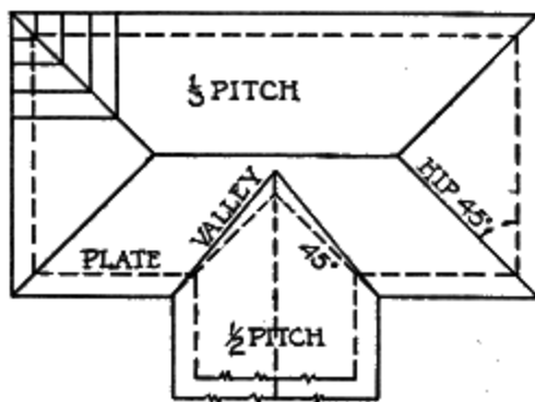
Fig. 87. Plan of Uneven Pitches
