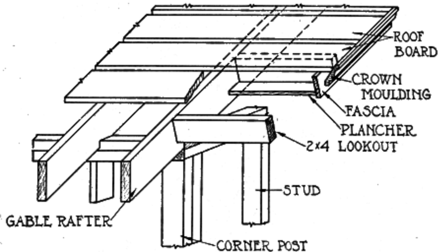
Fig. 97-b. Box Cornice.
