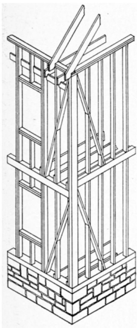
Fig. 18. Half-Frame House
