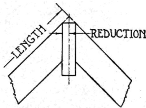
Fig. 56. Reduction of Common Rafter for Ridge Piece.
