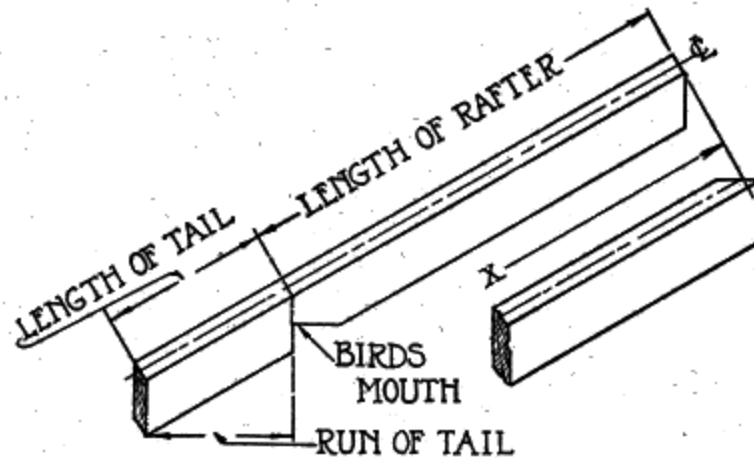
Fig. 48. Rafter Length
