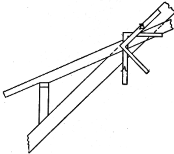
Fig. 86. Laying off Cut of Shed Rafter
