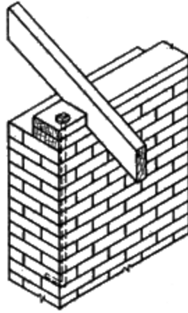
Fig. 151. Attaching Plate to Brick Wall
