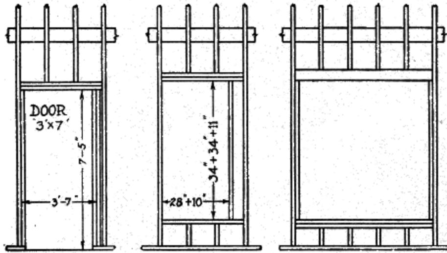
Fig. 37. Framing Wall Openings
