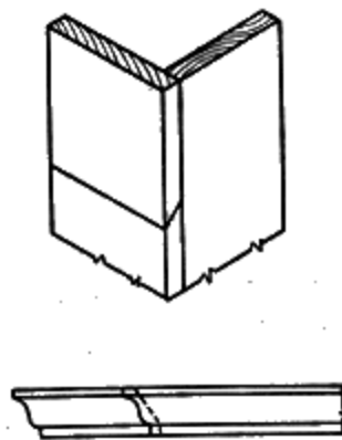
Fig. 101. Spliced Corner Boards and Moulding
