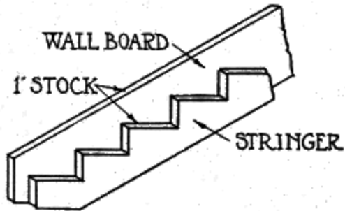
Fig. 125. Stringer for Attic Stair
