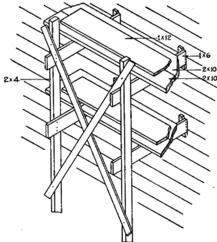
Fig. 93. Scaffolding
