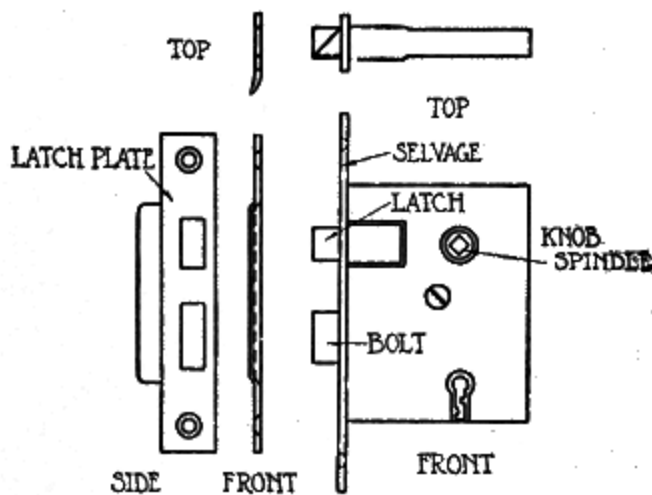
Fig. 141. Mortise Lock
