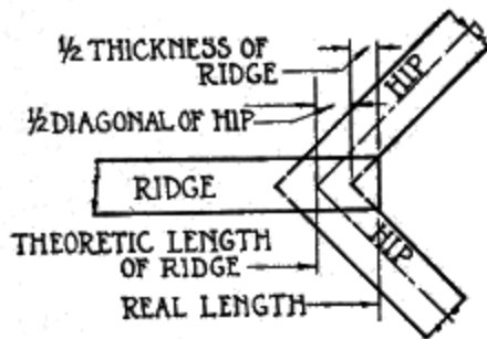
Fig. 54. Length of Ridge Piece
