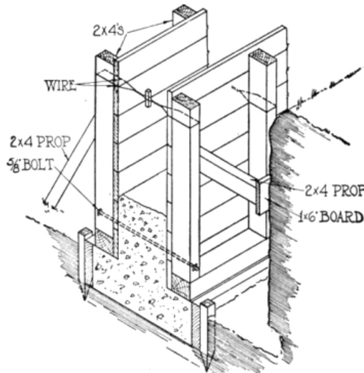
Fig. 12. "Form" for Concrete
