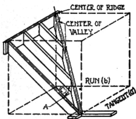
Fig. 58-b. Valley Rafter
