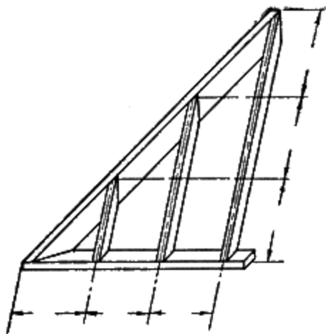
Fig. 67. Determining Length of Jack Rafters
