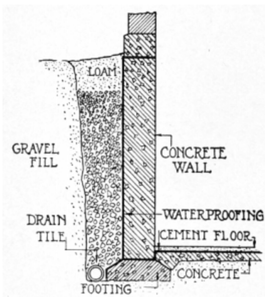
Fig. 7. Foundation Detail
