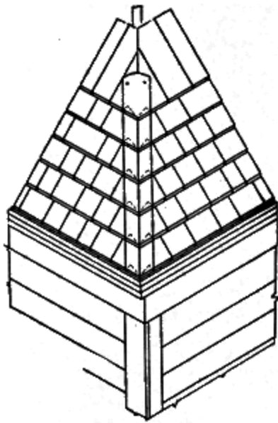
Fig. 105. Shingle Tins Fig. 106. Valley
