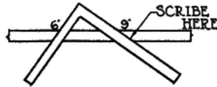
Fig. 88-b. Fig. 88-c. Side Cuts of Jacks for Uneven Pitches
