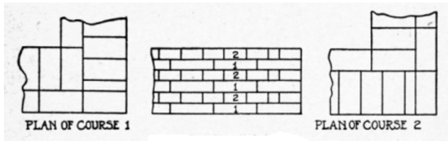
Fig. 9. English Bond
