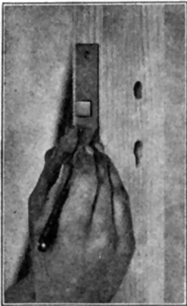
Fig. 143. Locating Selvage Gain
