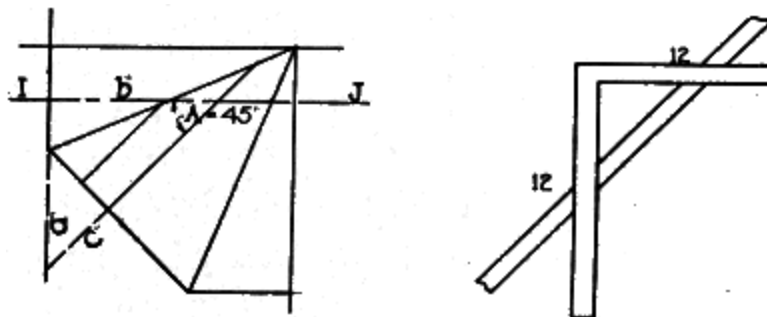
Fig. 85-a. Fig. 85-b. Framing an Intercepted Jack
