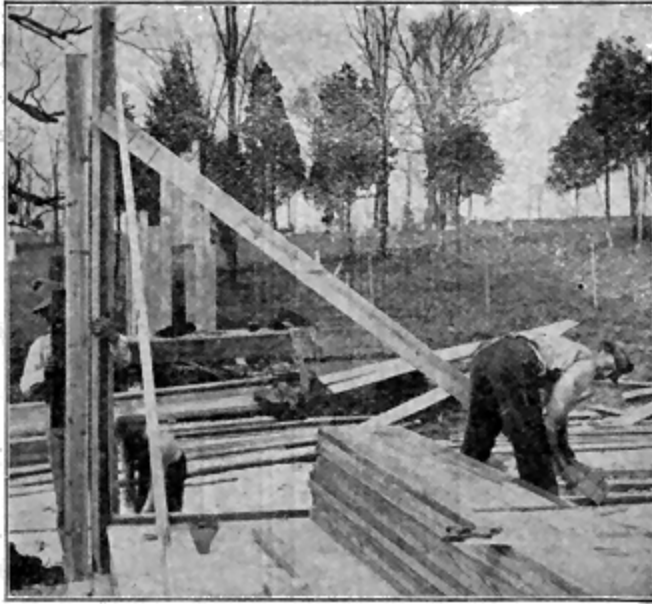
Fig. 33. Corner Post Being Plumbed and Stayed
