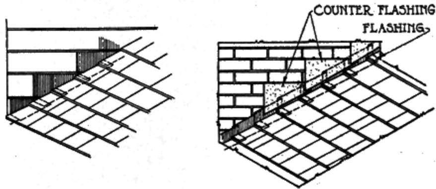
Fig. 108. Flashing Fig. 109. Flashed and Counter-flashed
