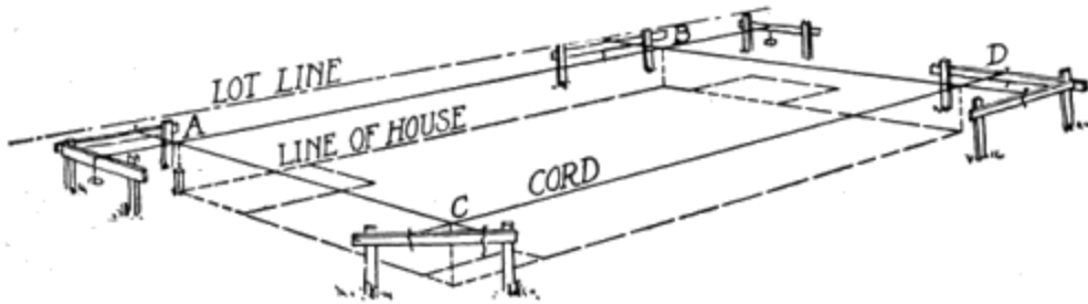
Fig. 4. Batter Boards
