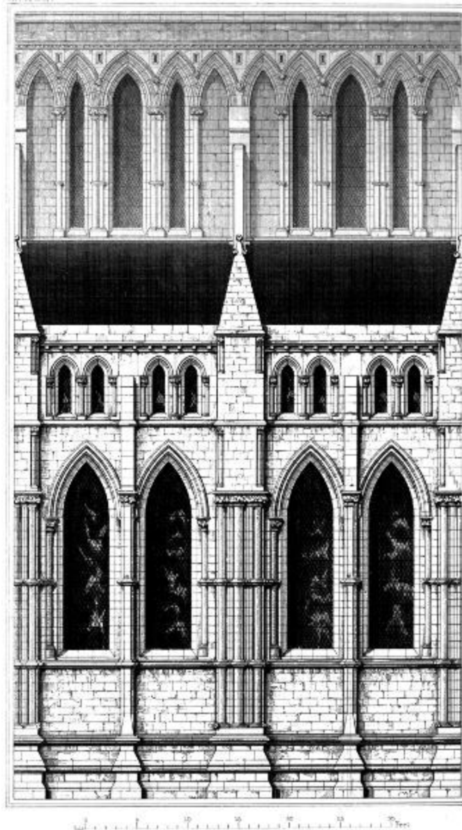
Exterior LINCOLN CATHEDRAL. Choir
