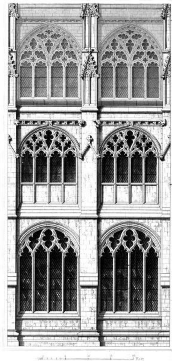
Exterior ELY CATHEDRAL. Choir
