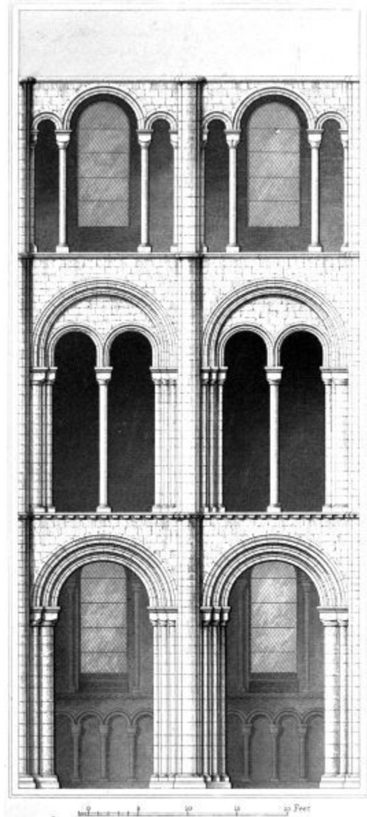
Interior ELY CATHEDRAL. Nave
