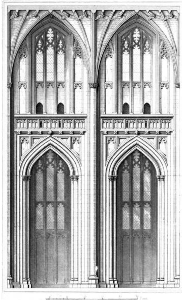
Interior WINCHESTER CATHEDRAL. Nave
