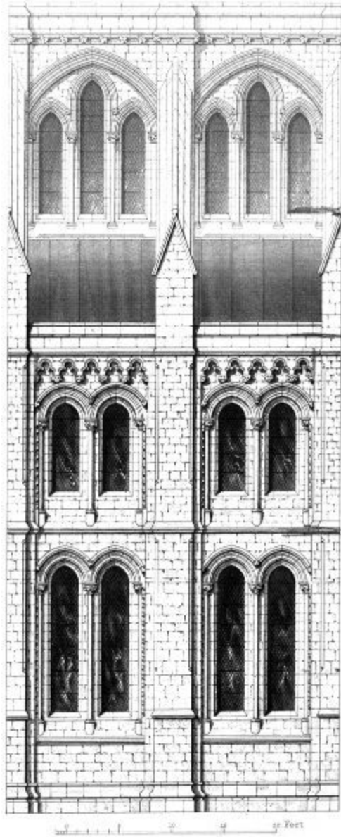
Exterior ELY CATHEDRAL. Presbytery
