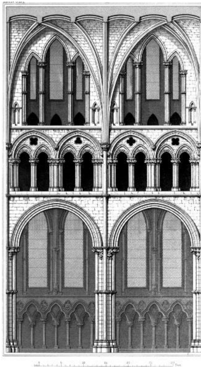
Interior LINCOLN CATHEDRAL. Choir
