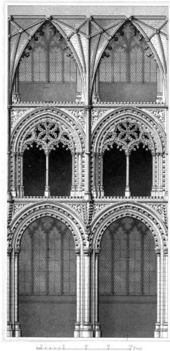
Interior ELY CATHEDRAL. Choir
