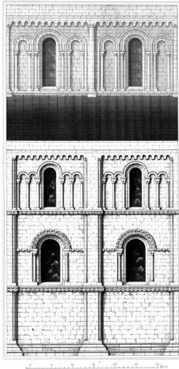
Exterior PETERBOROUGH CATHEDRAL. Choir
