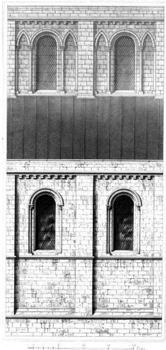
Exterior RIPON CATHEDRAL. Choir
