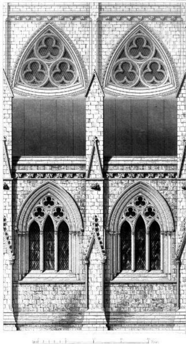
Exterior LICHFIELD CATHEDRAL. Nave
