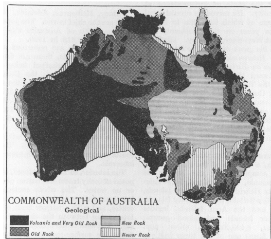
COMMONWEALTH OF AUSTRALIA Geological
