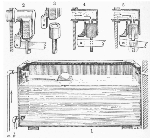
Ball-cock
