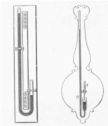
Siphon Barometer; Wheel Barometer
