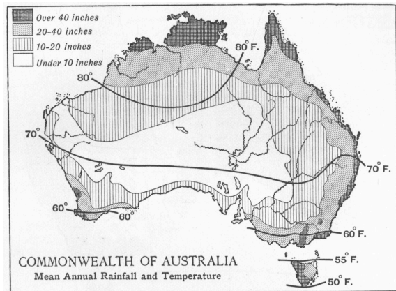
COMMONWEALTH OF AUSTRALIA Mean Annual Rainfall and Temperature
