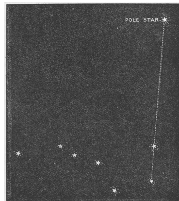
The Constellation of the Great Bear. The two stars on the right are the Pointers
