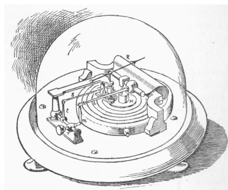
Aneroid Barometer
