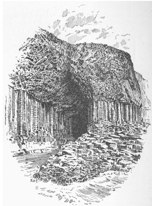
Basaltic Columns, Fingal's Cave, Island of Staffa
