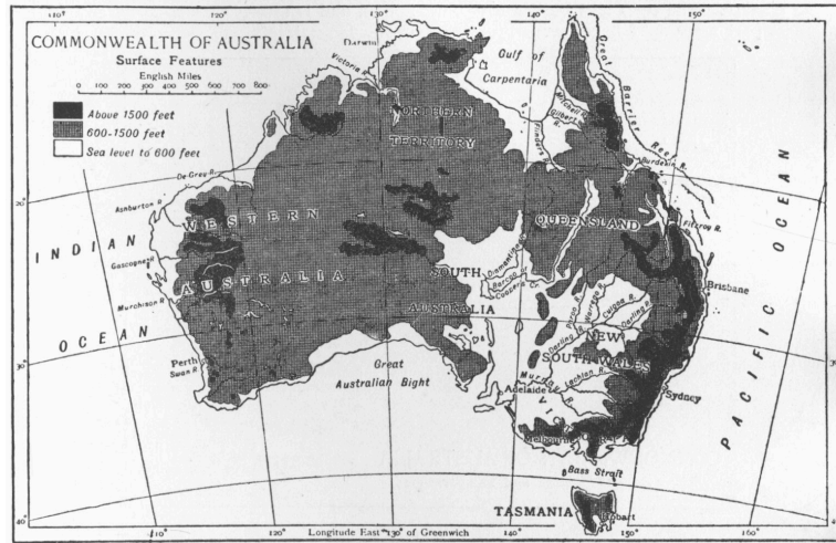
COMMONWEALTH OF AUSTRALIA Surface Features
