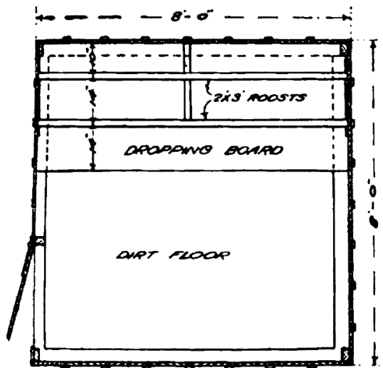
FLOOR PLAN
