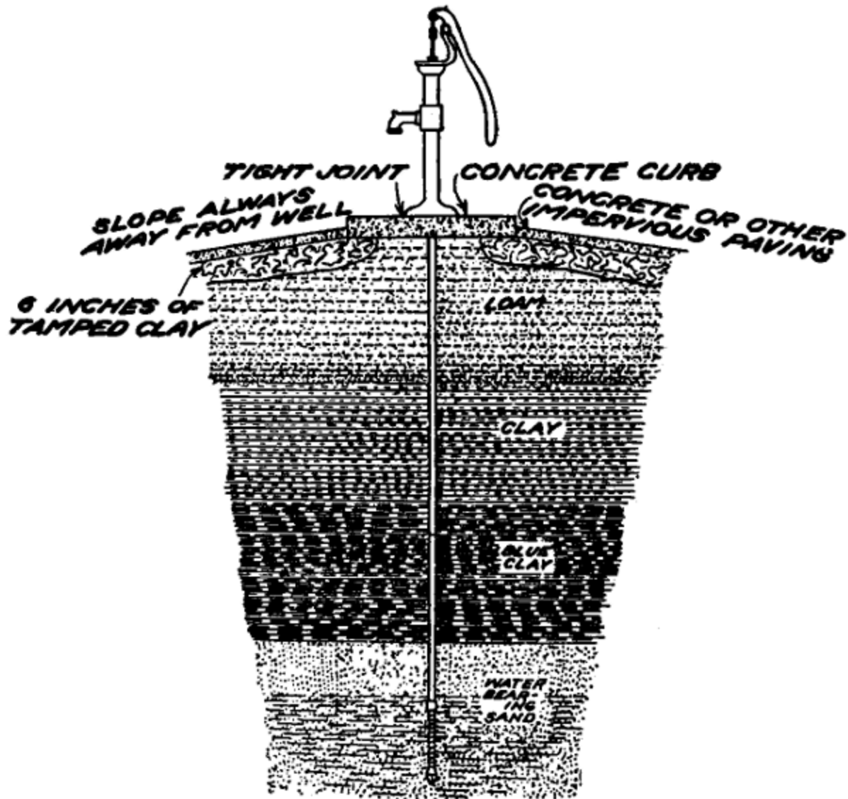
Fig. 20.—Driven well.
