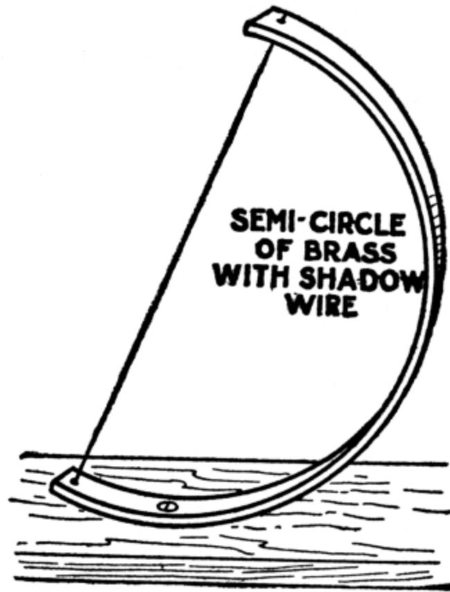
FIG. 47.—BRASS SEMI-CIRCLE WITH SHADOW WIRE.
