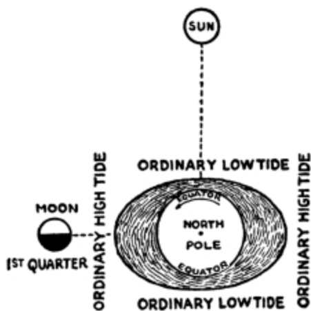
FIG. 115.—How NEAP TIDES ARE FORMED.
