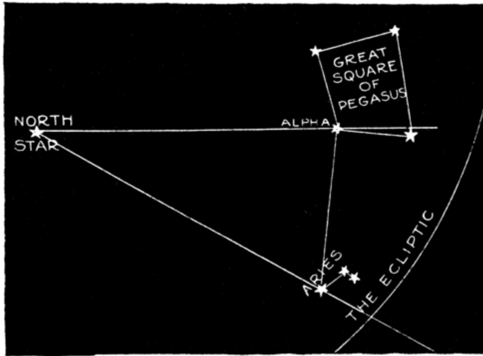
FIG. 175.—CONSTELLATIONS OF ARIES THE RAM.
