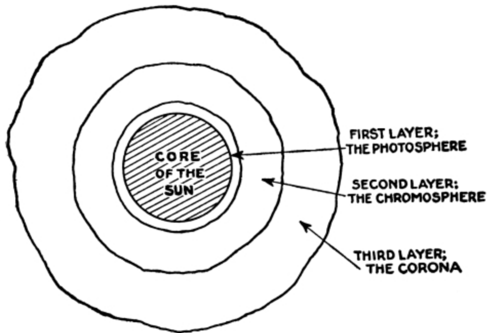
FIG. 33.—CROSS SECTION OF THE SUN.
