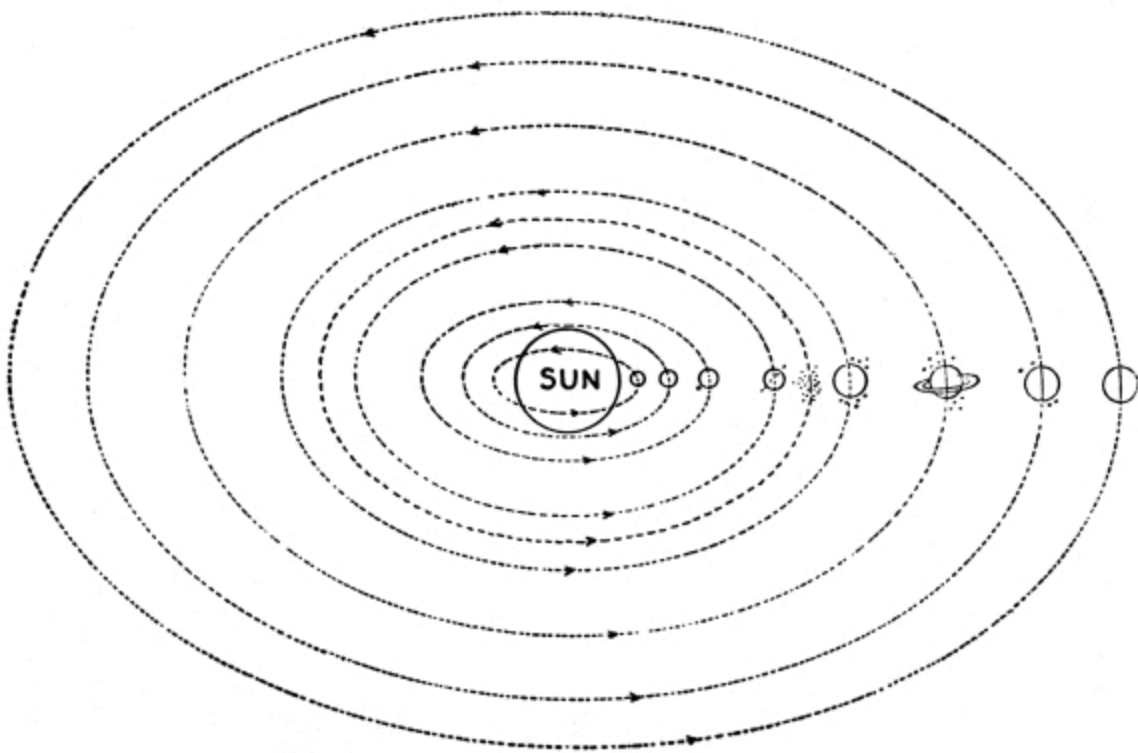
FIG. 62.—SOLAR SYSTEM IN PERSPECTIVE.
