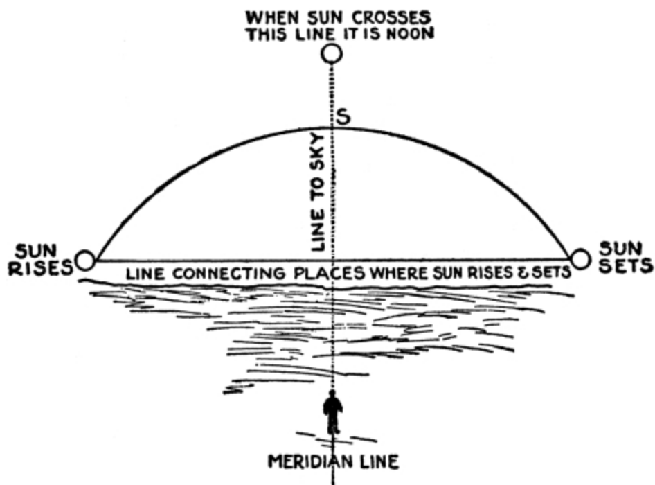
FIG. 162.—DIAGRAM SHOWING HOW TO FIND SOLAR NOON.
