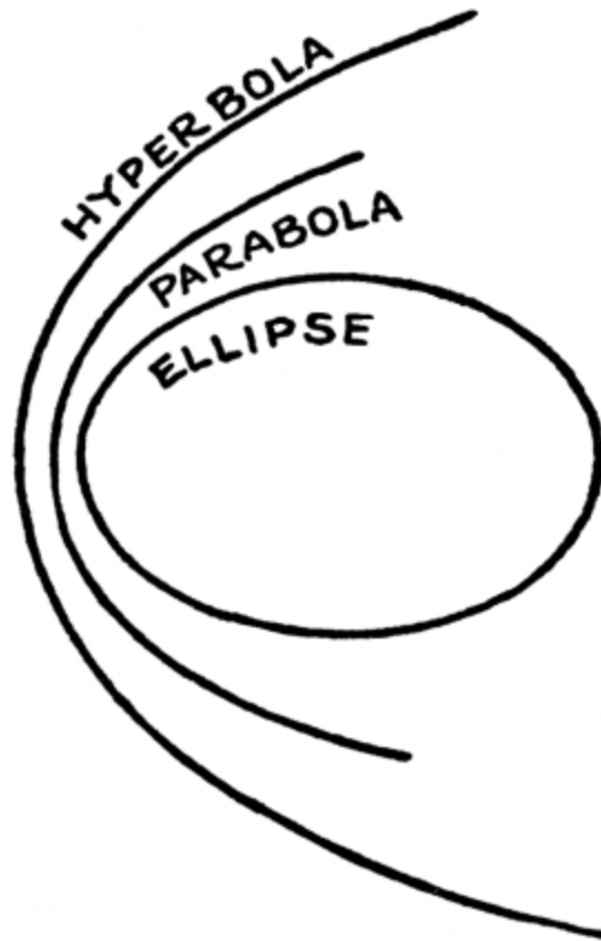
FIG. 129.—AN ELLIPSE, PARABOLA AND HYPERBOLA.
