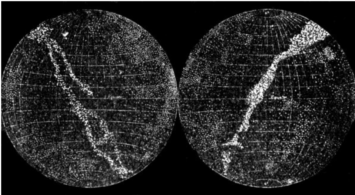
FIG. 133.—THE MILKY WAY.
