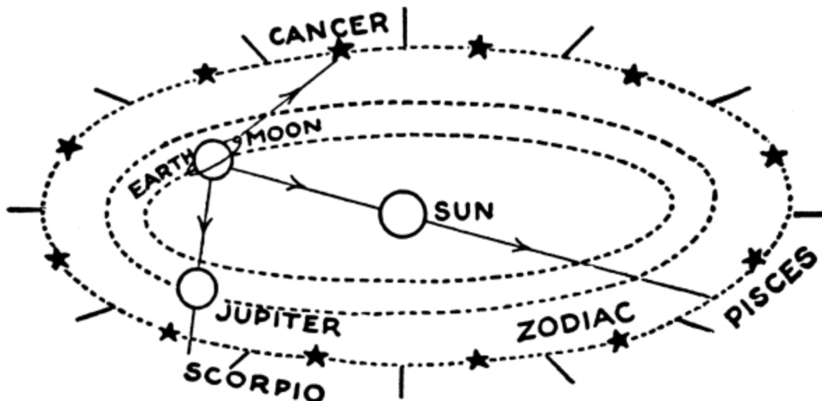
FIG. 171.—THE ZODIAC AS WE KNOW IT TODAY.
