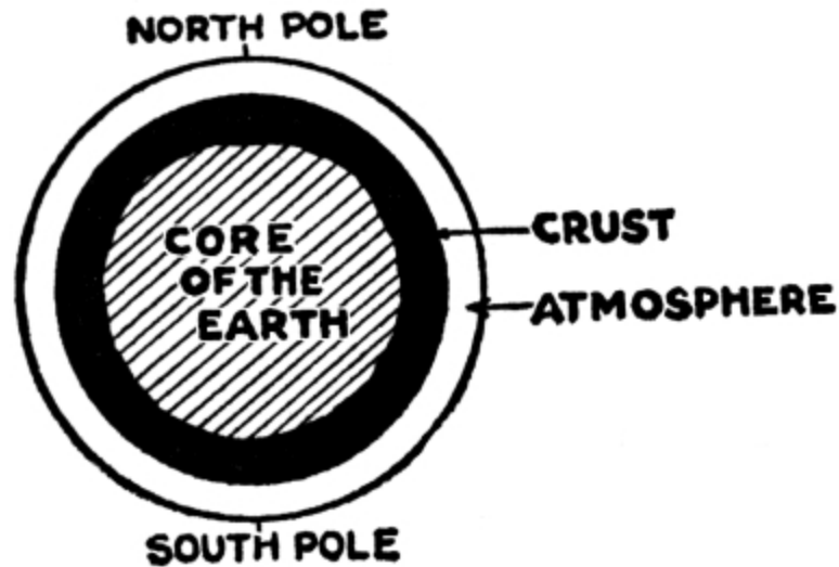
FIG. 70.—CROSS SECTION OF THE EARTH.
