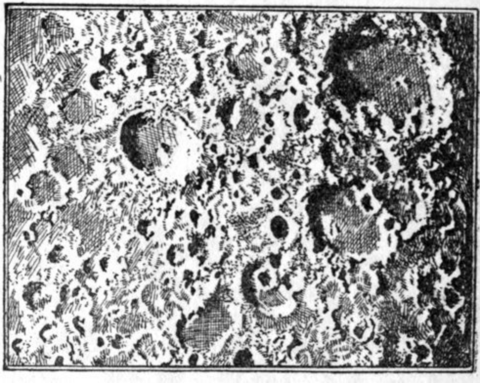
FIG. 105.—REAL VOLCANOES.
