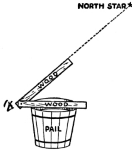
FIG. 97.—TWO STICKS ACROSS BUCKET OF WATER.
