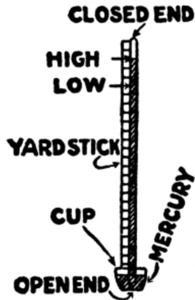
FIG. 36.—BAROMETER COMPLETE.
