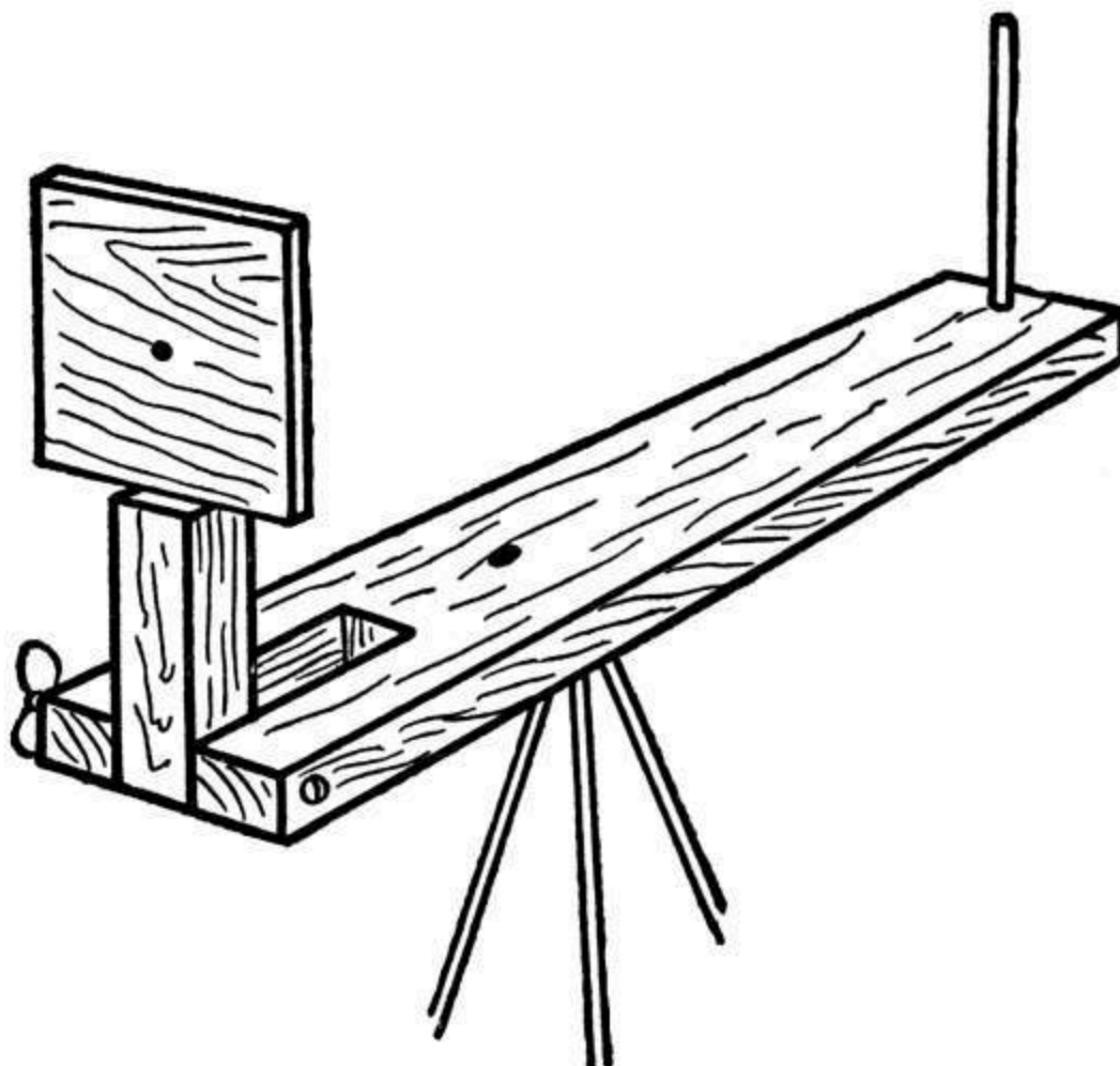
FIG. 44.—HELIOGRAPH COMPLETE.
