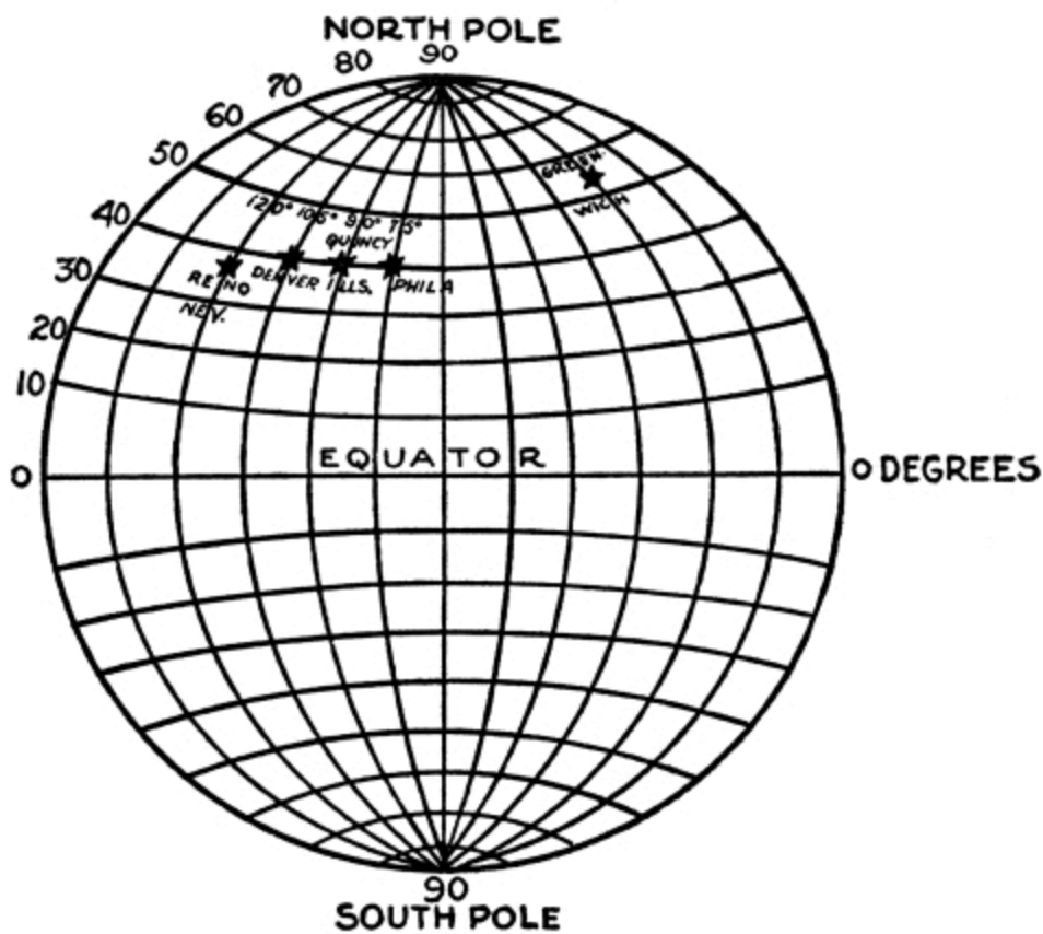
FIG. 94.—EARTH SURFACE DIVIDED INTO DEGREES.
