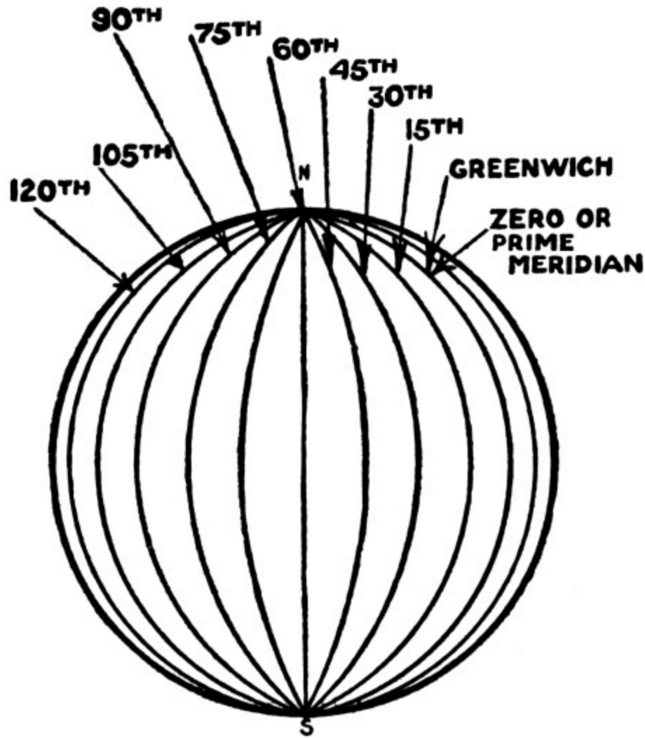
FIG. 164.—THE EARTH DIVIDED INTO 24 STANDARD MERIDIANS.
