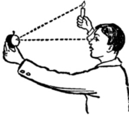
FIG. 141.—LIGHT REFLECTED BY AN APPLE.
