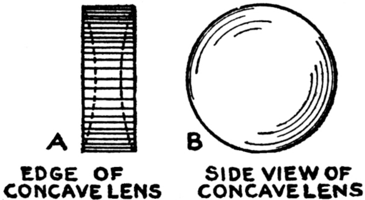
FIG. 147.—CONCAVE LENS.
