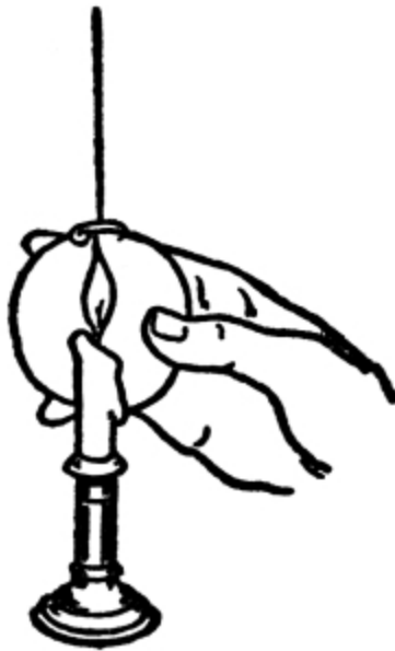
FIG. 83.—POSITION OF THE EARTH AND SUN IN SUMMER.
