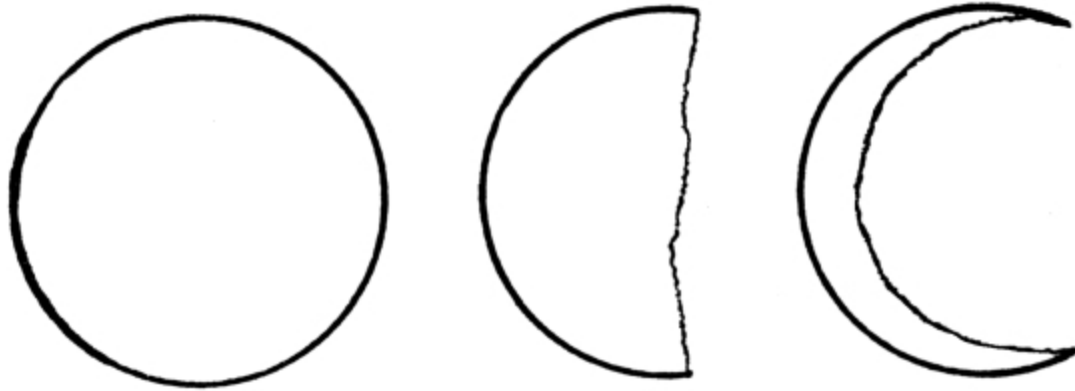
FIG. 54.—THREE VIEWS OF VENUS.
