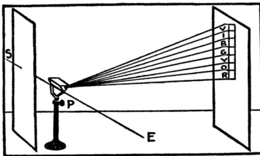
FIG. 145.—PRISM FORMING A SPECTRUM.
