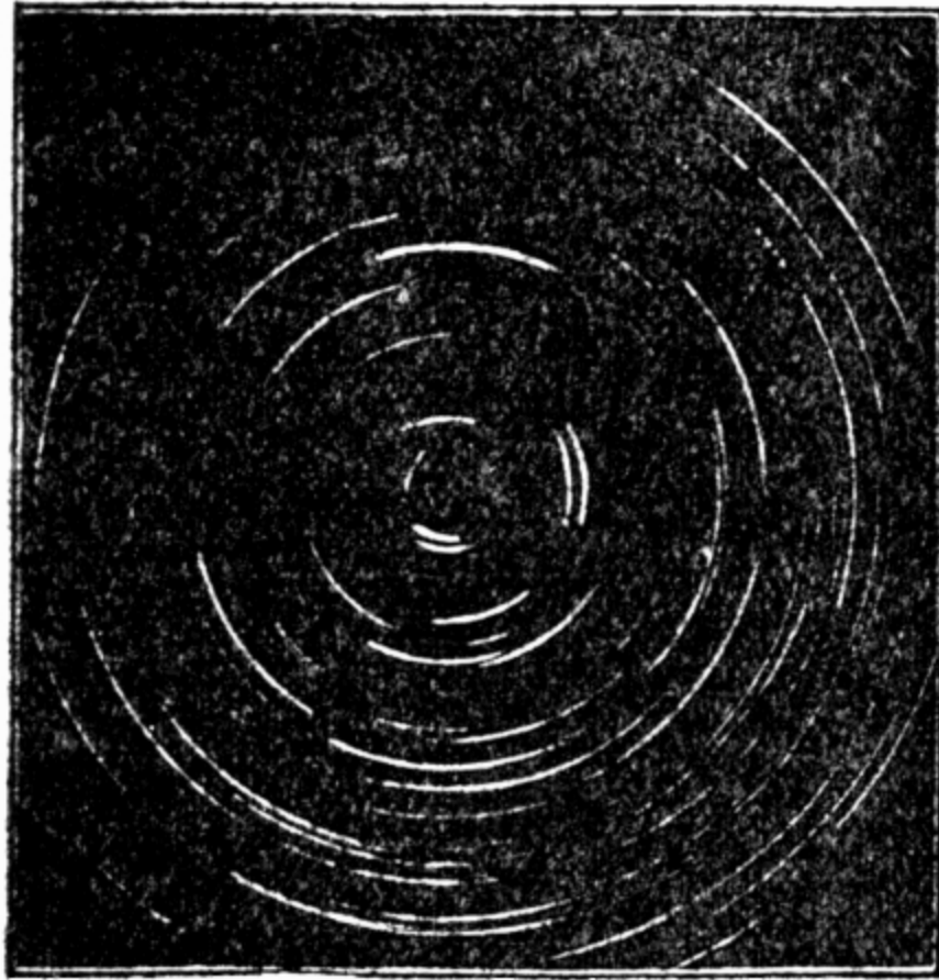
FIG. 181. STAR TRAILS.
