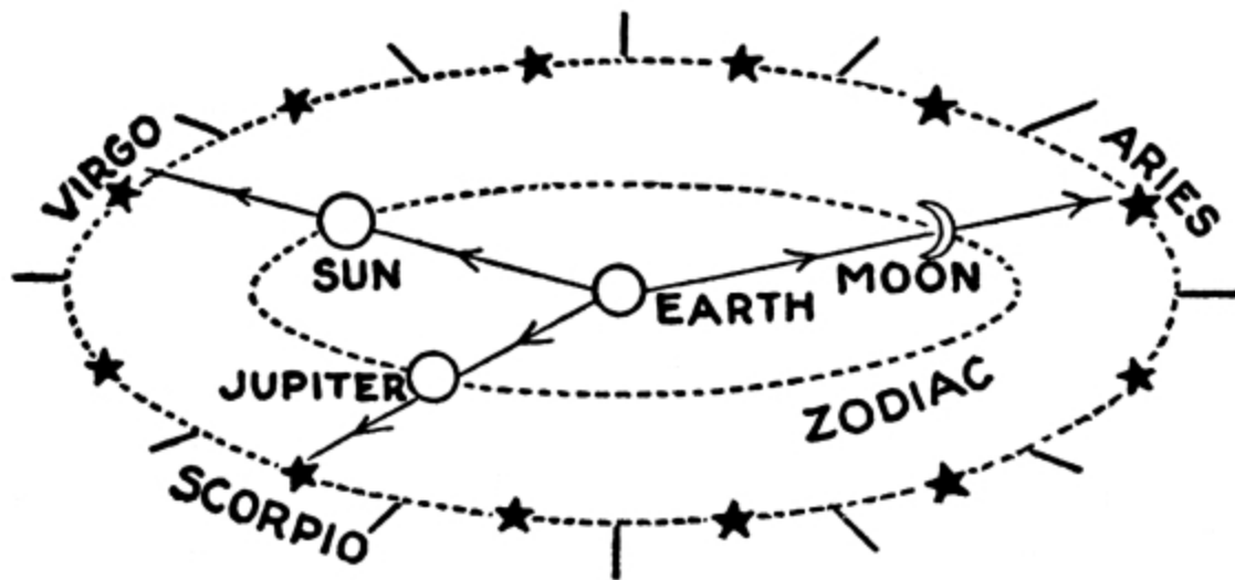
FIG. 170.—THE ZODIAC AS INVENTED BY THE ANCIENTS.
