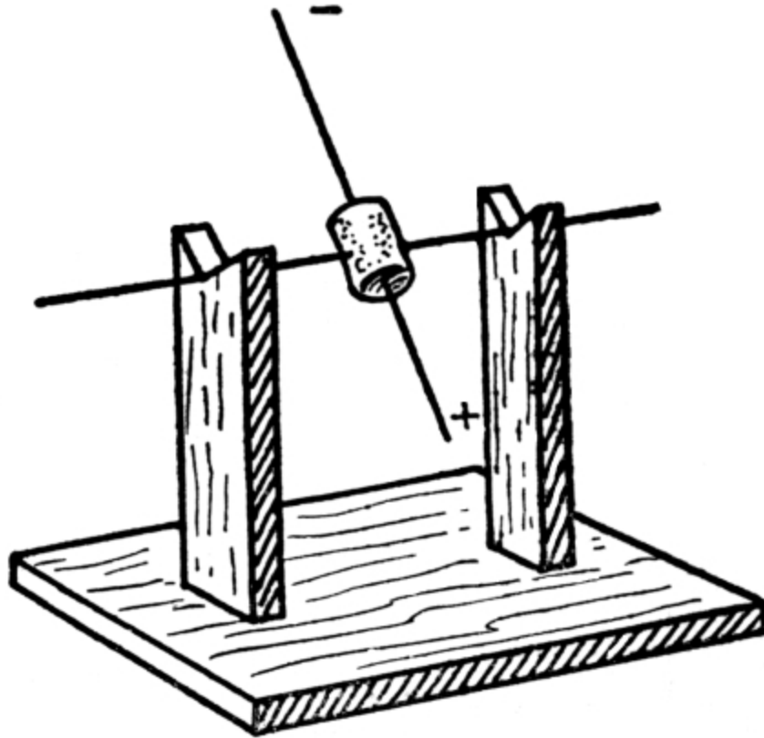
FIG. 92.—DIPPING NEEDLE COMPLETE.
