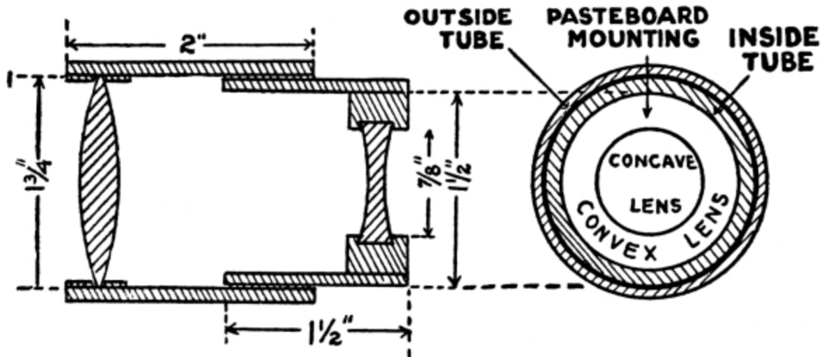
FIG. 155.—OPERA GLASS TELESCOPE. CROSS SECTION.
