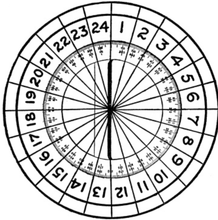
FIG. 163.—CIRCLE DIVIDED INTO 360 DEGREES AND 24 HOURS.
