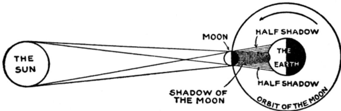
FIG. 123.—THE SUN ECLIPSED BY THE MOON (DIAGRAM).
