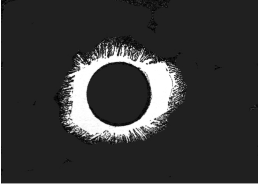
FIG. 125.—TOTAL ECLIPSE OF THE SUN, FROM PHOTO.
