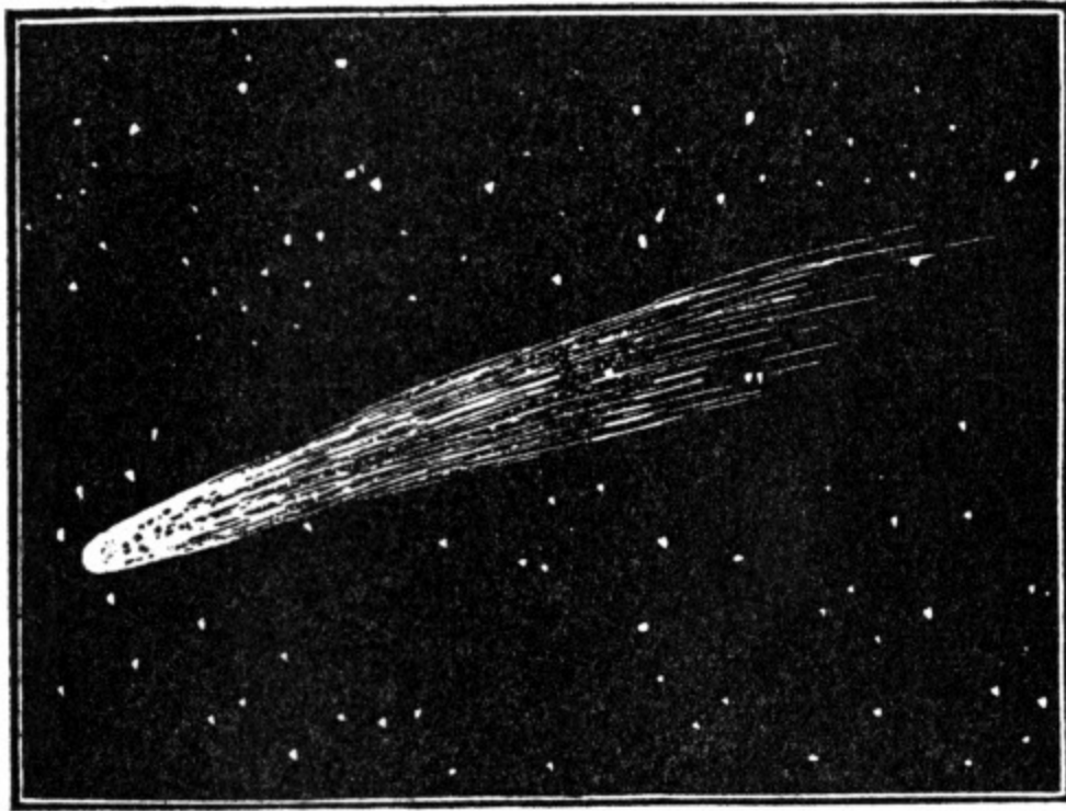
FIG. 131.—HALLEY'S COMET, FROM PHOTO.
