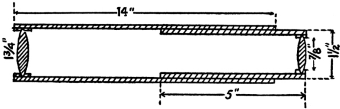
FIG. 156.—TELESCOPE. CROSS SECTION VIEW.
