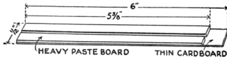
FIG. 153.—PASTEBOARD MOUNTING OF LENS.
