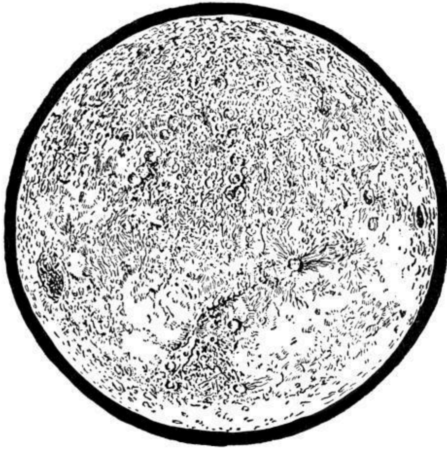
FIG. 158.—FULL VIEW OF MOON.
