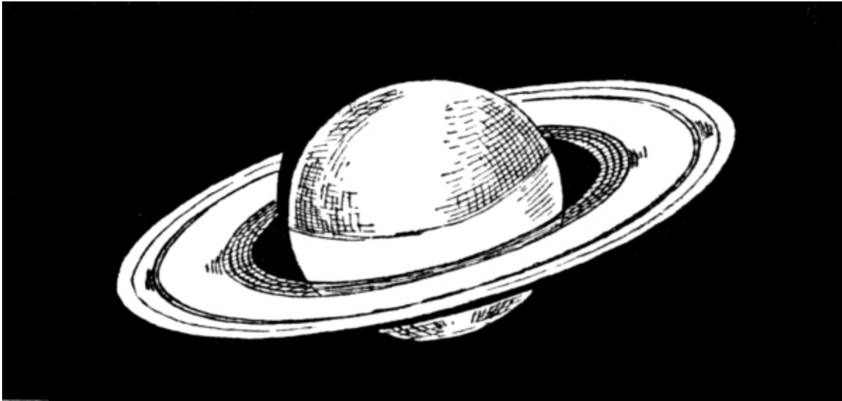
FIG. 57.—SATURN.
