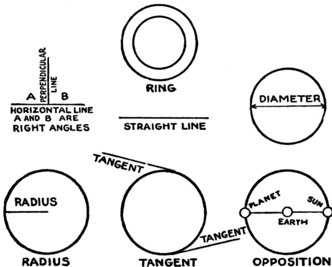
FIG. 185.—GEOMETRICAL FIGURES.
