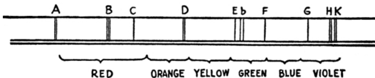
FIG. 183.—FRAUNHOFER'S LINES.
