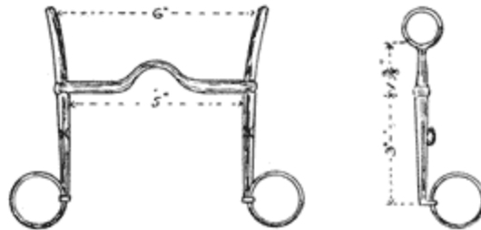
Fig. 39.—Properly constructed Curb for ordinary Hunter. Side View.
