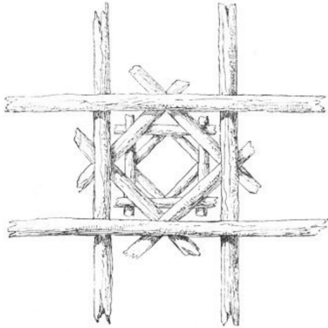
FIG. 61.—Armenian "Lantern;" from Botta.
