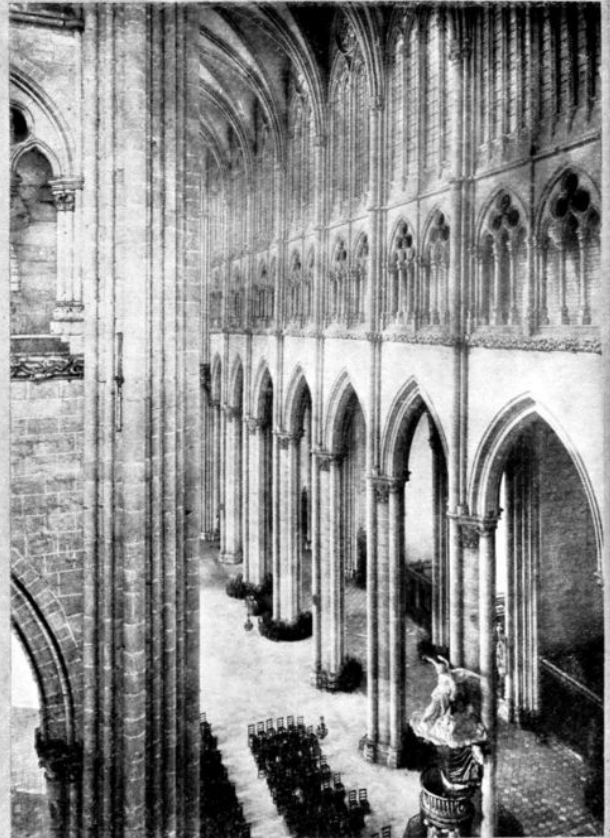
Amiens Cathedral - Kattenrath's photo.
