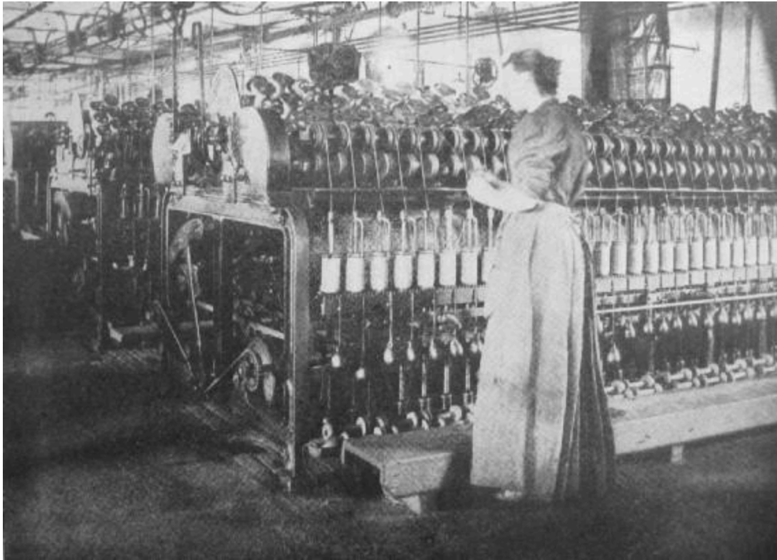
DRAWING FRAME Drawing the Roving Finer.
