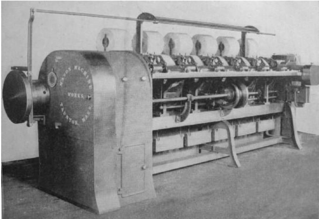
COTTON COMB, USED FOR LONG STAPLE
