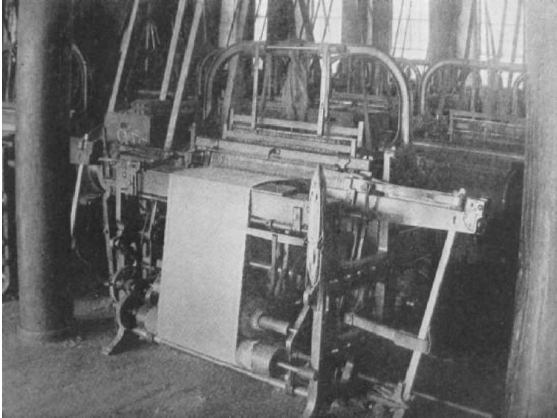
A PLAIN POWER LOOM WEAVING LINEN
