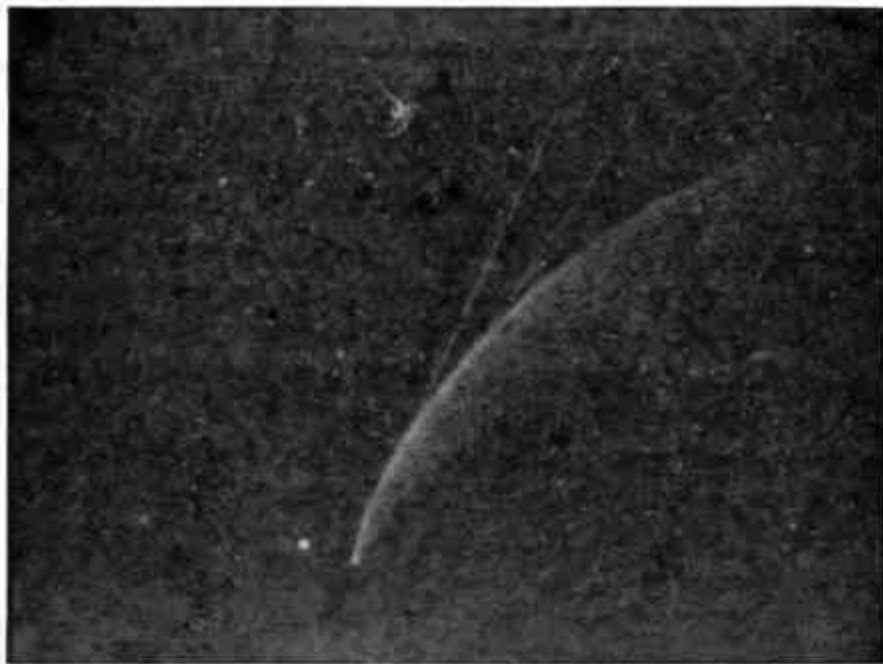
FIG. 49.—Great Comet of 1858.
