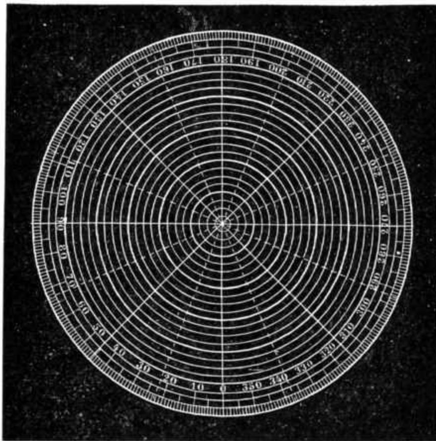
FIG. 81.—Division of the Circumference into 360 degrees.
