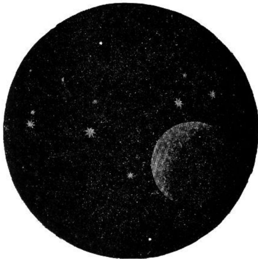
FIG. 26.—Occultation of the Pleiades by the Moon.
