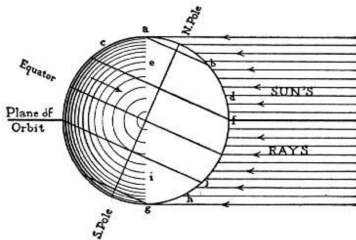
FIG. 61.—Inclination of the Earth.
