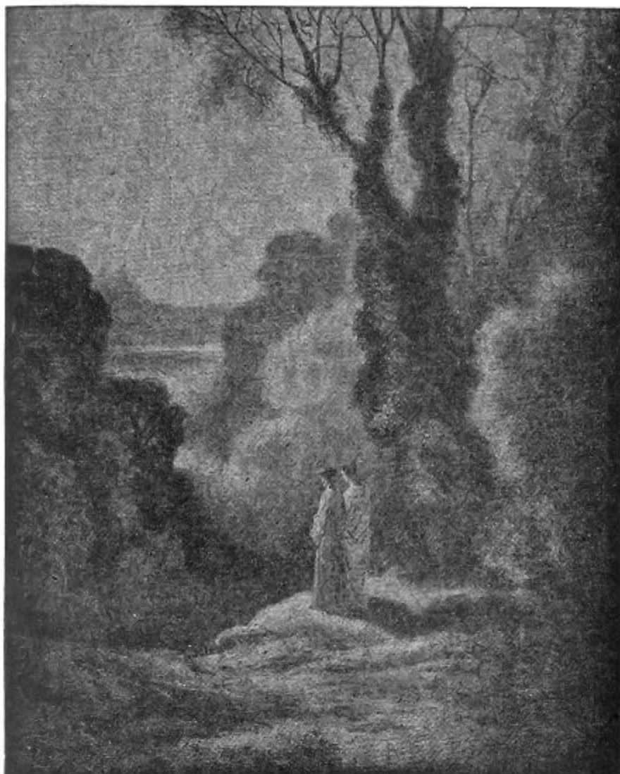
FIG. 36.—The Evening Star.
