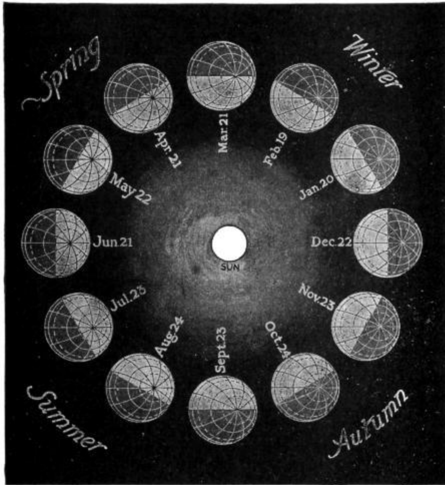
FIG. 60.—Motion of the Earth round the Sun.
