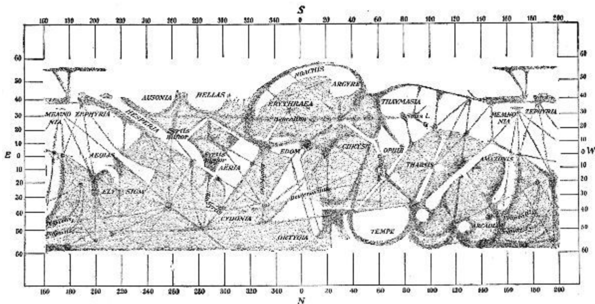
FIG. 43.—Chart of Mars.
