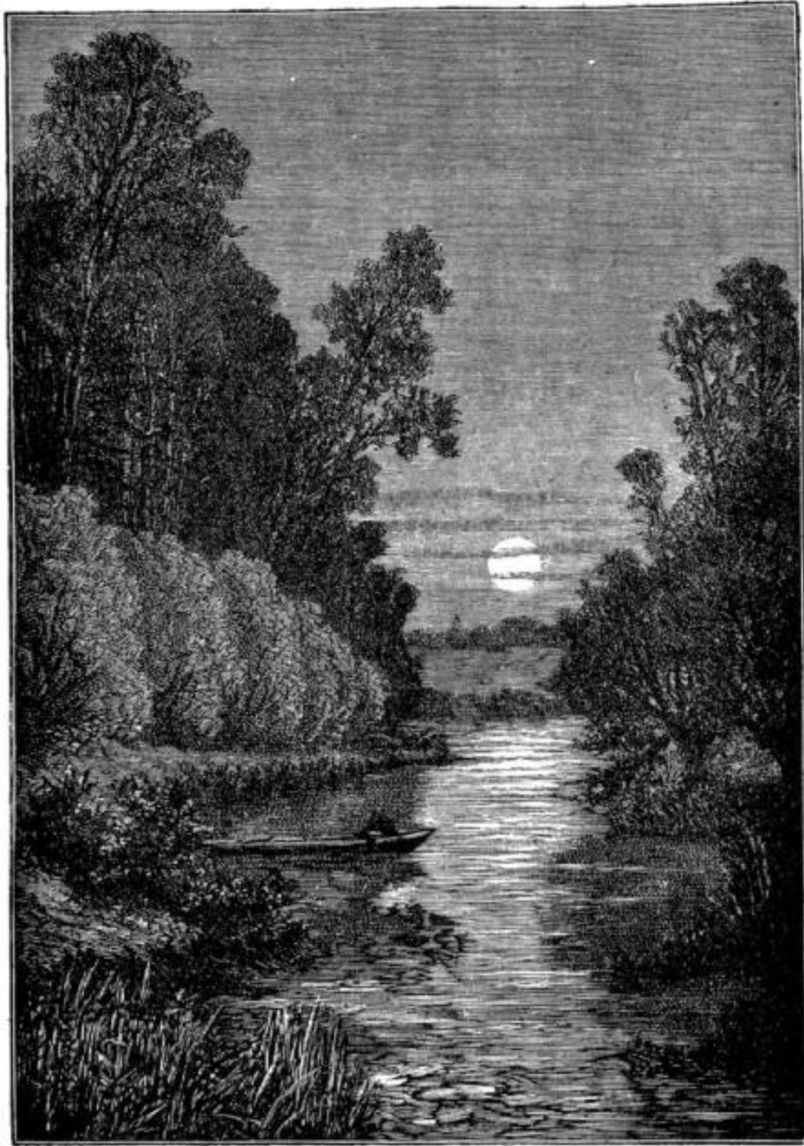
FIG. 64.—The Full Moon slowly rises.
