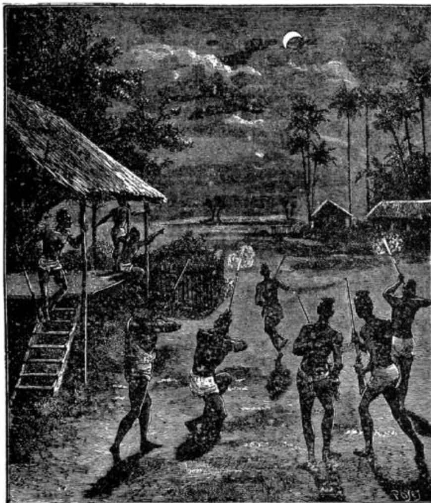
FIG. 76.—Eclipse of the Moon at Laos (February 27, 1877).
