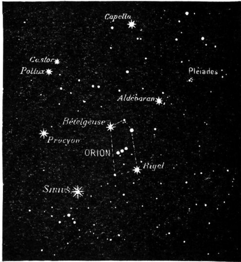
FIG. 12.—Orion and his celestial companions.
