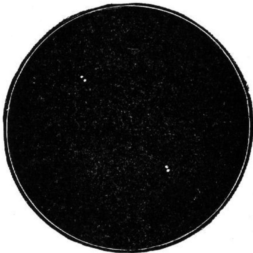
FIG. 19.—Quadruple star \epsilon of the Lyre.
