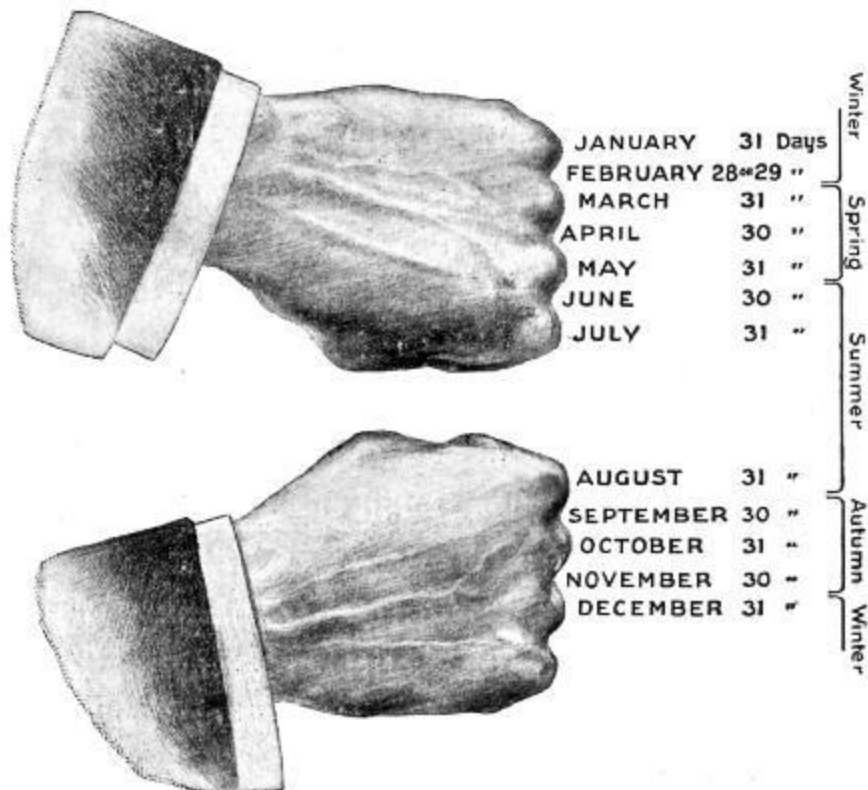
FIG. 63.—To find the long and short months.
