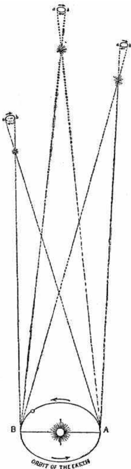
FIG. 84.—Small apparent ellipses
