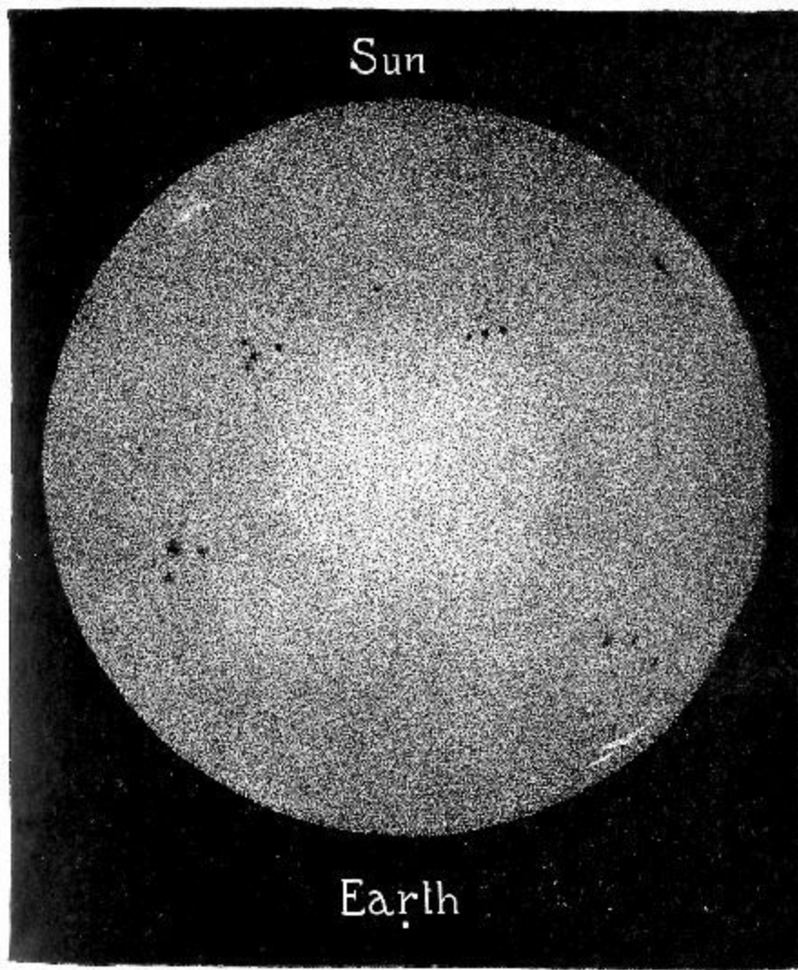
FIG. 28.—Comparative sizes of the Sun and Earth.
