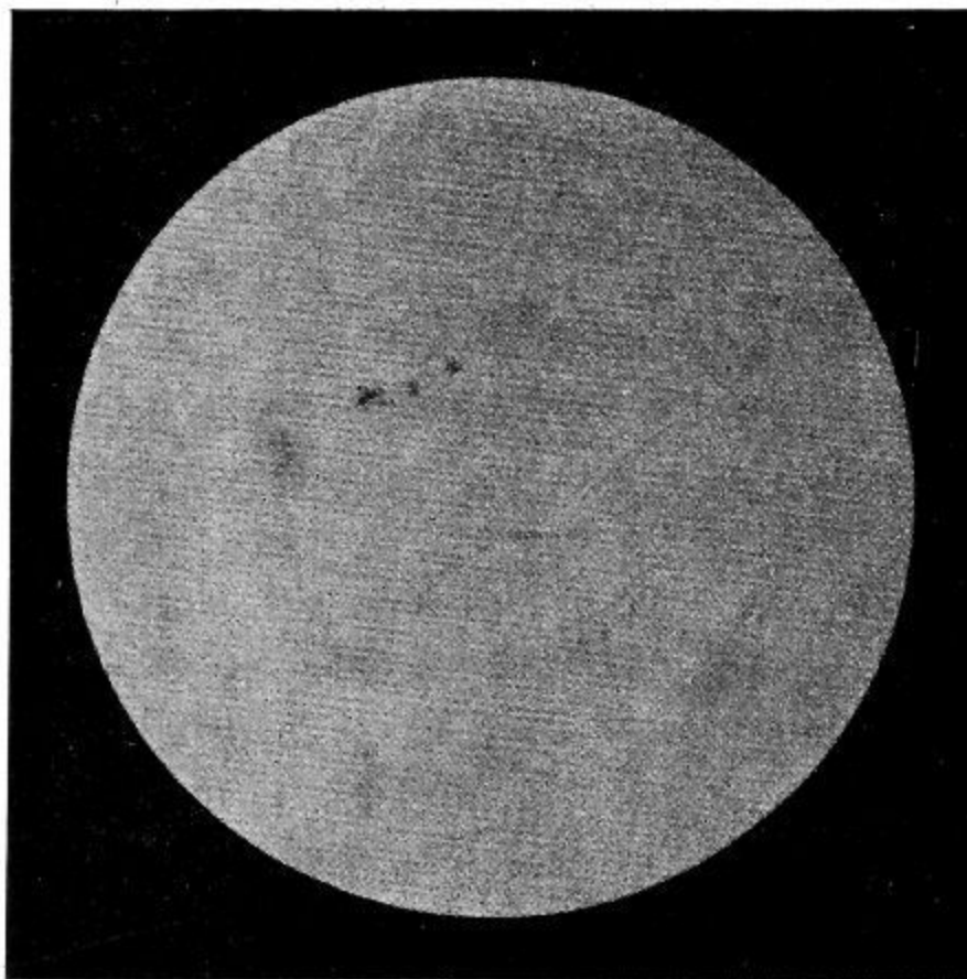
FIG. 29.—Direct photograph of the Sun.
