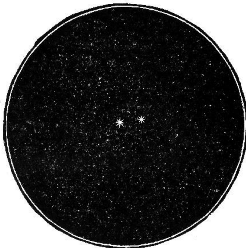
FIG. 17.—The double star Mizar.
