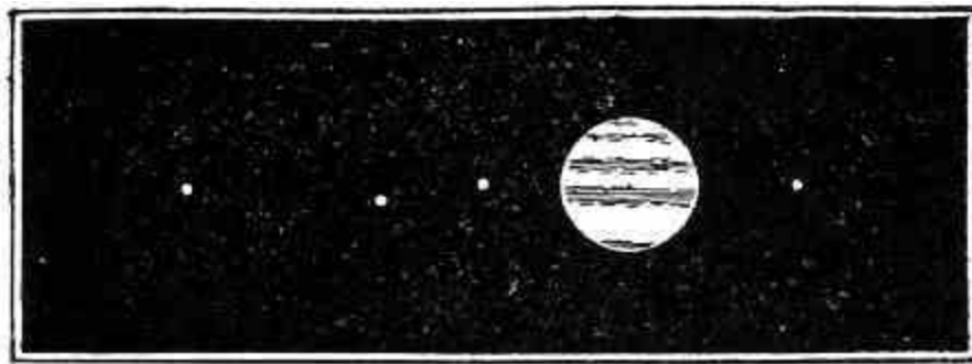
FIG. 46.—Jupiter and his four principal satellites.
