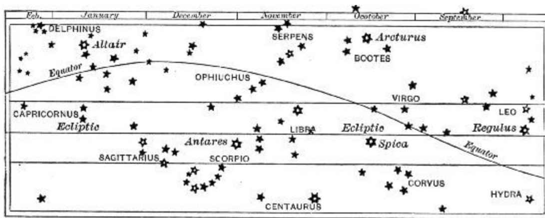
FIG. 10.—The Constellations of the Zodiac: summer and autumn; Capricorn, Archer, Scorpion, Balance, Virgin, Lion.
