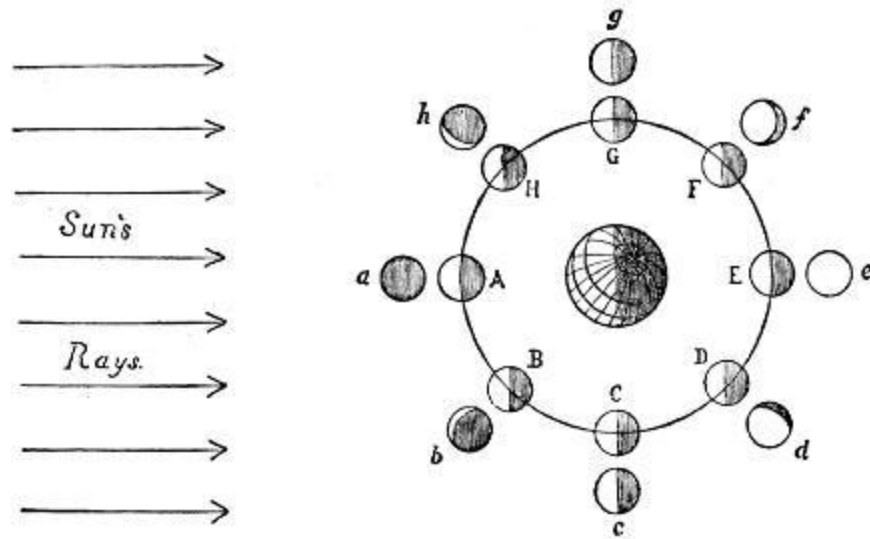
FIG. 70.—The Moon's Phases.
