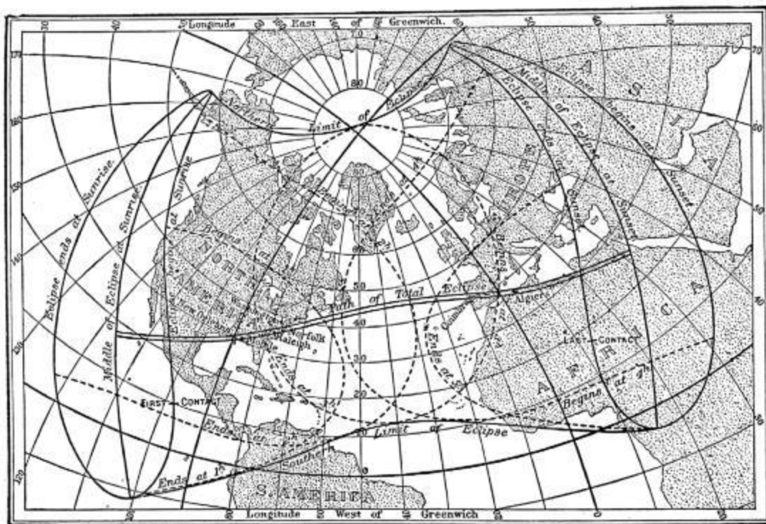
FIG. 77.—The path of the Eclipse of May 28, 1900.
