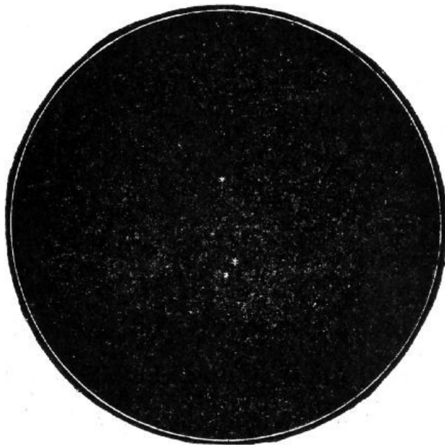
FIG. 18.—Triple star \zeta in Cancer.
