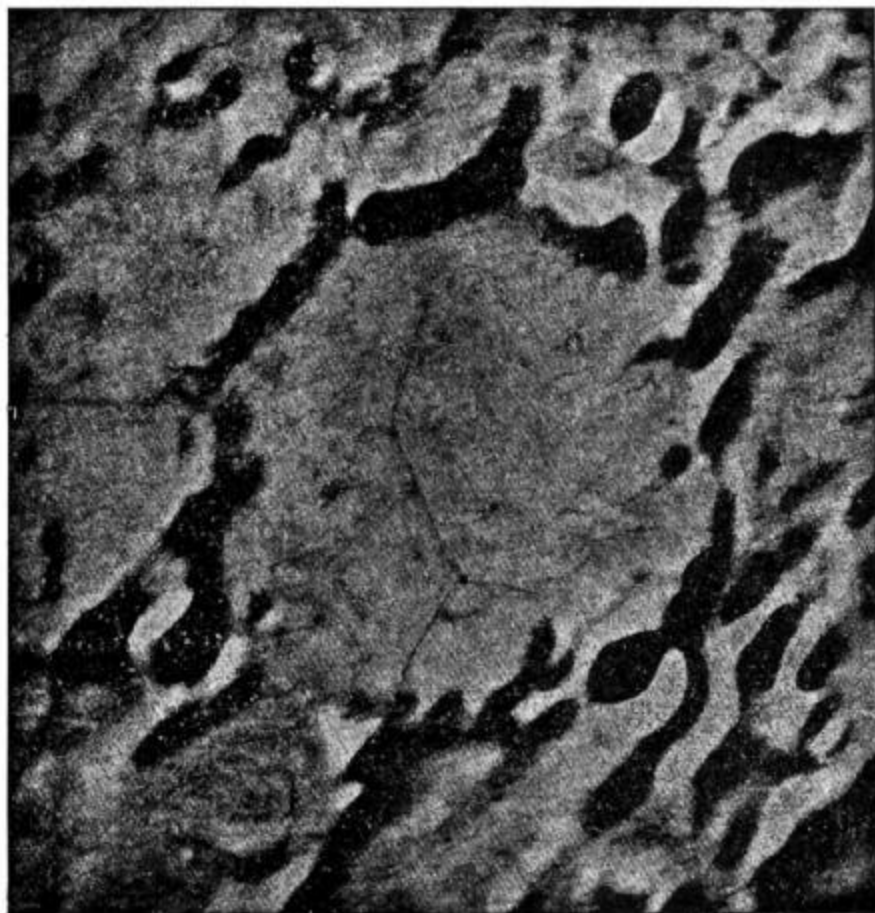
FIG. 73.—Flammarion's Lunar Ring.
