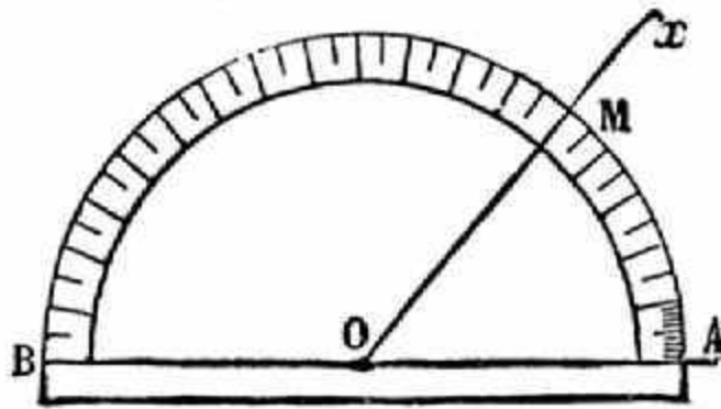
FIG. 80.—Measurement of Angles.
