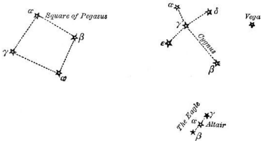
FIG. 9.—The Swan, Vega, the Eagle.
