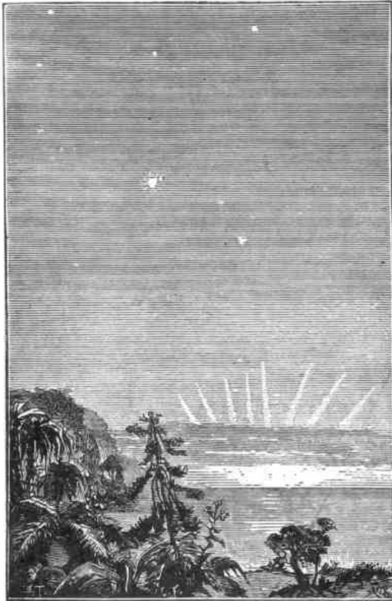
FIG. 44.—The Earth viewed from Mars.
