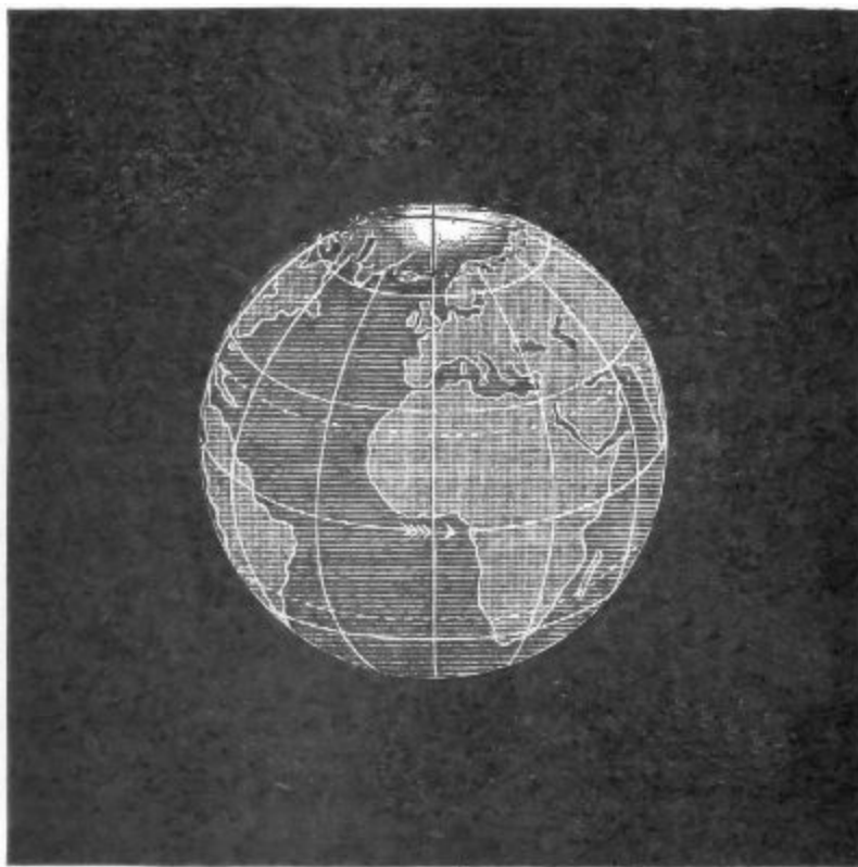
FIG. 2.—The earth in space. June solstice, midday.
