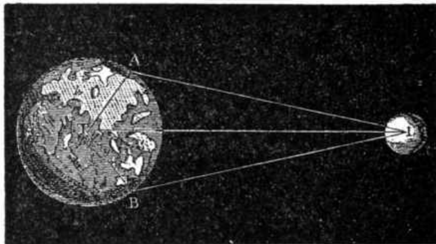
FIG. 82.—Measurement of the distance of the Moon.
