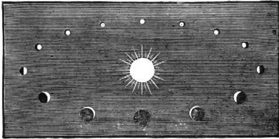
FIG. 37.—Successive phases of Venus.
