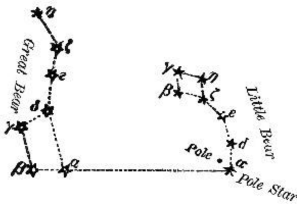
FIG. 4.—To find the Pole-Star.
