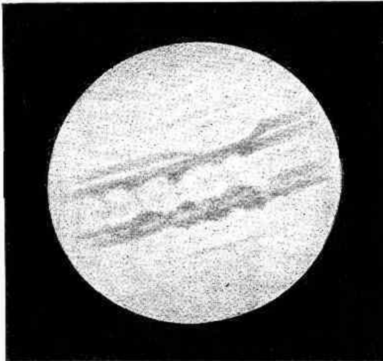
FIG. 45.—Telescopic aspect of Jupiter.
