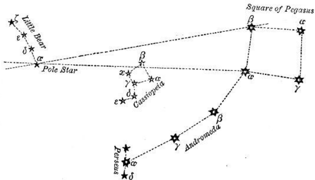
FIG. 6.—To Find Pegasus and Andromeda.
