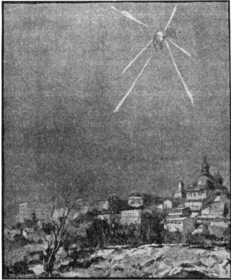
FIG. 57.—Explosion of a Fire-Ball above Madrid, February 10, 1896.
