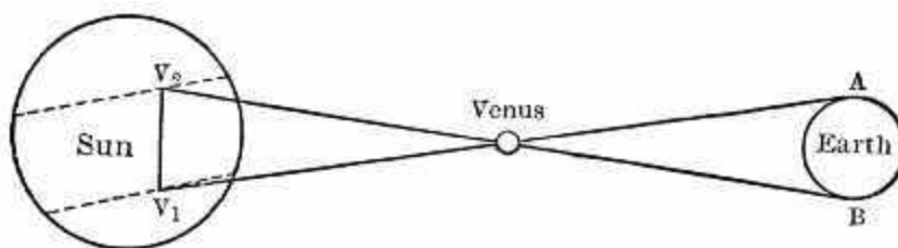
FIG. 83.—Measurement of the distance of the Sun.
