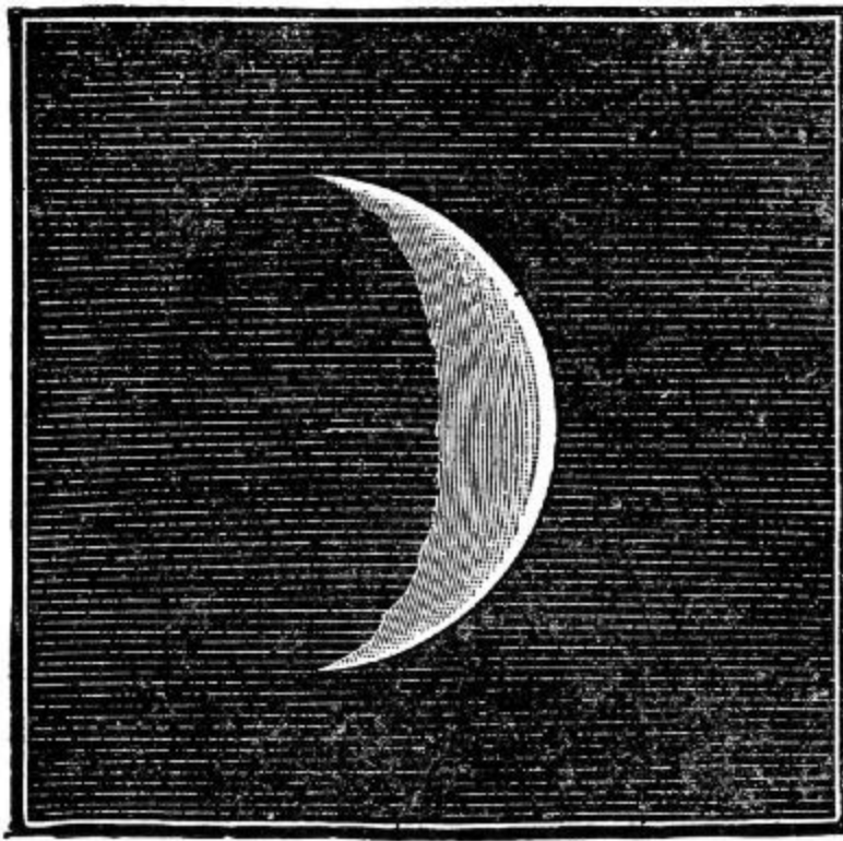
FIG. 38.—Venus at greatest brilliancy.
