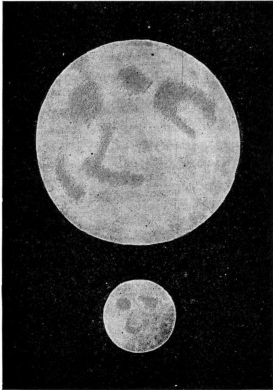
FIG. 65.—The Moon viewed with the unaided eye.
