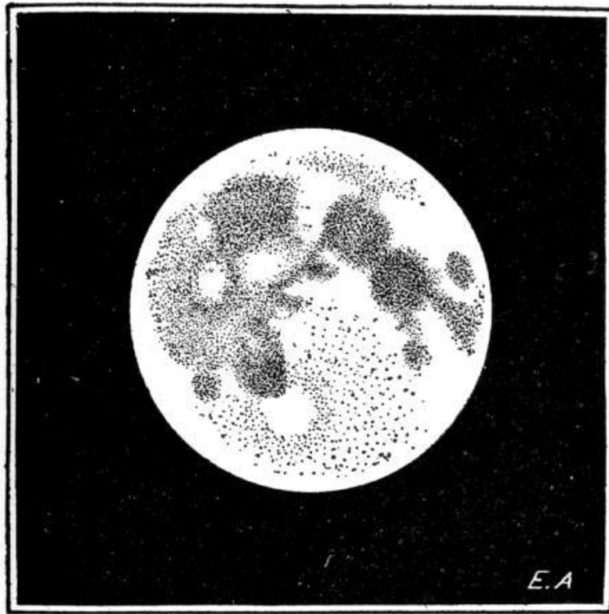
FIG. 66.—The Man's head in the Moon.
