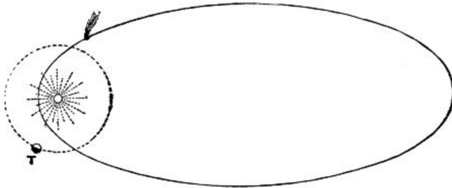
FIG. 52.—The orbit of a Periodic Comet.
