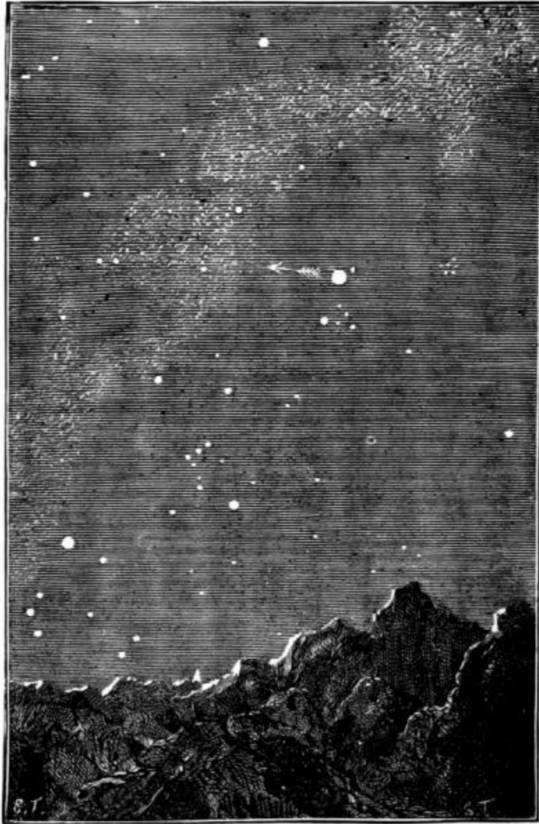
FIG. 35.—The Earth viewed from Mercury.
