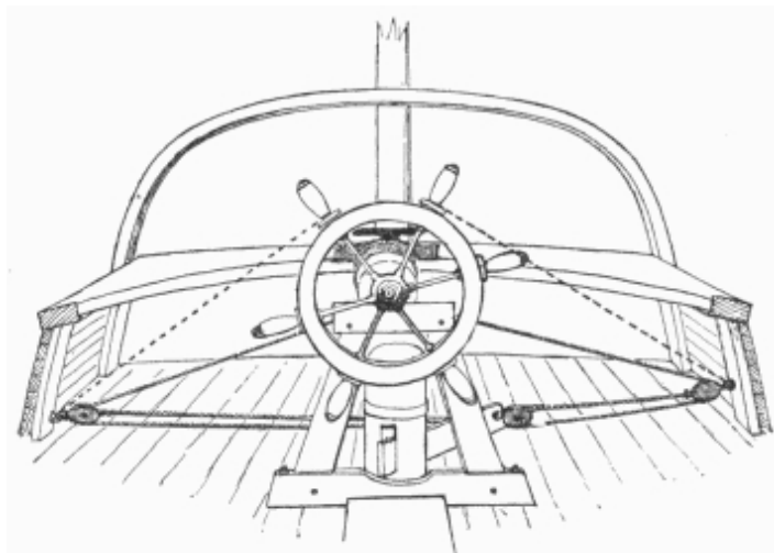
Steering-gear of the Spray . The dotted lines are the ropes used to lash the wheel. In practice the loose ends were belayed, one over the other, around the top spokes of the wheel.
