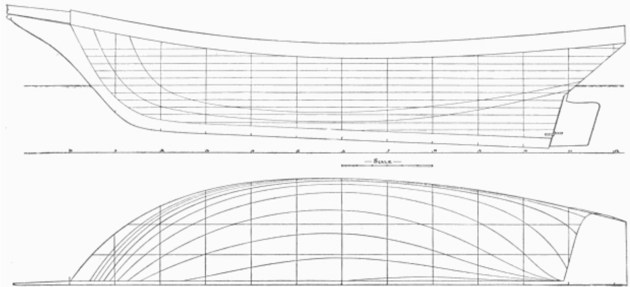
Lines of the Spray .
