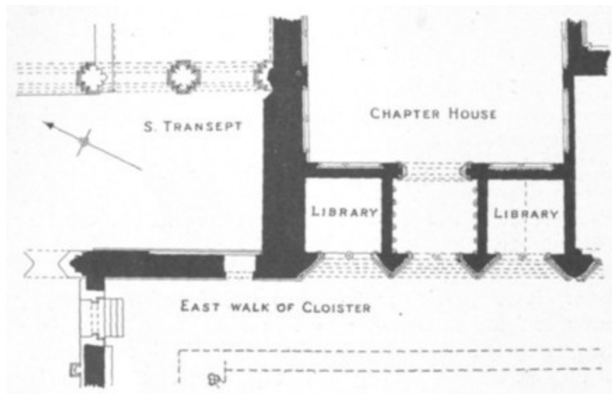
Fig. 23. Groundplan of part of Furness Abbey.
