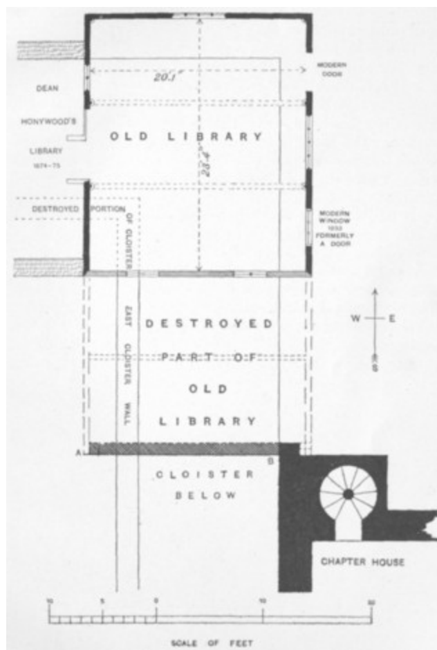
Fig. 38. Plan of the Old Library, Lincoln Cathedral.
