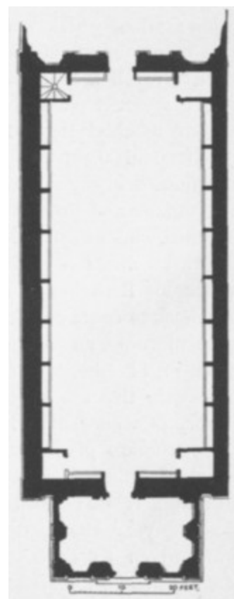
Fig. 120. Ground-plan of the Ambrosian Library at Milan. Reduced from that given by P. P. Boscha.
