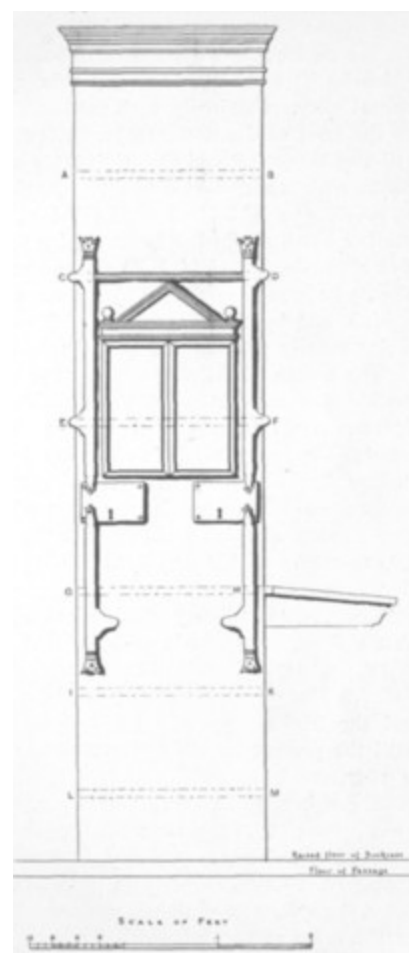
Fig. 71. Elevation of one bookcase in the Library of Corpus Christi College, Oxford.
