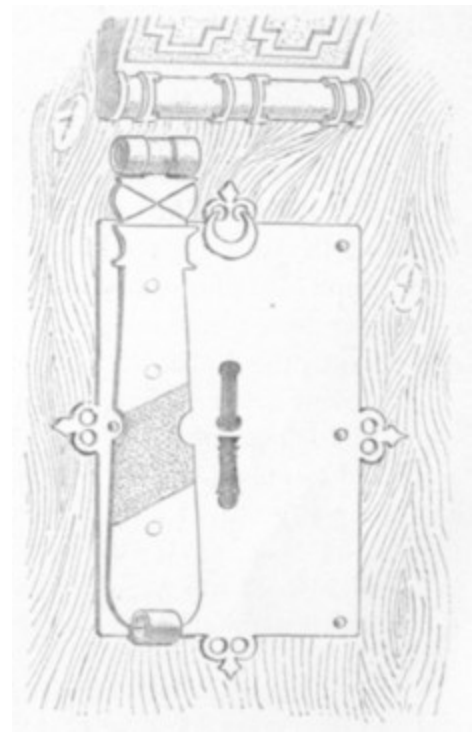
Fig. 67. Lock at end of book-desk. Trinity Hall.
