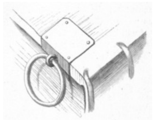
Fig. 86. Ring for attachment of chain, Wells.
