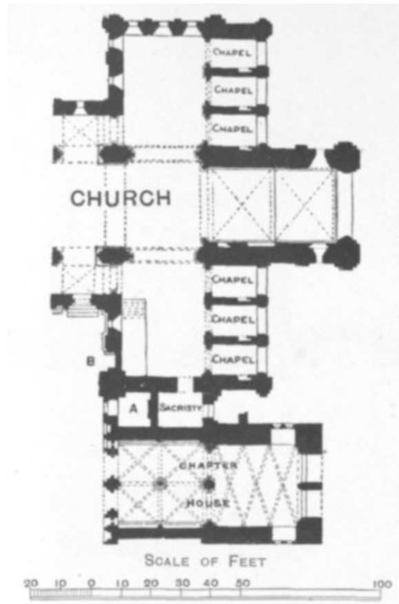
Fig. 22. Groundplan of part of Kirkstall Abbey, Yorkshire.
