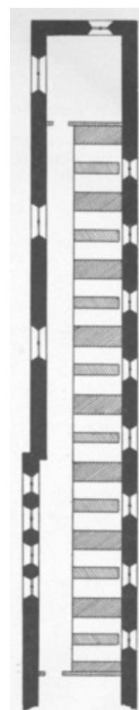
Fig. 42. Plan of the Library in Wells Cathedral. Scale 1/10 inch=1 foot.
