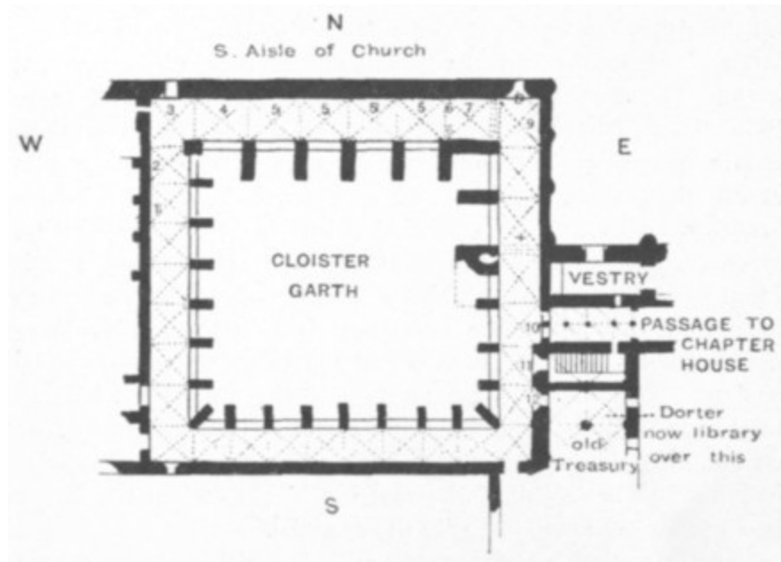
Fig. 25. The cloister, Westminster Abbey. From Mr Micklethwaite's plan of the buildings.
