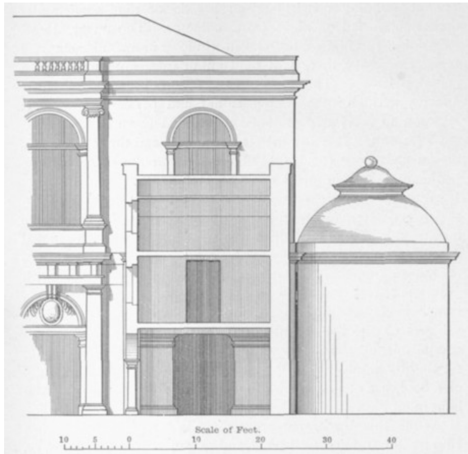
Fig. 126. Part of Wren's elevation of the east side of the Library of Trinity College, Cambridge, with a section of the north range of Neville's Court, shewing the door to the Library from the first floor.
