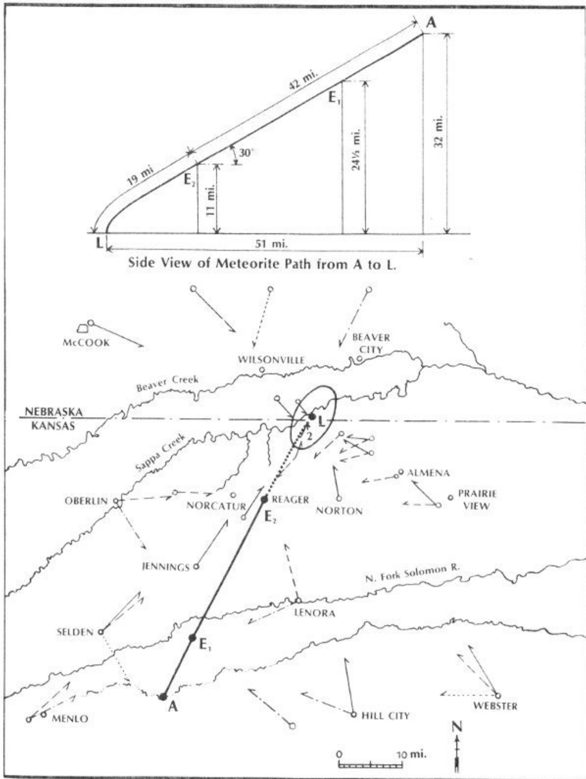
Path of the Norton meteorite.
