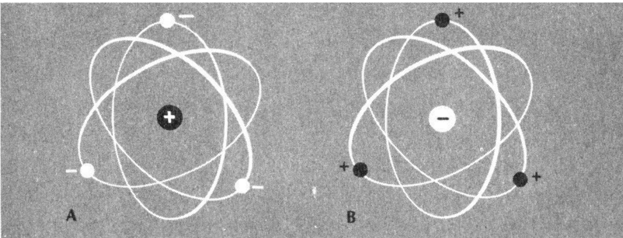
A. Representation of the structure of an atom of ordinary terrestrial matter. The nucleus is positively charged and around it circle negatively charged electrons.
