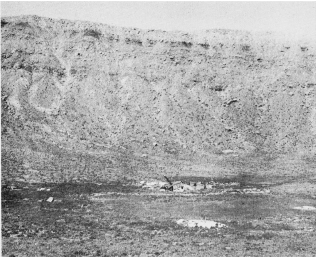
View of the interior of the Canyon Diablo crater showing the steep inner slopes of the huge basin.
