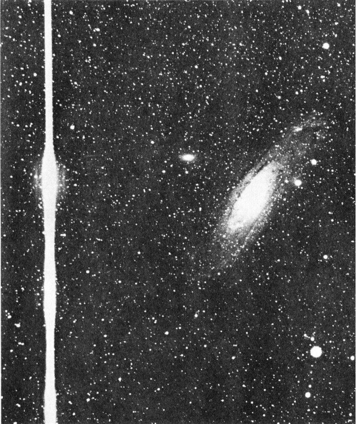
COURTESY OF AMERICAN MUSEUM OF NATURAL HISTORY Fireball speeding across field of camera during the photographing of the Great Spiral Nebula in Andromeda, by Josef Klepešta, at the Prague Observatory, Czechoslovakia, September 12, 1923.
