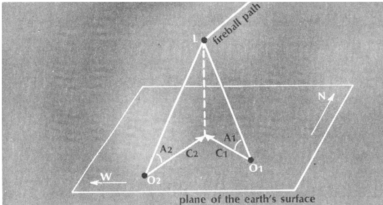
Method for locating a point on a fireball path. (In this case the point of disappearance, L.)
