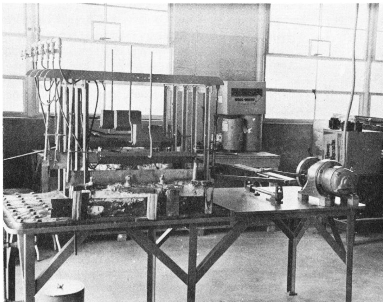
The 6-blade meteorite gang-saw in the machine shop at the Institute of Meteoritics.
