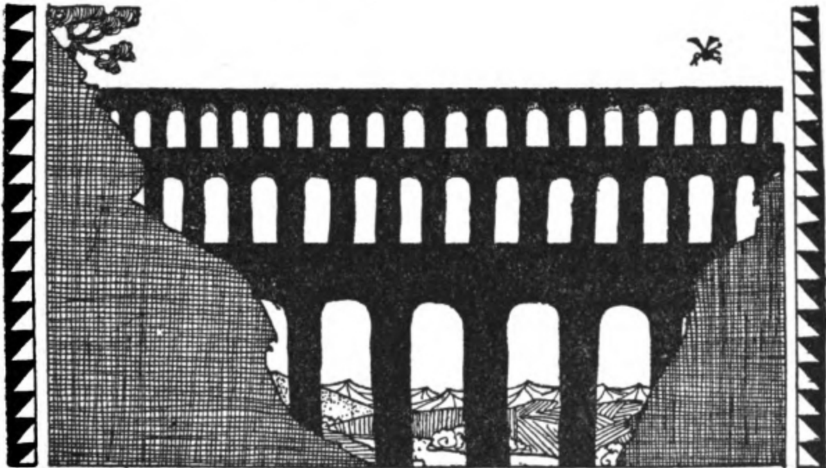
Roman Aqueduct.
