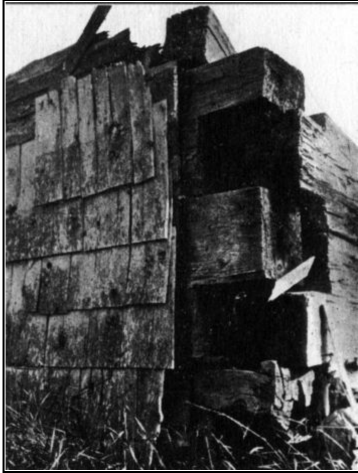
DOVETAILED LOGS AT THE CORNER OF THE BUNKER GARRISON HOUSE DURHAM, N. H. Built ca. 1690. From a photograph made in 1911
