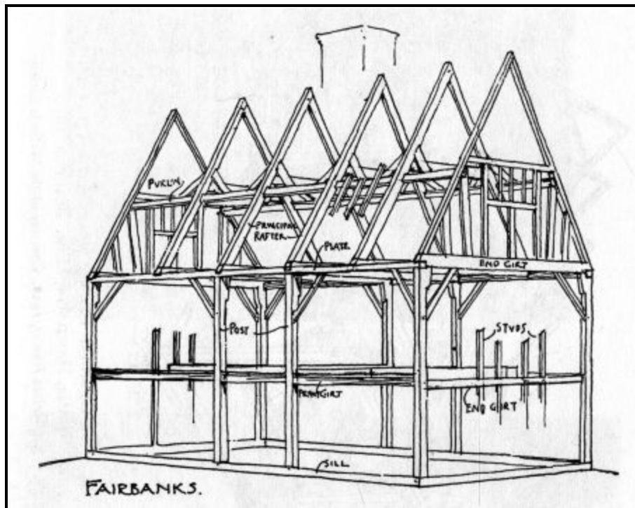
THE FRAME OF THE FAIRBANKS HOUSE
