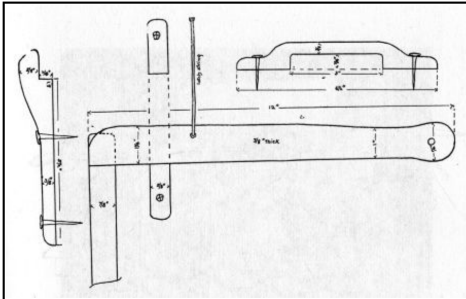
WOODEN LATCH OF ABOUT 1710
