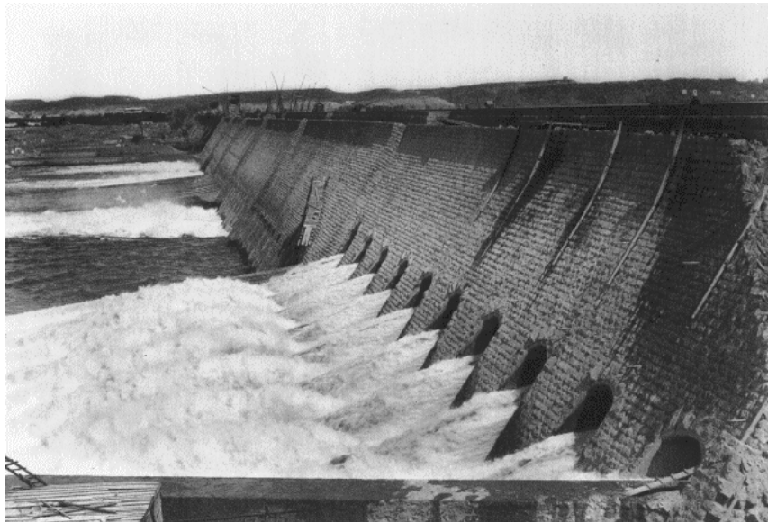
THE GREAT DAM, ASSOUAN, EGYPT
