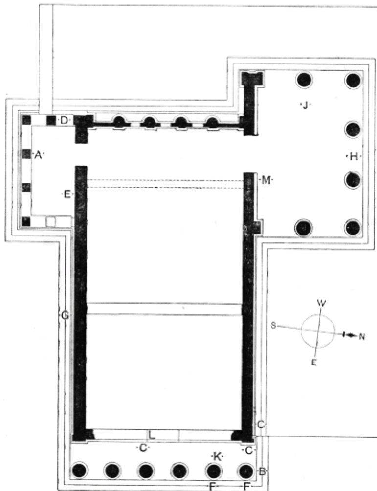
Fig. 18.—Ground Plan of the Erechtheion.
