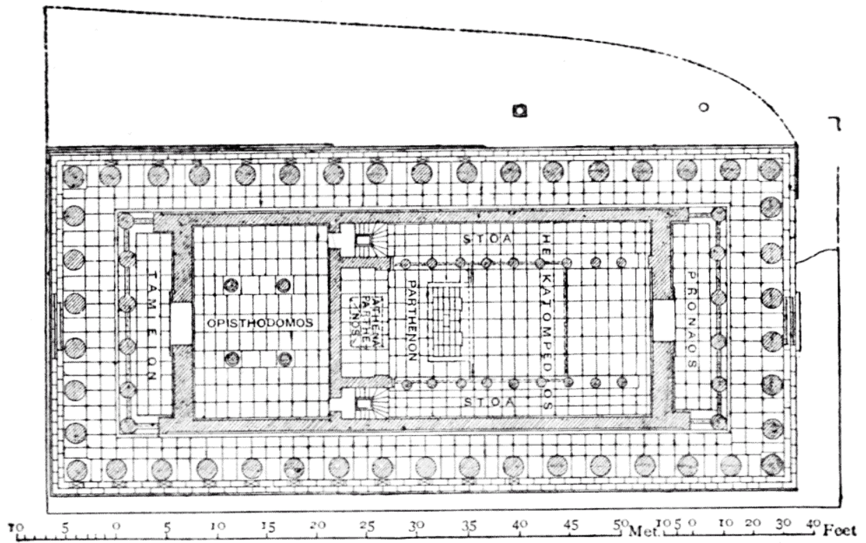
Fig. 6.—Plan of the Parthenon. (From Michaelis.)
