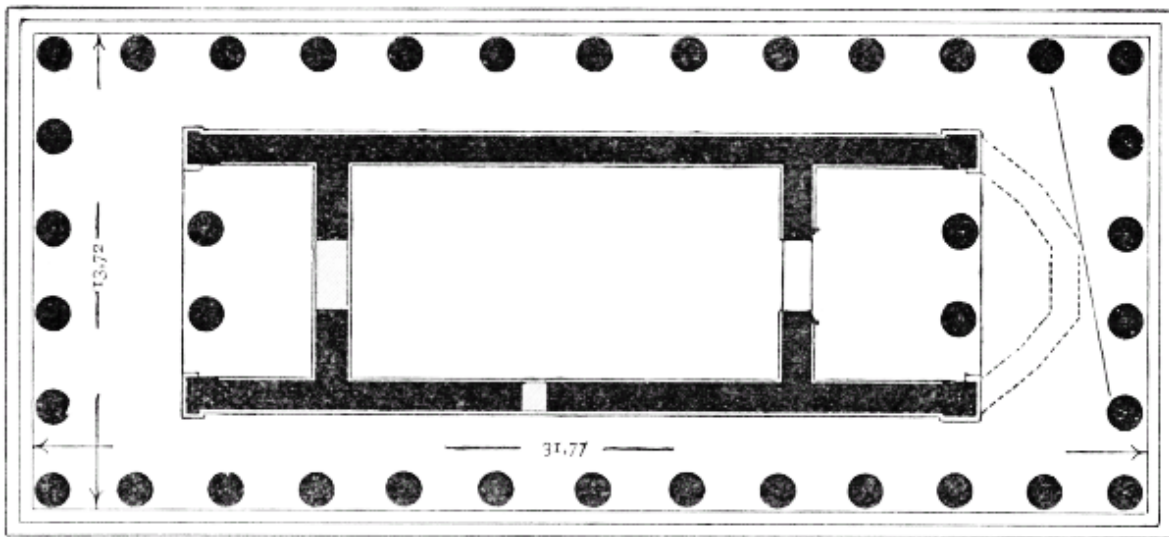
Fig. 15.—Plan of the Theseion. (From Baumeister.)
