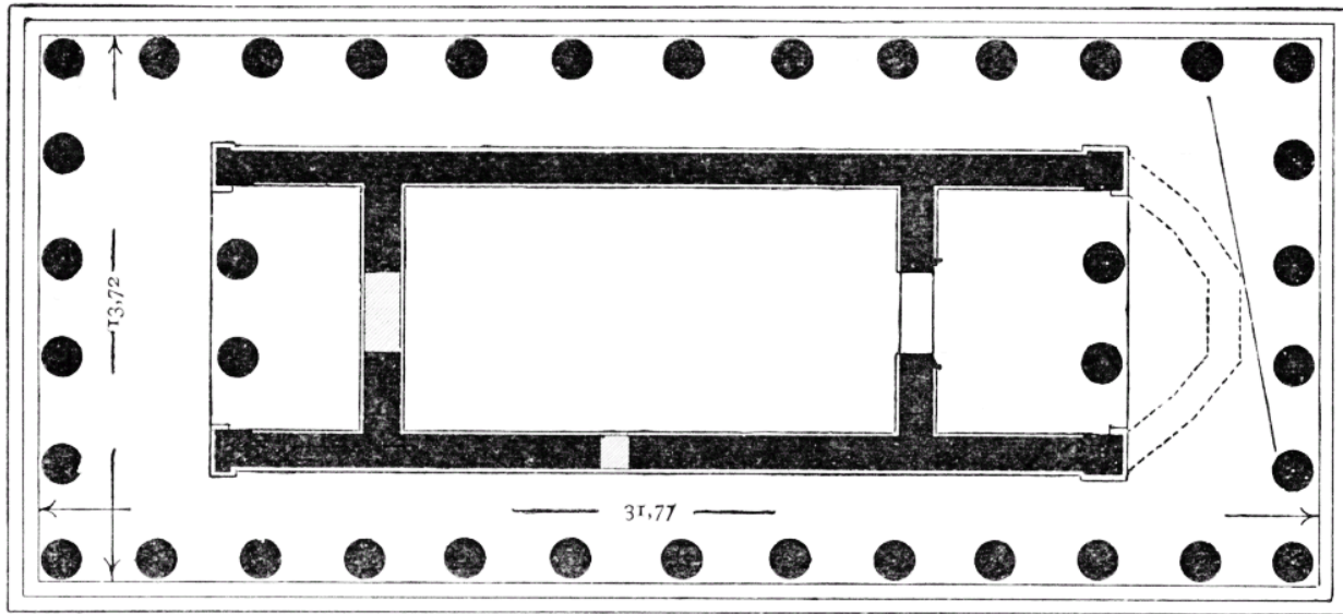
Fig. 15.— Plan of the Theseion. (From Baumeister.)
