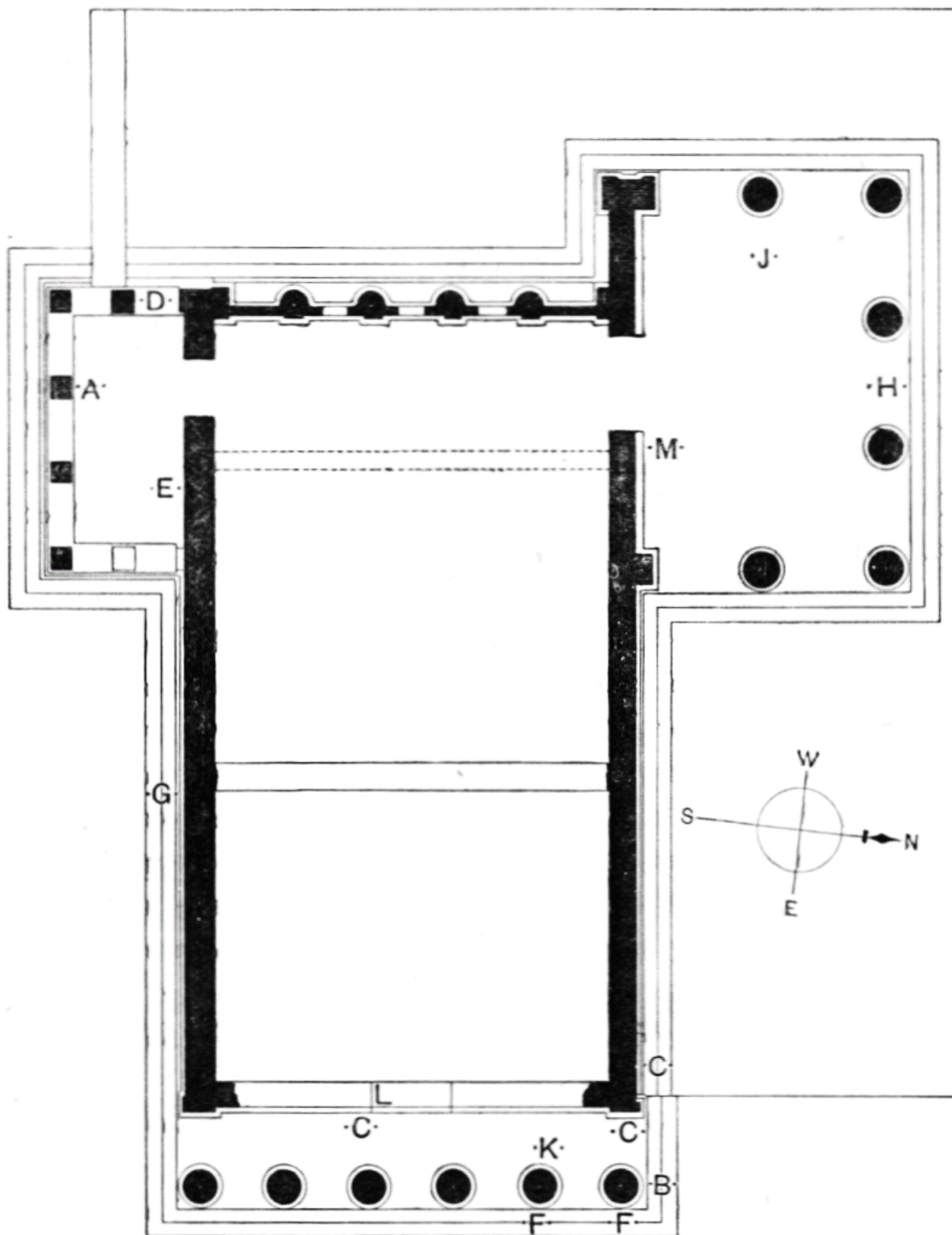
Fig. 18.—Ground Plan of the Erechtheion.
