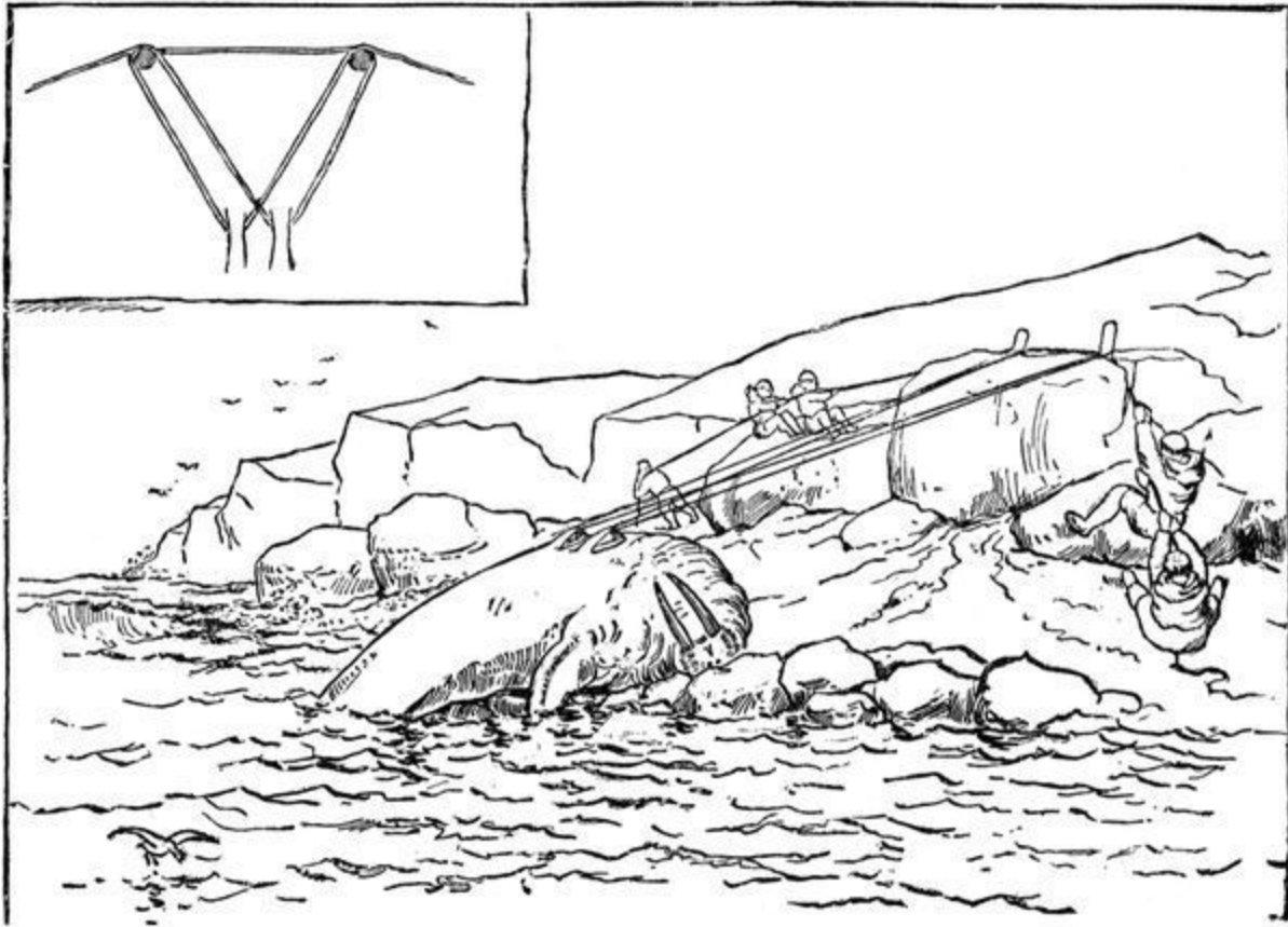
FIG. 58.—Principle of tackle utilised by Eskimo, landing a walrus. Above, on left, detail of the arrangement of the rope round stakes. (After Elliot.)
