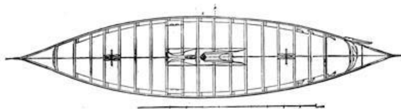
PLAN OF VIKING SHIP.
