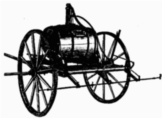
228. A truck-mounted barrel hand spray pump.
